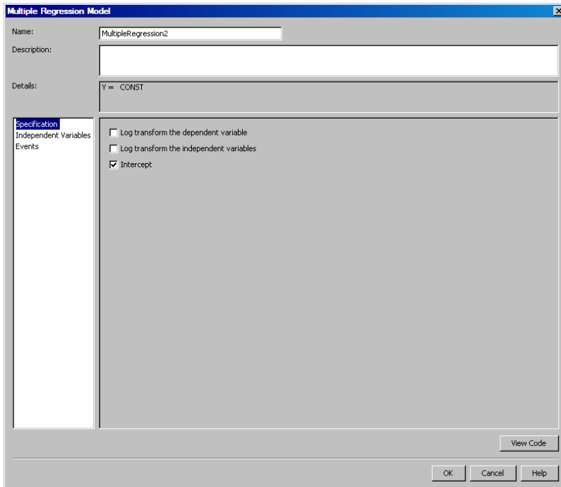
Display 17.6 Multiple Regression Model Dialog Box
