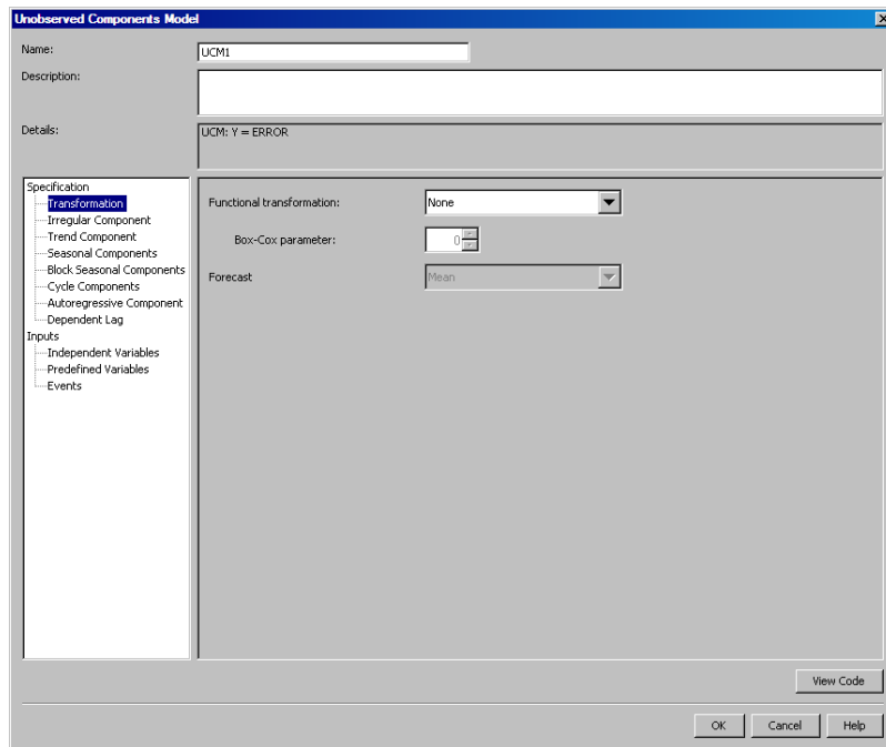
Display 17.3 Unobserved Components Model Dialog Box
