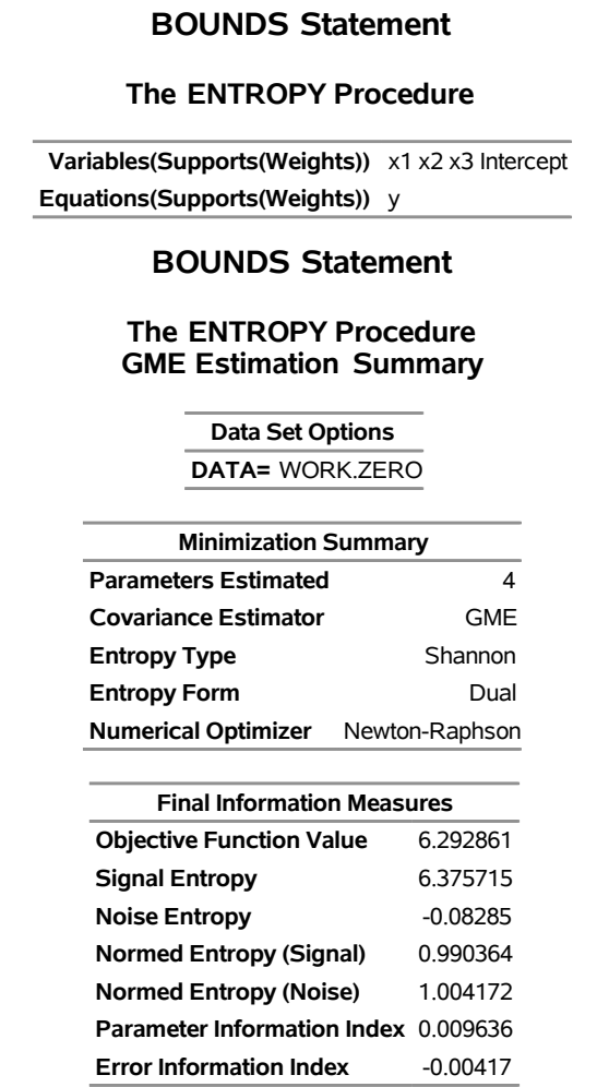
Figure 13.23 Output from Bounded Estimation
