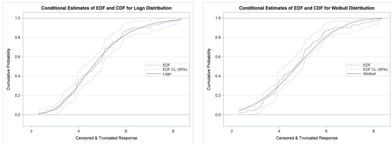
Figure 29.9 Comparing EDF and CDF Estimates for Lognormal and Weibull Models Fitted to Truncated and Censored Data
