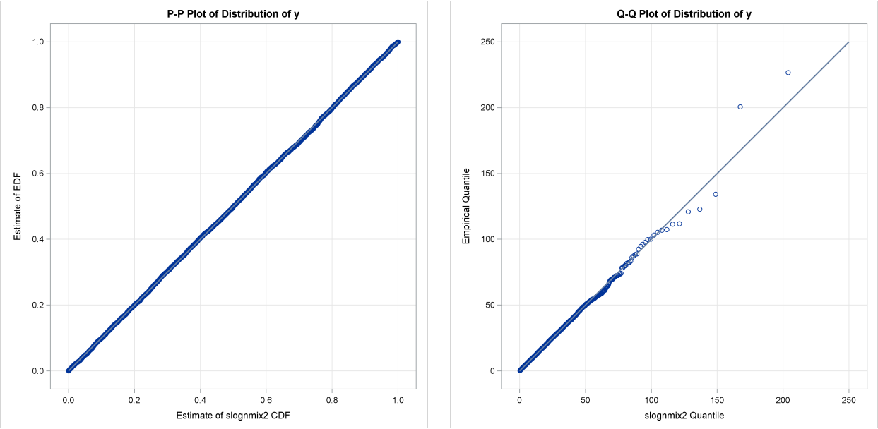
Output 29.7.3 P-P and Q-Q Plots to Evaluate SLOGNMIX2 Fit
