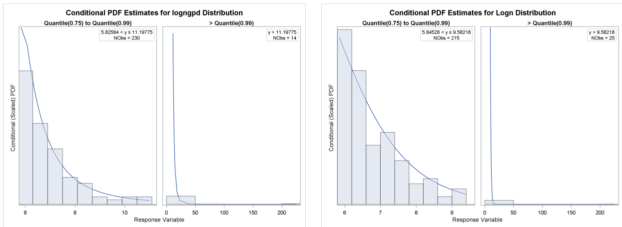
Output 29.4.5 Conditional PDF Plots for Right-Tail Regions of LOGNGPD (Left) and Lognormal (Right) Models
