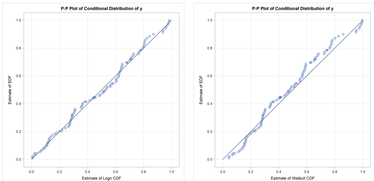
Figure 29.10 P-P Plots for Lognormal and Weibull Models Fitted to Truncated and Censored Data
