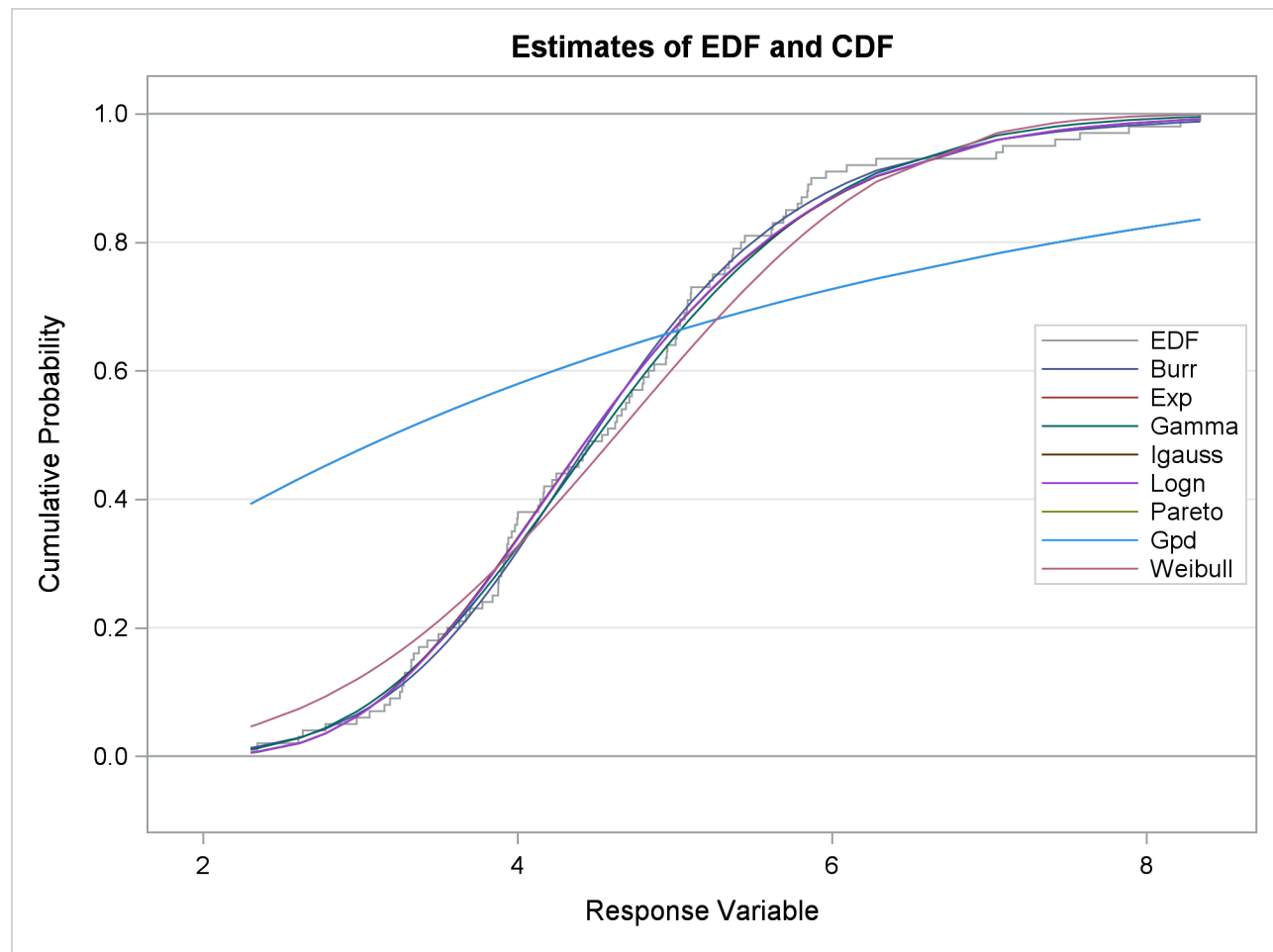
Figure 29.2 Comparison of EDF and CDF Estimates of the Fitted Models
