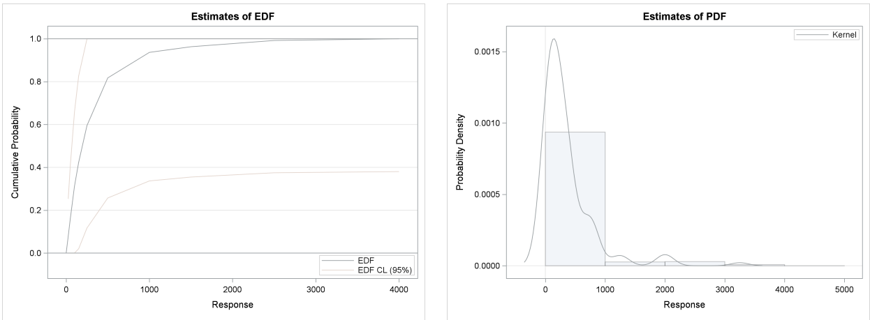
Output 29.6.1 Nonparametric Distribution Estimates for Interval-Censored Data
