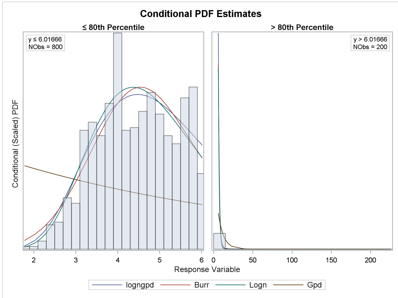
Output 29.4.3 Comparison of the Conditional PDF Estimates of the Fitted Models
