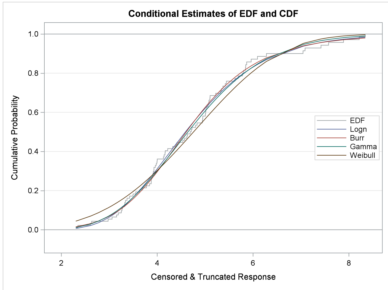
Figure 29.8 EDF and CDF Estimates for the Truncated and Censored Data
