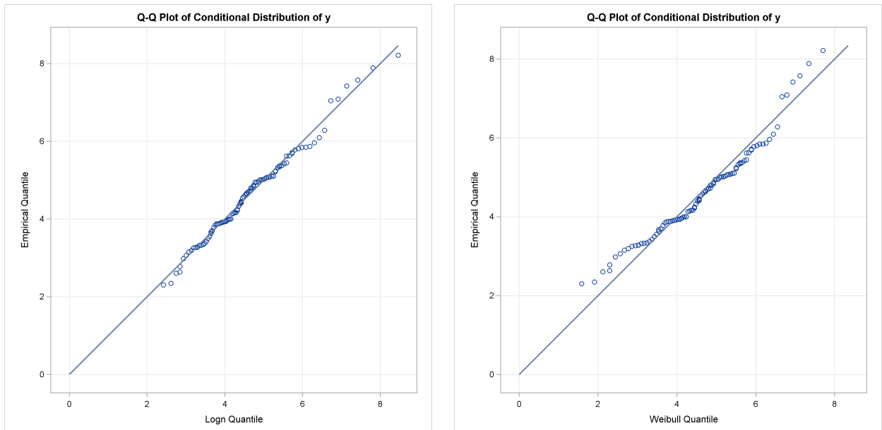
Figure 29.11 Q-Q Plots for Lognormal and Weibull Models Fitted to Truncated and Censored Data
