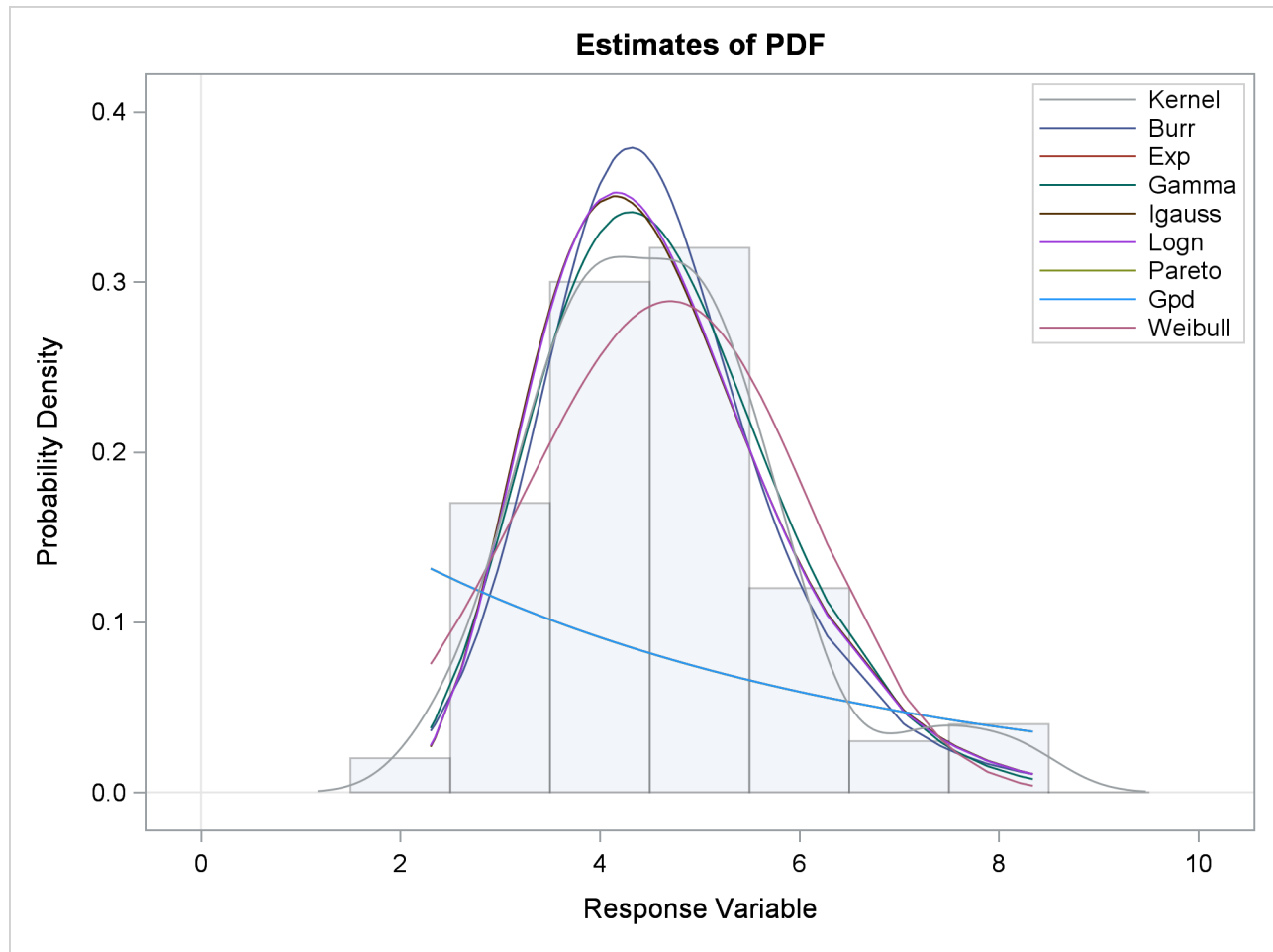
Figure 29.3 Comparison of PDF Estimates of the Fitted Models
