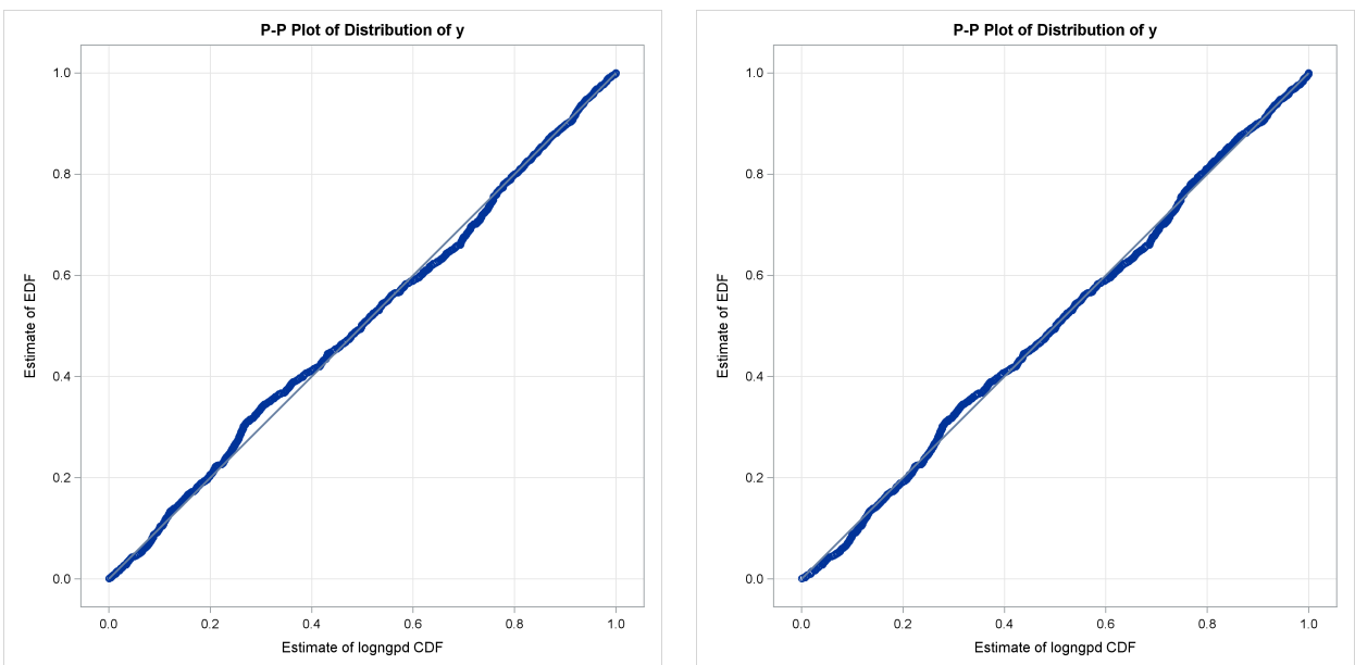
Output 29.4.2 P-P Plots for LOGNGPD Model with Maximum Likelihood (Left) and Cramér–von Mises (Right) Estimators
