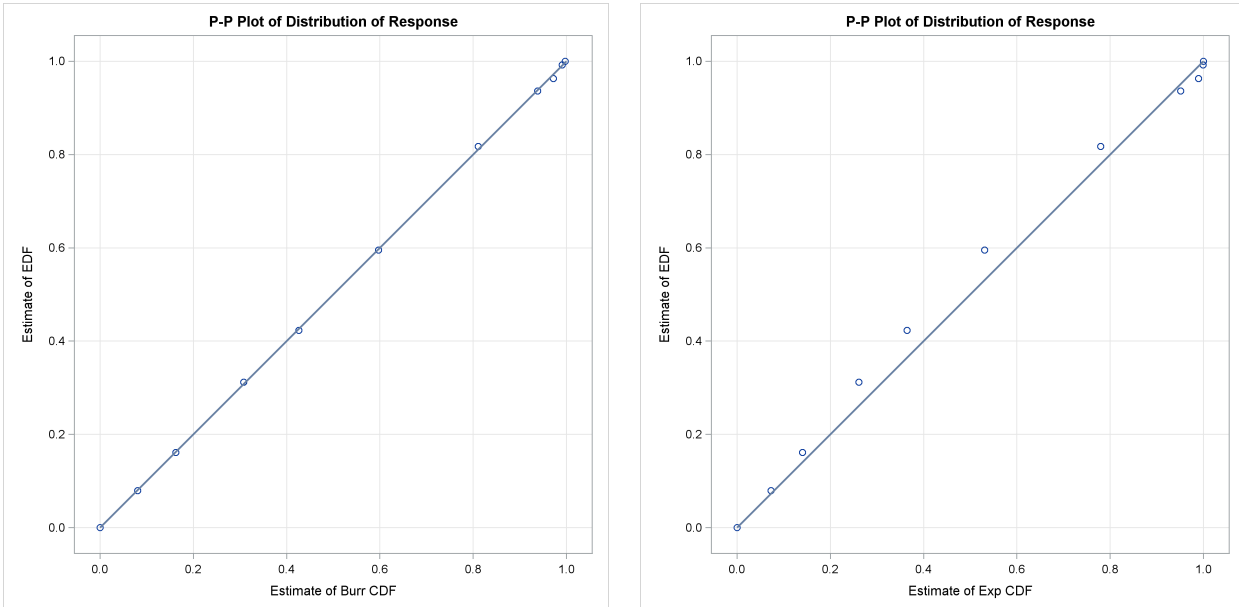
Output 29.6.4 P-P Plots of Burr and Exponential Distributions for Interval-Censored Data
