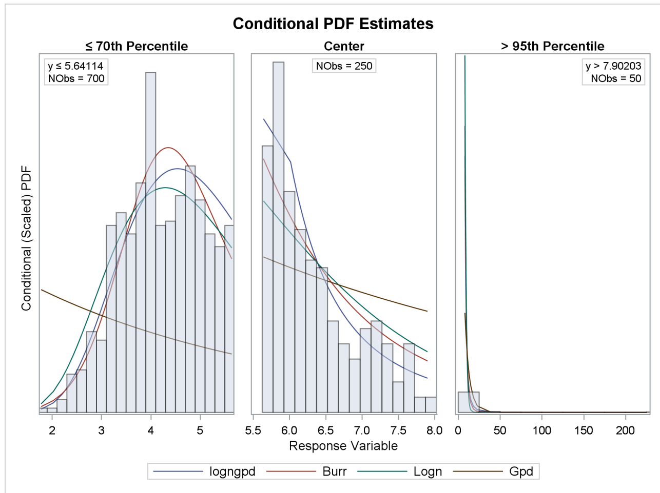
Output 29.3.3 Comparison of the Conditional PDF Estimates of the Fitted Models
