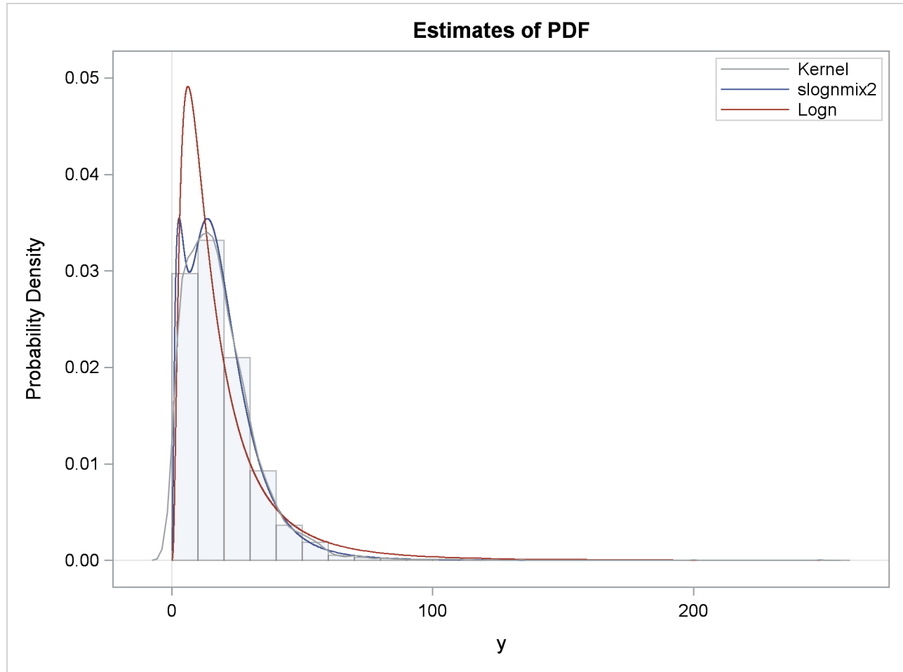
Output 29.7.2 Comparison of PDF Estimates of the Fitted Models
