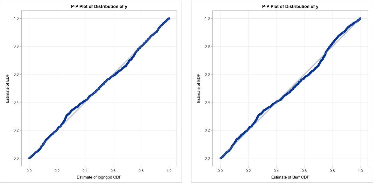
Output 29.3.4 P-P Plots for the LOGNGPD and BURR Distribution Models
