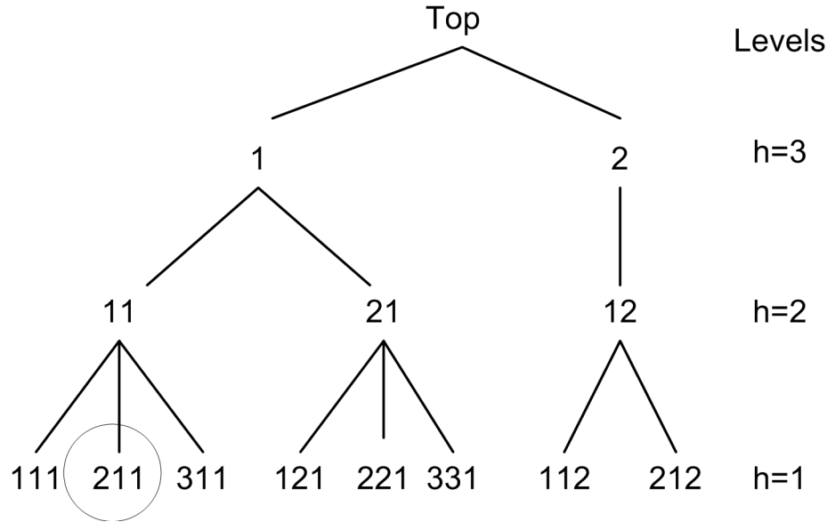
Figure 24.26 Node Indices for a Three-Level Tree
