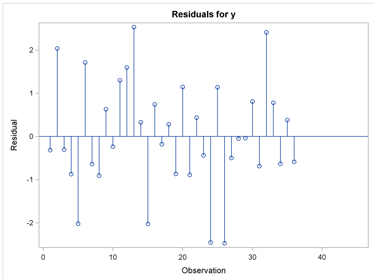
Output 8.8.1 Residuals Plot
