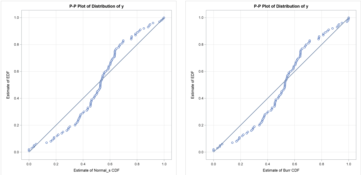
Output 29.2.5 Comparison of EDF and CDF Estimates of NORMAL_S and BURR Models
