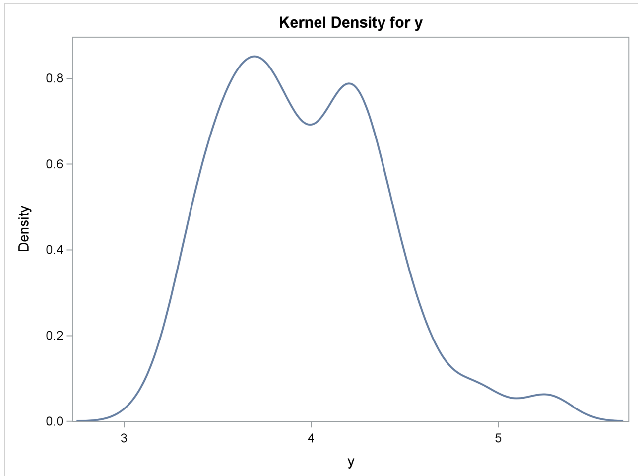
Figure 25.24 Empirical PDF Plot
