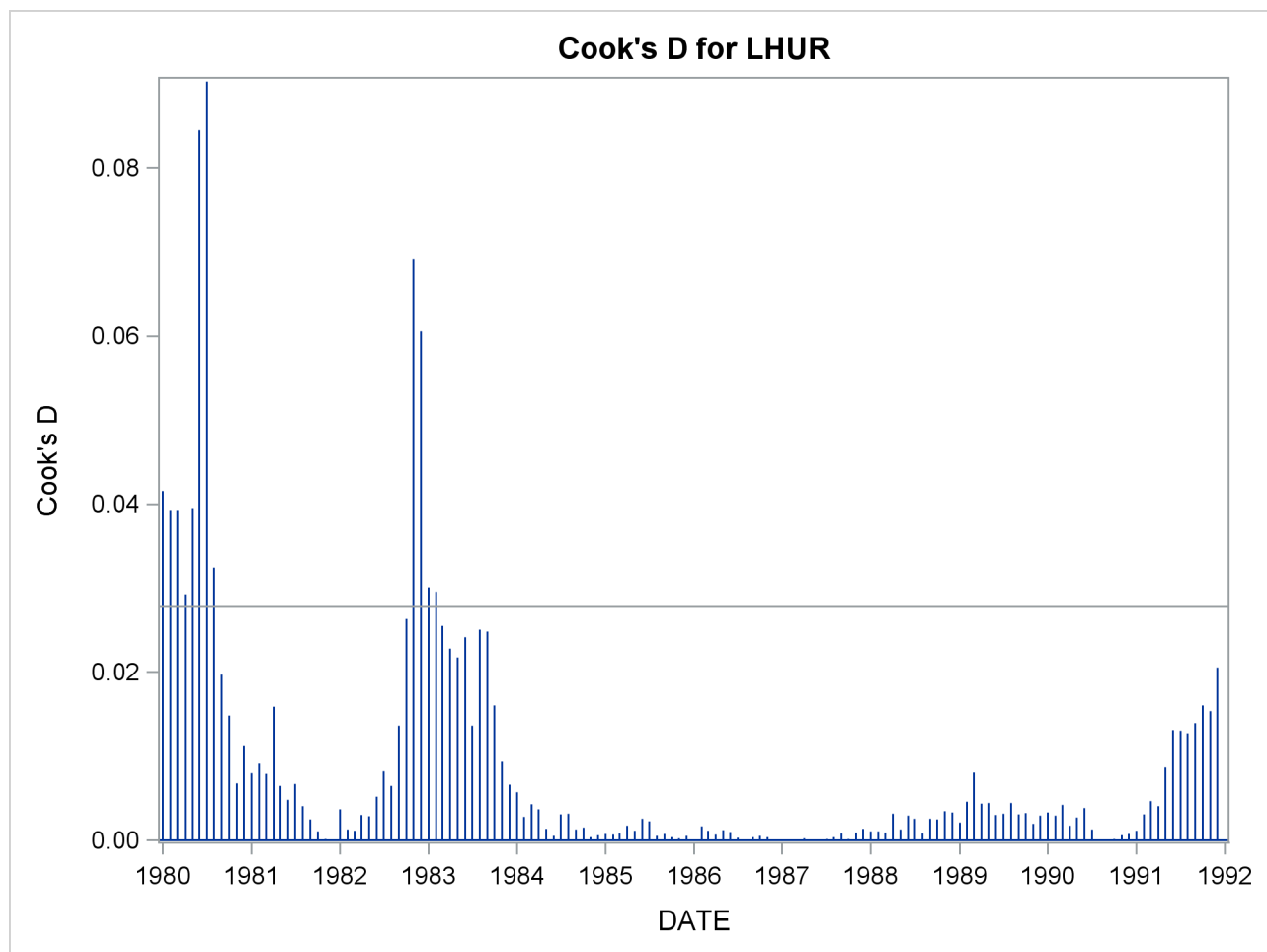
Output 25.20.4 Cook's D Plot
