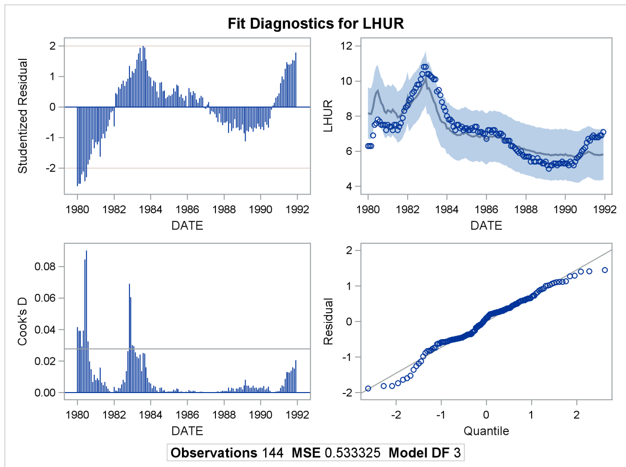
Output 25.20.1 Diagnostics Plots
