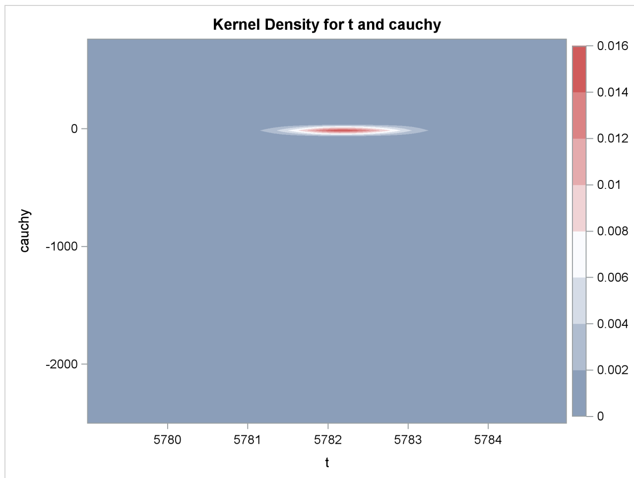
Output 25.14.2 Bivariate Density of t and Cauchy, Kernel Density for t and Cauchy
