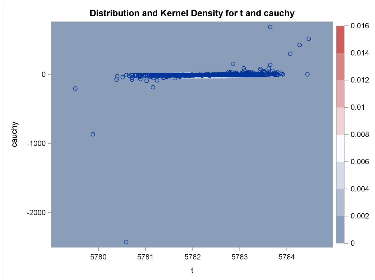
Output 25.14.3 Bivariate Density of t and Cauchy, Distribution and Kernel Density for t and Cauchy
