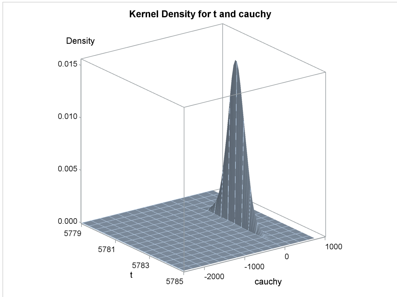
Output 25.14.5 Bivariate Density of t and Cauchy, Kernel Density for t and Cauchy
