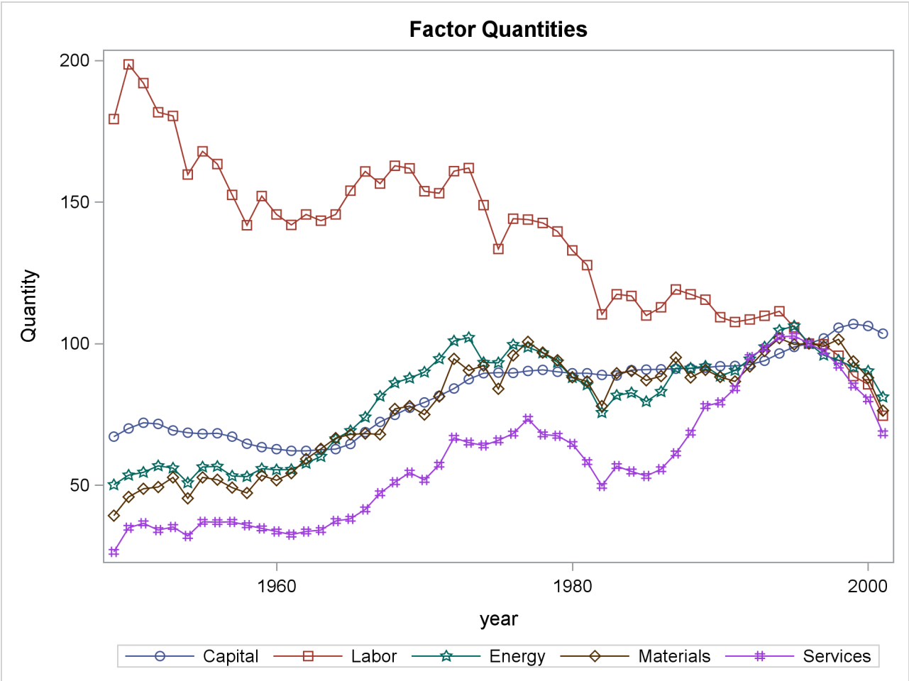
Output 25.21.1 Changes in Variables over Time
