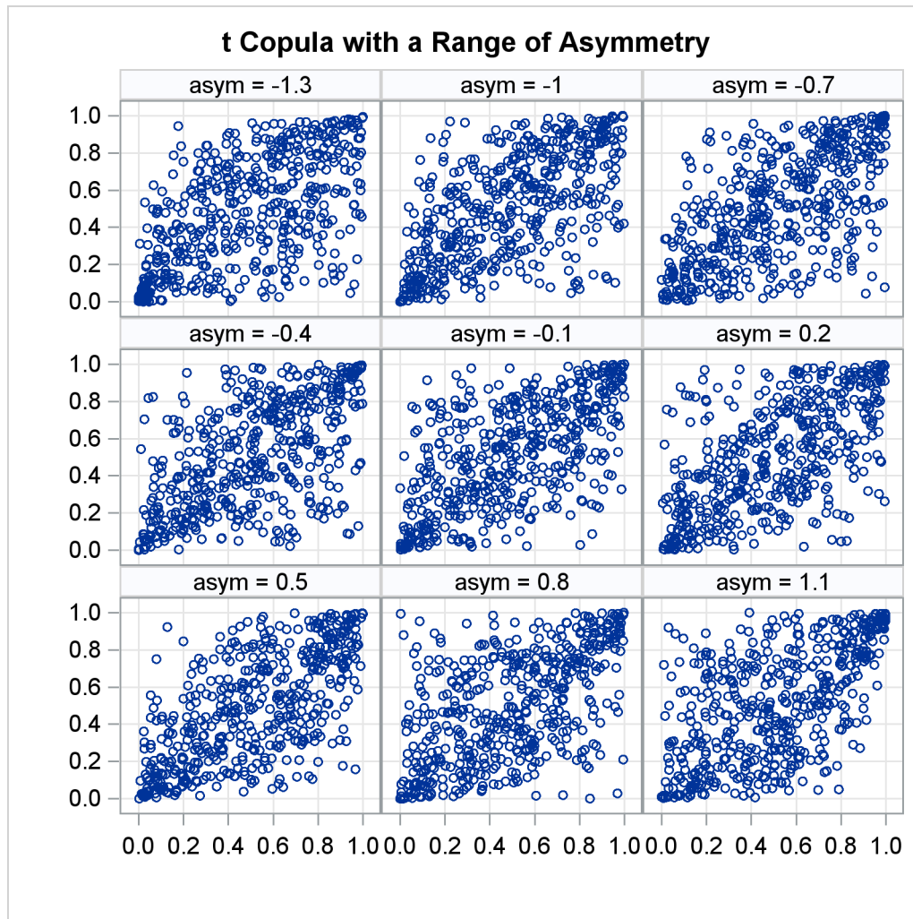
Figure 25.74 t Copula with Asymmetry
