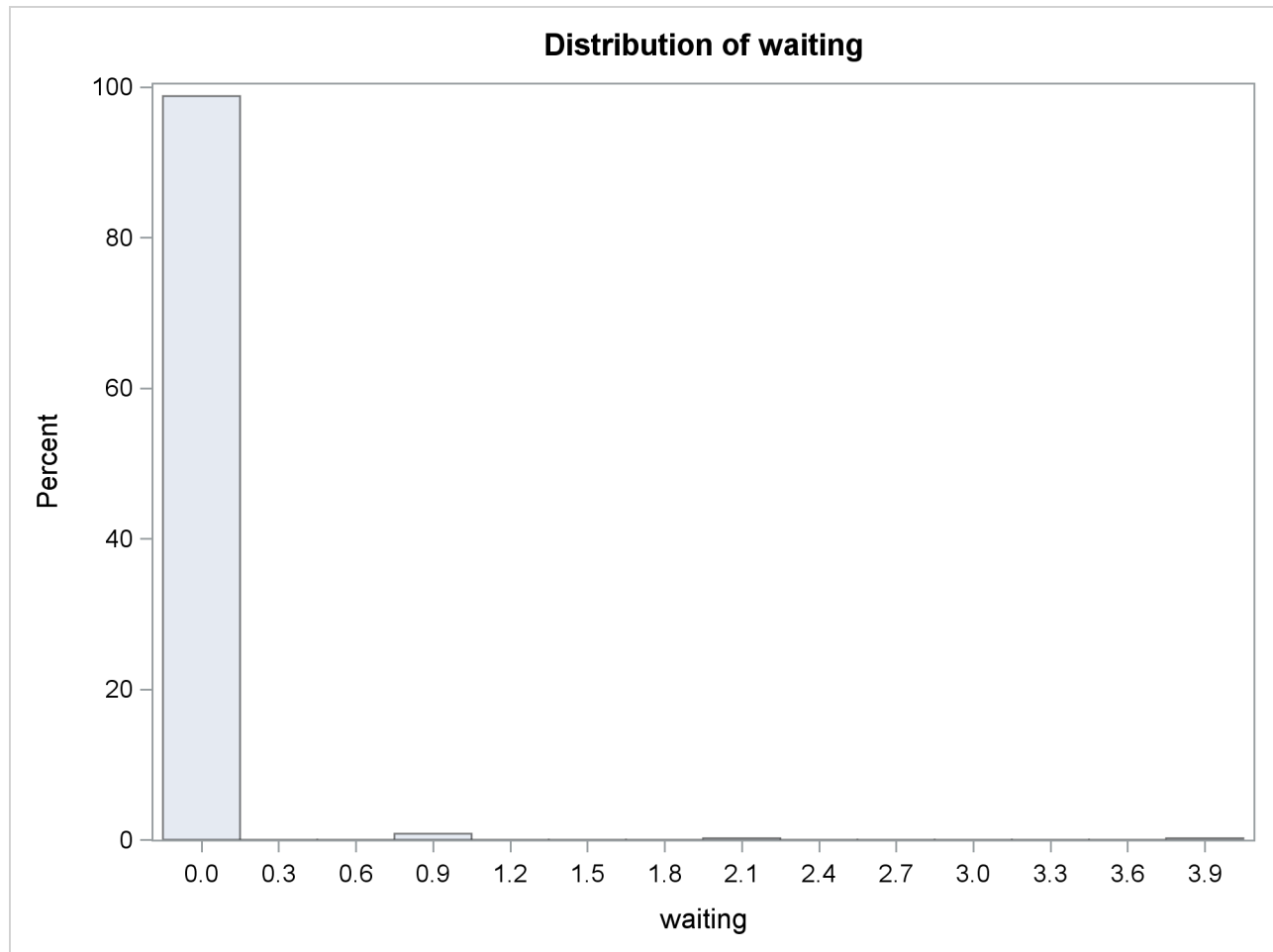
Figure 25.73 Distribution of Number of Clients Waiting
