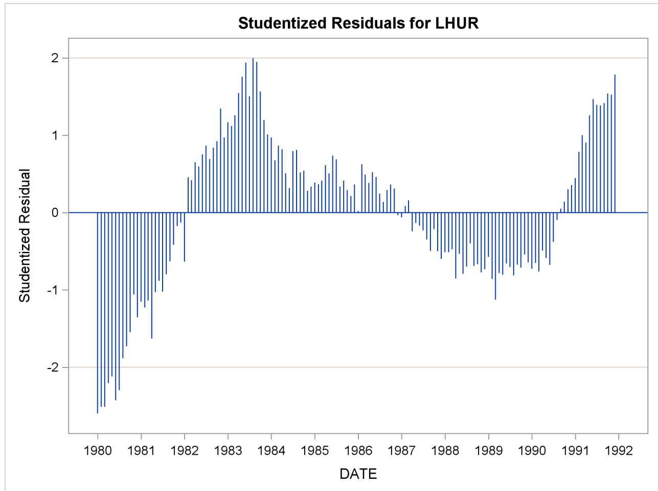
Output 25.20.3 Studentized Residuals Plot
