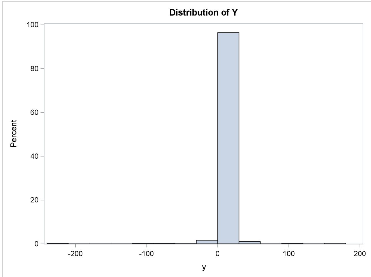
Output 25.12.1 Distribution of Y
