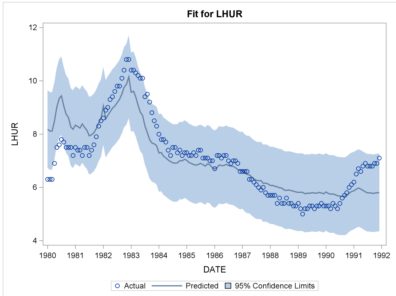
Output 25.20.5 Predicted versus Actual Plot
