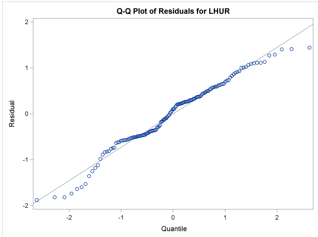
Output 25.20.9 Q-Q Plot of Residuals
