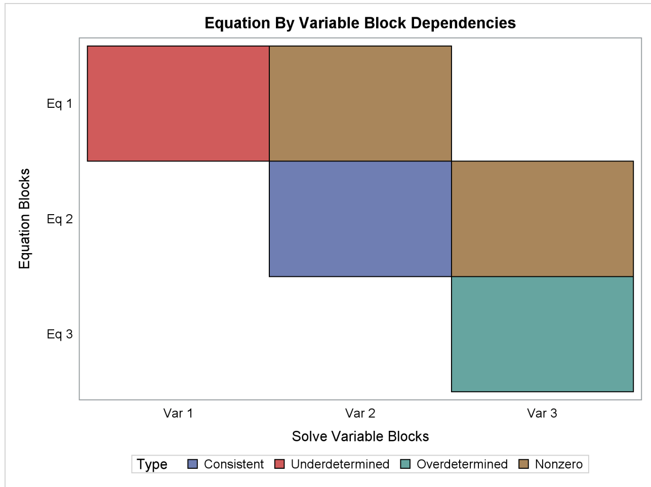
Figure 25.92 Block Dependency Analysis
