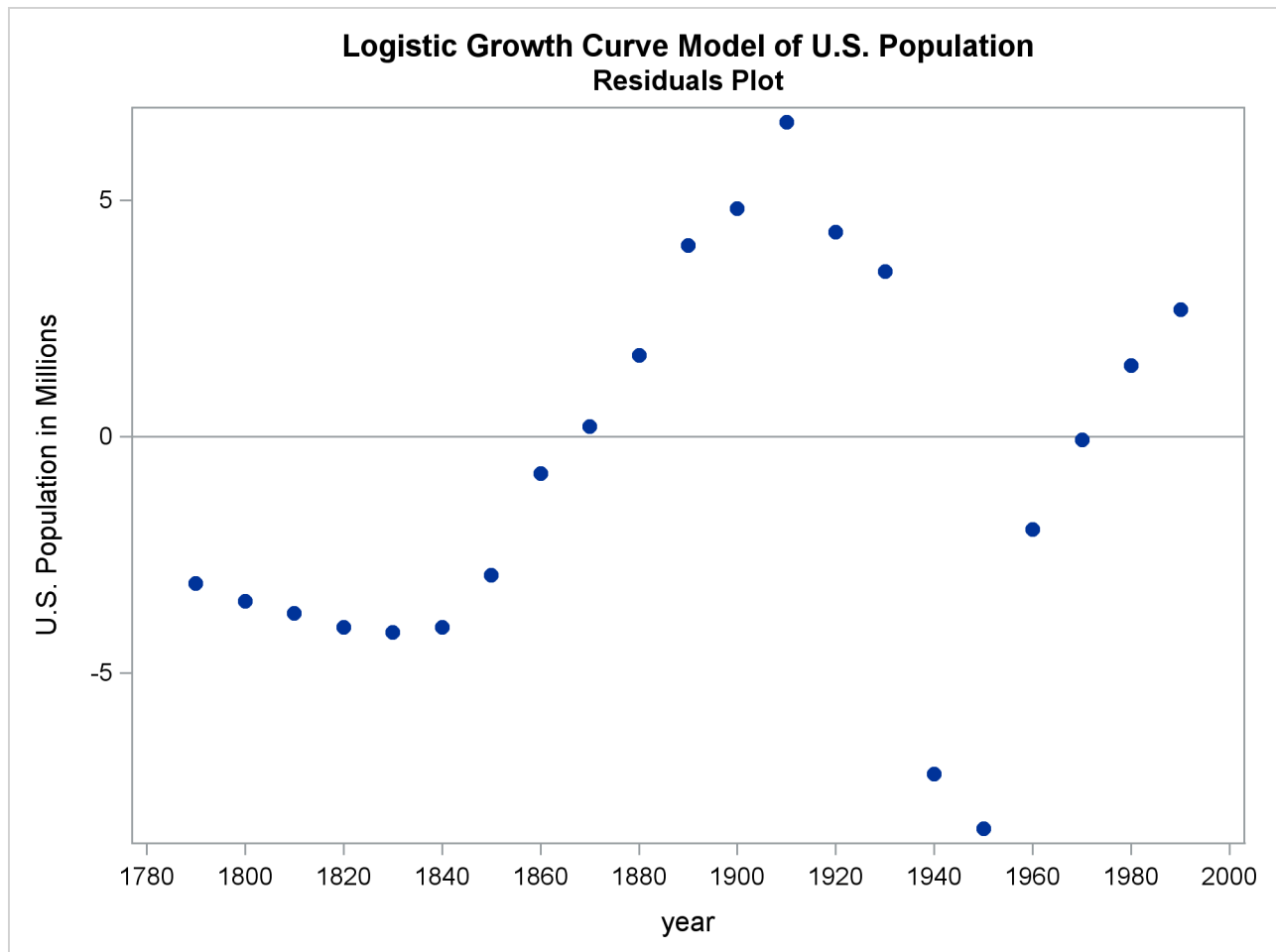
Output 25.1.4 Residual for Population Model (Actual–Predicted)
