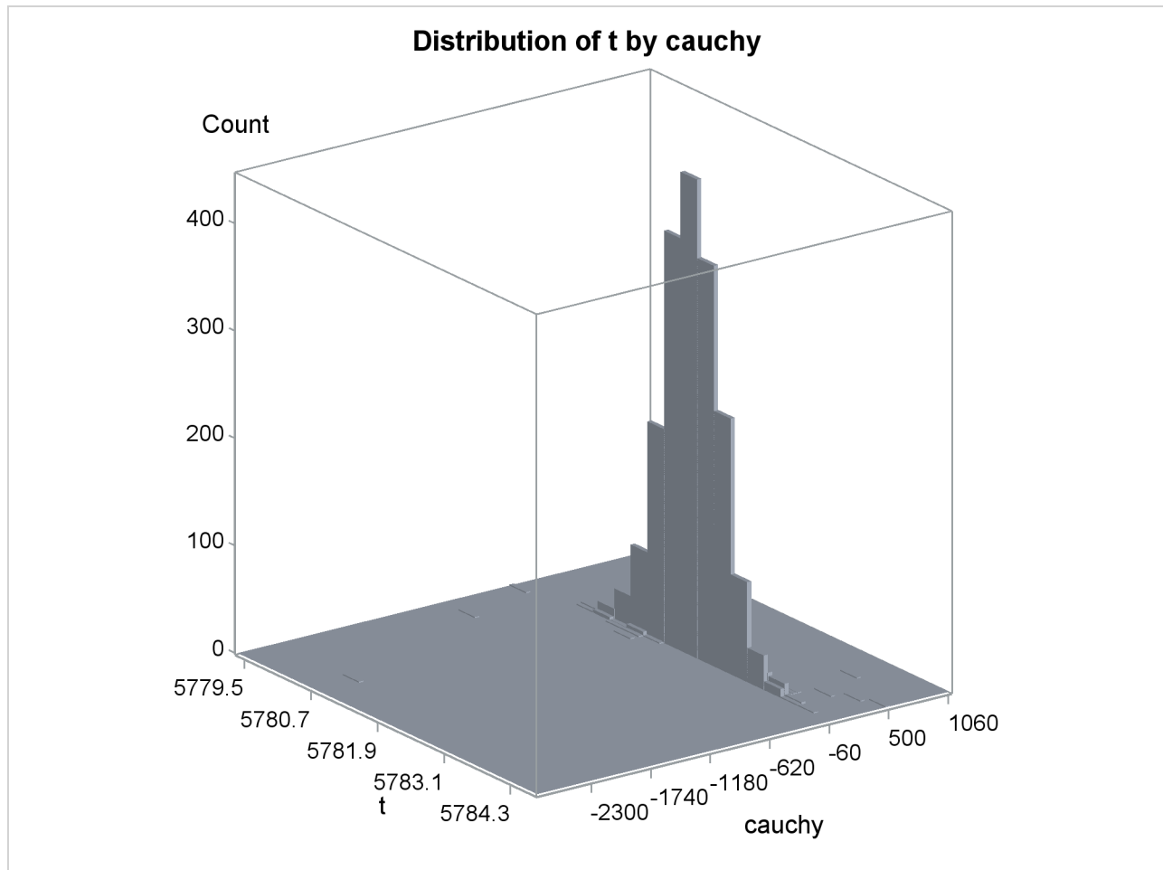
Output 25.14.4 Bivariate Density of t and Cauchy, Distribution of t by Cauchy
