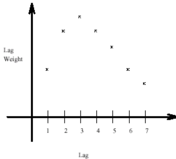
Figure 25.64 Polynomial Distributed Lags
