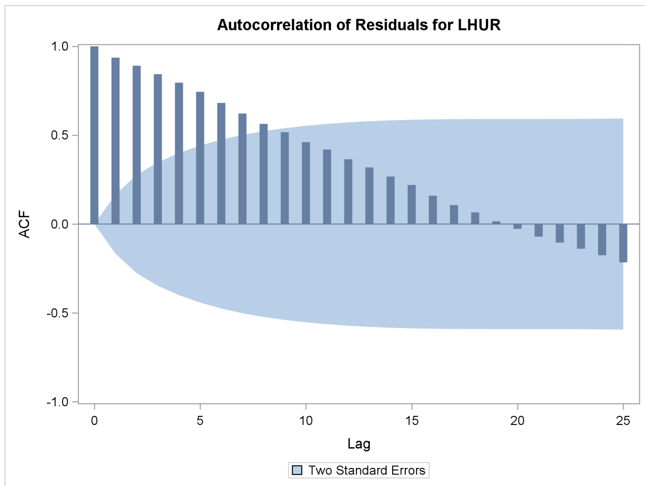
Output 25.20.6 Autocorrelation of Residuals Plot
