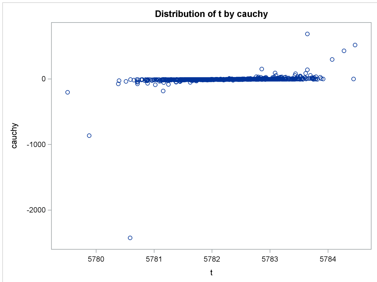
Output 25.14.1 Bivariate Density of t and Cauchy, Distribution of t by Cauchy
