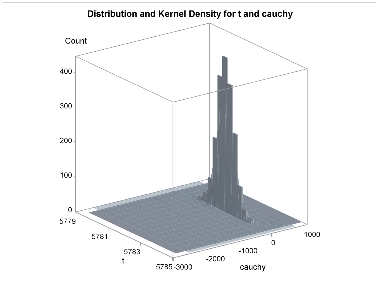
Output 25.14.6 Bivariate Density of t and Cauchy, Distribution and Kernel Density for t and Cauchy
