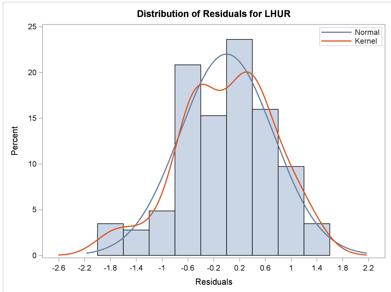
Output 25.20.10 Histogram of Residuals
