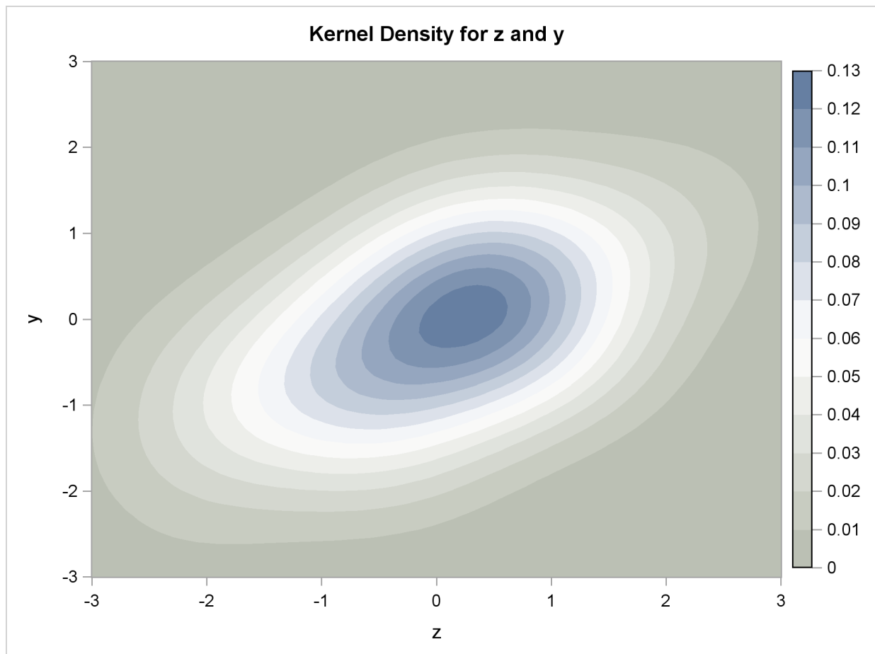
Figure 25.76 Kernel Density of a Bivariate Normal Produced by 100 Pseudo-Random Draws
