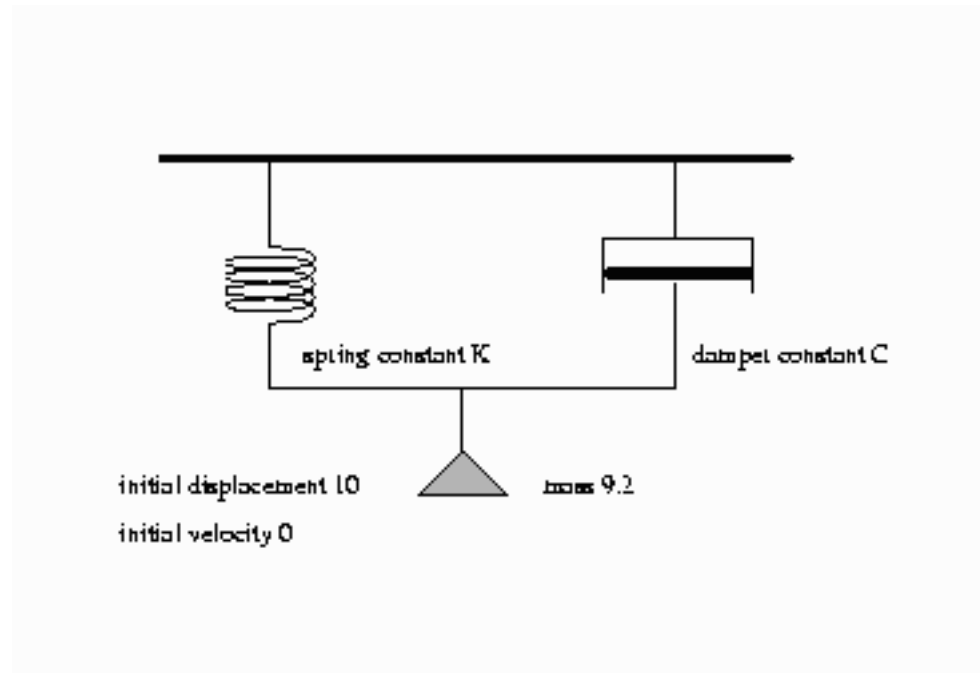
Figure 25.99 Spring and Damper System Model
