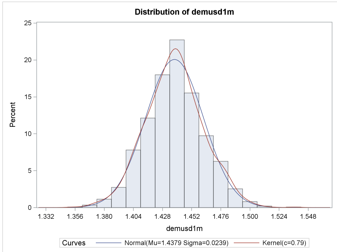
Figure 25.72 Distribution of DEMUSD1M
