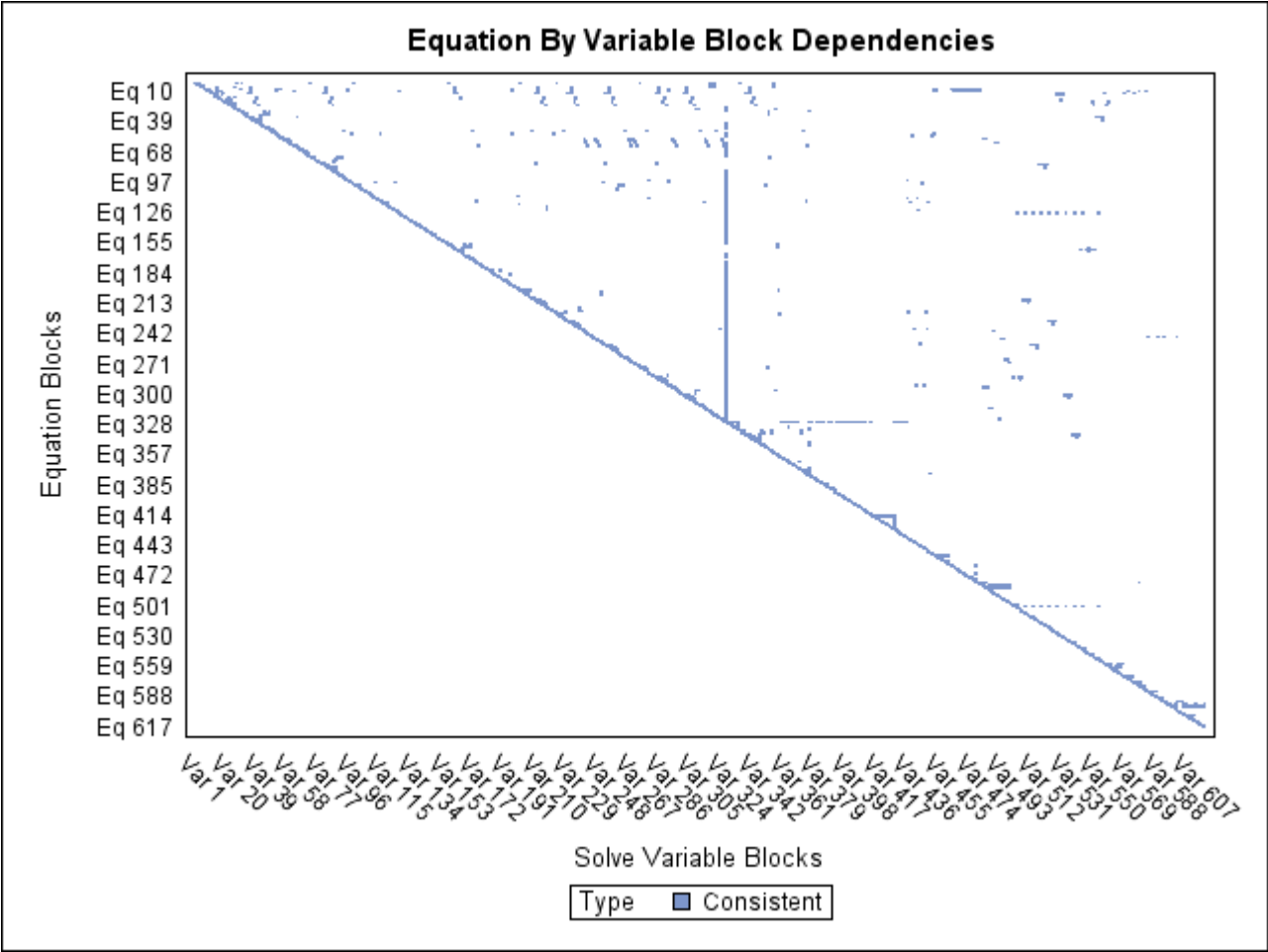
Figure 25.94 Block Triangular Form of U.S. Agriculture Model
