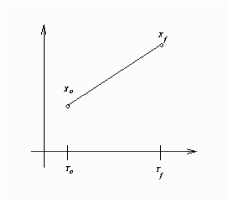
Figure 25.55 Form of X Used for Integration in Goal Seeking
