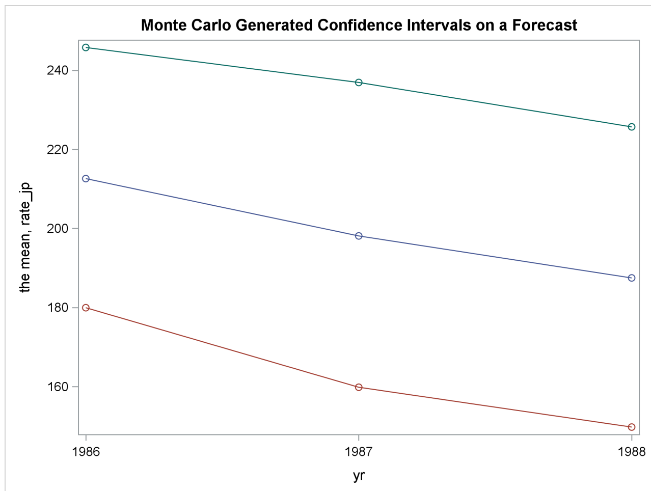
Figure 25.12 Monte Carlo Confidence Interval Plot
