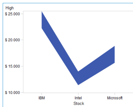
Figura A2.20 Diagramma a fasce
