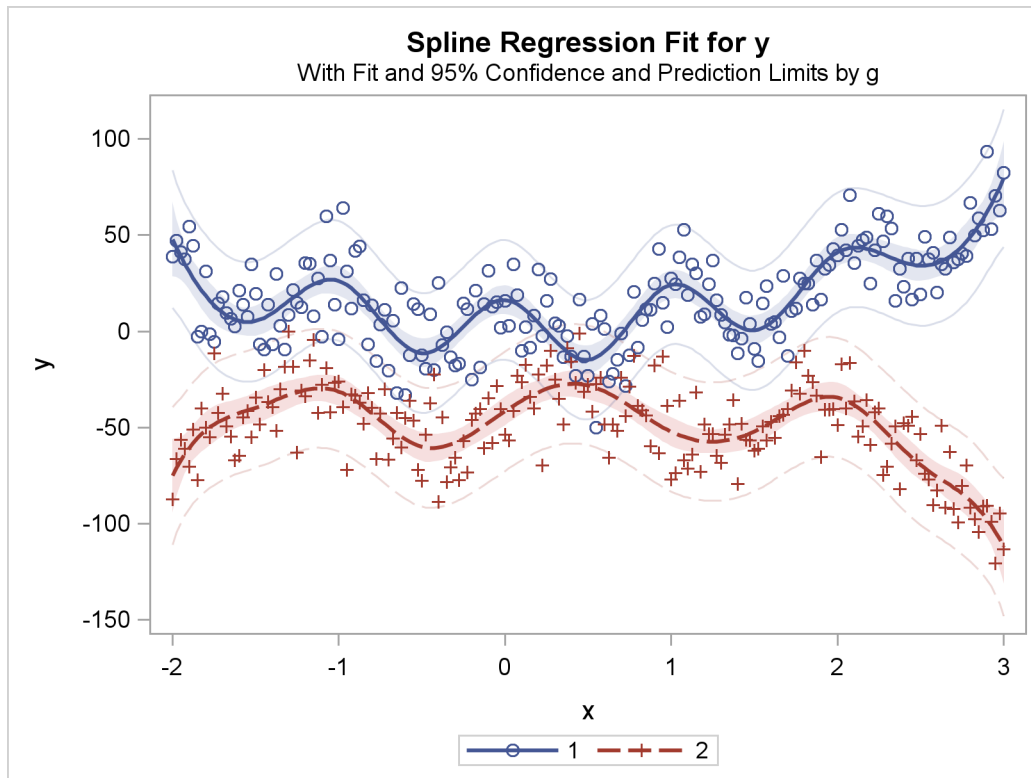
Figure 90.40 Separate Curves, Separate Intercepts
