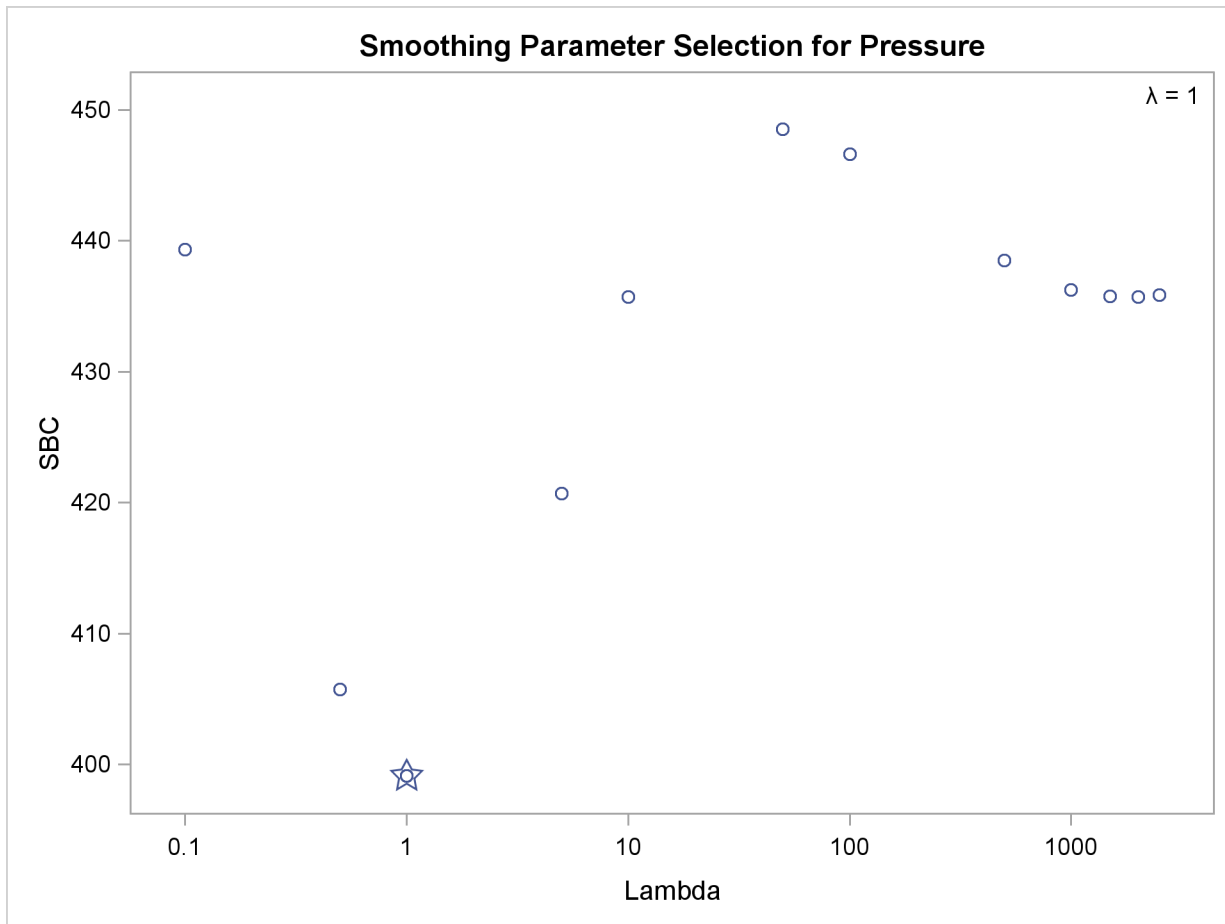
Output 90.3.4 Change in Atmospheric Pressure, SBC, Over the Range of Both Minima
