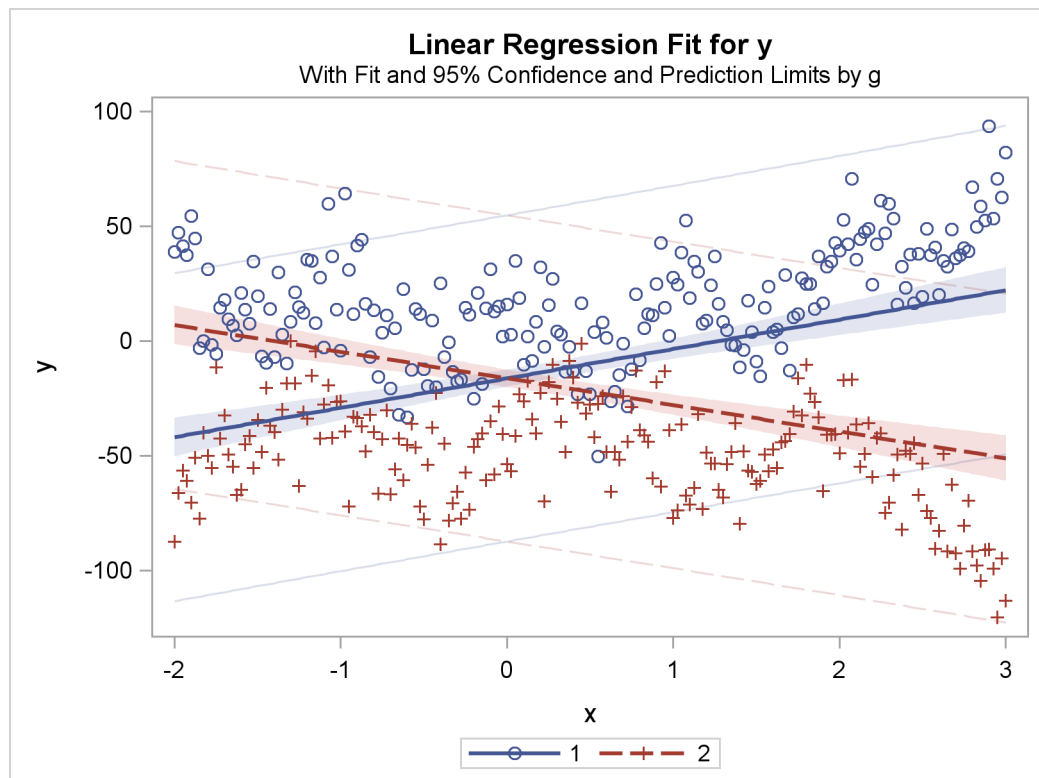
Figure 90.35 Separate Slopes, Same Intercept
