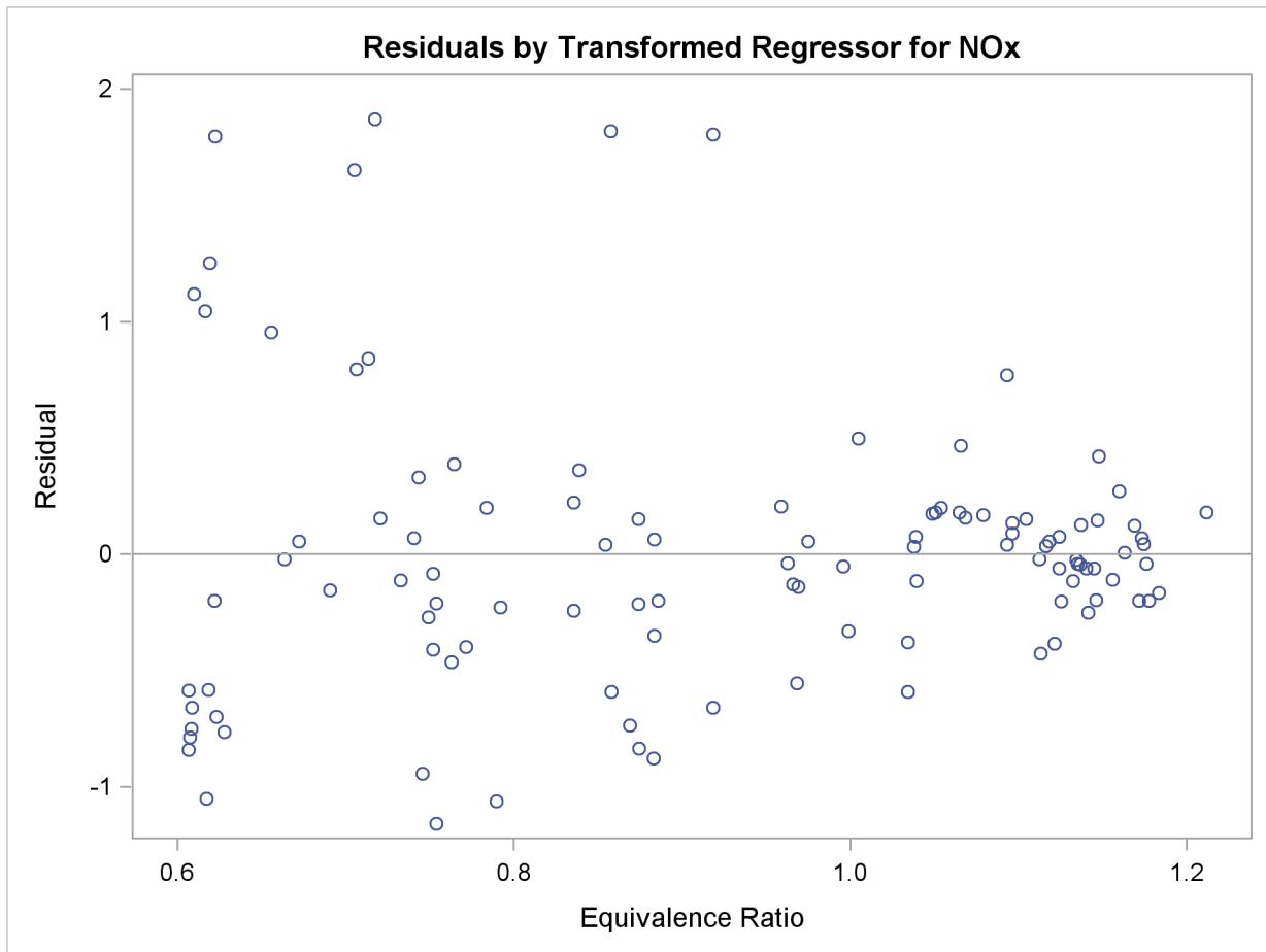
Figure 90.3 Residuals
