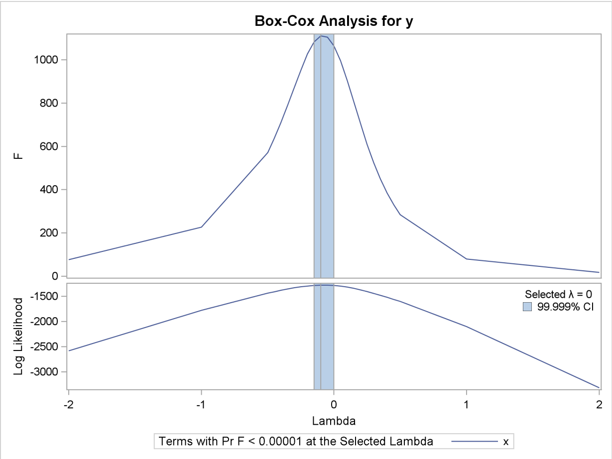
Figure 90.16 Basic Box-Cox Example, Several Options Demonstrated
