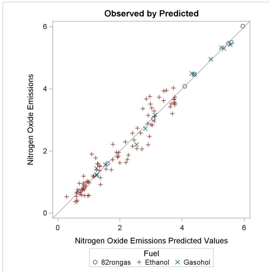
Figure 90.9 Observed by Predicted
