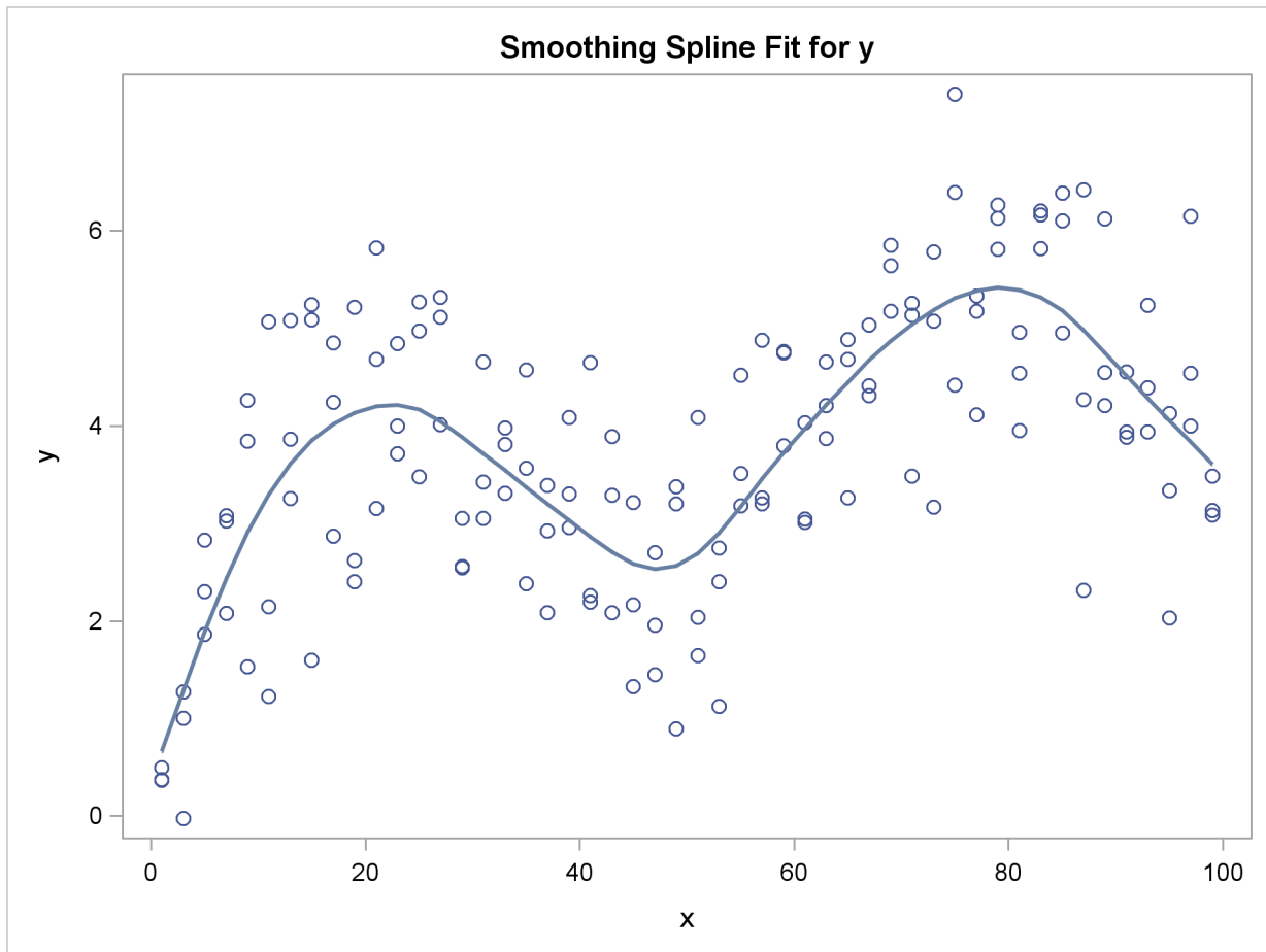
Figure 90.41 Smoothing Spline Displayed with ODS Graphics
