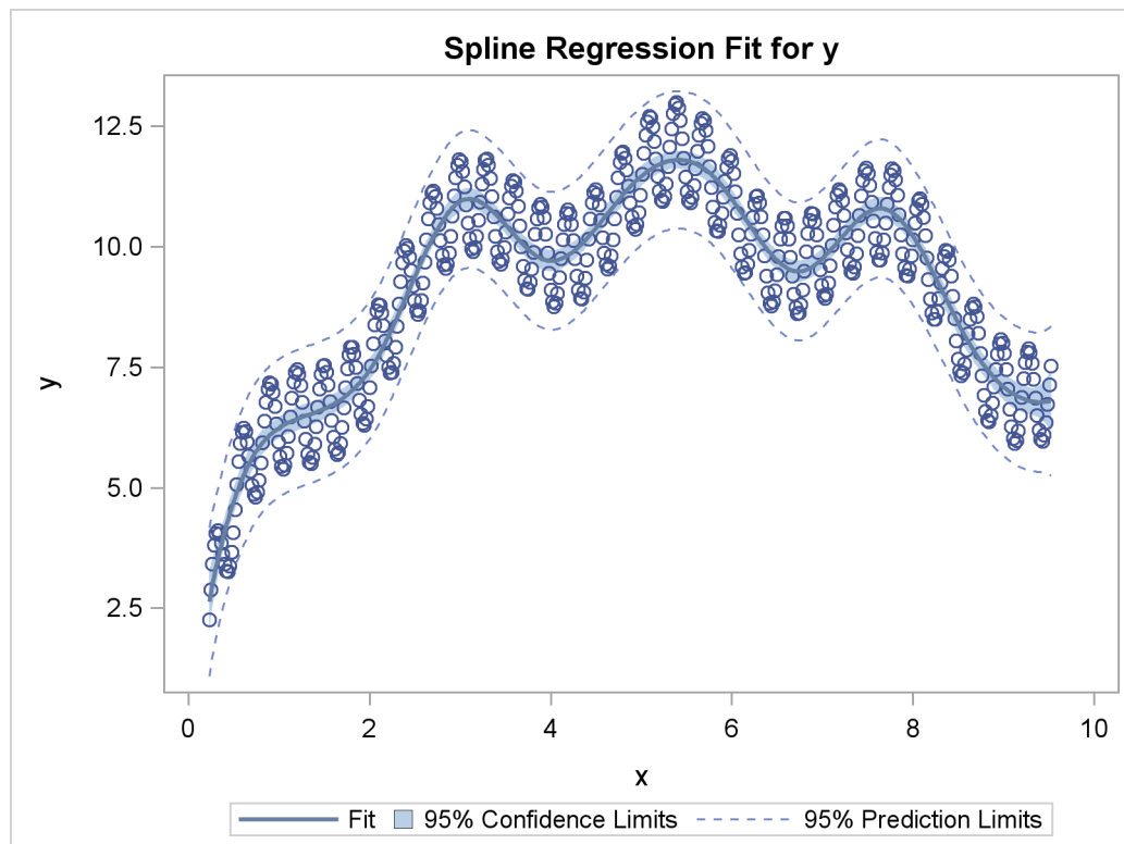
Figure 90.30 A Nonlinear Regression Function
