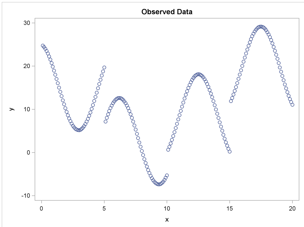
Figure 90.20 The Original Scatter Plot
