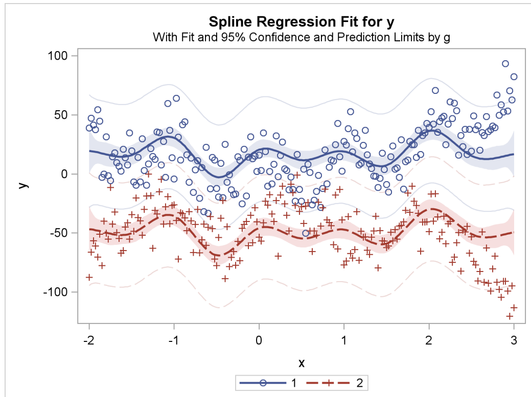
Figure 90.34 Parallel Curves, Separate Intercepts
