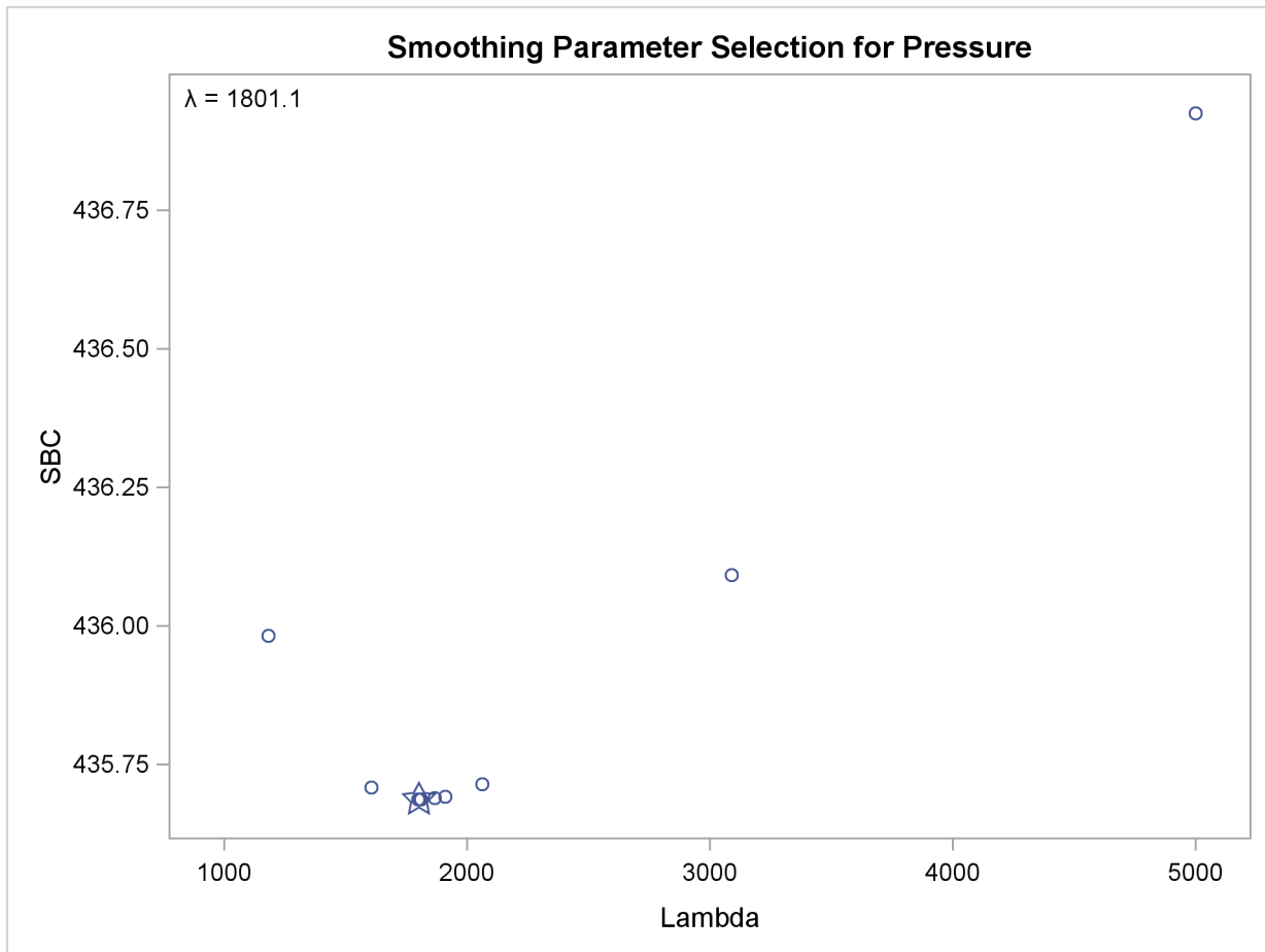
Output 90.3.3 Change in Atmospheric Pressure, SBC, Lambda > 1
