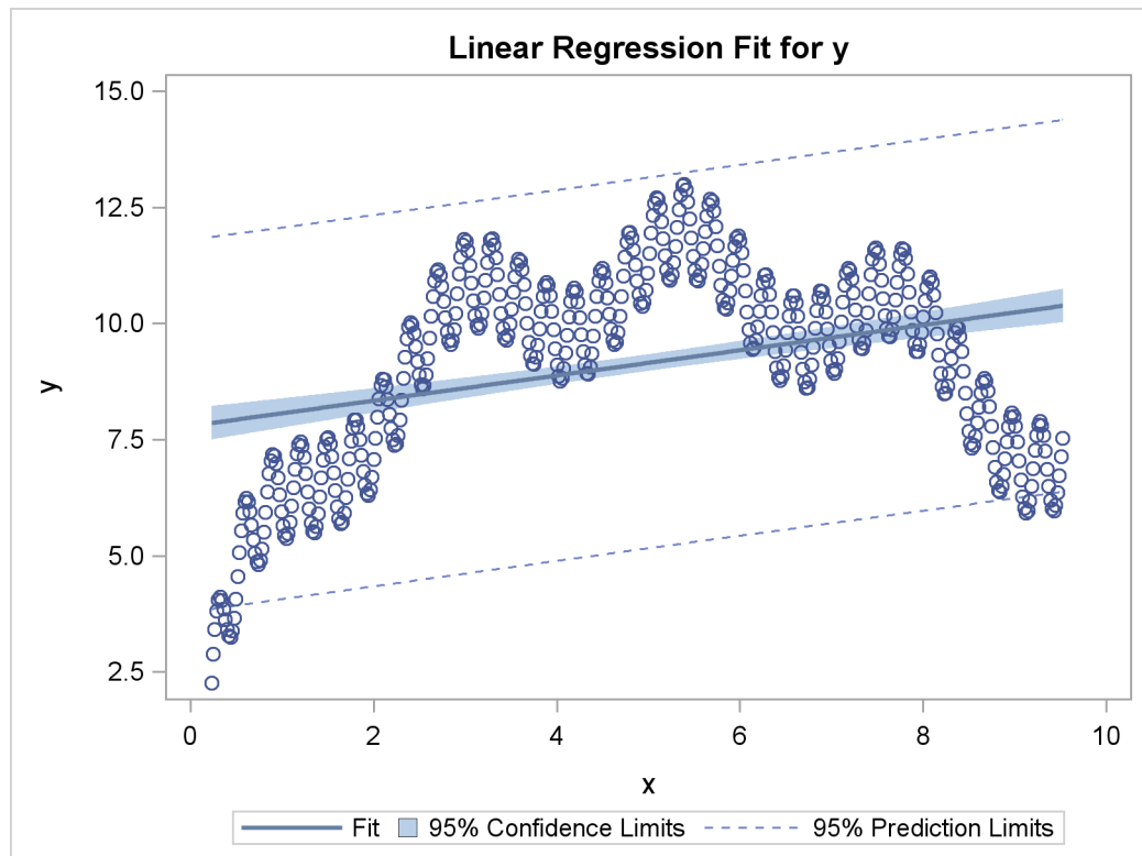
Figure 90.28 Linear Regression
