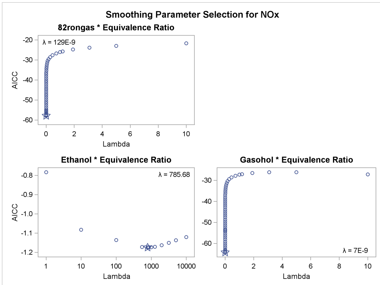
Figure 90.11 Penalized B-Splines
