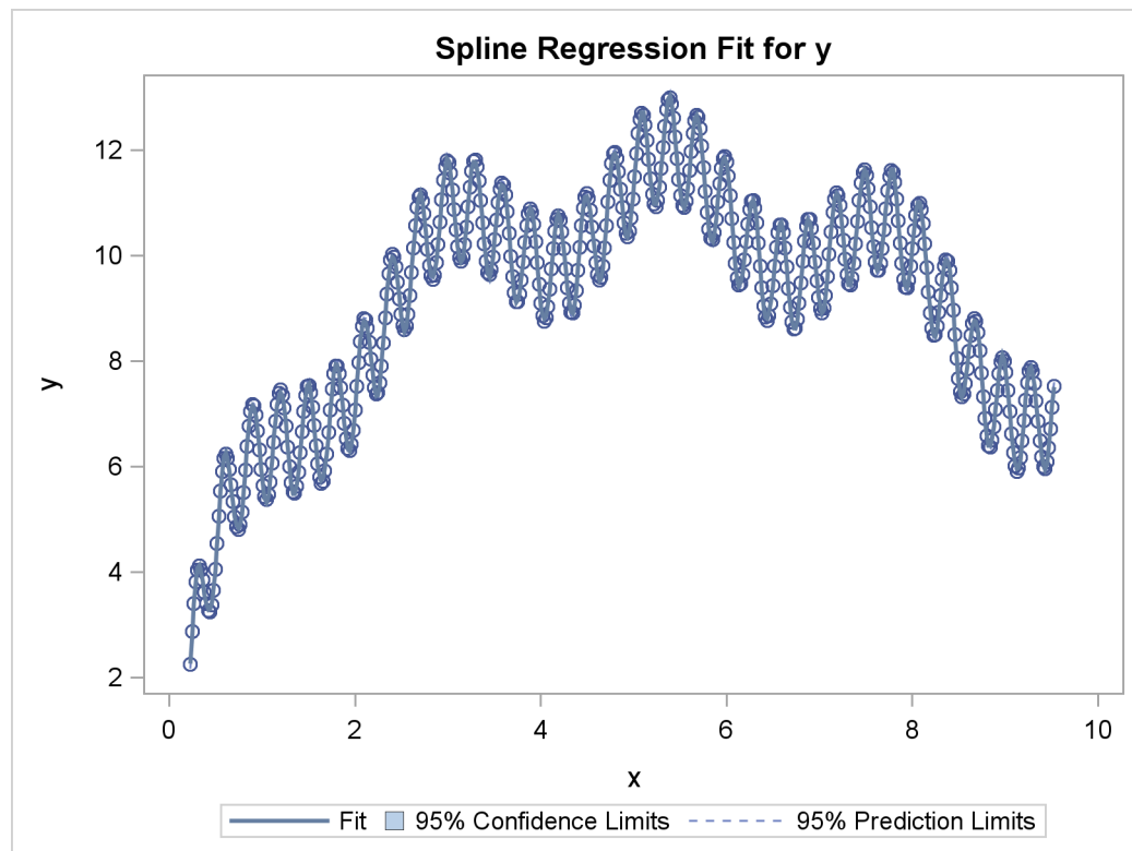
Figure 90.31 A Less-Smooth Nonlinear Regression Function
