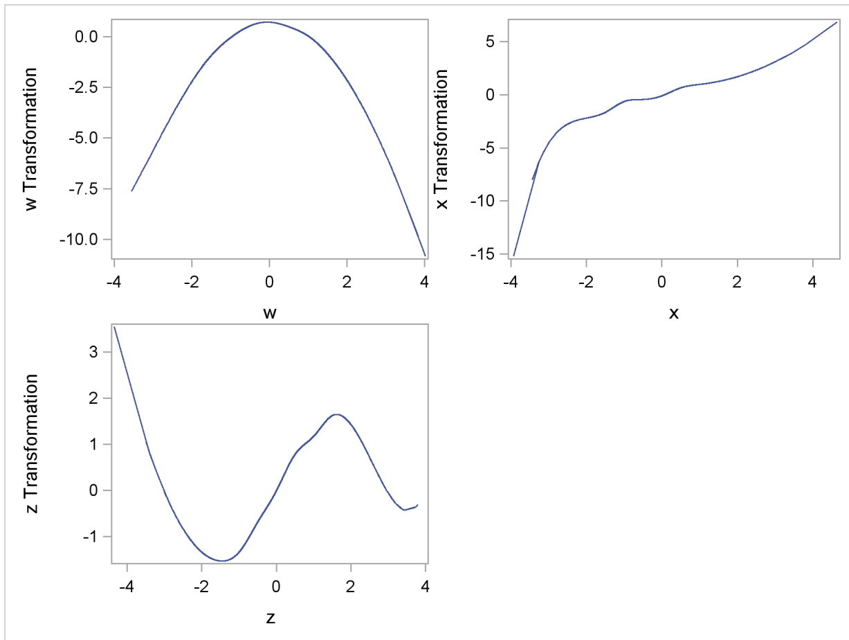
Figure 90.27 Scoring Spline Variables Example
