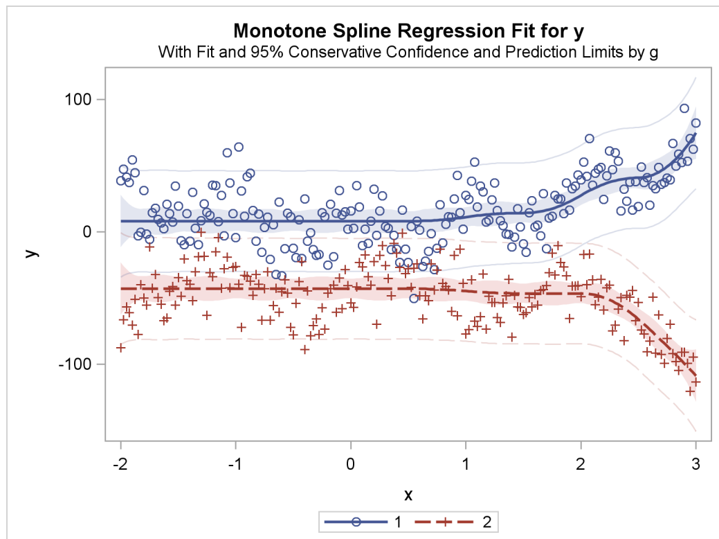
Figure 90.39 Separate Monotone Curves, Separate Intercepts
