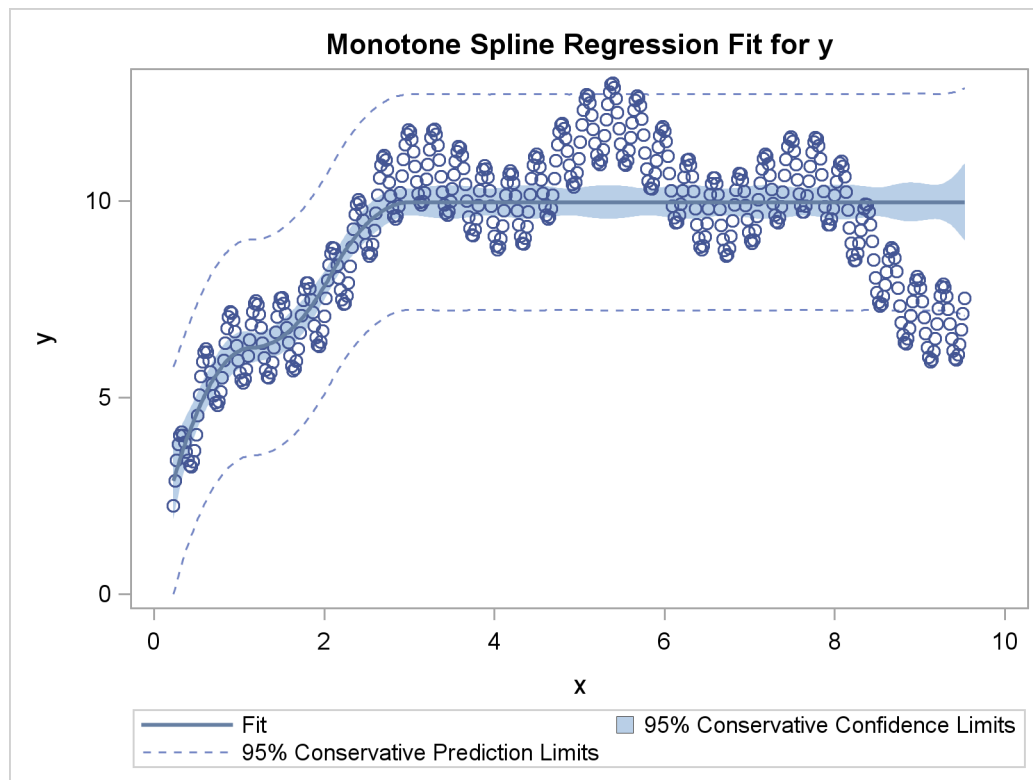
Figure 90.29 A Monotone Regression Function
