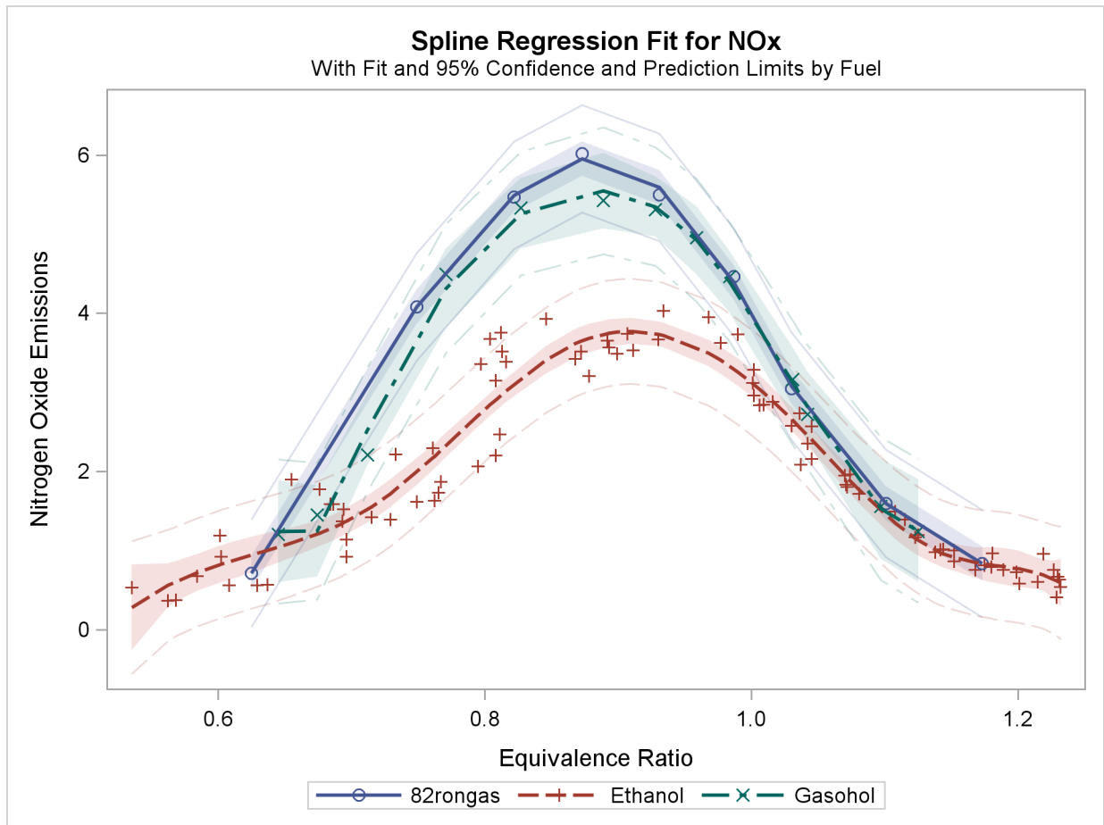
Figure 90.8 Fitting Curves through a Scatter Plot
