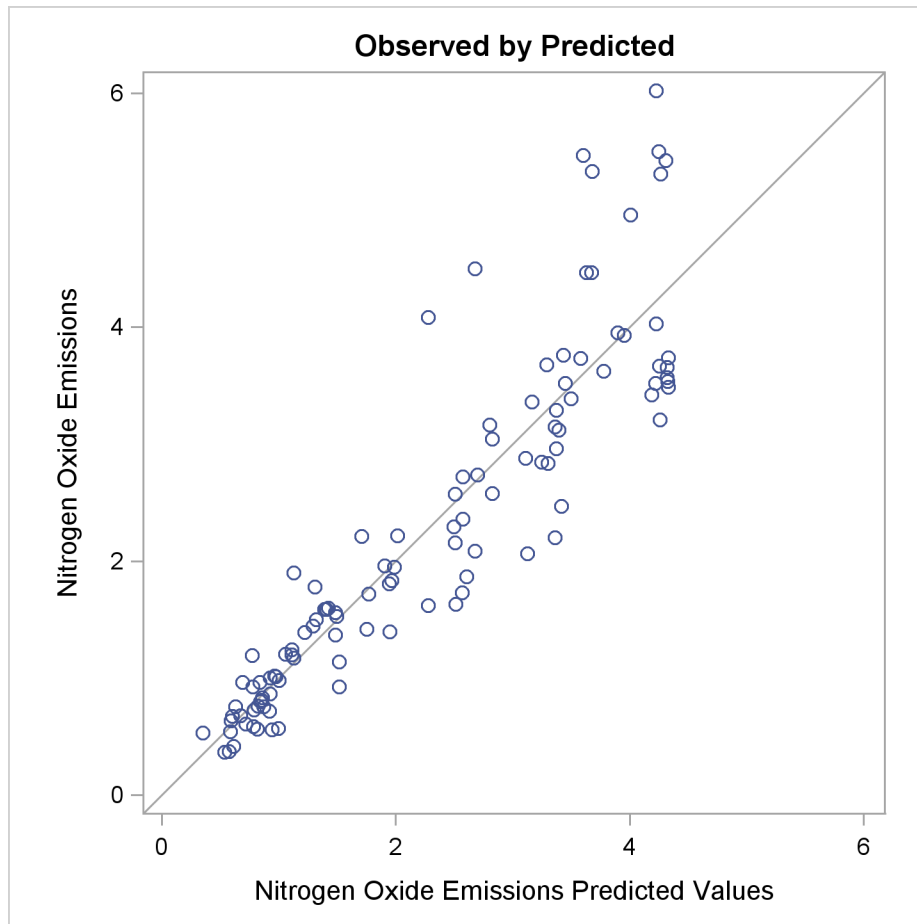
Figure 90.5 Observed by Predicted
