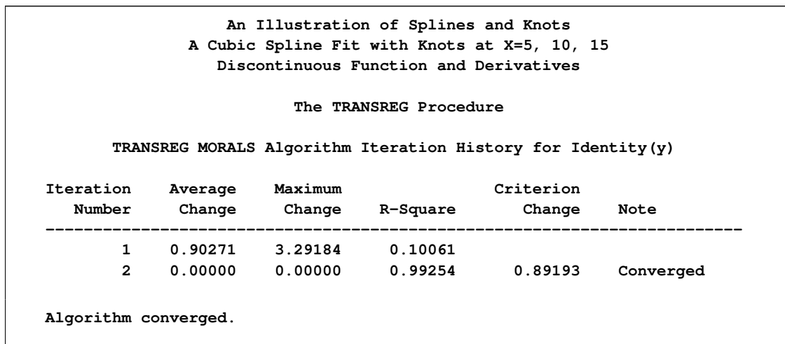
Figure 90.24 Discontinuous Spline Fit
