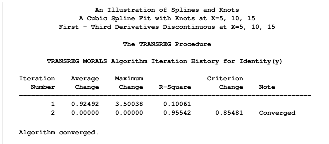
Figure 90.23 Spline with Discontinuous Derivatives
