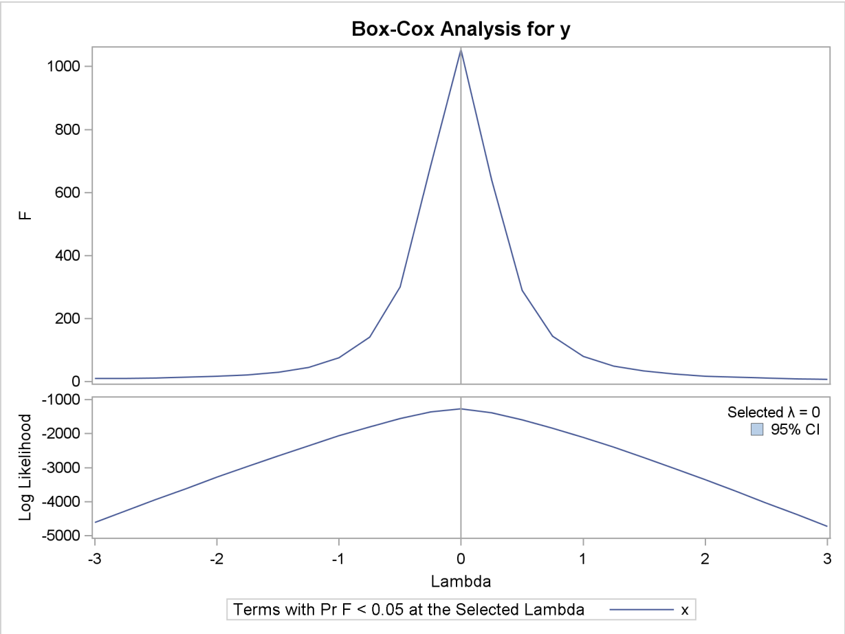
Figure 90.14 Basic Box-Cox Example, Default Output
