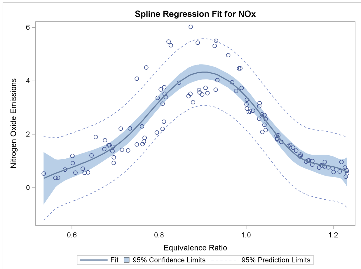
Figure 90.4 Fitting a Curve through a Scatter Plot
