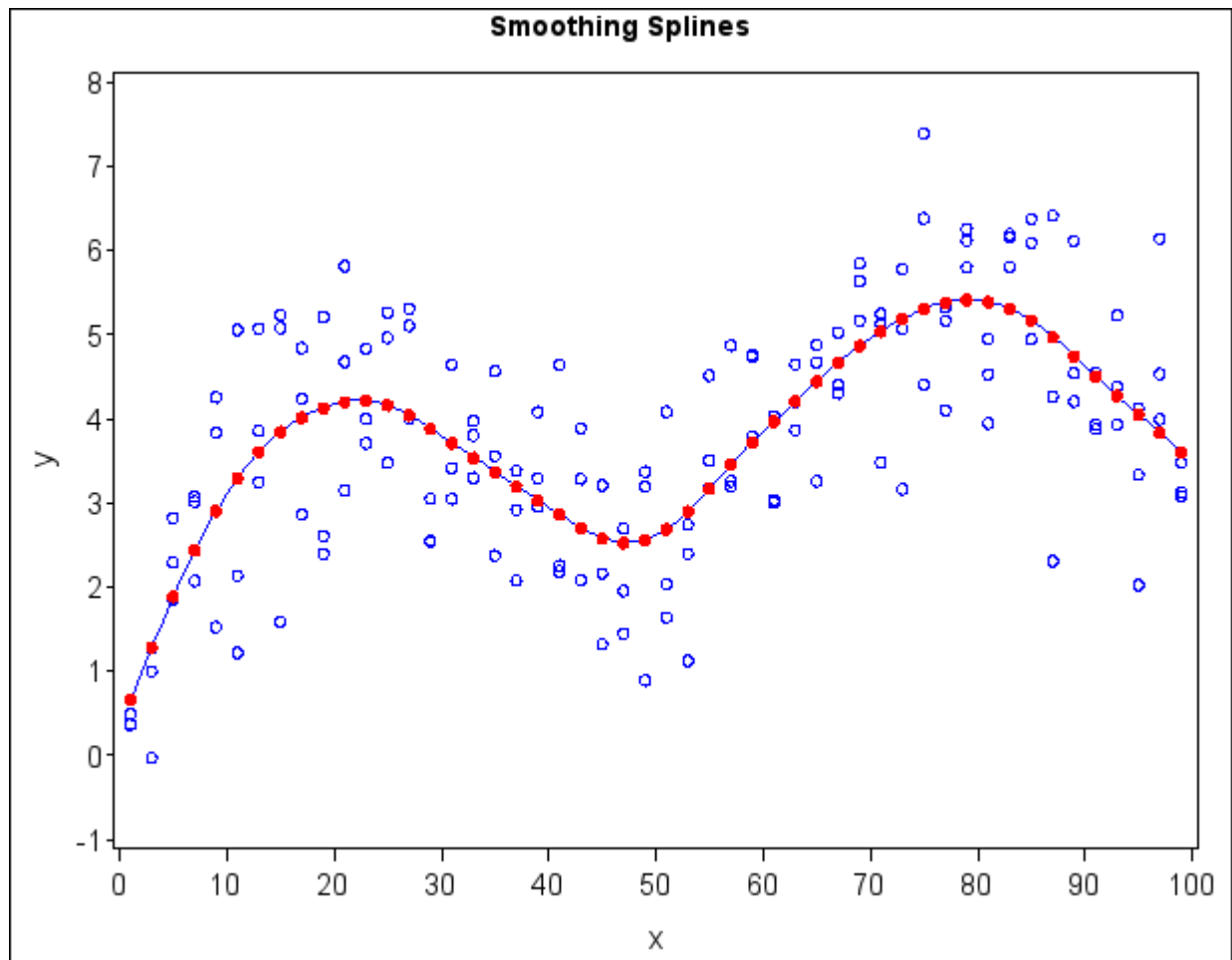
Figure 90.42 Smoothing Spline Created by PROC TRANSREG and PROC GPLOT, Overlaid
