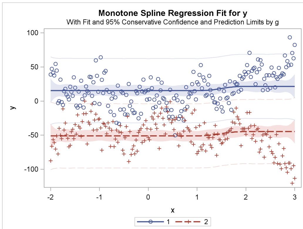
Figure 90.33 Parallel Monotone Curves, Separate Intercepts
