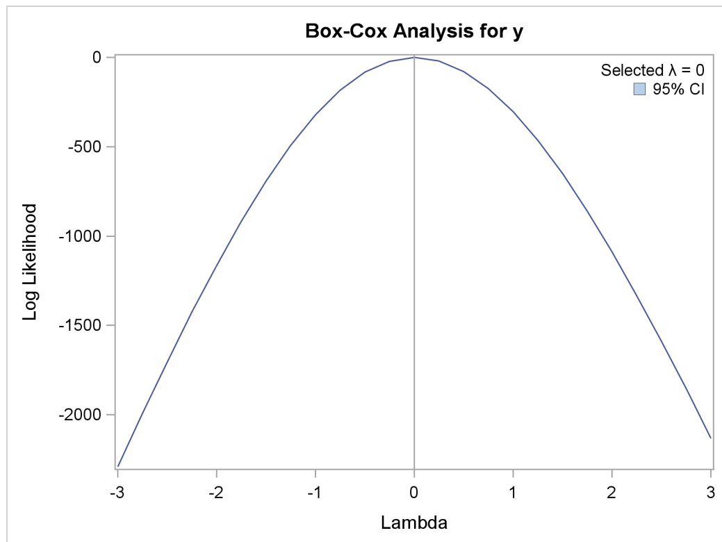
Figure 90.18 Box-Cox with No Independent Variable
