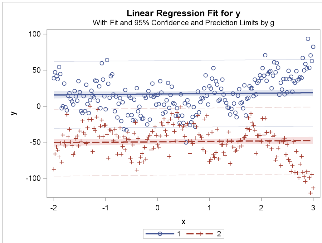
Figure 90.32 Parallel Lines, Separate Intercepts
