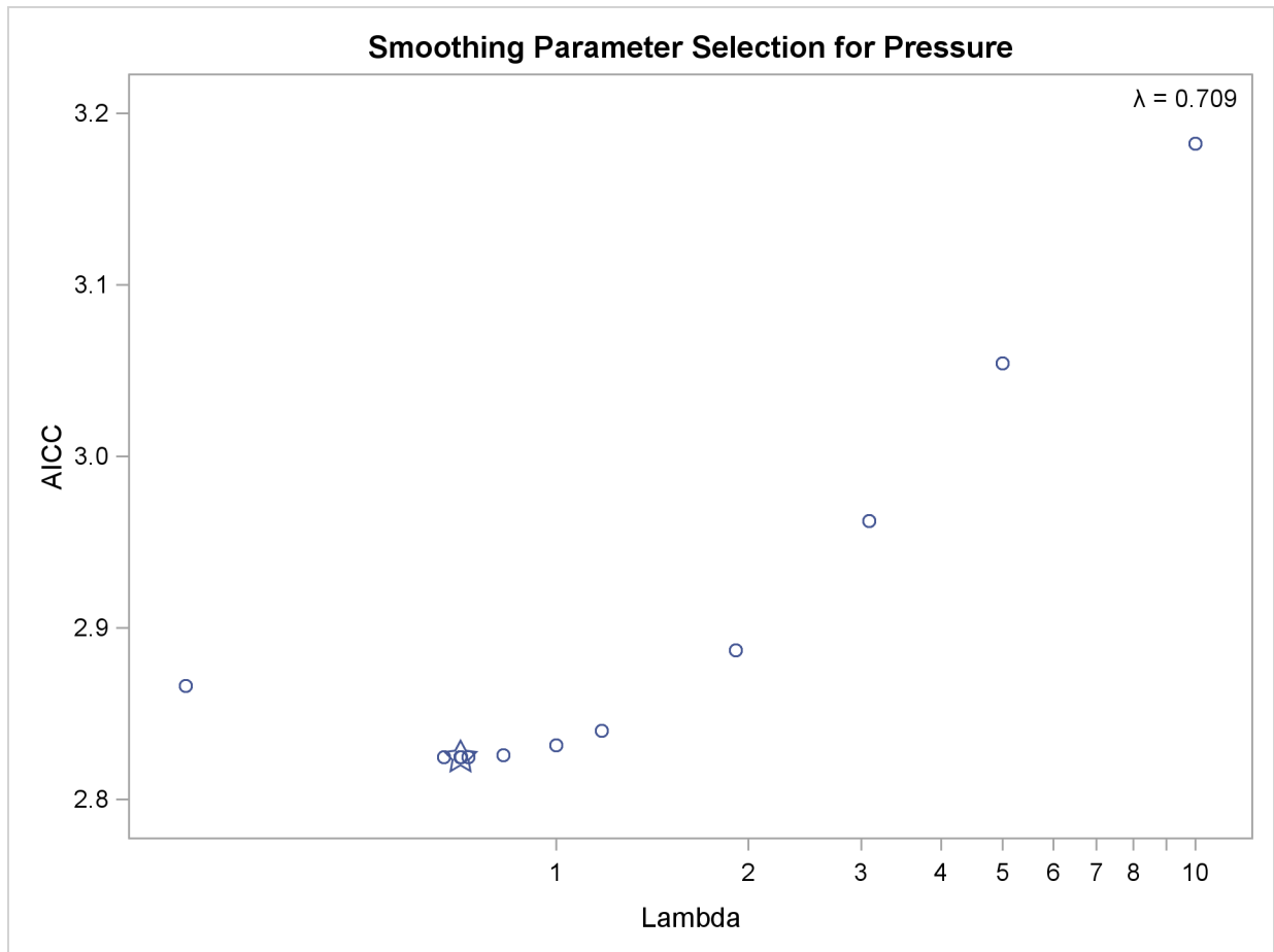
Output 90.3.1 Change in Atmospheric Pressure, AICC
