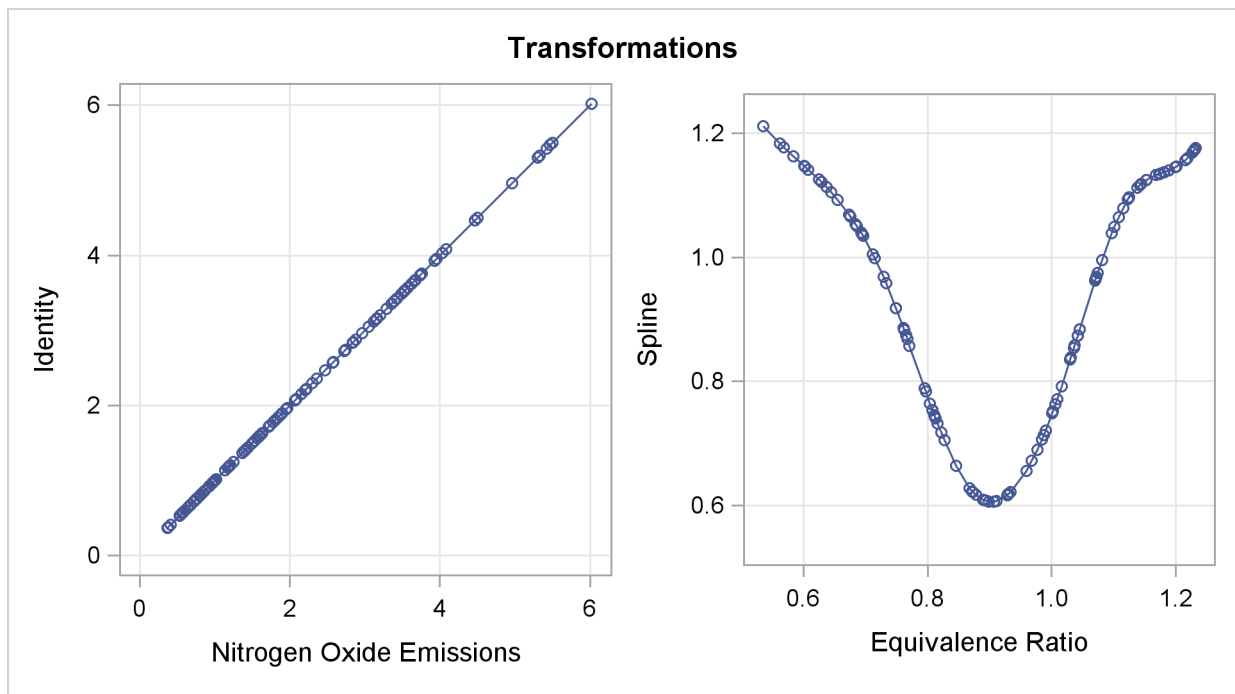
Figure 90.2 Transformations
