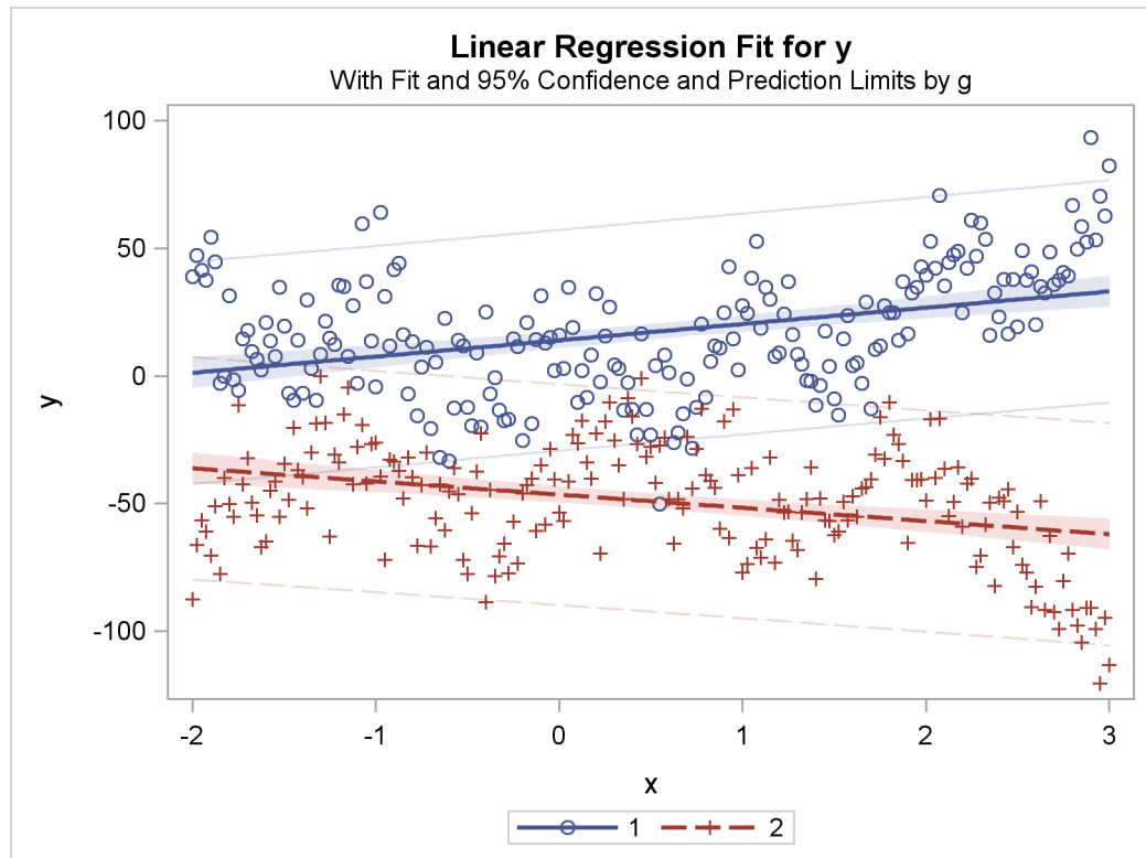
Figure 90.38 Separate Slopes, Separate Intercepts
