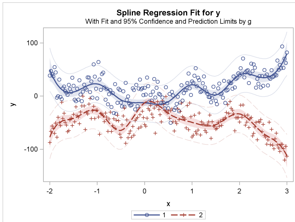
Figure 90.37 Separate Curves, Same Intercept
