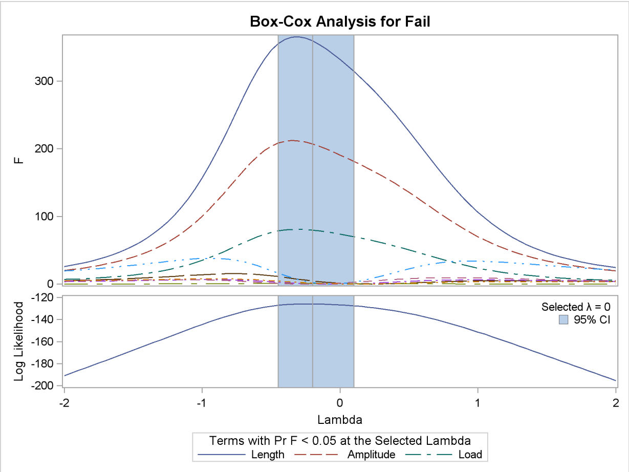
Output 90.2.1 Box-Cox Yarn Data
