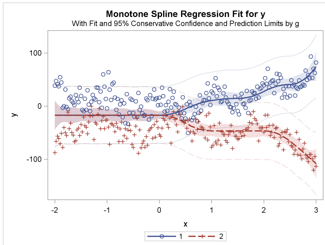
Figure 90.36 Separate Monotone Curves, Same Intercept
