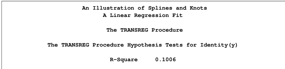
Figure 90.19 A Linear Regression Fit
