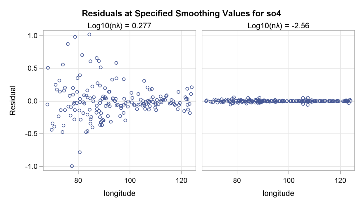
Output 90.3.7 Panel of Residuals by Longitude Plots
