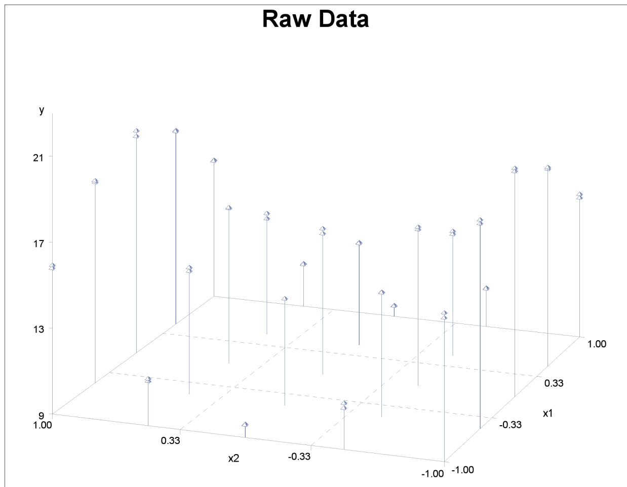
Figure 90.1 Plot of Data Set MEASURE
