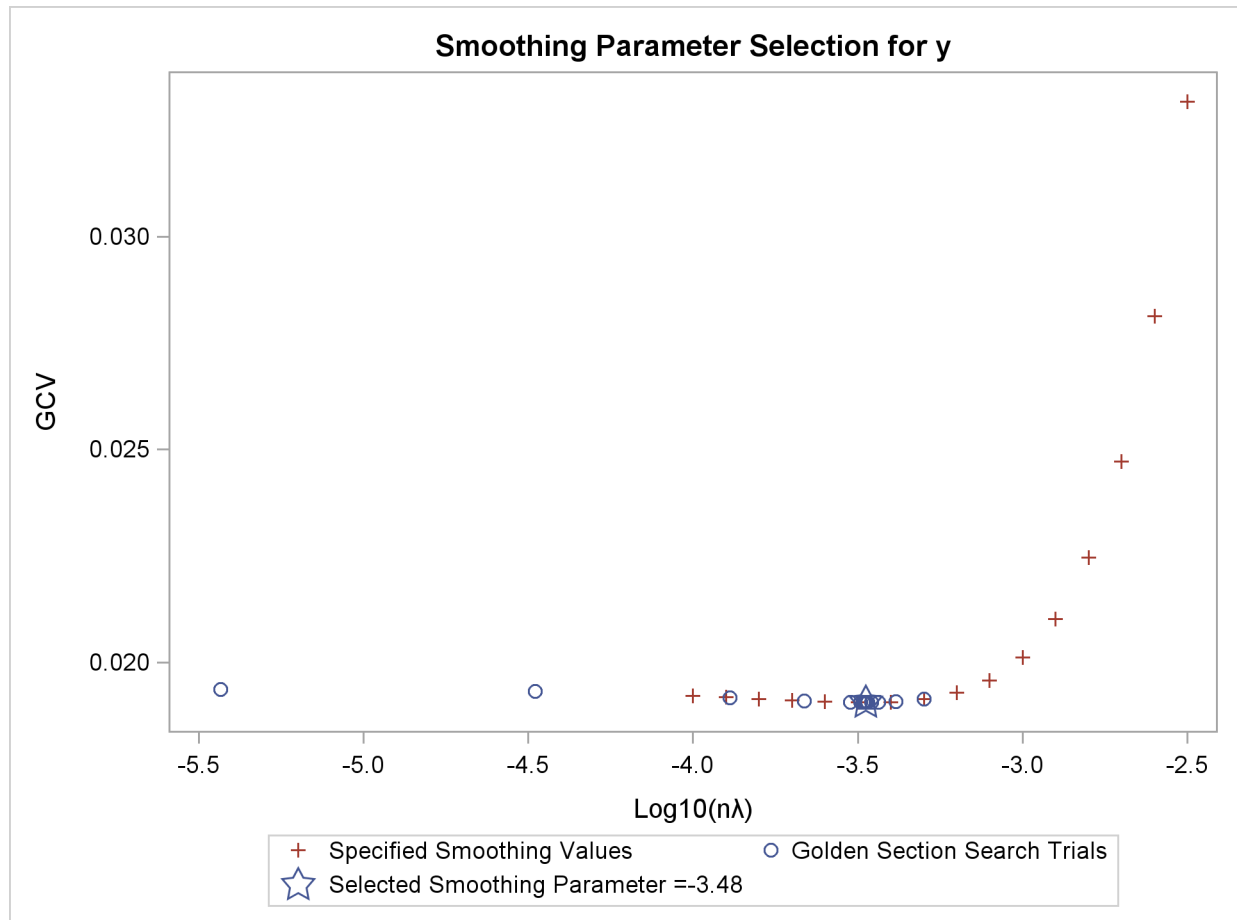
Figure 90.3 The GCV Criterion by \log_{10}(n\lambda)
