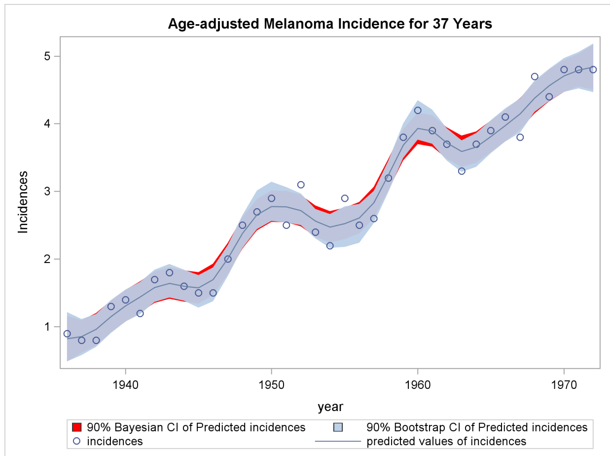
Output 90.5.4 Comparison of Bayesian and Bootstrap Confidence Interval for Data Set MELANOMA
