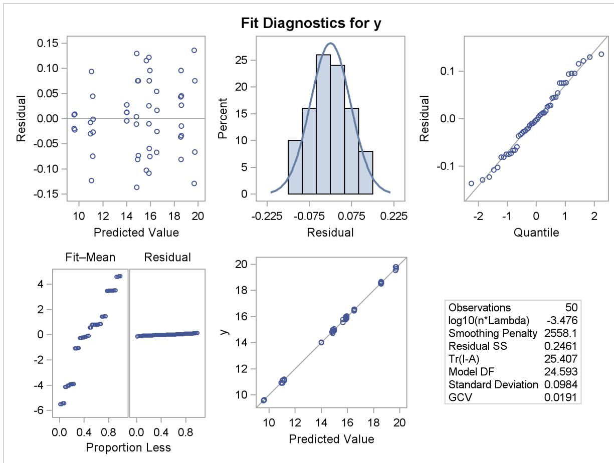
Figure 90.7 Fit Diagnostics
