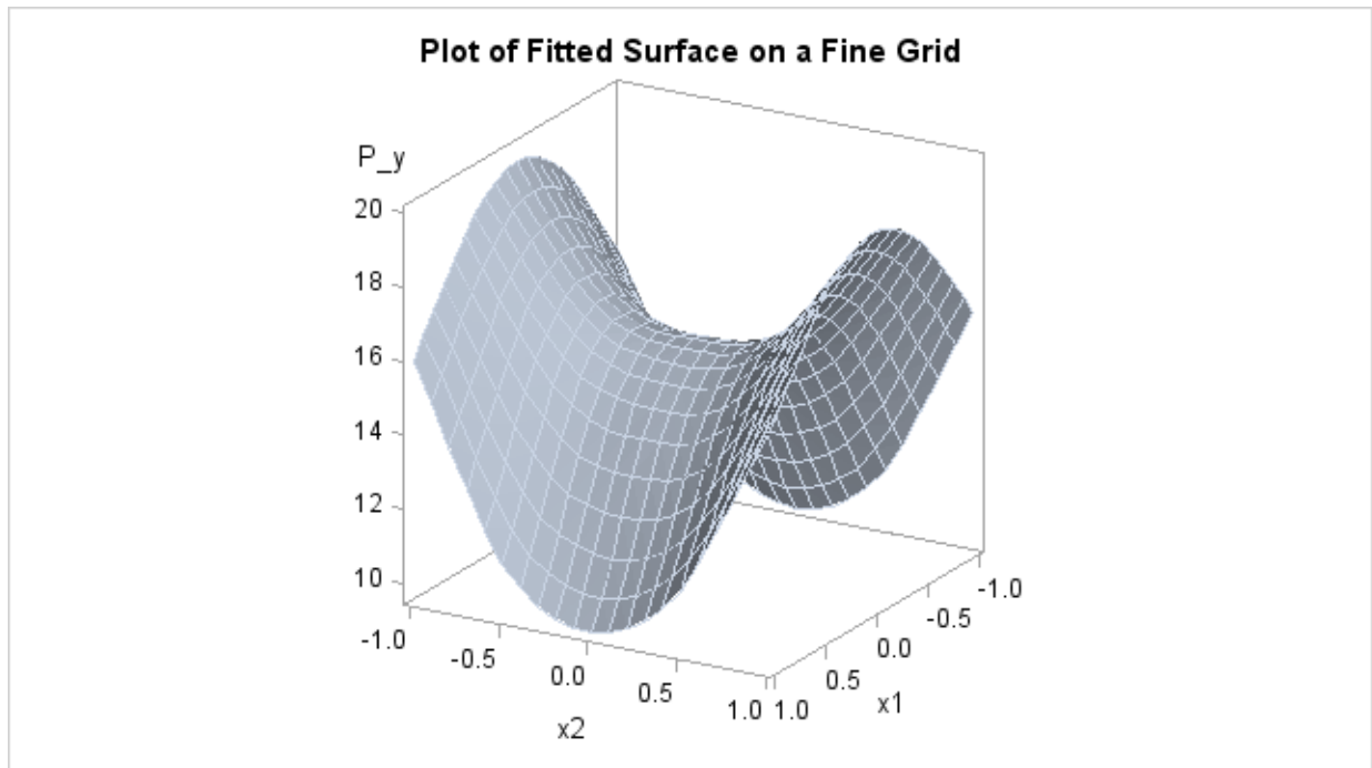
Figure 90.6 Plot of TPSPLINE Fit
