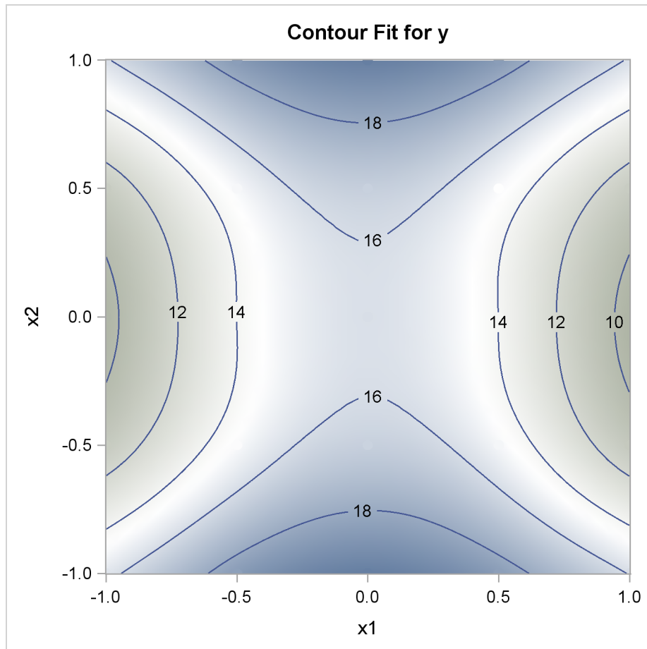
Figure 90.2 Fitted Surface from PROC TPSPLINE
