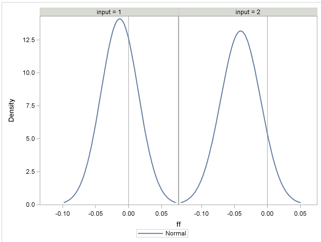
Figure 81.4 Frequency Plot for ff for Each Set of Input Values
