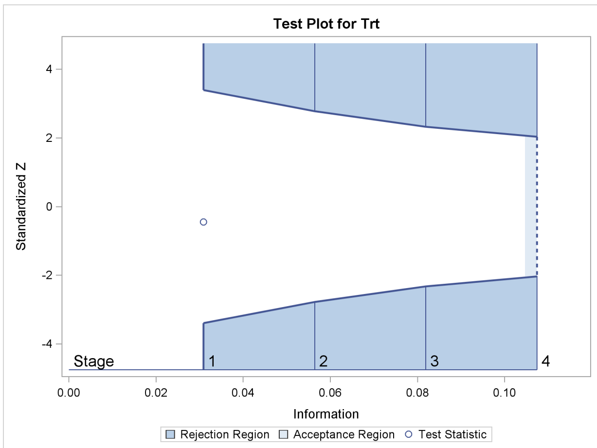
Figure 79.12 Sequential Test Plot
