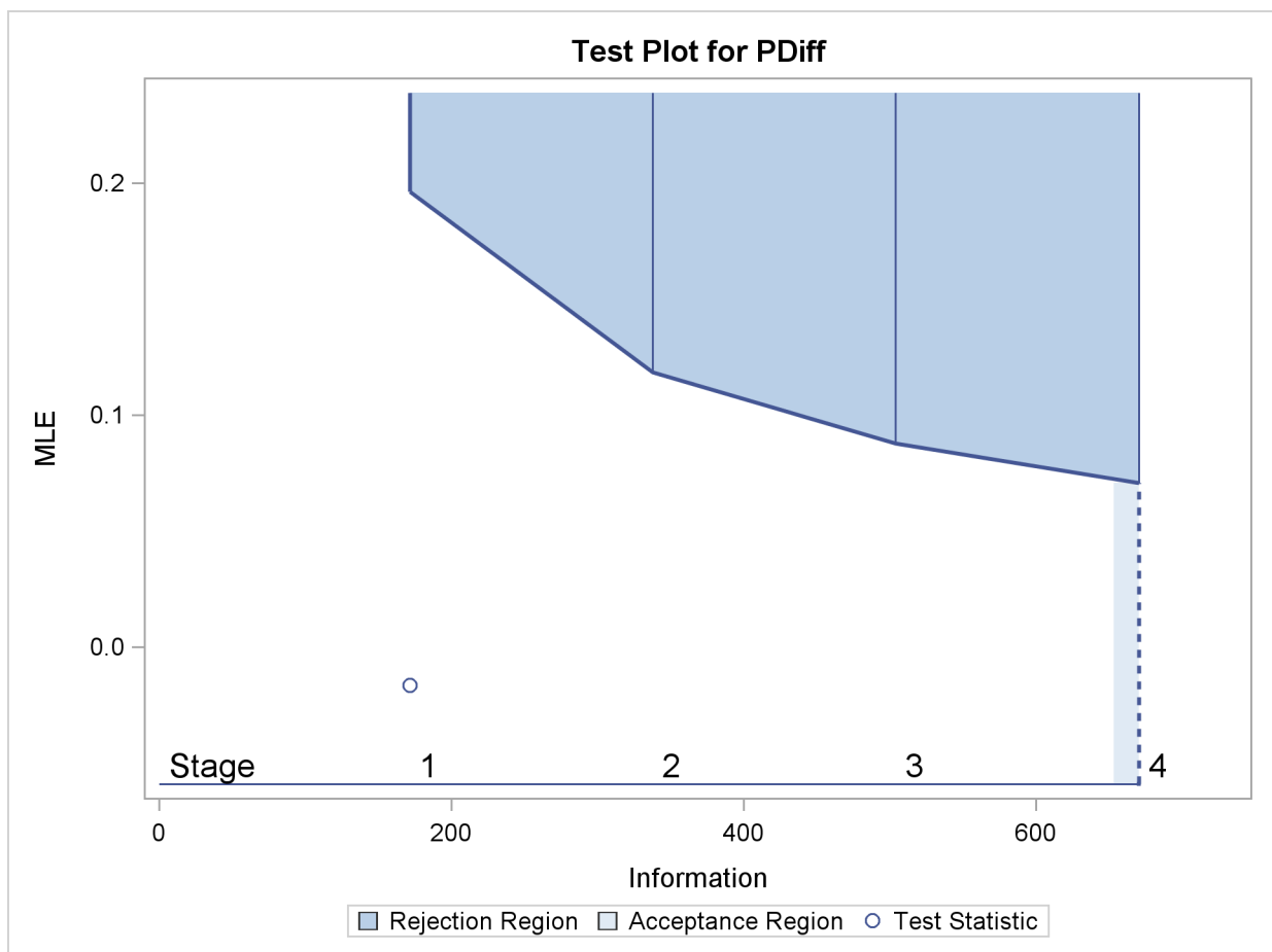
Output 79.4.10 Sequential Test Plot
