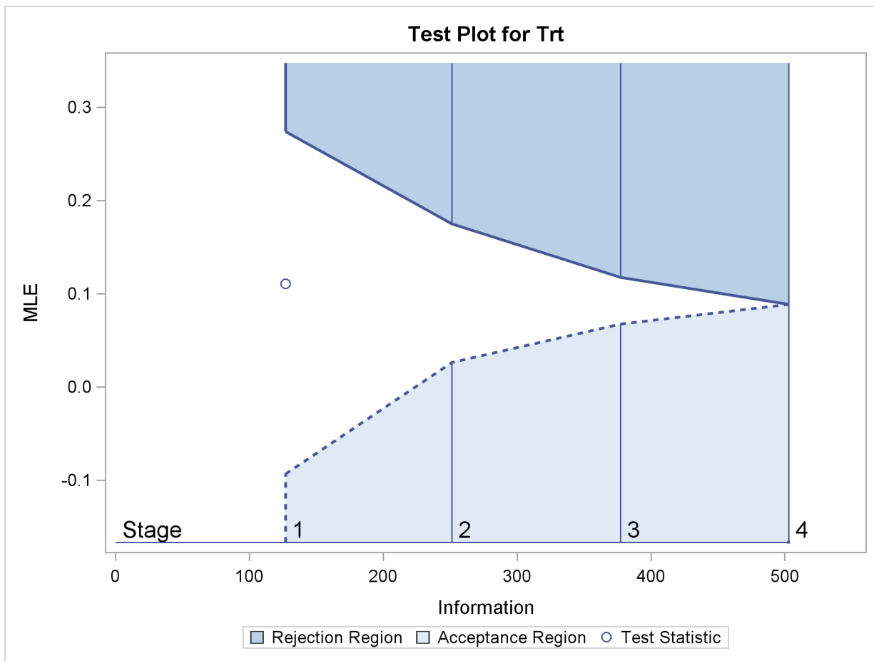
Output 79.1.13 Sequential Test Plot
