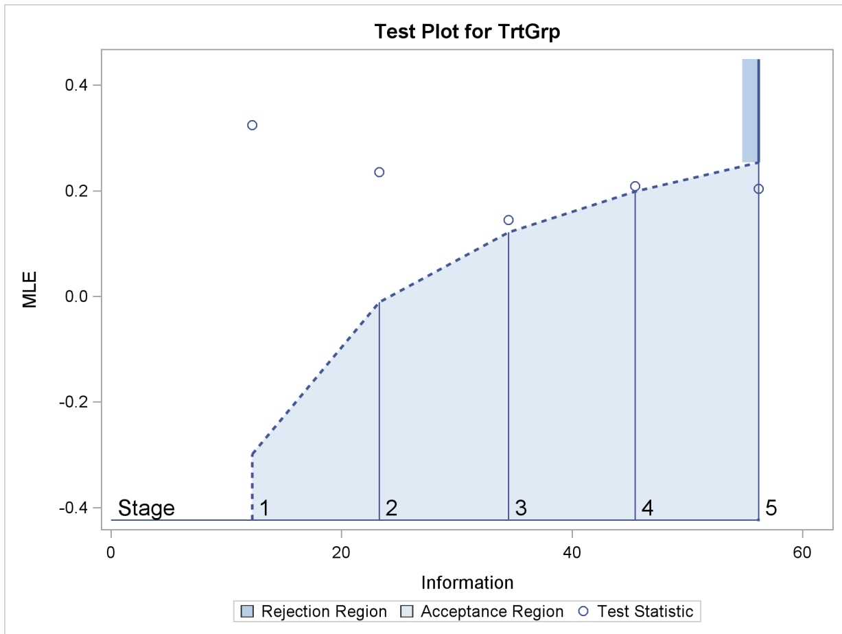
Output 79.5.15 Sequential Test Plot
