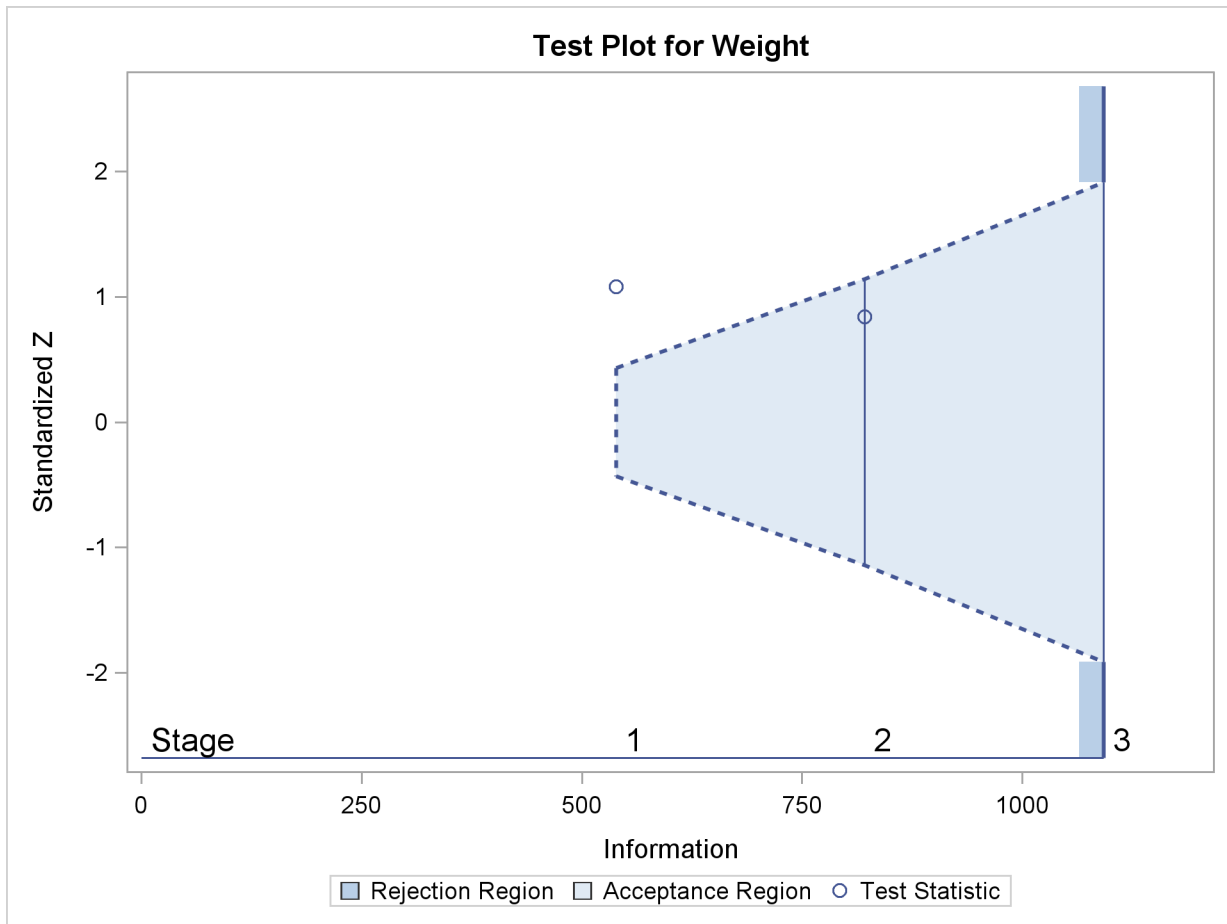
Output 79.3.18 Sequential Test Plot
