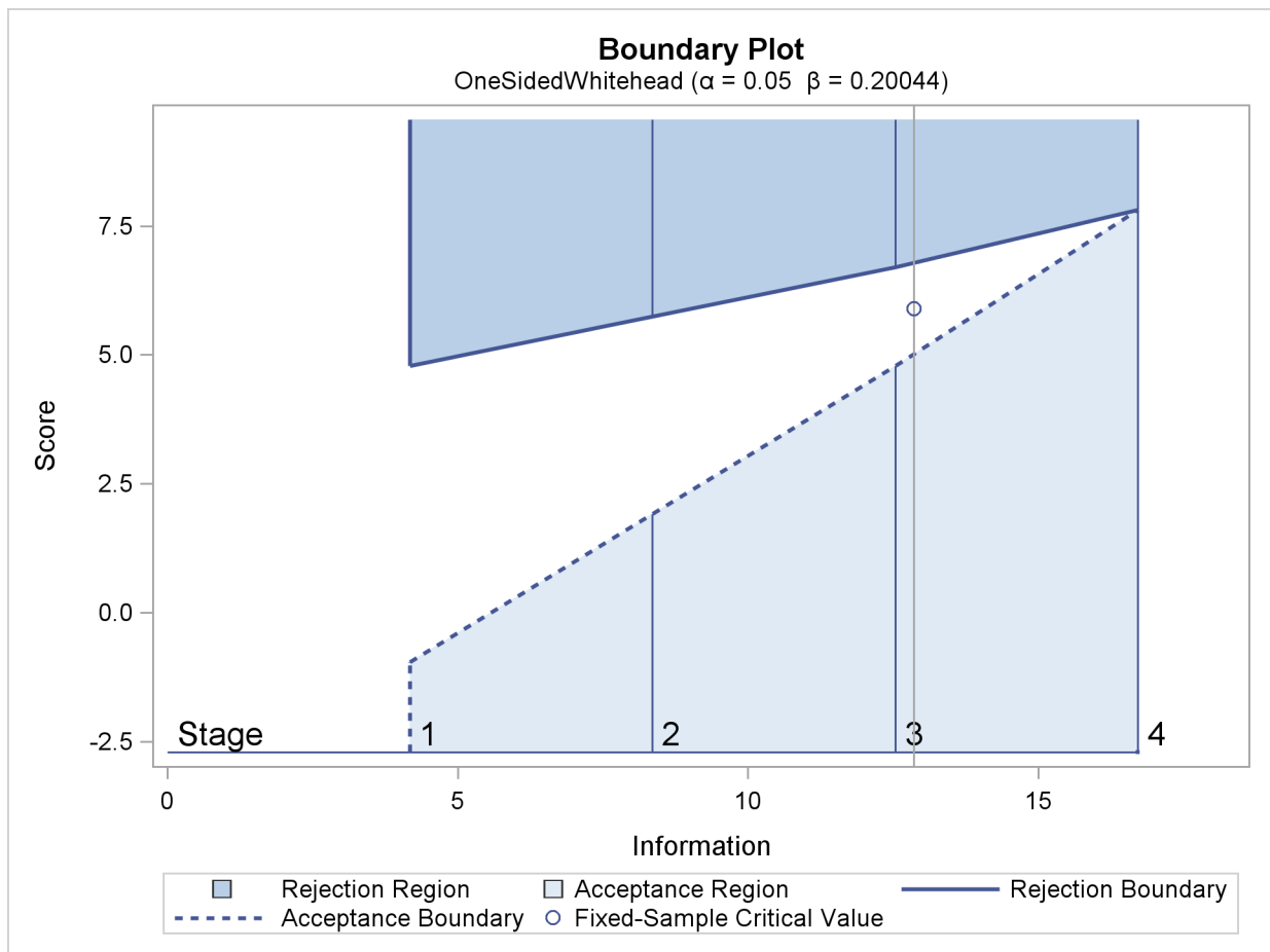
Output 79.6.3 Boundary Plot
