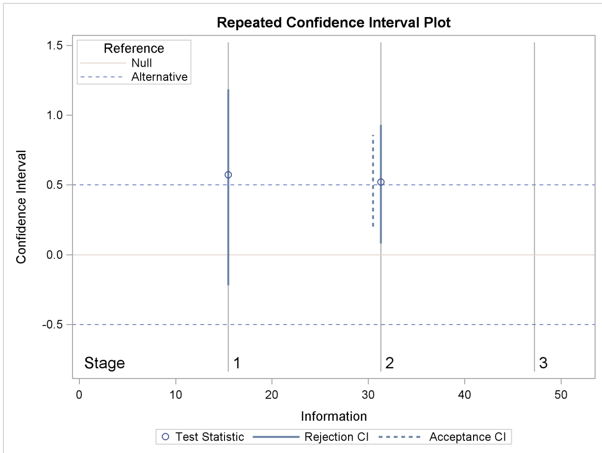
Output 79.8.17 Repeated Confidence Intervals Plot
