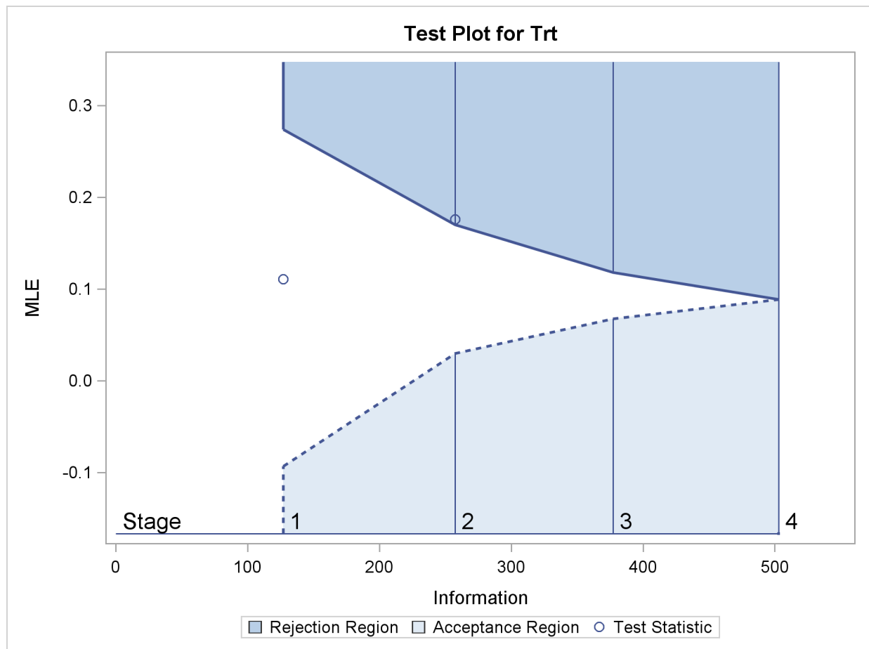
Output 79.1.16 Sequential Test Plot
