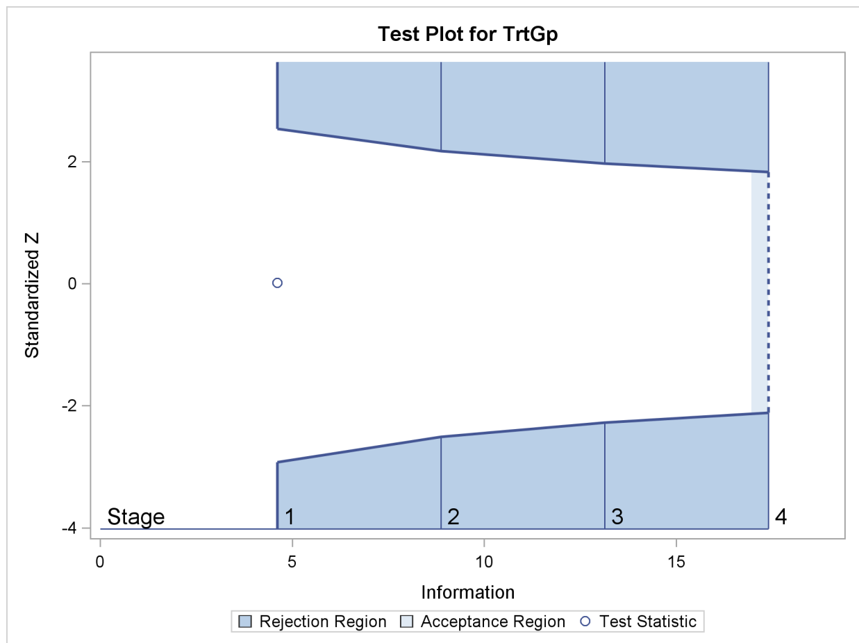
Output 79.7.12 Sequential Test Plot
