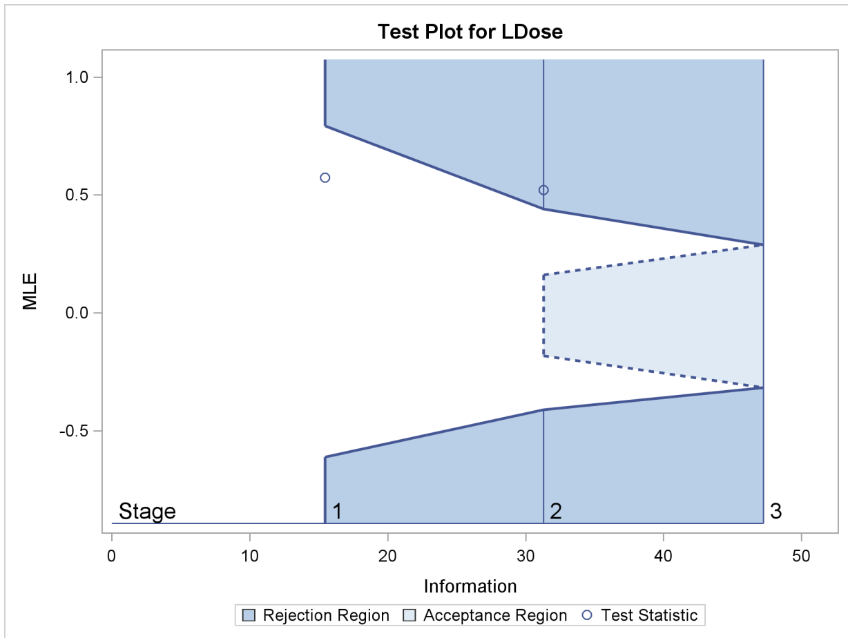
Output 79.8.14 Sequential Test Plot
