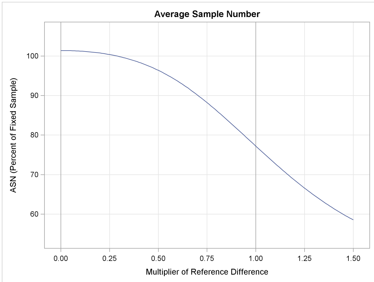
Output 79.2.16 ASN Plot
