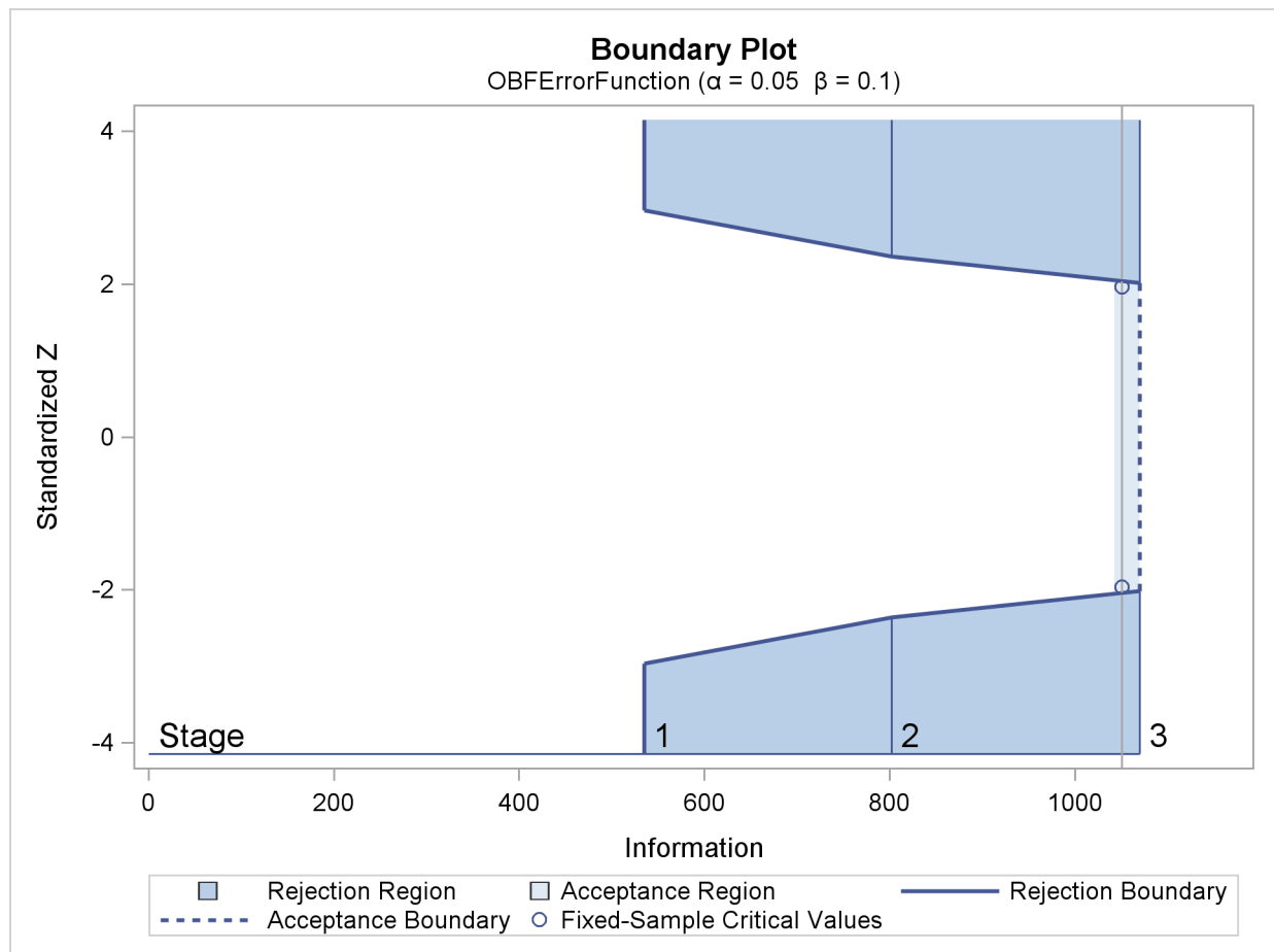
Output 79.2.3 Boundary Plot
