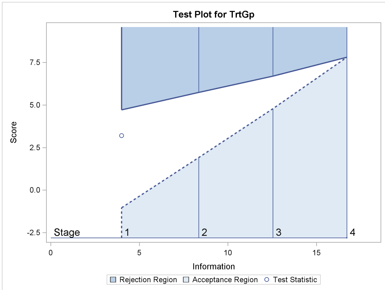
Output 79.6.12 Sequential Test Plot
