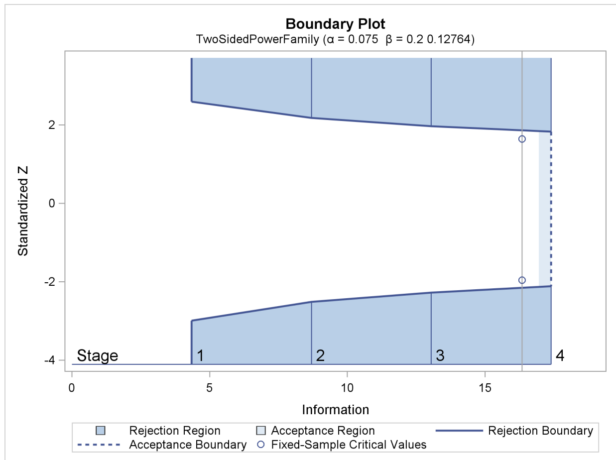
Output 79.7.3 Boundary Plot
