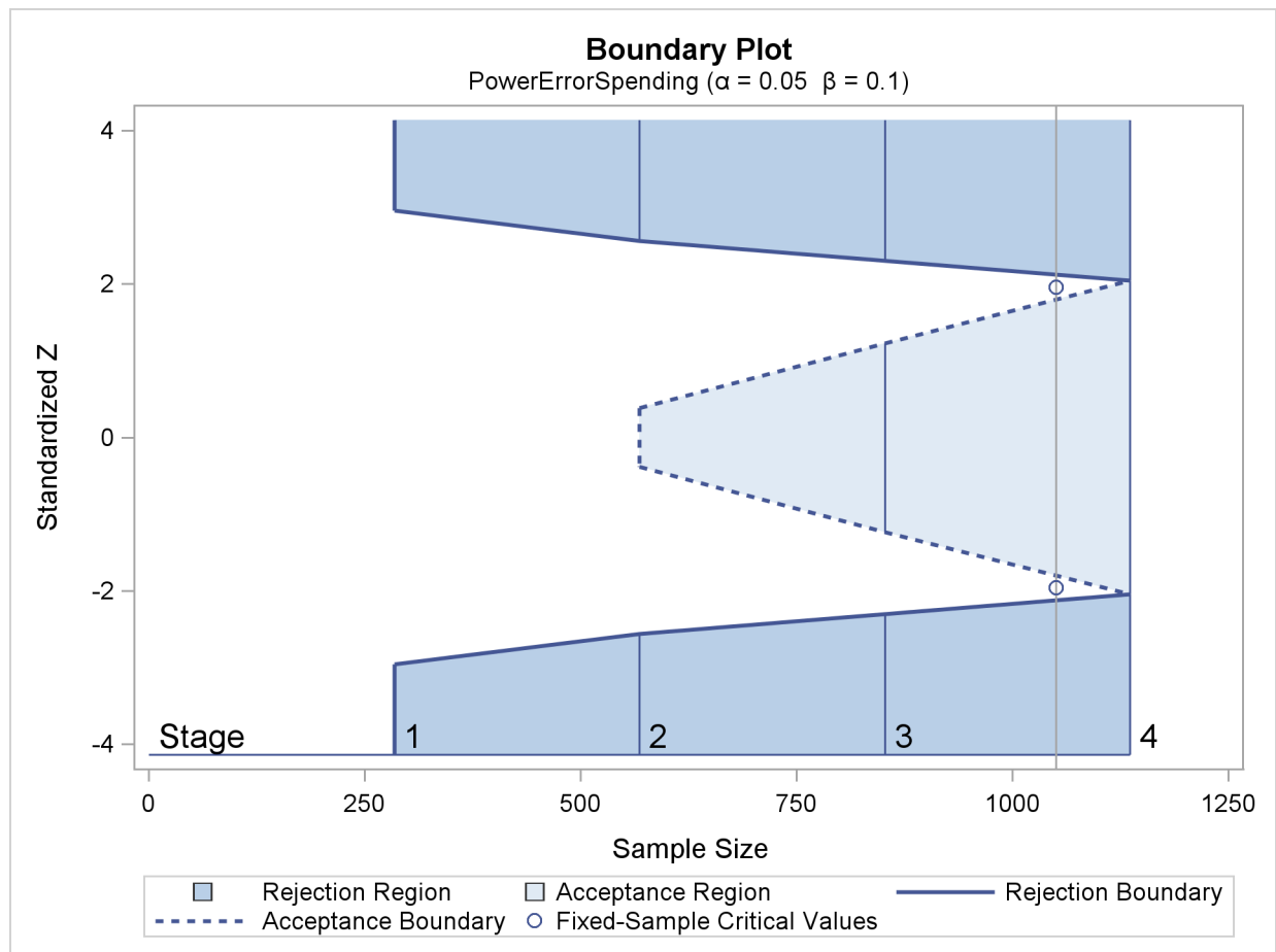
Figure 79.20 Boundary Plot for Two-Sided Test
