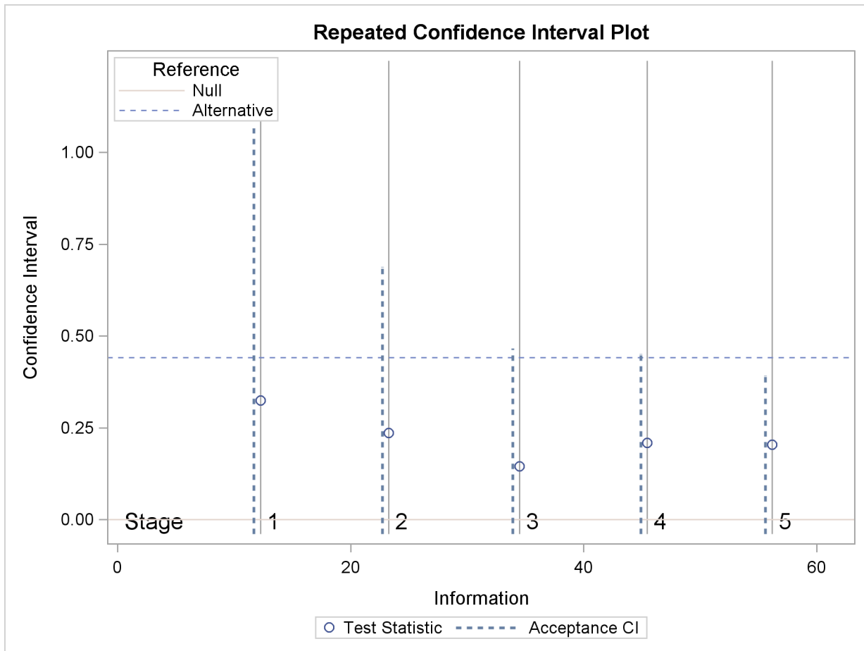
Output 79.5.18 Repeated Confidence Intervals Plot
