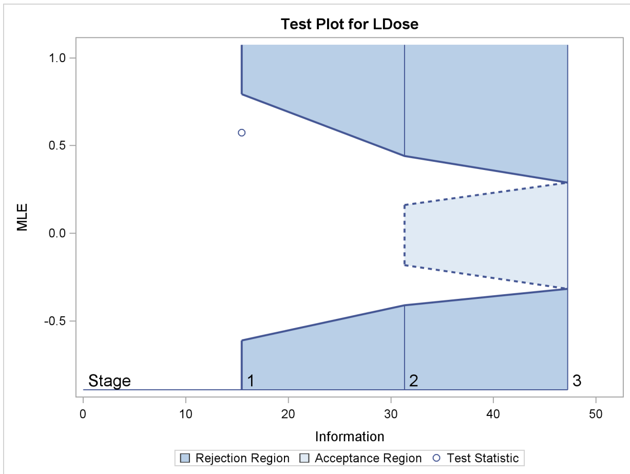
Output 79.8.10 Sequential Test Plot
