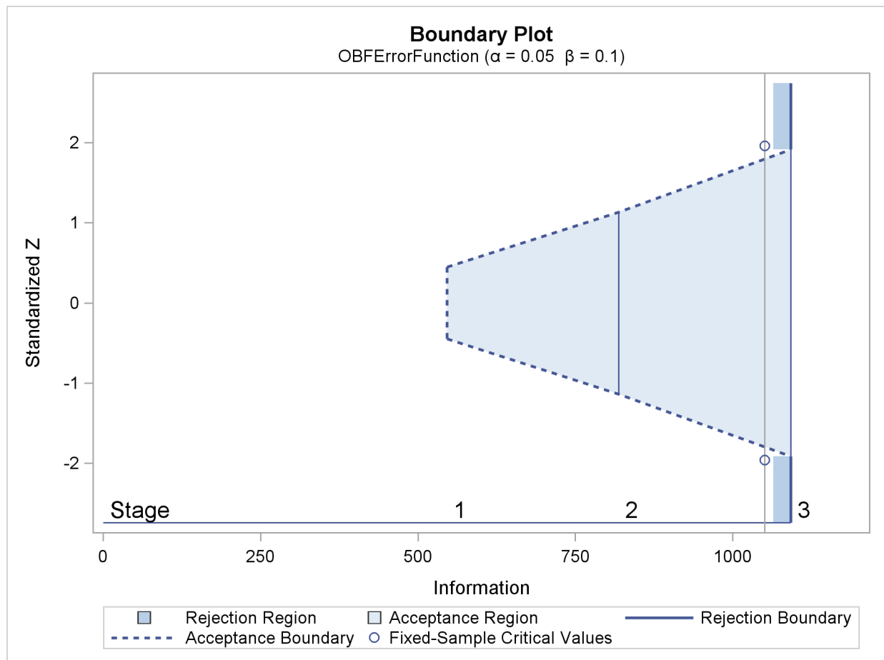
Output 79.3.3 Boundary Plot
