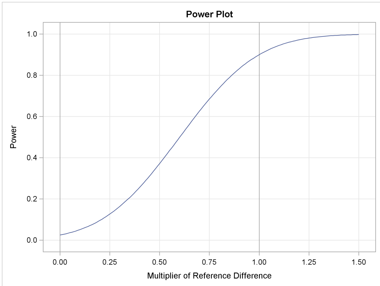
Output 79.3.16 Power Plot
