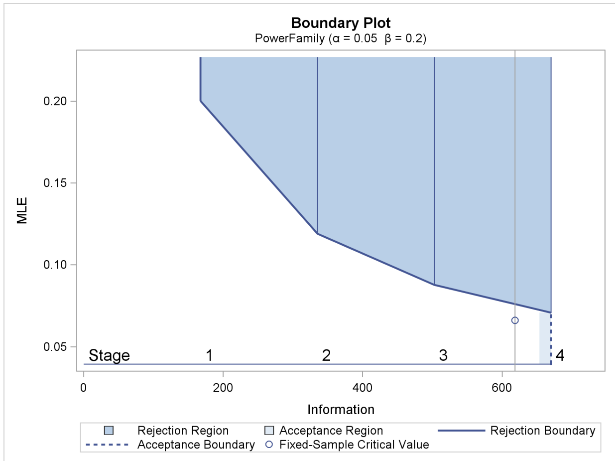
Output 79.4.3 Boundary Plot
