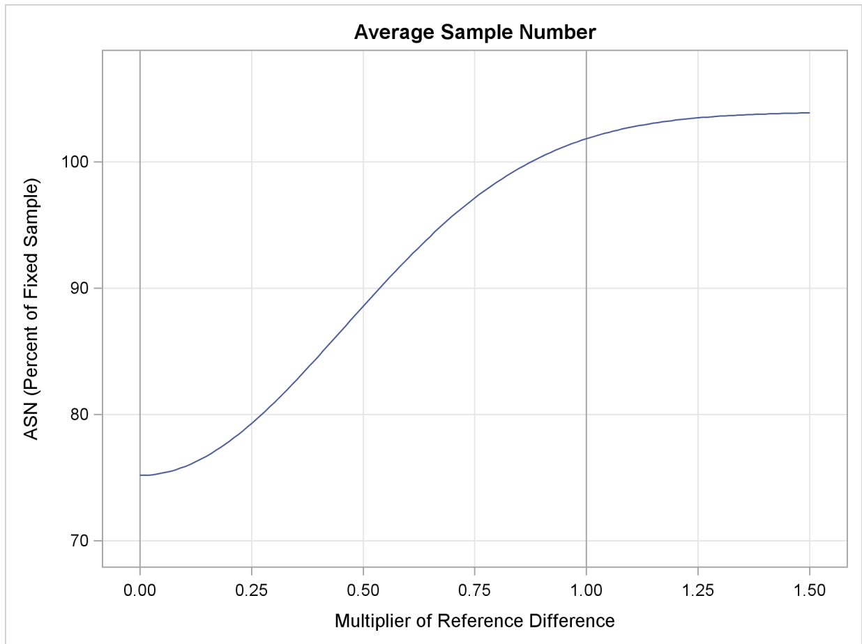
Output 79.3.15 ASN Plot
