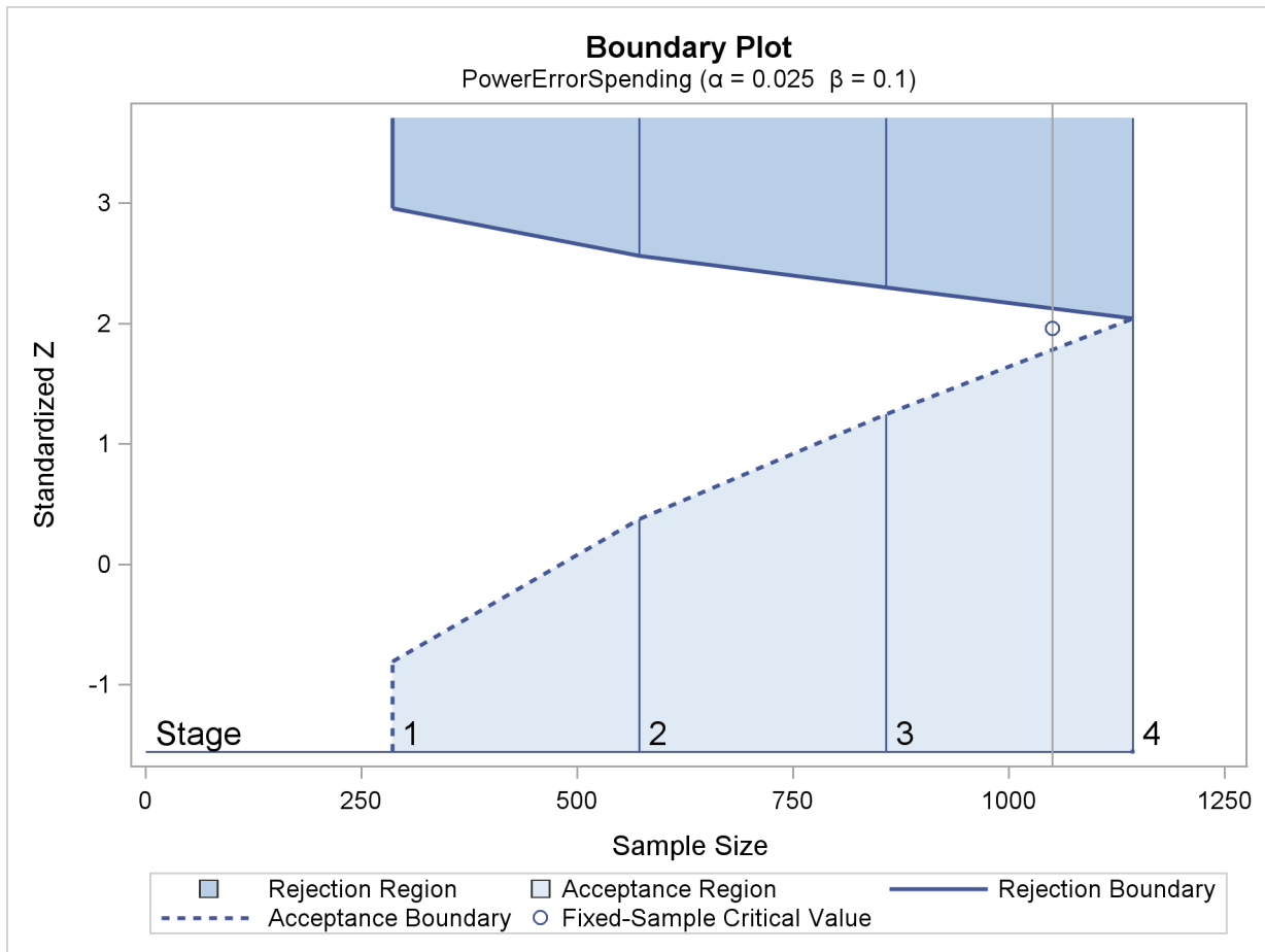
Figure 79.19 Boundary Plot for One-Sided Test
