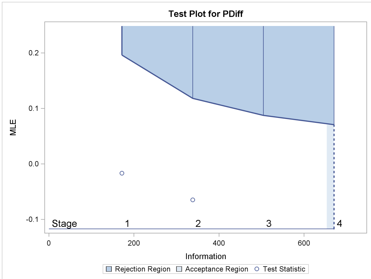
Output 79.4.13 Sequential Test Plot
