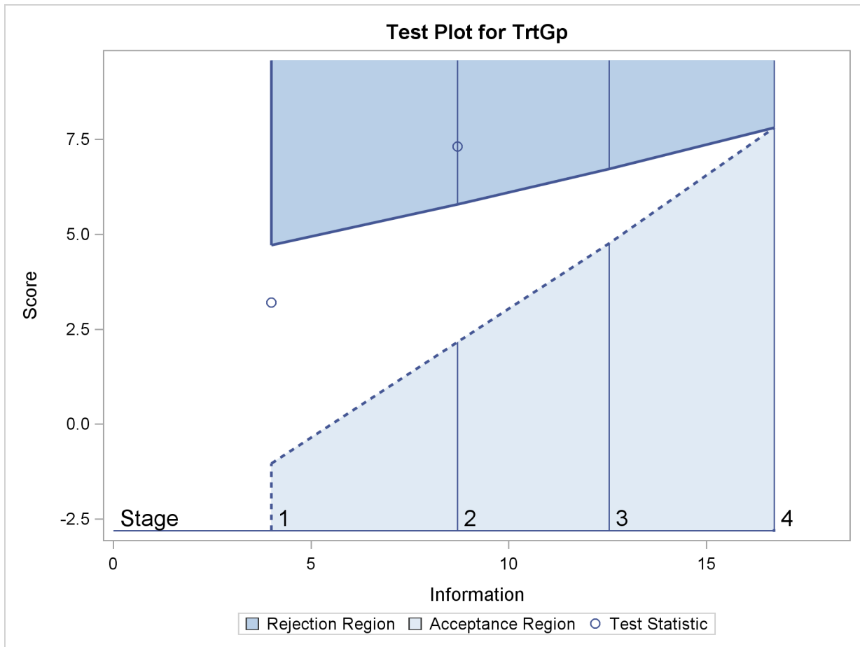
Output 79.6.16 Sequential Test Plot
