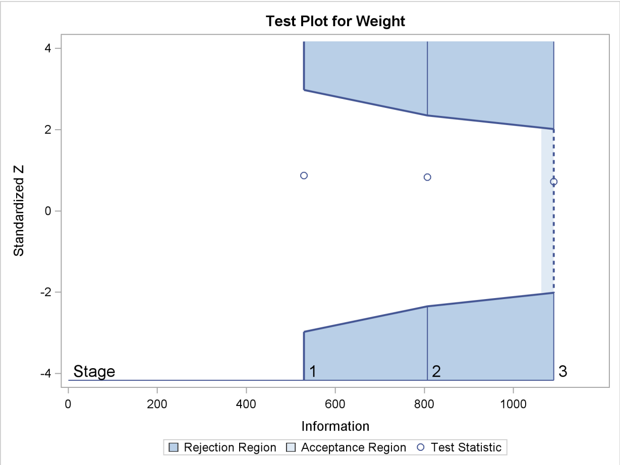
Output 79.2.19 Sequential Test Plot
