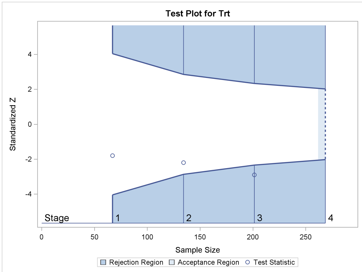
Figure 79.1 Sequential Plot for Two-Sided Test
