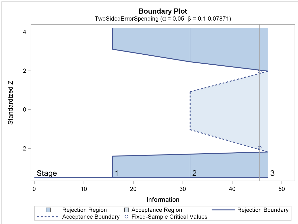
Output 79.8.3 Boundary Plot
