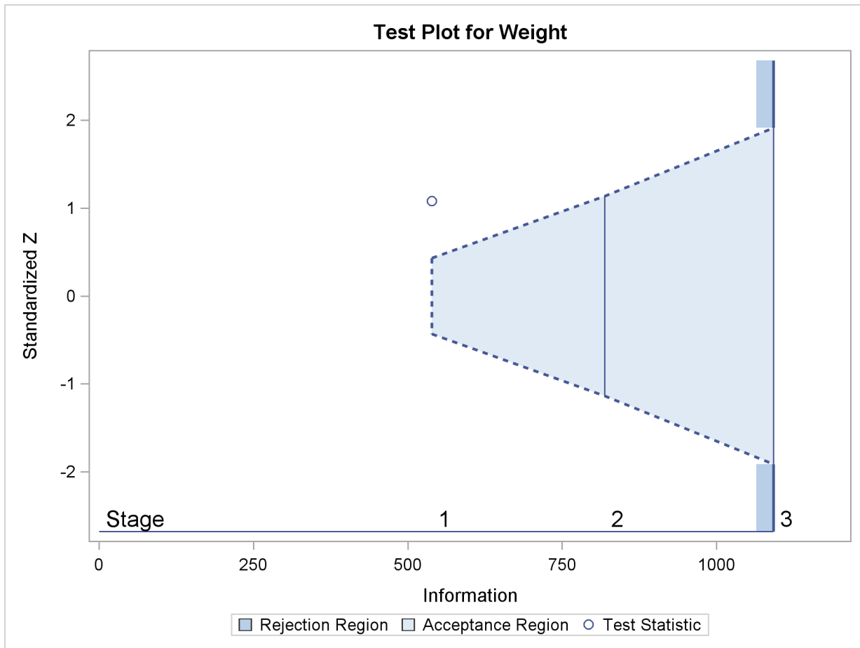
Output 79.3.11 Sequential Test Plot
