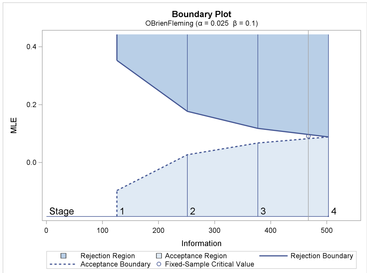
Output 79.1.3 O'Brien-Fleming Boundary Plot
