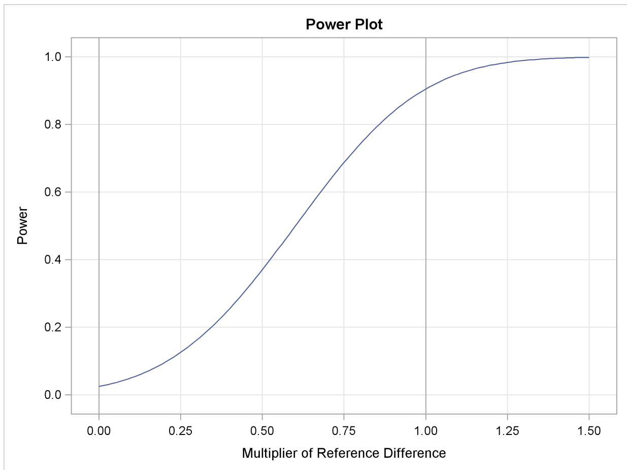
Output 79.2.17 Power Plot
