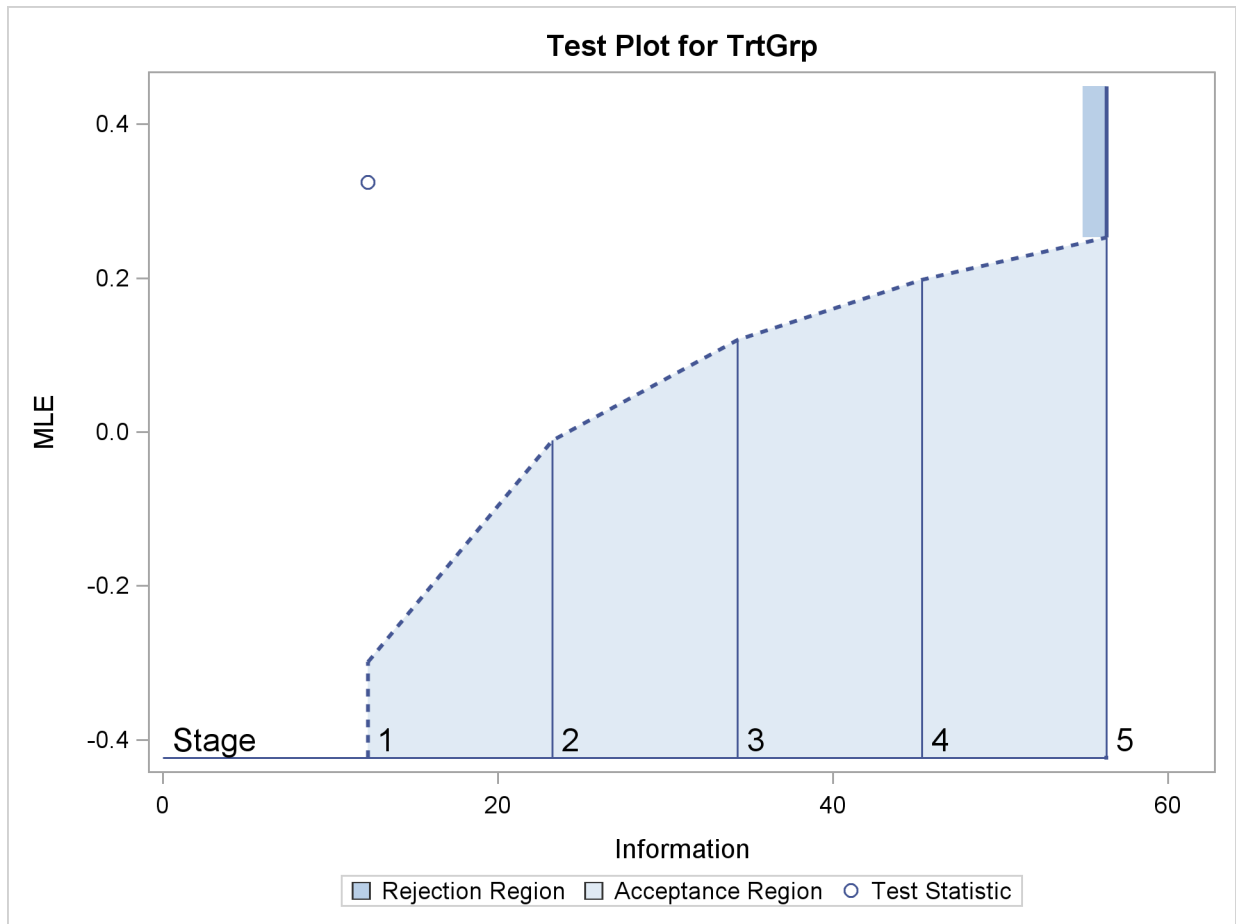
Output 79.5.10 Sequential Test Plot
