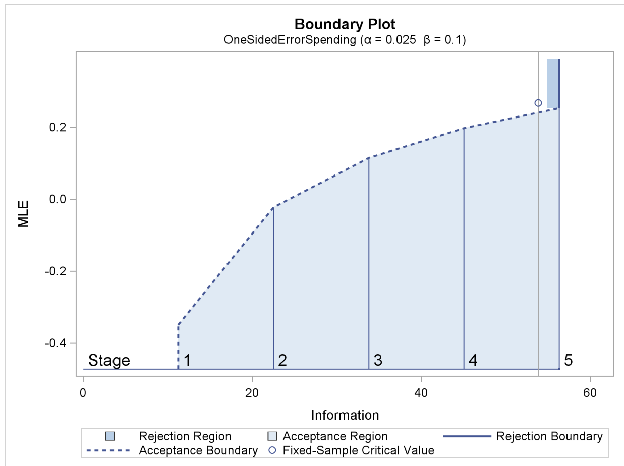
Output 78.5.3 Boundary Plot
