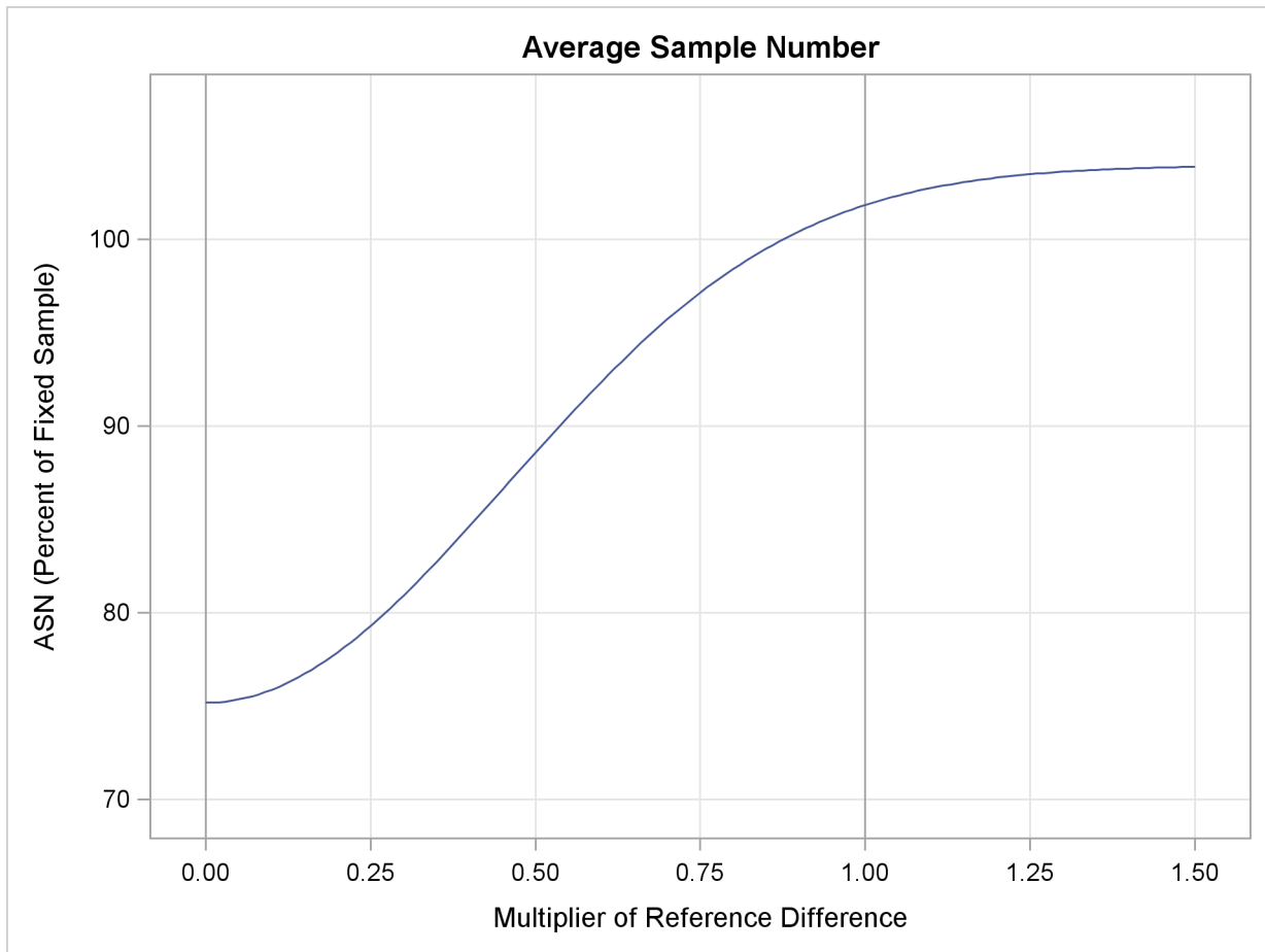
Output 78.3.15 ASN Plot
