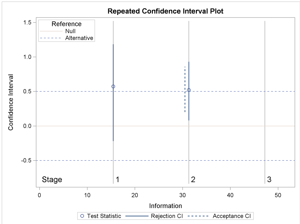
Output 78.8.17 Repeated Confidence Intervals Plot
