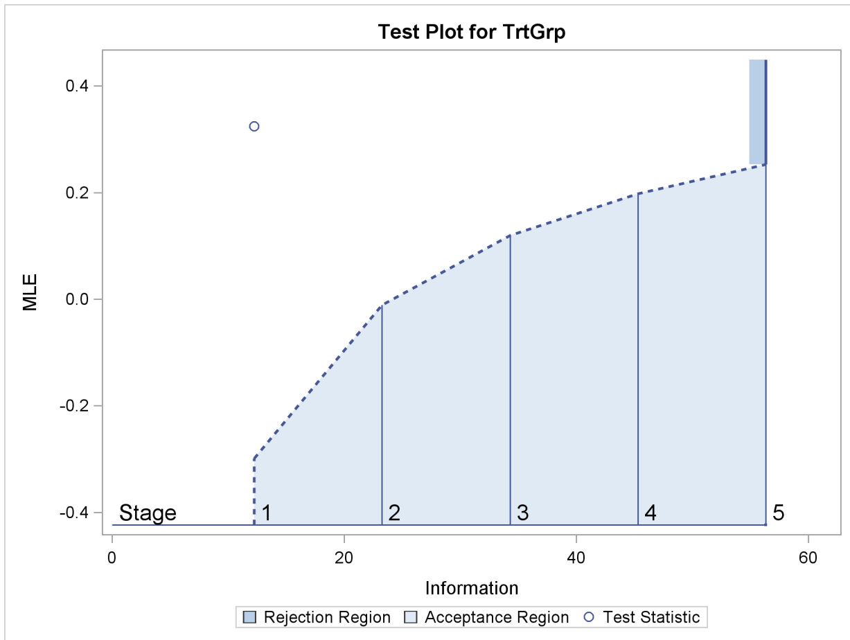
Output 78.5.10 Sequential Test Plot
