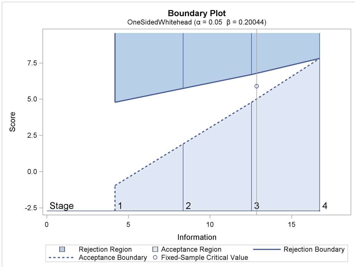
Output 78.6.3 Boundary Plot
