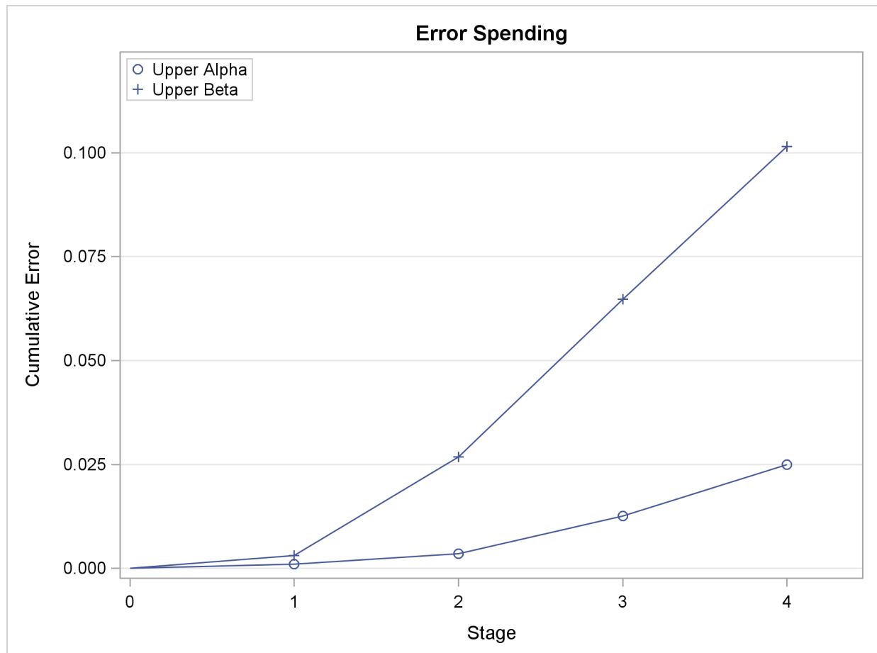
Output 78.1.11 Error Spending Plot
