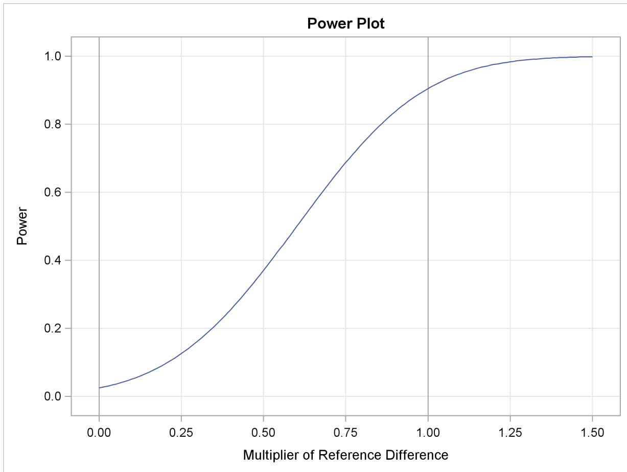
Output 78.2.17 Power Plot
