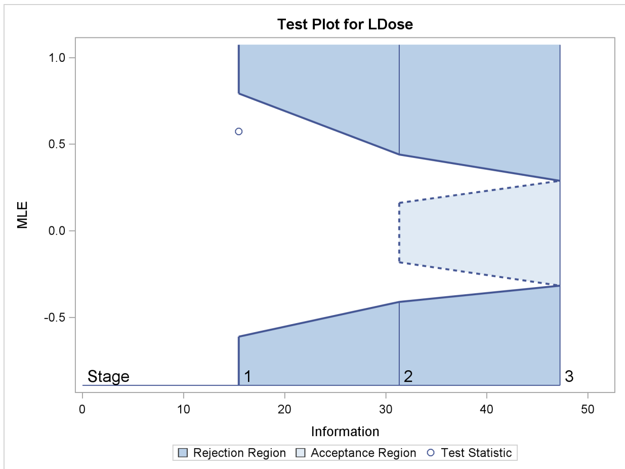
Output 78.8.10 Sequential Test Plot
