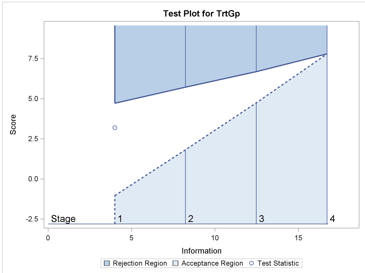
Output 78.6.12 Sequential Test Plot
