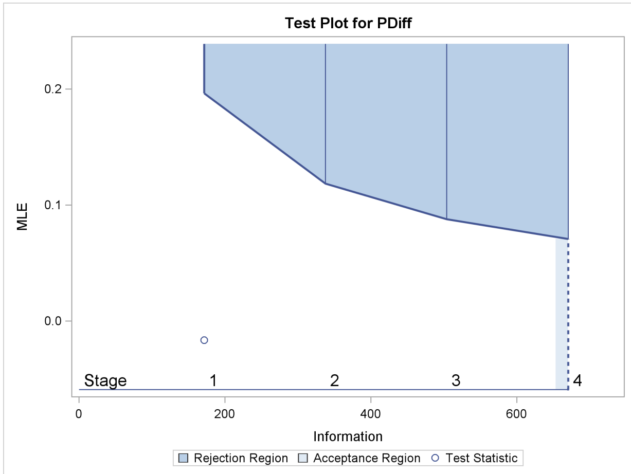
Output 78.4.10 Sequential Test Plot
