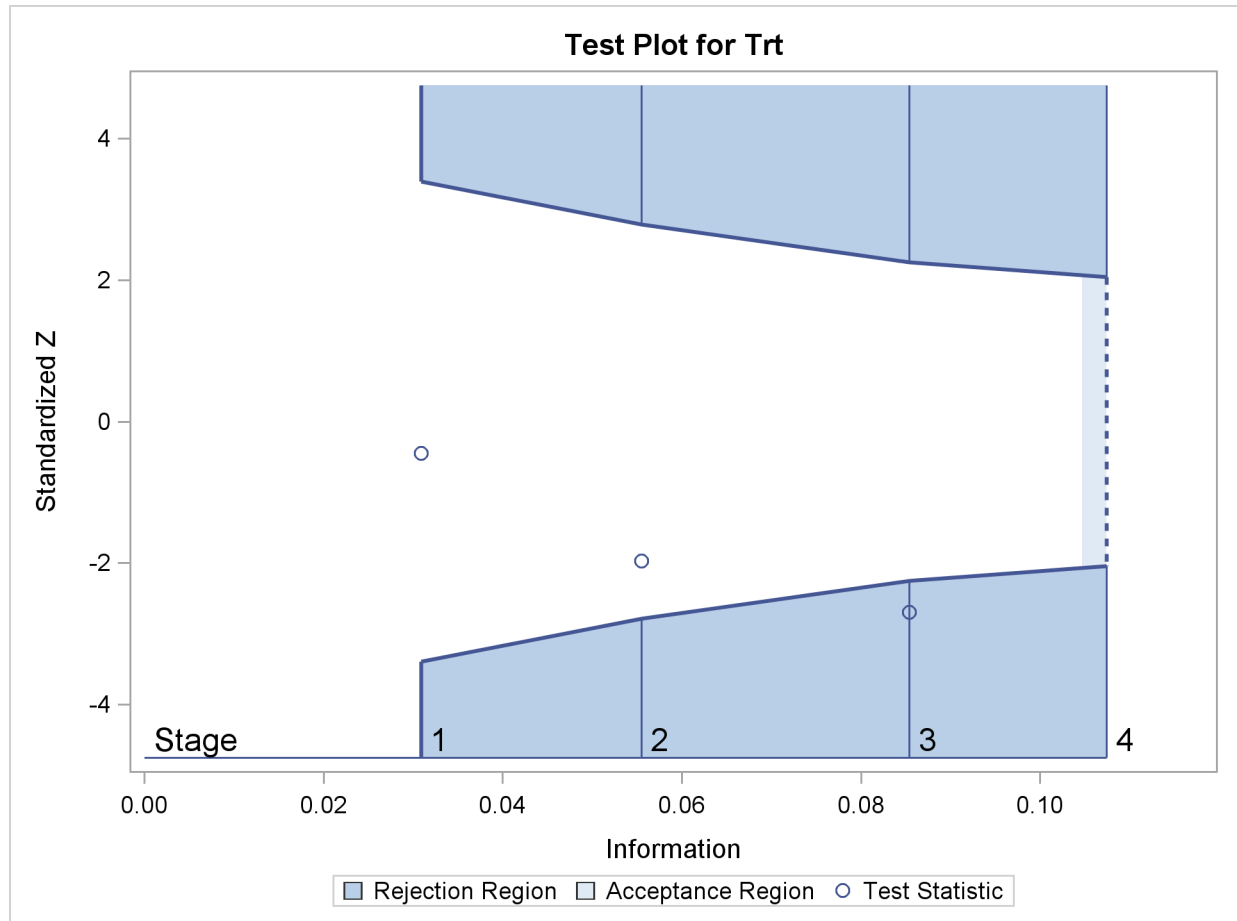
Figure 78.17 Sequential Test Plot
