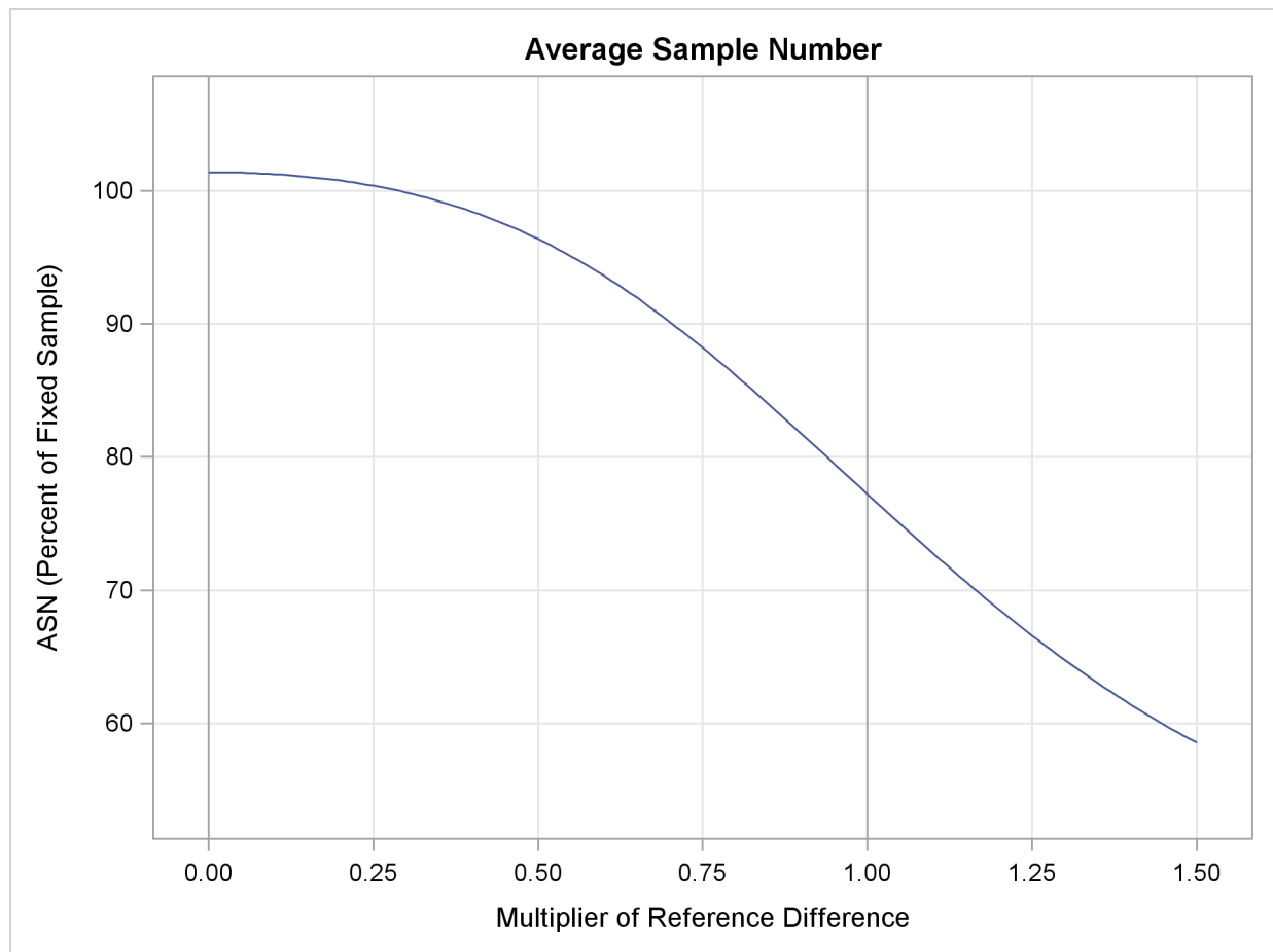
Output 78.2.16 ASN Plot
