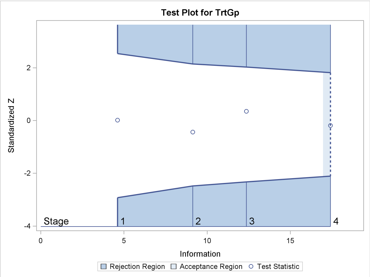
Output 78.7.16 Sequential Test Plot
