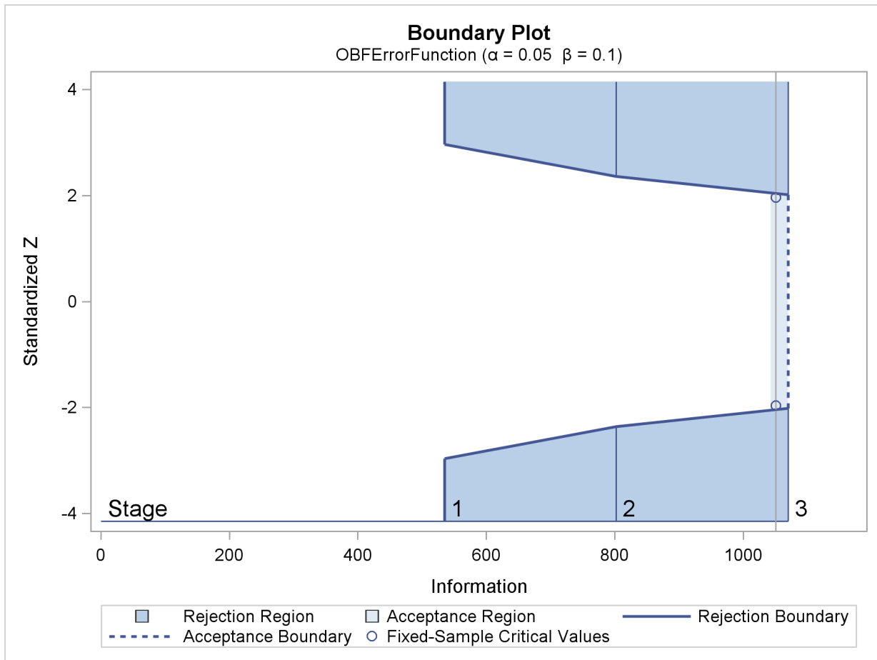
Output 78.2.3 Boundary Plot
