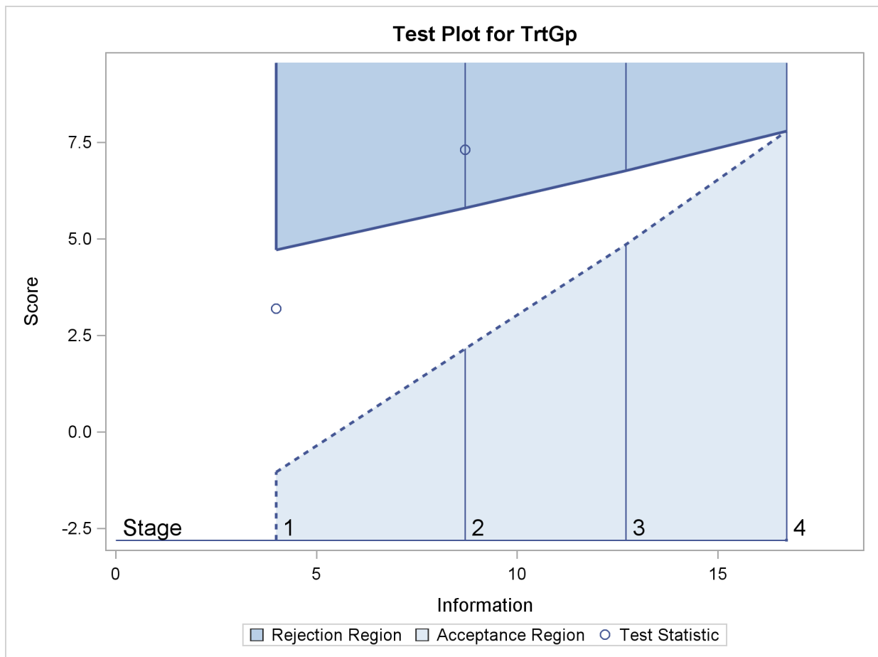
Output 78.6.16 Sequential Test Plot
