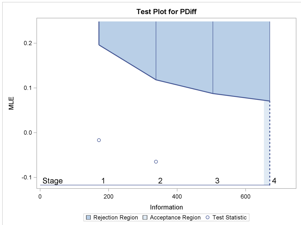
Output 78.4.13 Sequential Test Plot
