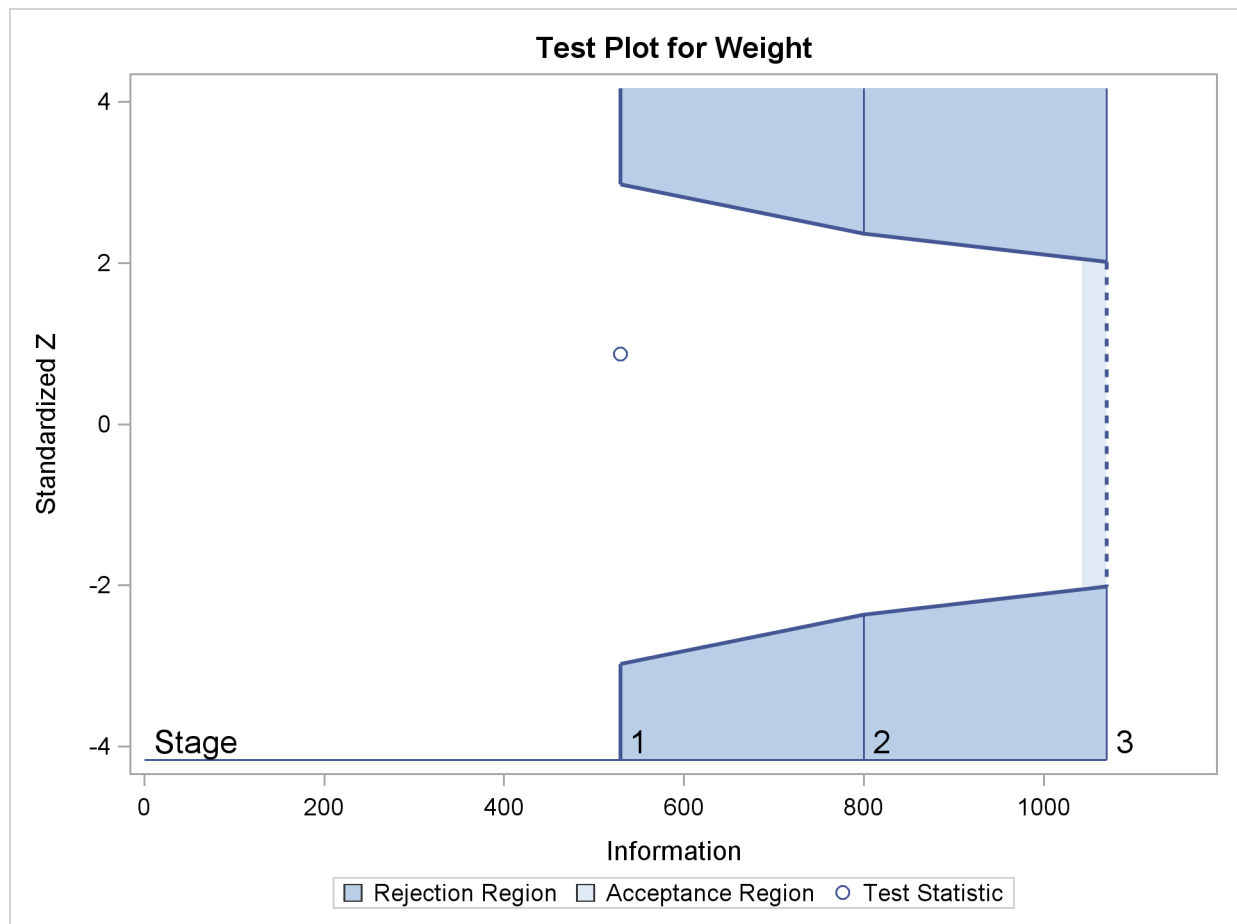
Output 78.2.11 Sequential Test Plot
