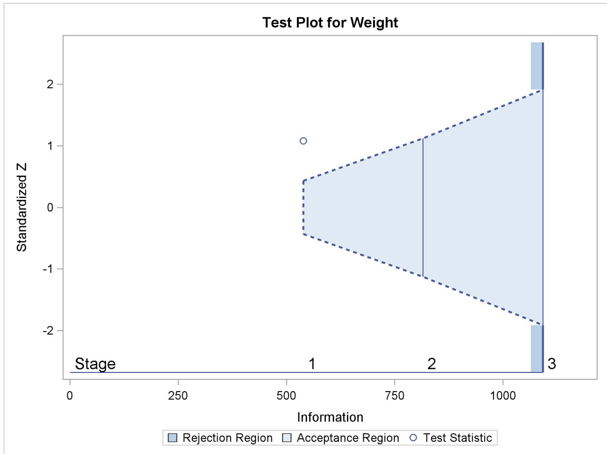
Output 78.3.11 Sequential Test Plot
