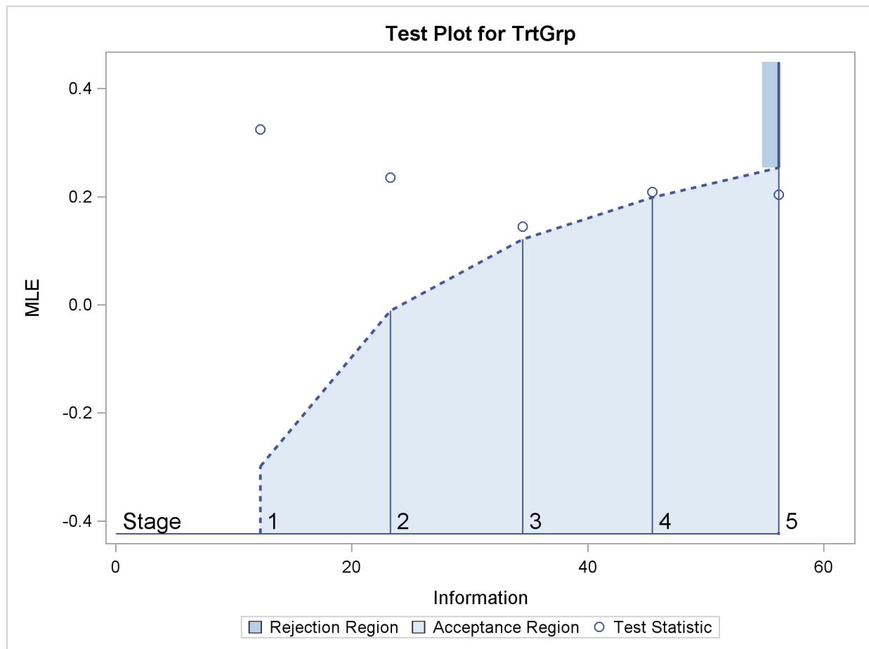
Output 78.5.15 Sequential Test Plot
