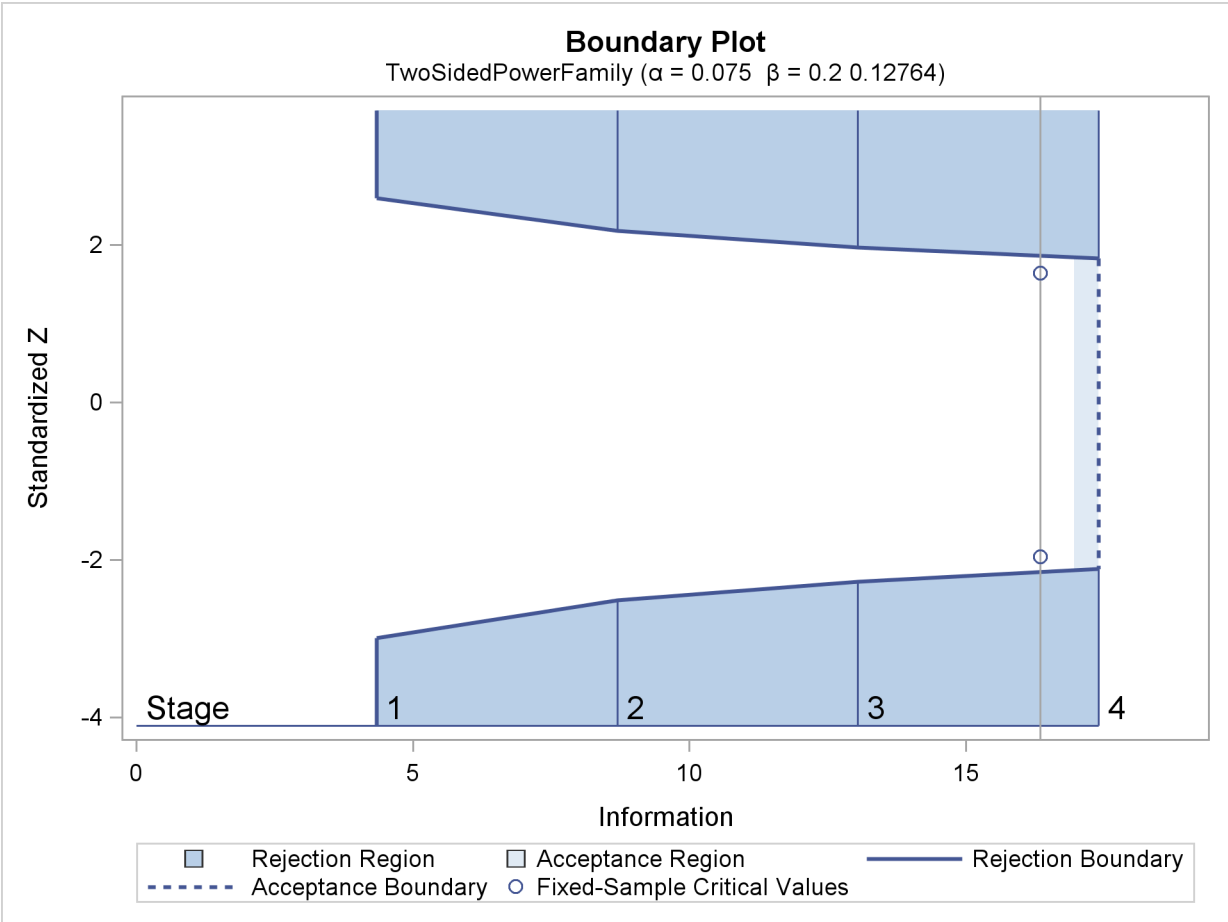
Output 78.7.3 Boundary Plot
