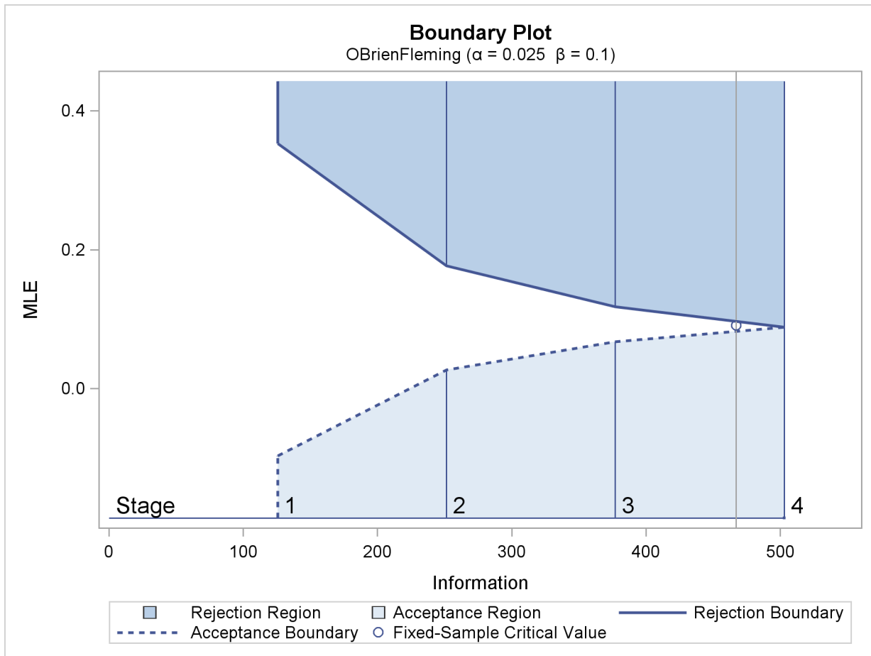
Output 78.1.3 O'Brien-Fleming Boundary Plot
