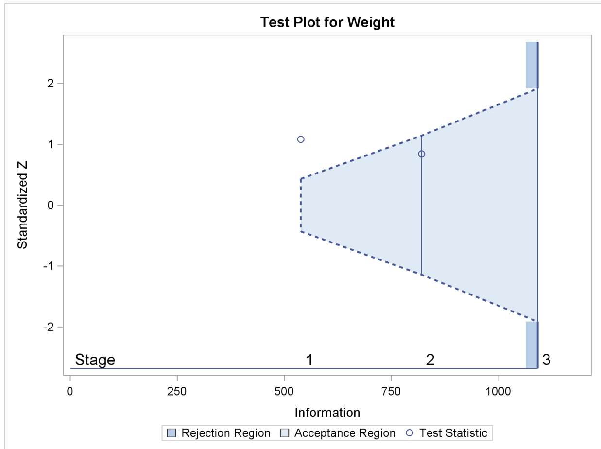
Output 78.3.18 Sequential Test Plot
