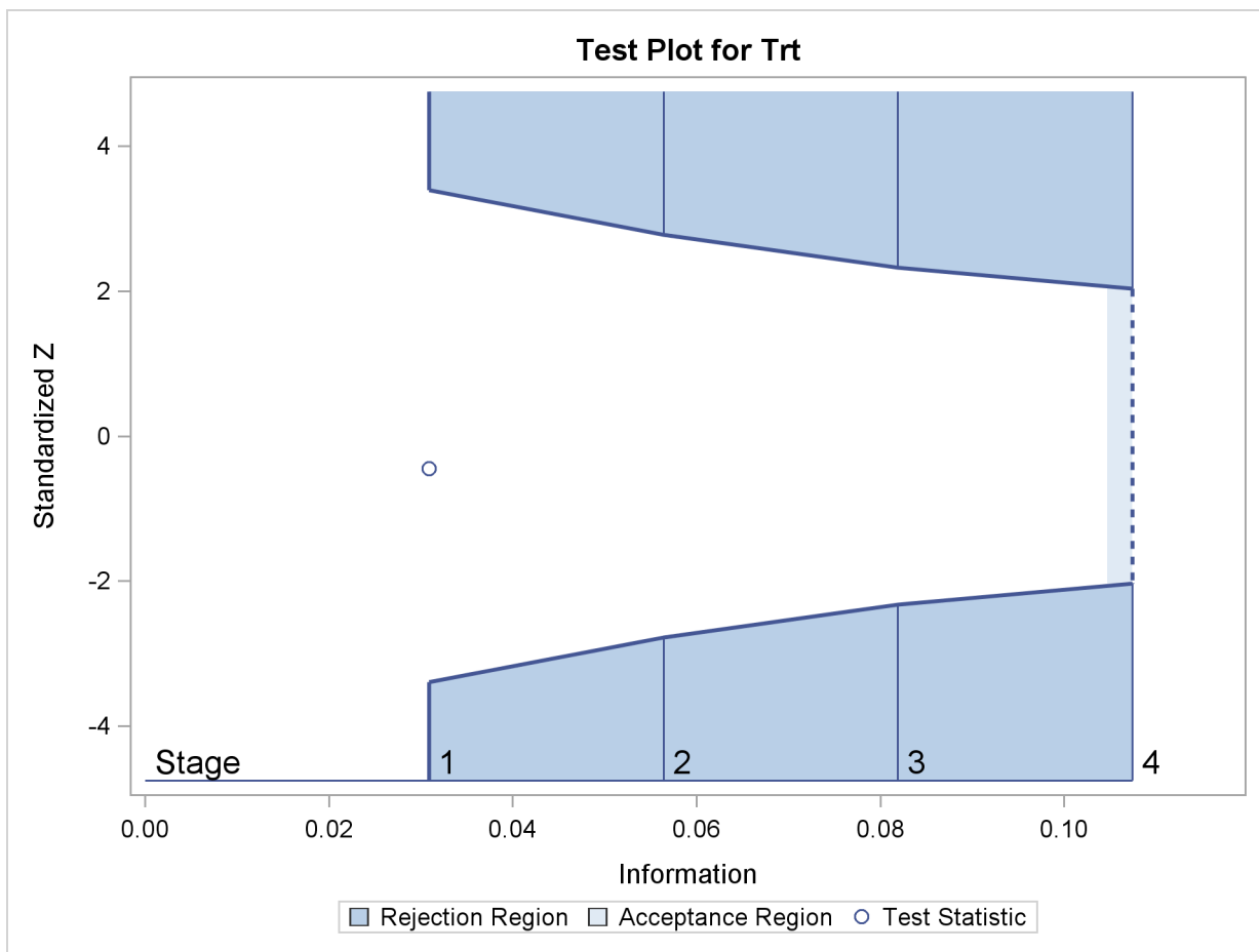
Figure 78.12 Sequential Test Plot
