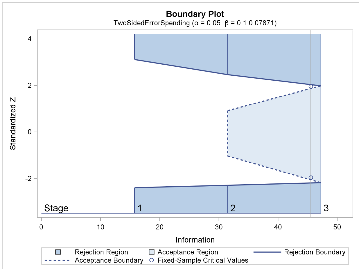
Output 78.8.3 Boundary Plot
