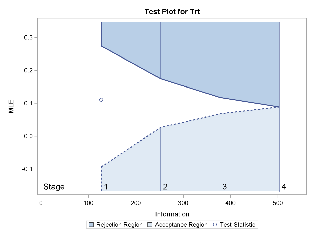
Output 78.1.13 Sequential Test Plot
