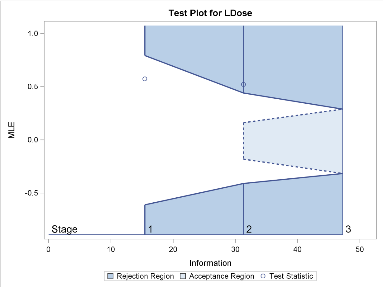
Output 78.8.14 Sequential Test Plot
