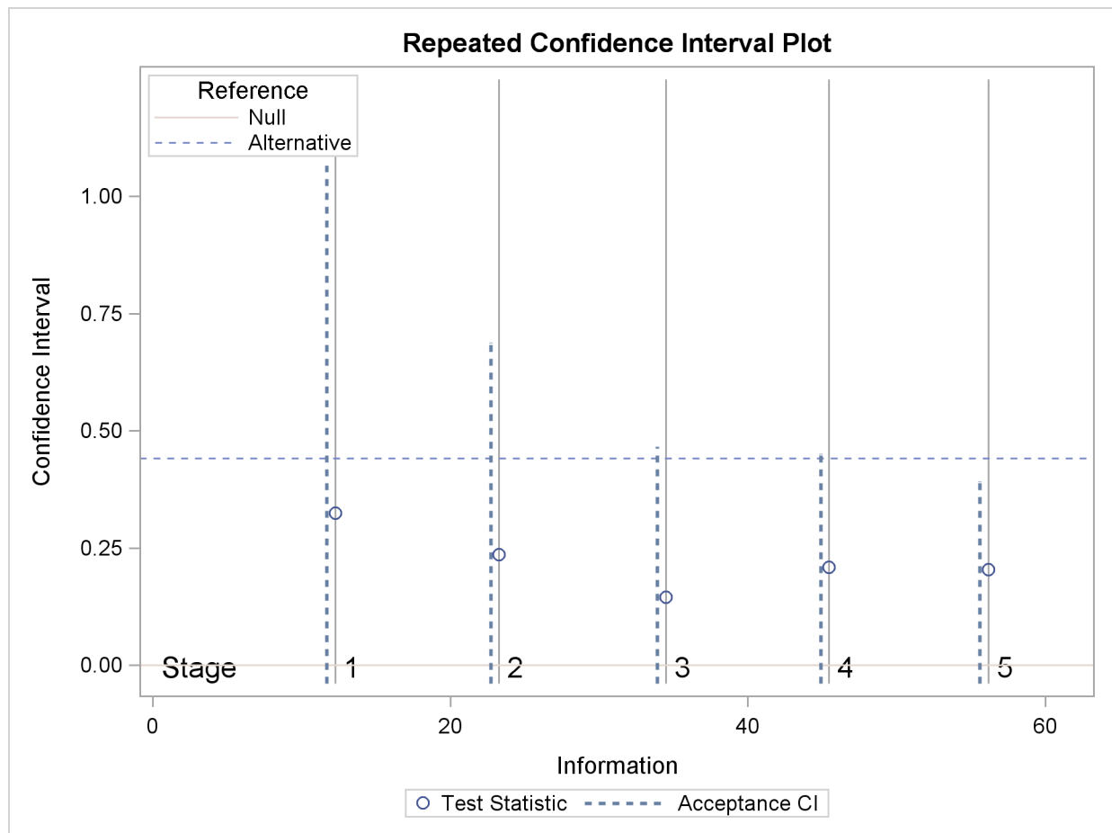
Output 78.5.18 Repeated Confidence Intervals Plot
