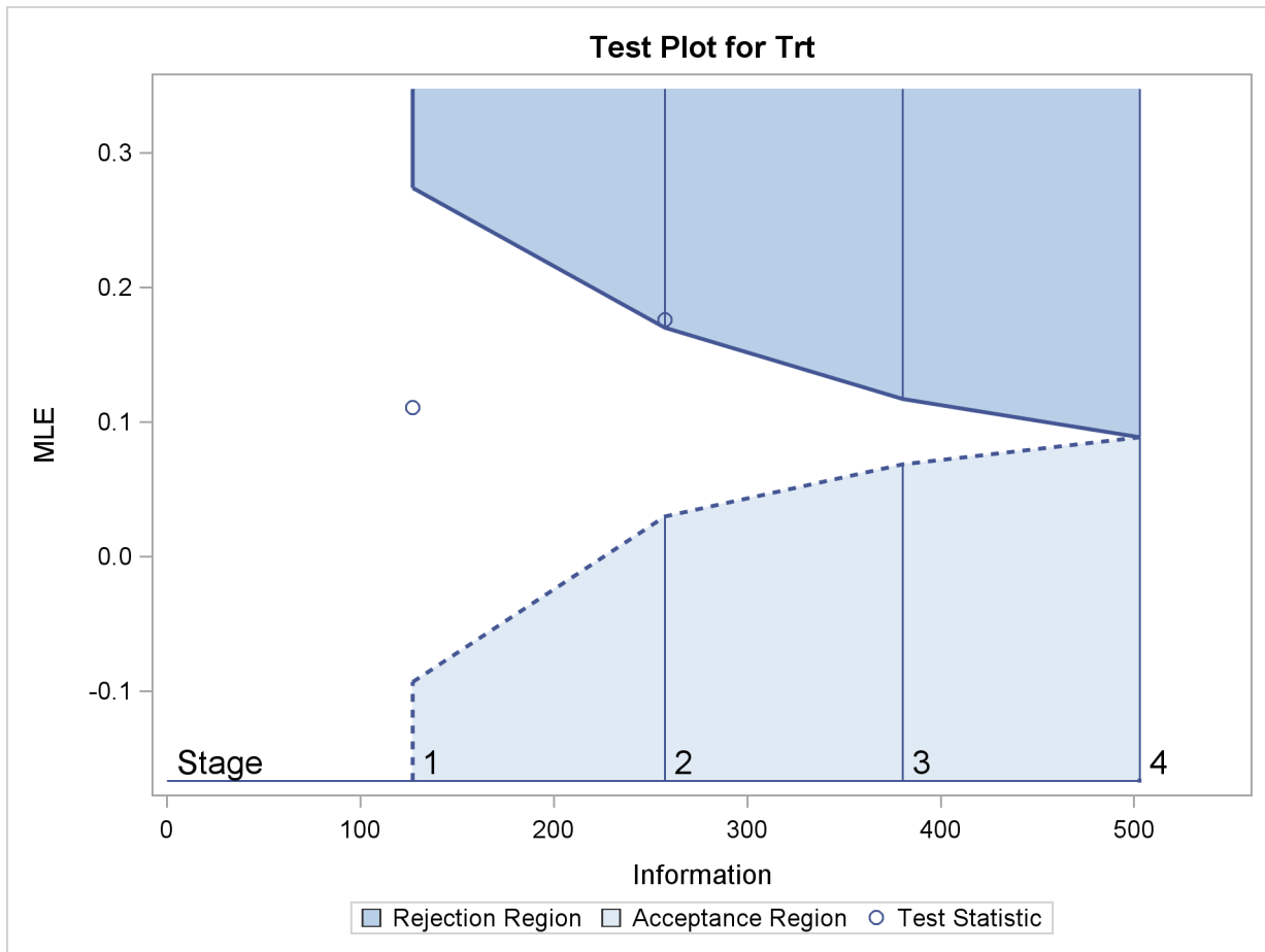
Output 78.1.16 Sequential Test Plot
