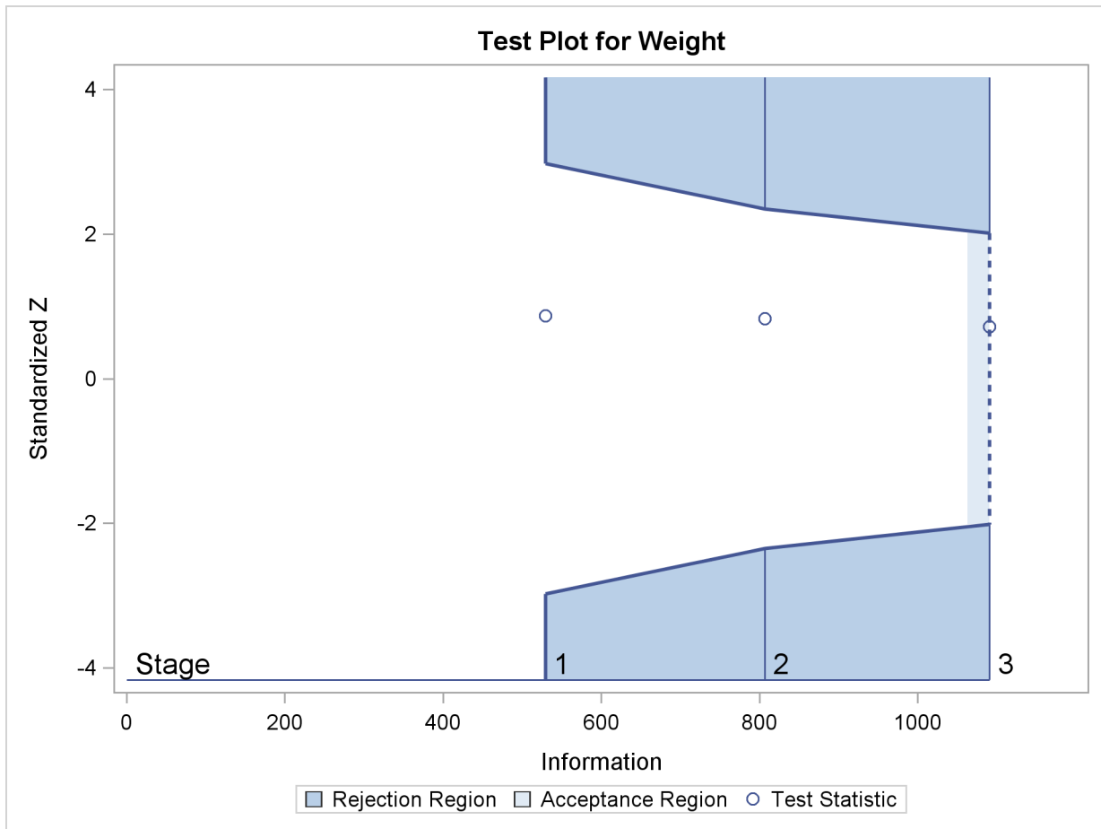
Output 78.2.19 Sequential Test Plot
