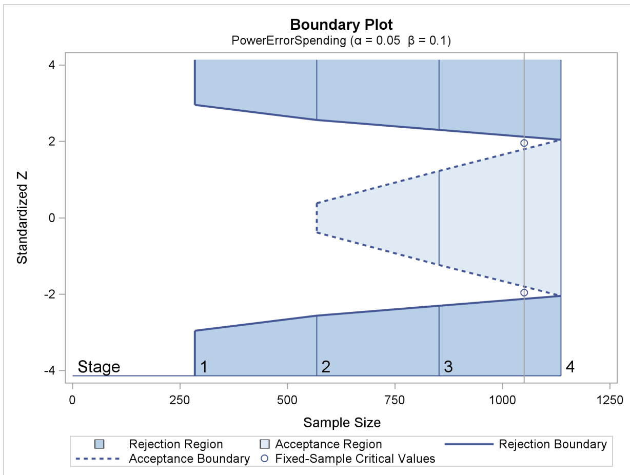
Figure 78.20 Boundary Plot for Two-Sided Test
