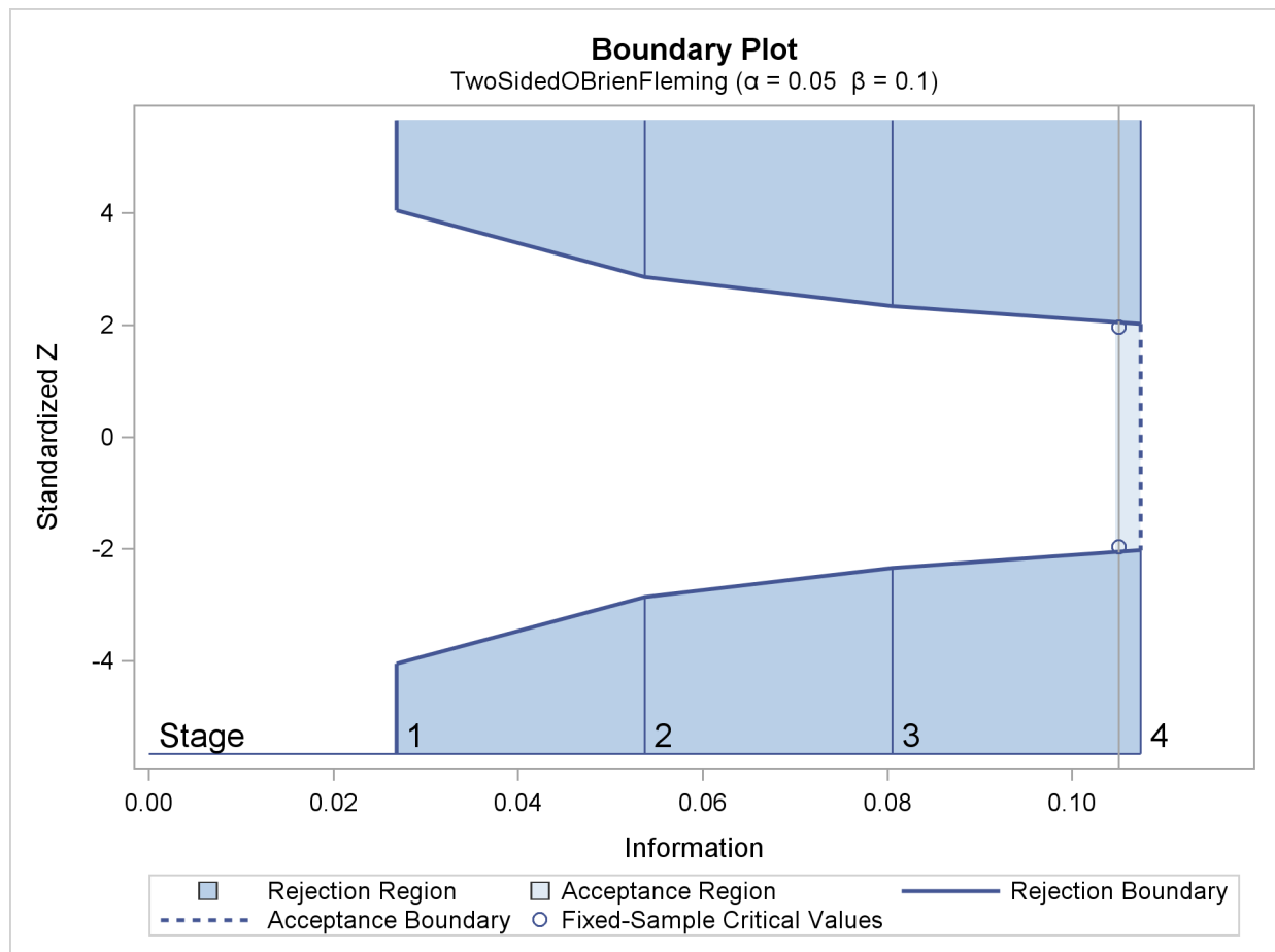
Figure 78.5 O'Brien-Fleming Boundary Plot
