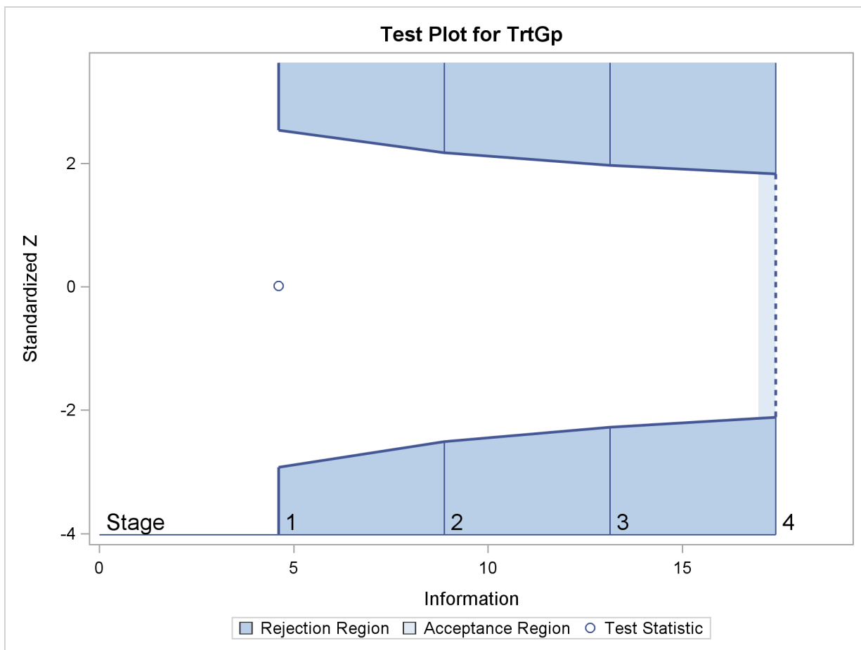
Output 78.7.12 Sequential Test Plot
