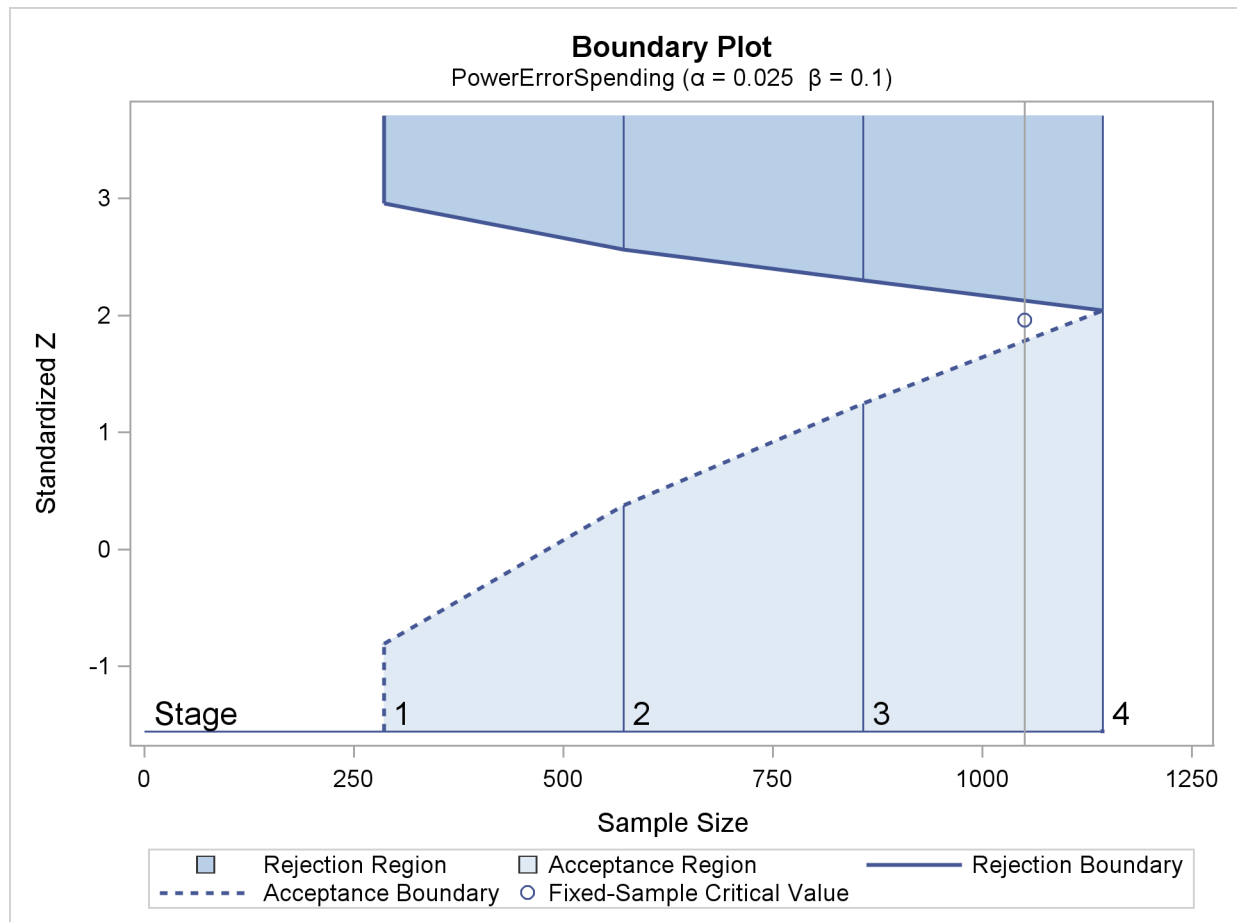
Figure 78.19 Boundary Plot for One-Sided Test
