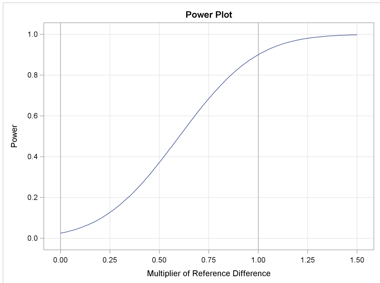
Output 78.3.16 Power Plot
