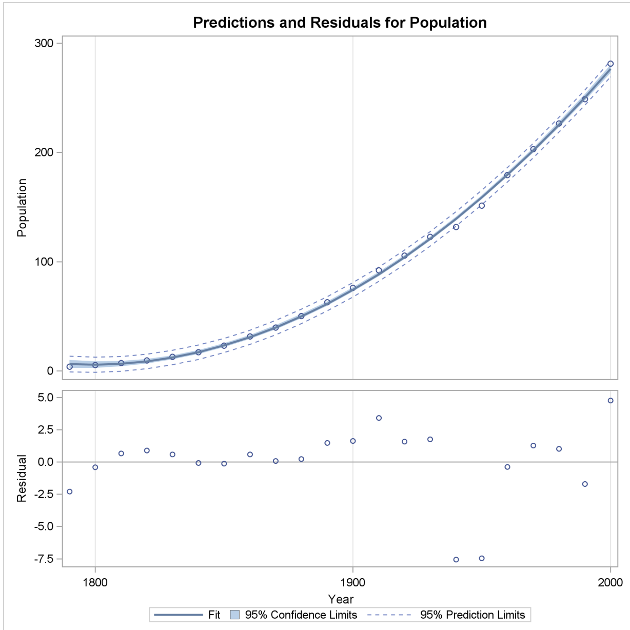
Figure 73.13 Predictions and Residuals by Year
