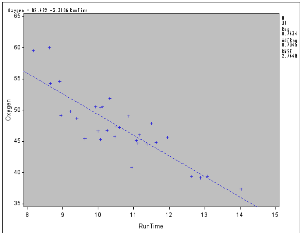
Figure 73.43 Simple Linear Regression
