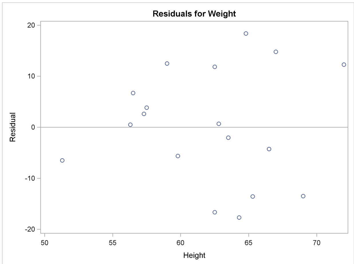
Figure 73.3 Residuals vs. Regressor
