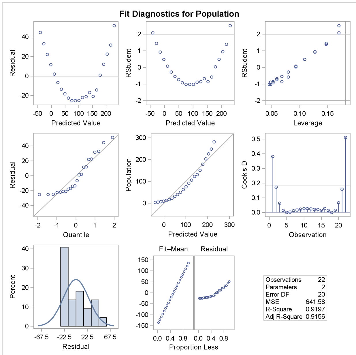
Figure 73.8 Diagnostics Panel
