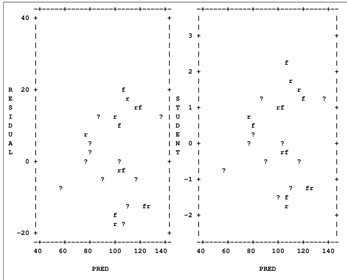
Figure 73.38 continued
