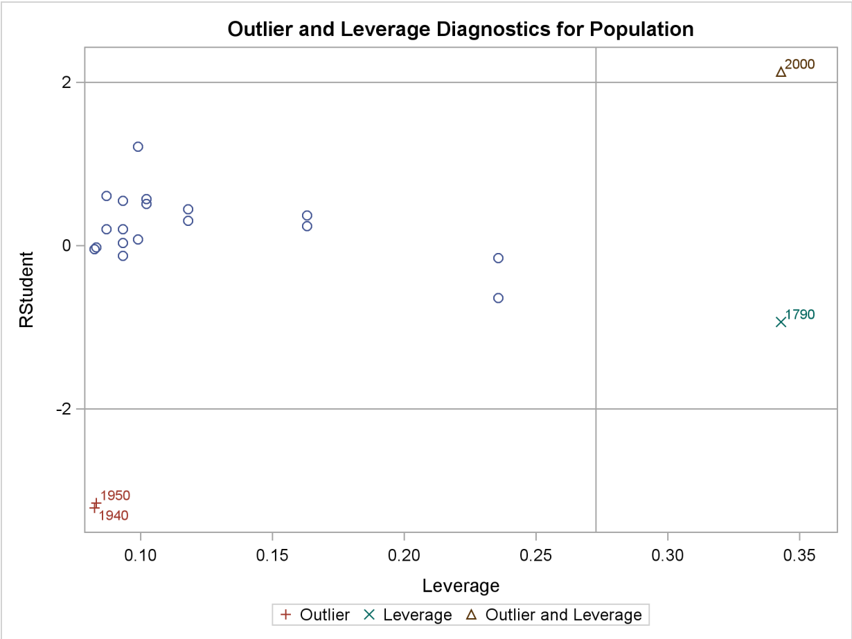
Figure 73.52 continued
