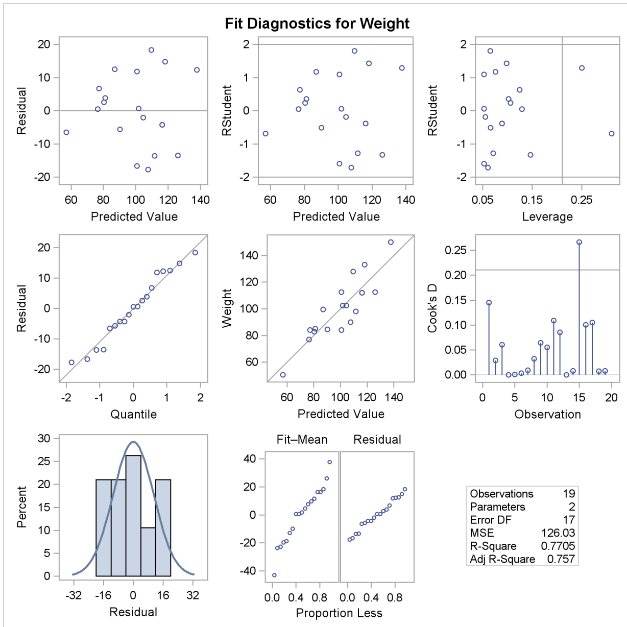
Figure 73.4 Fit Diagnostics
