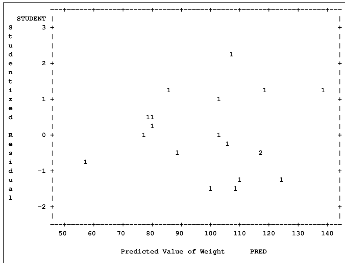
Figure 73.39 Plotting Studentized Residuals against Predicted Values
