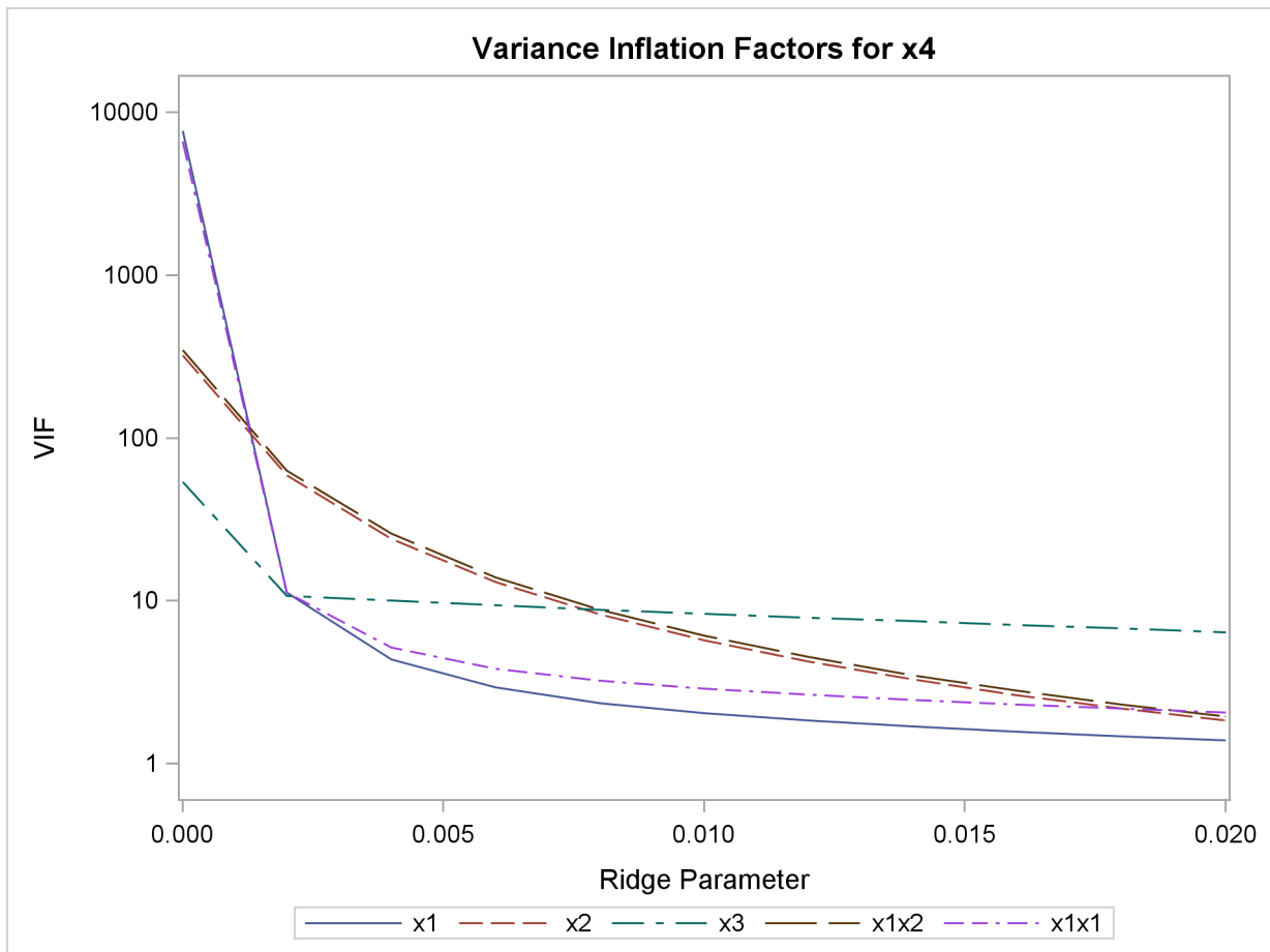
Output 73.5.3 VIF Traces
