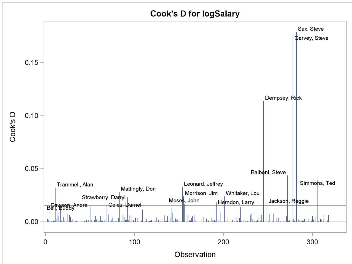
Output 73.1.13 Cook's D
