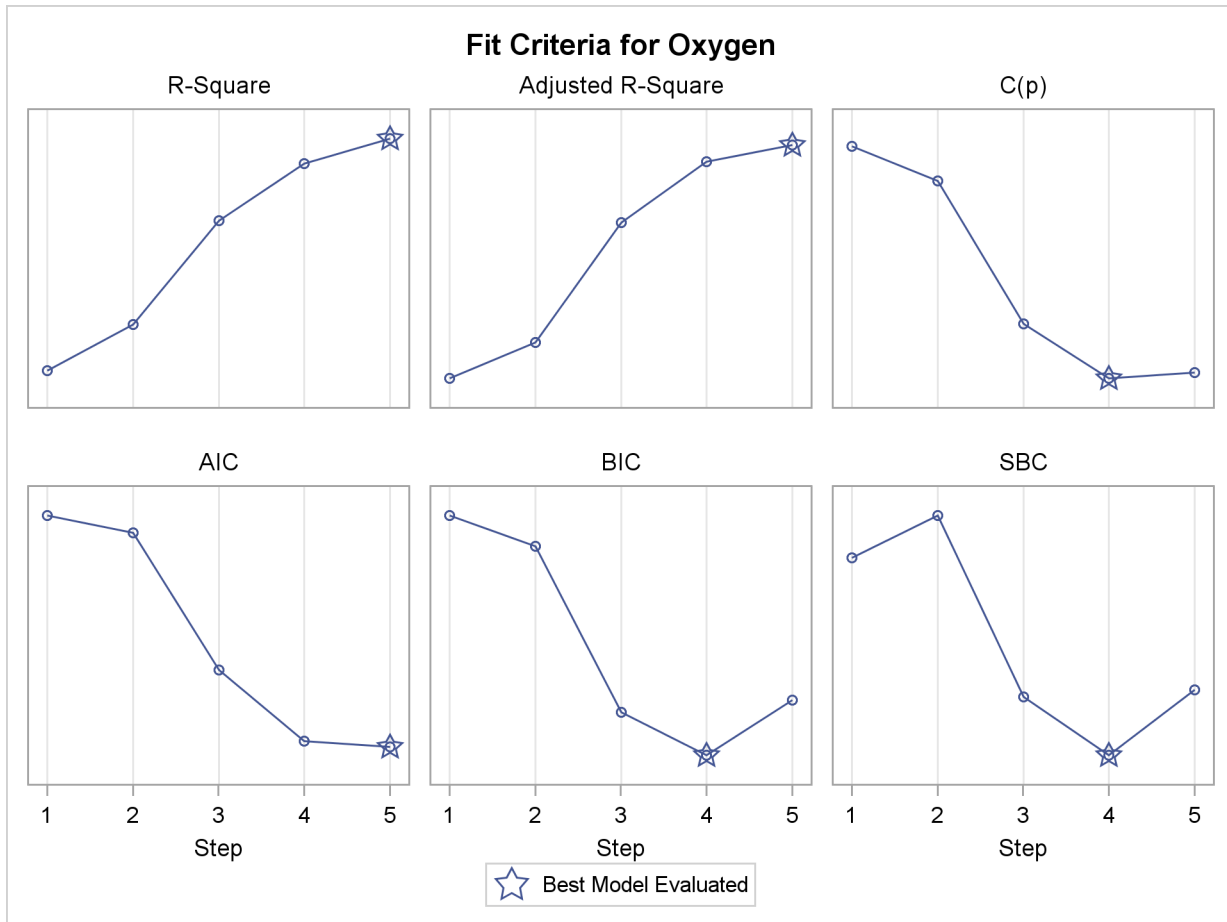
Output 73.2.5 Fit Criteria
