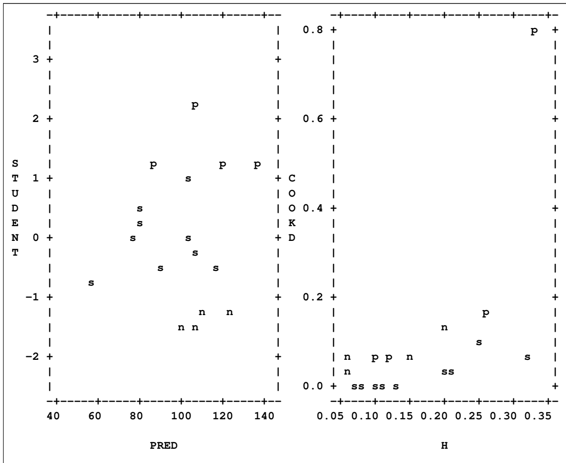
Figure 73.42 Painting Observations on More Than One Plot
