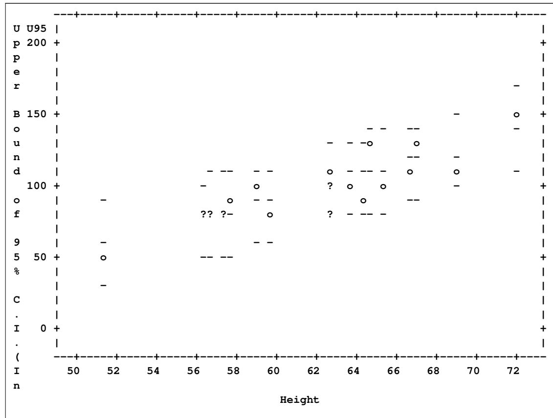
Figure 73.38 Side-by-Side Residual Plots for the Full and Reduced Models
