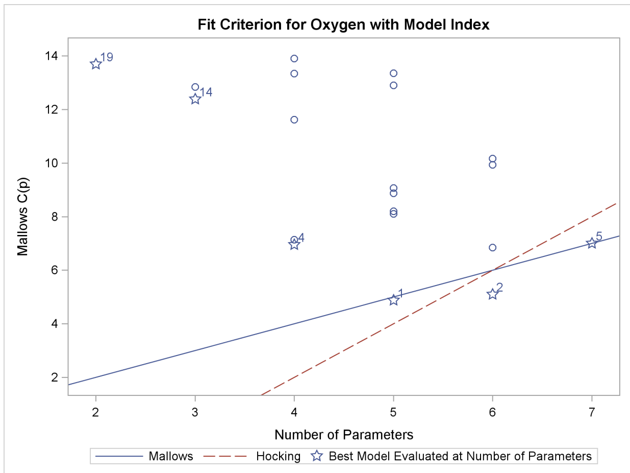
Output 73.2.11 C_p Criterion
