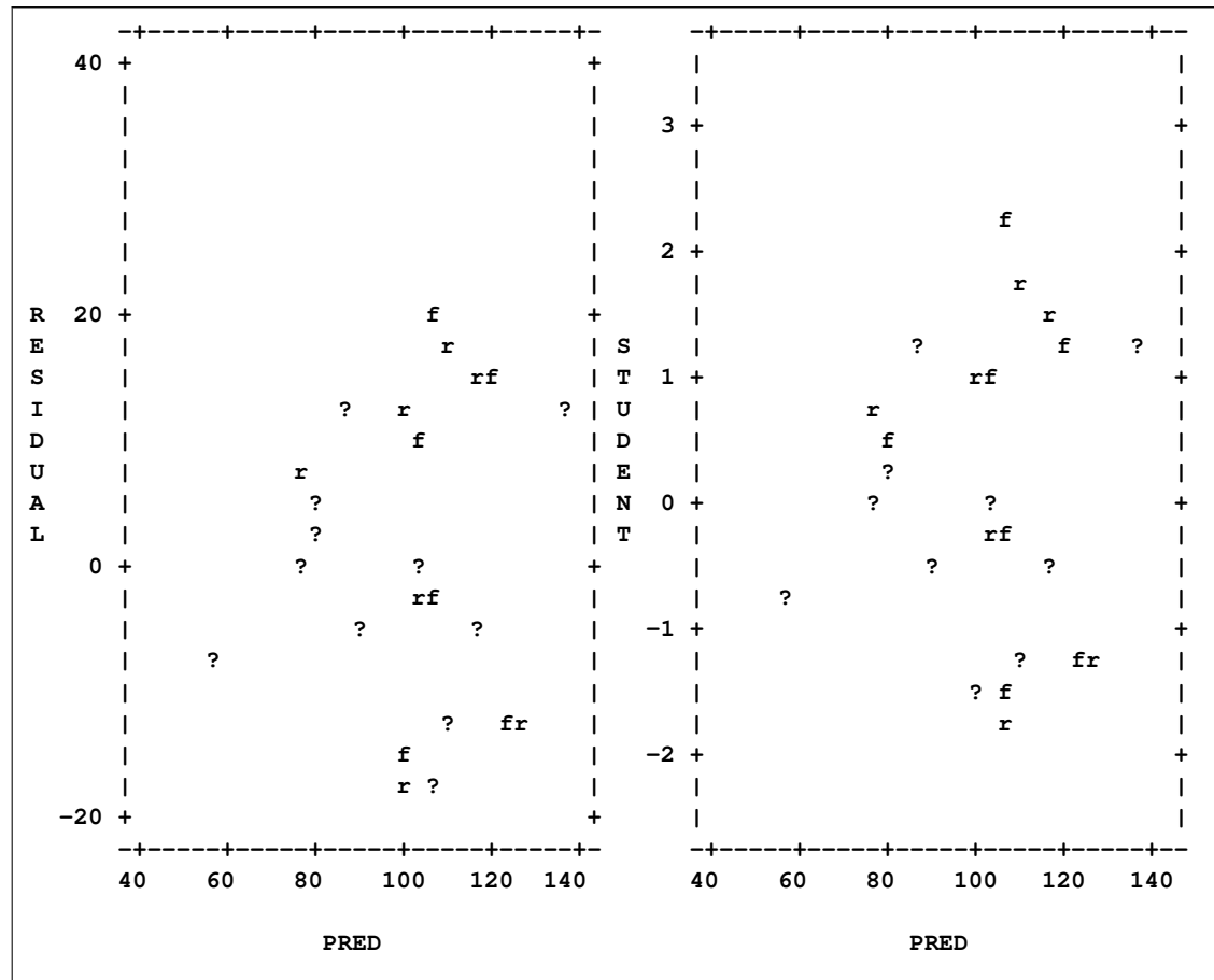
Figure 73.36 Overlaid Residual Plots for Full and Reduced Models
