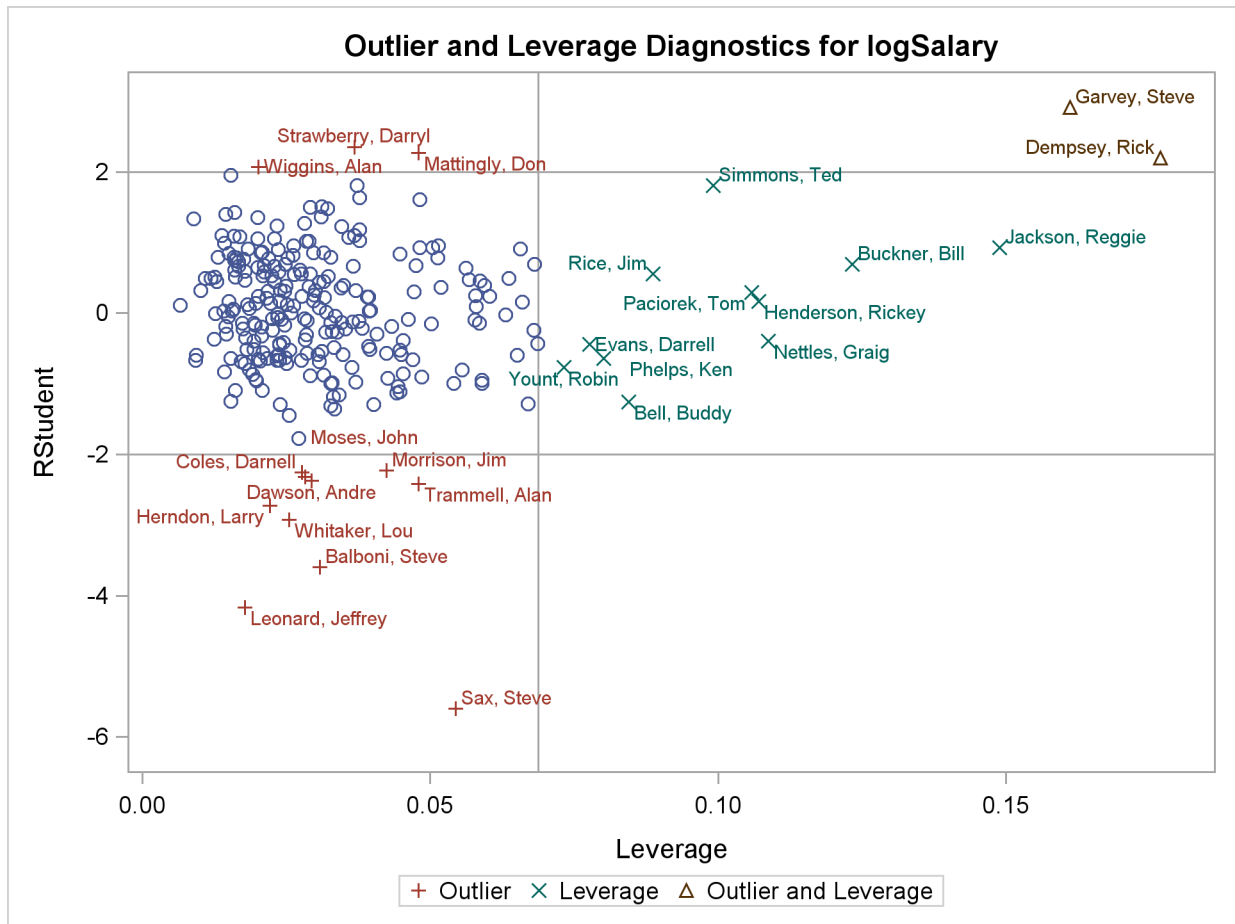
Output 73.1.11 Outlier and Leverage Diagnostics
