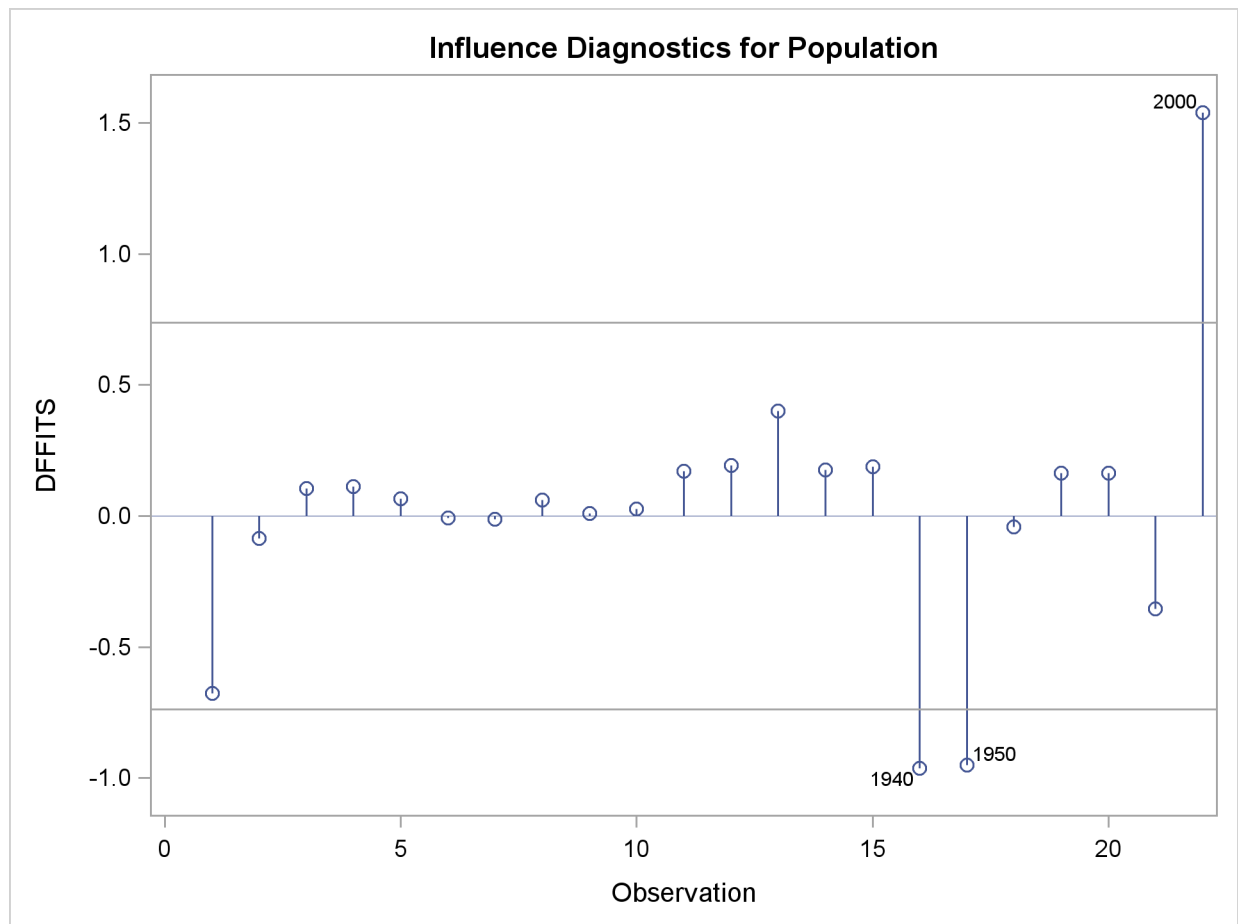
Figure 73.52 continued
