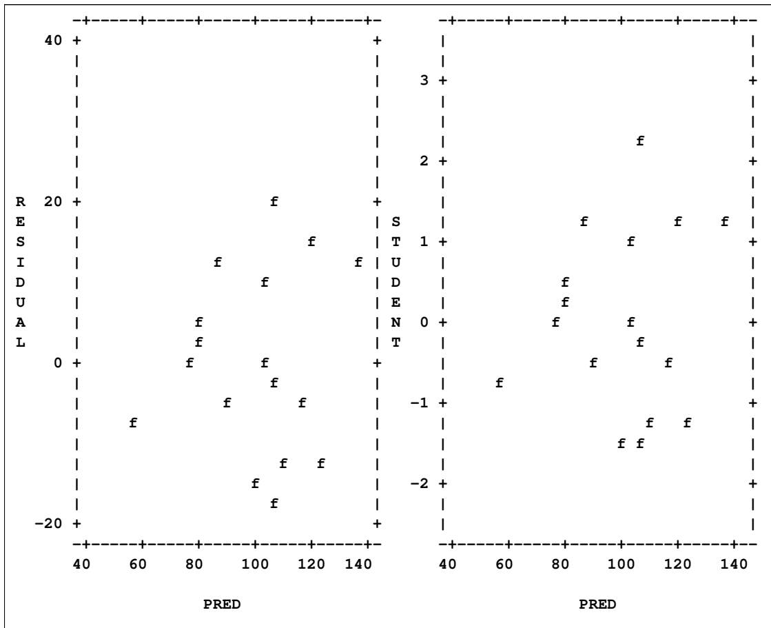
Figure 73.35 Collecting Residual Plots for the Full Model
