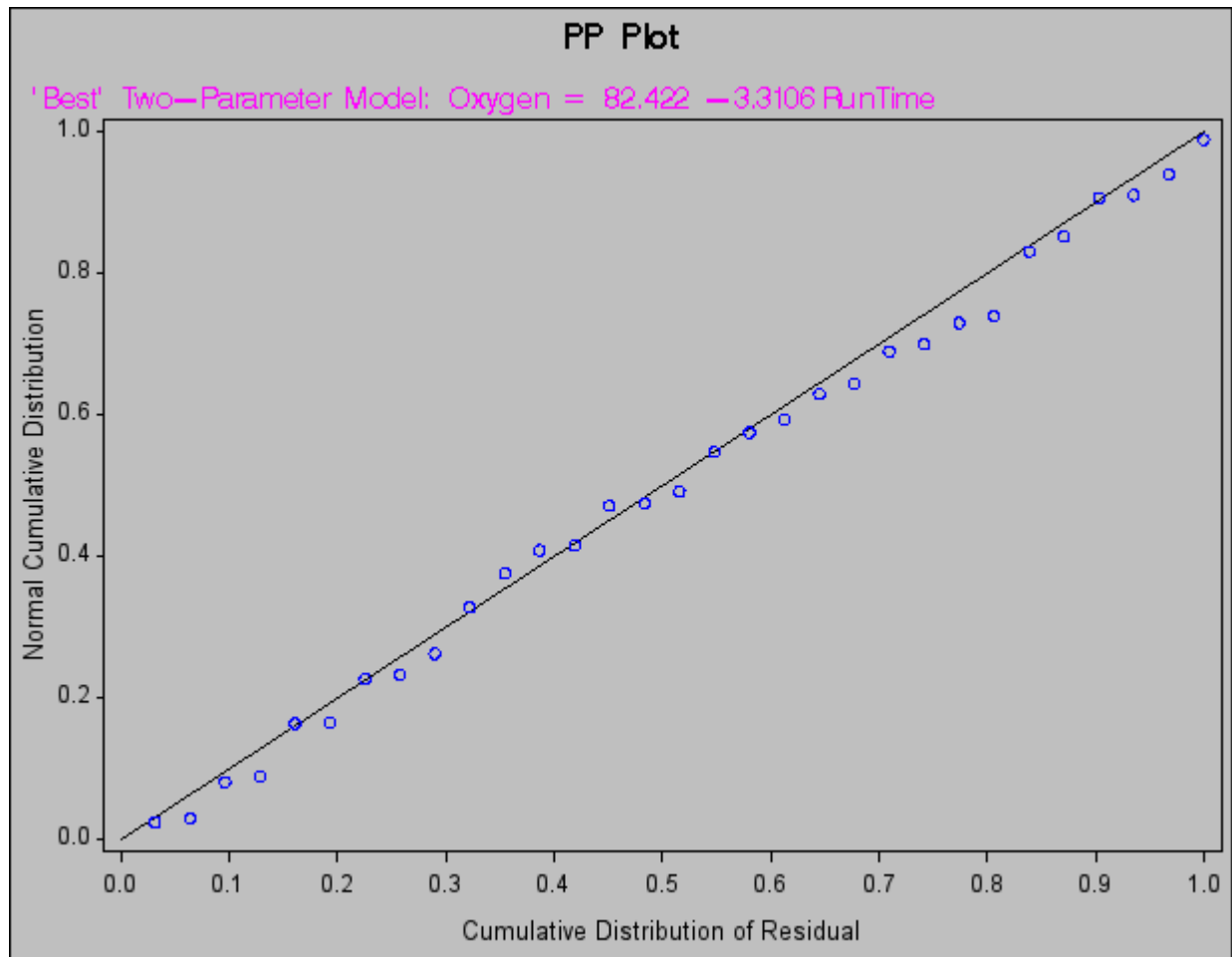
Figure 73.46 Normal Probability-Probability Plot for the Residuals
