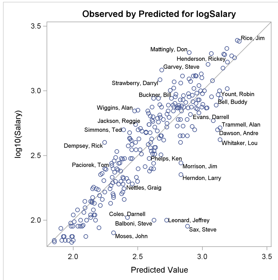
Output 73.1.12 Observed by Predicted Values
