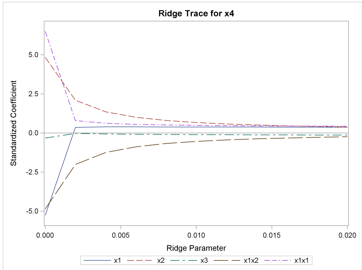
Output 73.5.4 Ridge Traces
