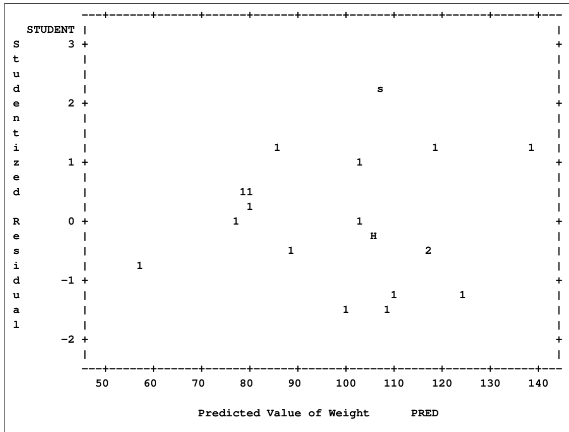
Figure 73.41 Painting Several Observations
