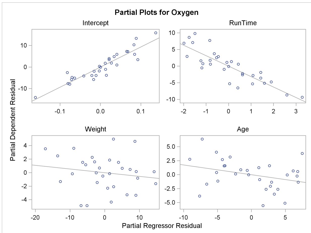
Figure 73.53 Partial Regression Leverage Plots
