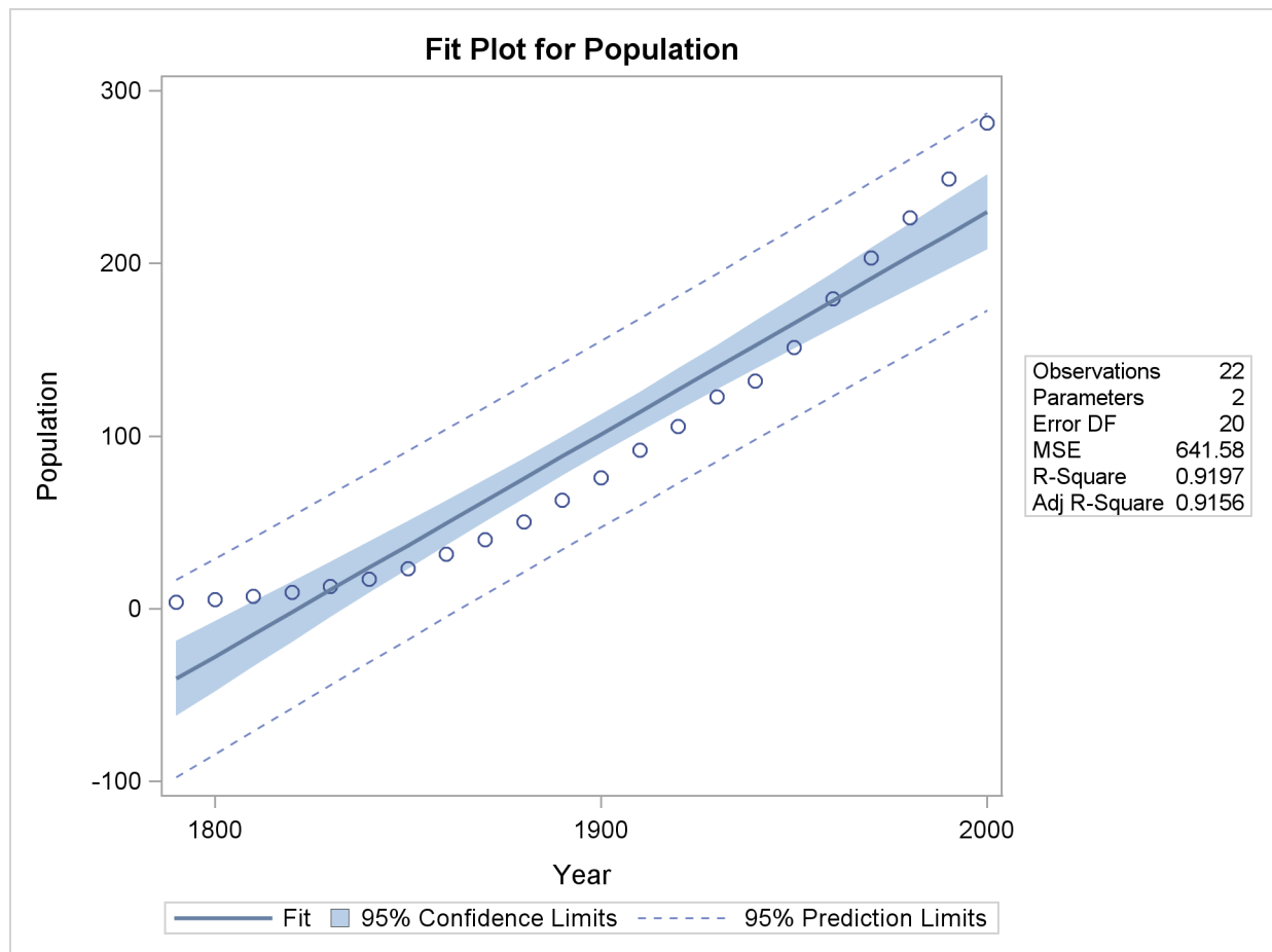
Figure 73.10 Fit Plot
