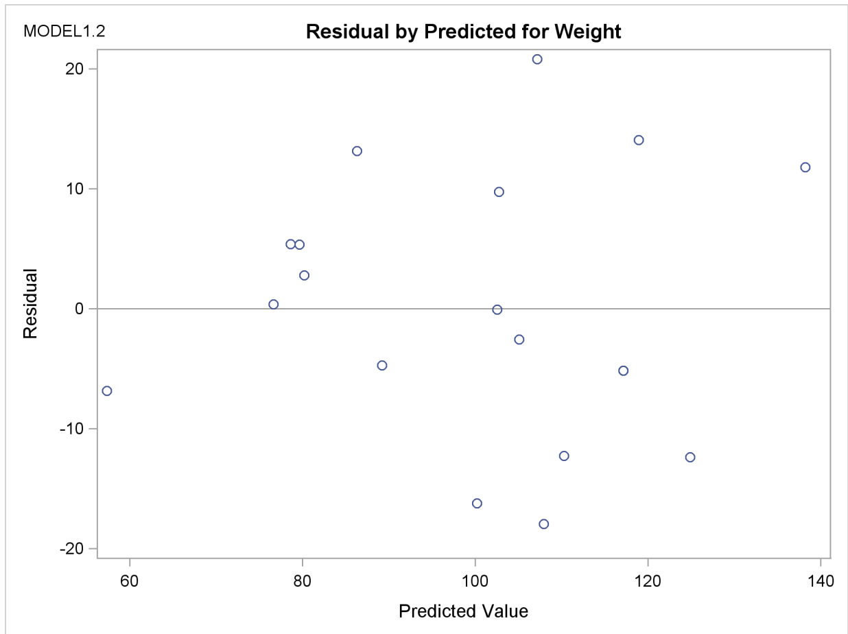
Figure 73.27 Interactive Analysis: Scatter Plot
