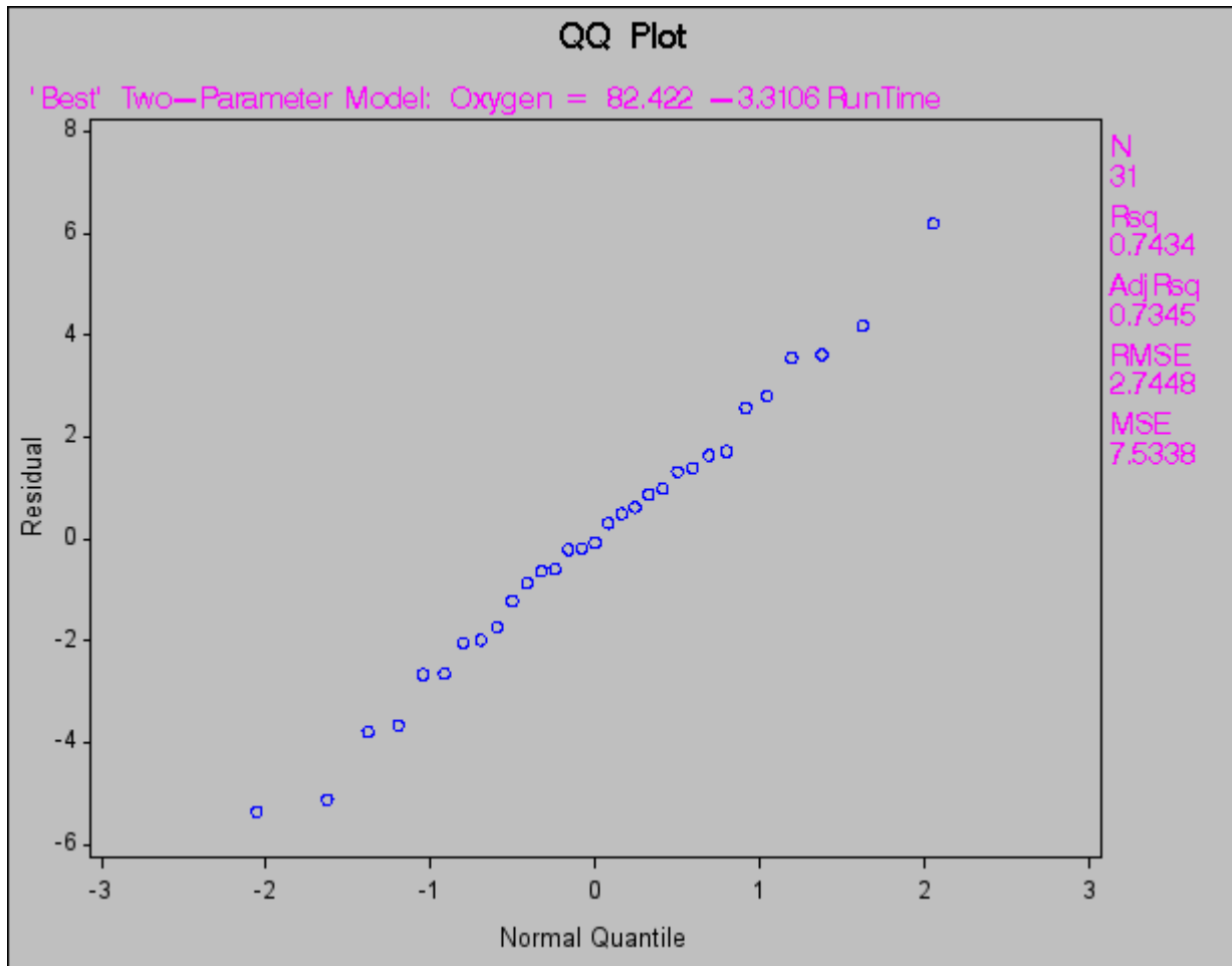
Figure 73.47 Normal Quantile-Quantile Plot for the Residuals
