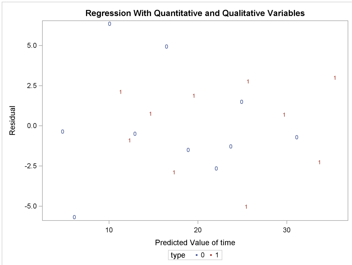
Output 73.4.3 Plot of Residual vs. Predicted Values
