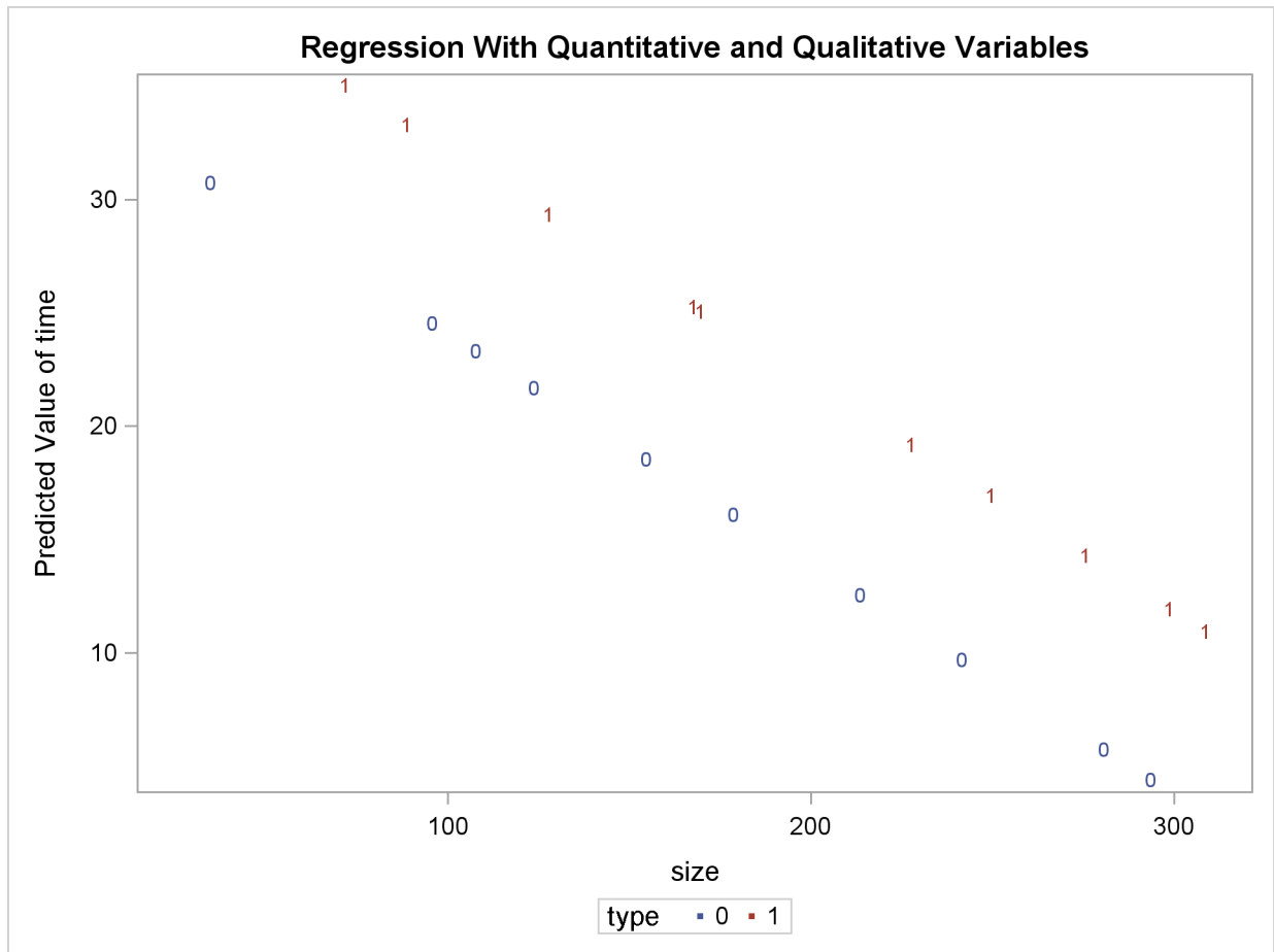
Output 73.4.4 Plot of Predicted vs. Size
