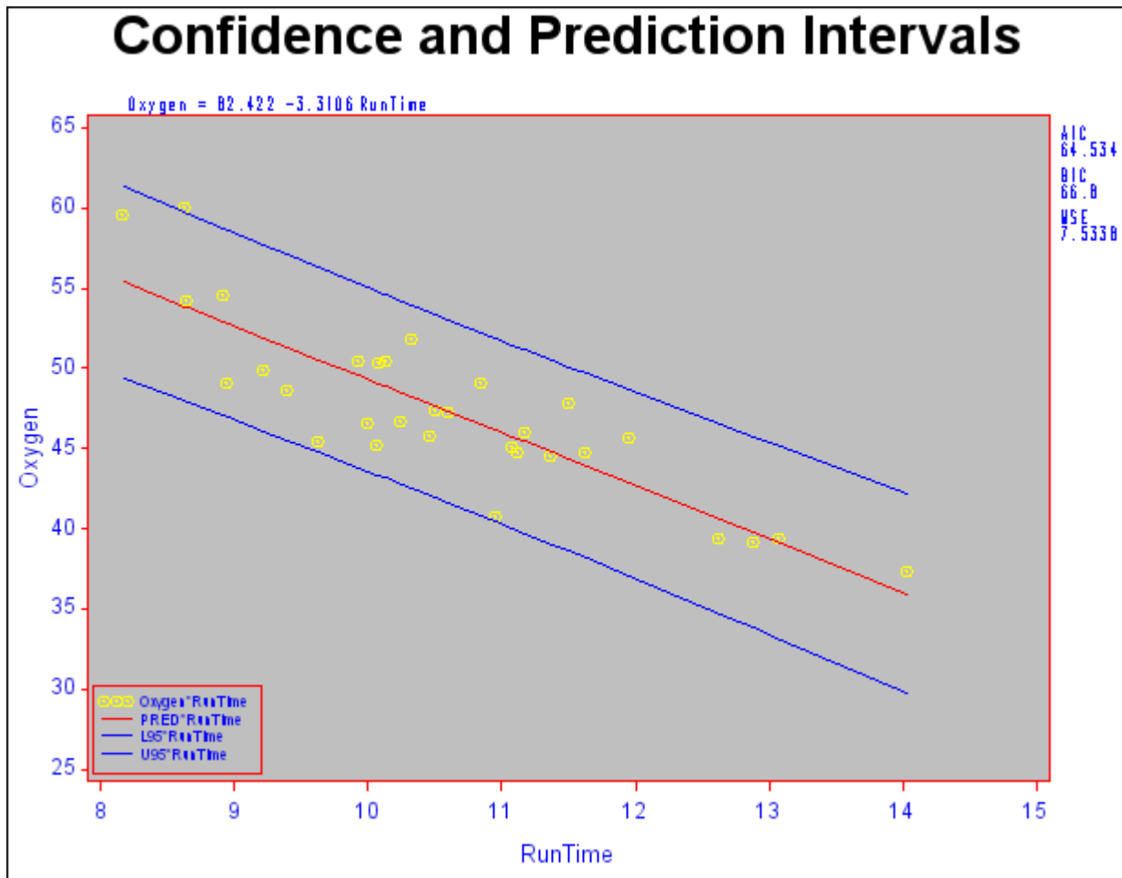
Figure 73.44 Simple Linear Regression
