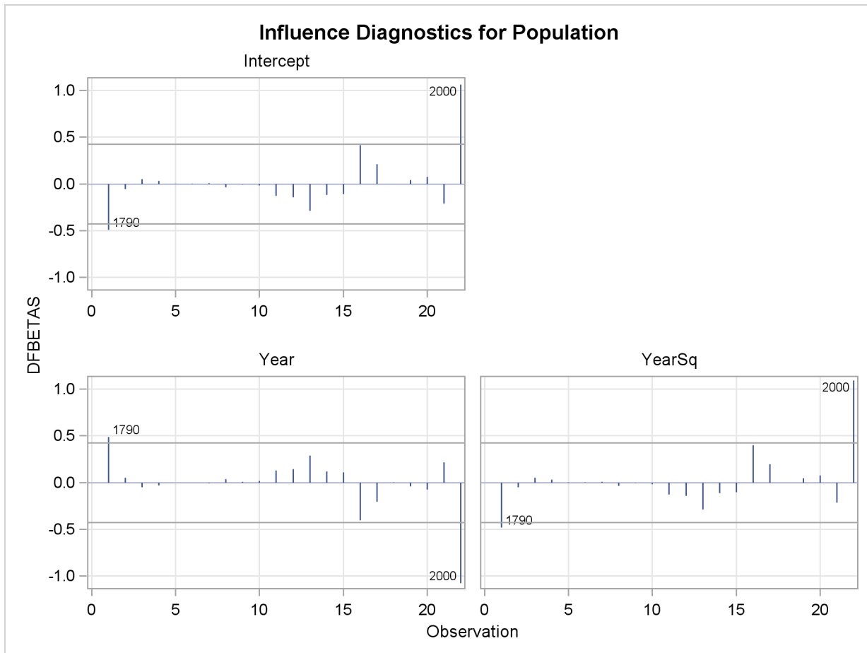
Figure 73.52 continued
