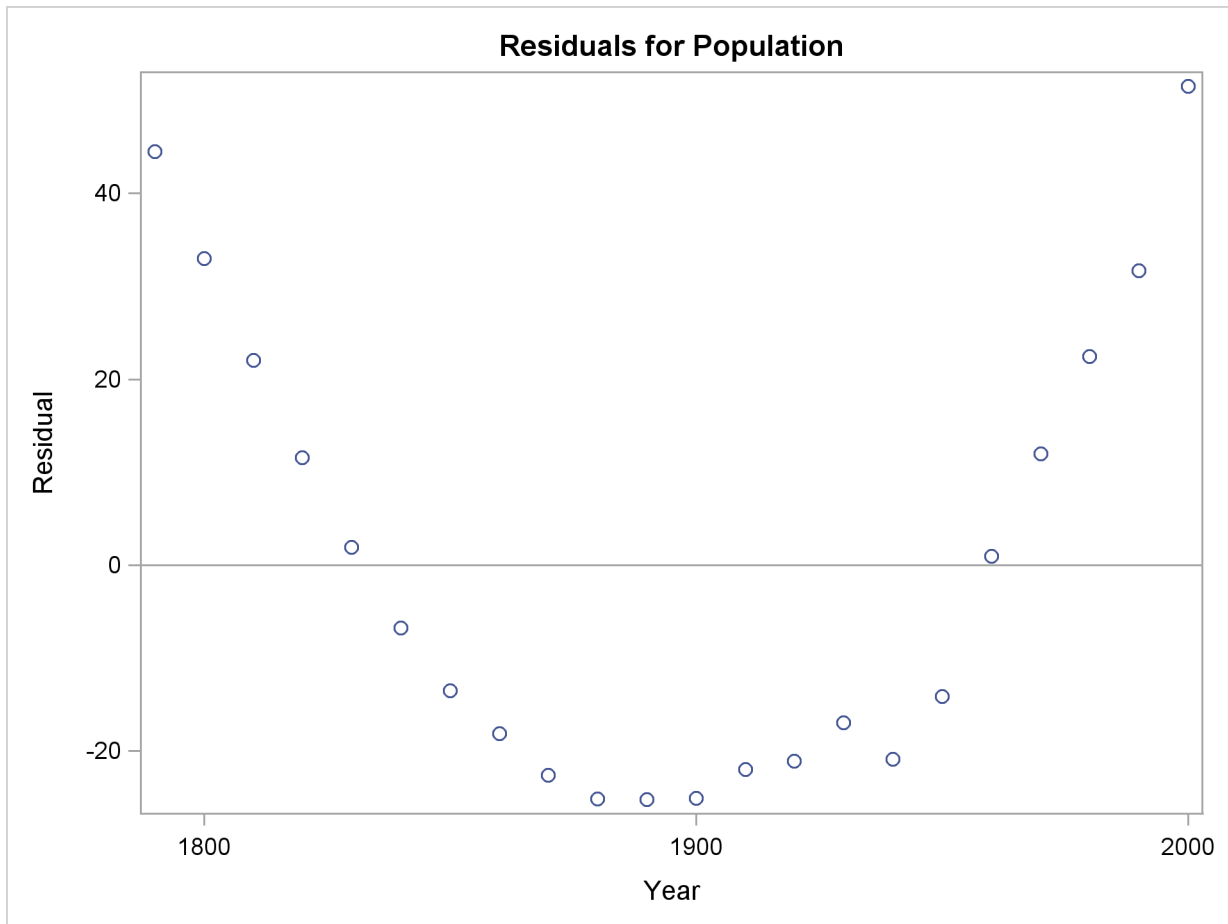
Figure 73.9 Residual Plot
