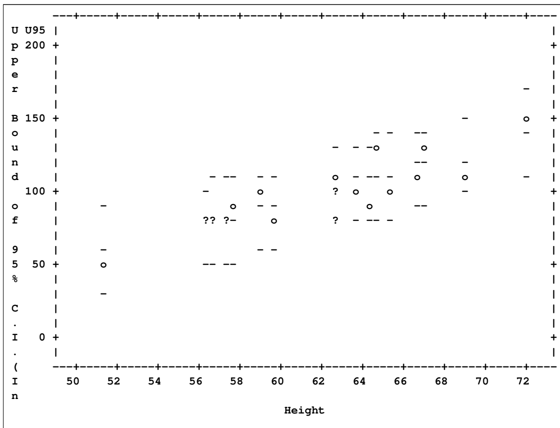
Figure 73.34 Scatter Plot Showing Data, Predicted Values, and Confidence Limits
