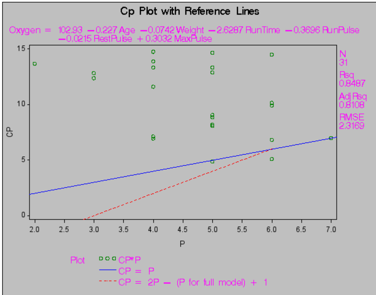
Figure 73.45 C_p Plot with Reference Lines
