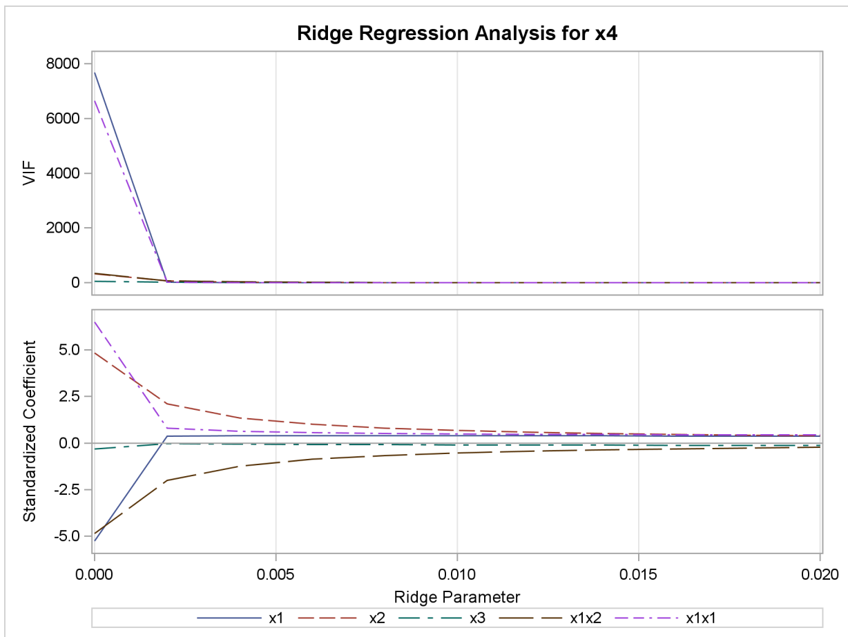
Output 73.5.1 Ridge Regression and VIF Traces
