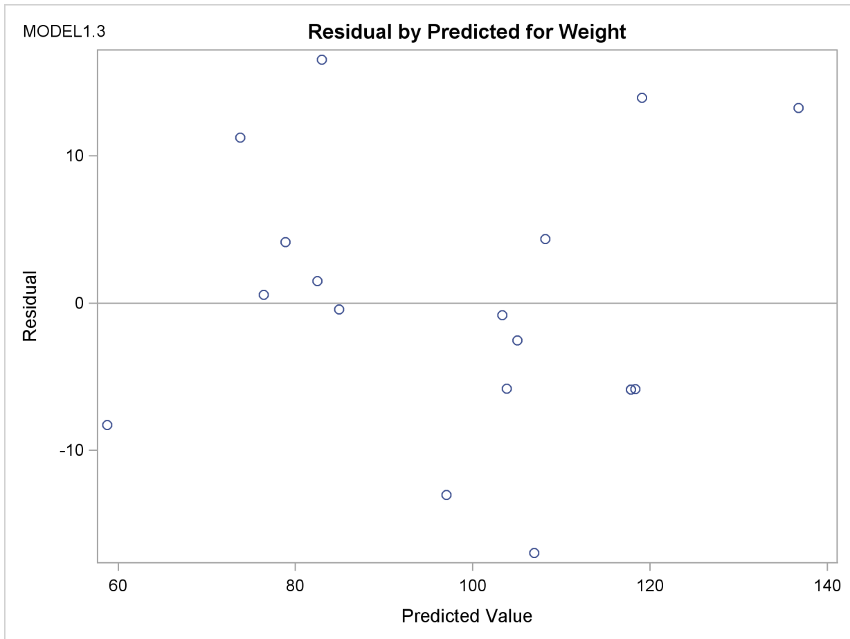
Figure 73.28 Interactive Analysis: Scatter Plot
