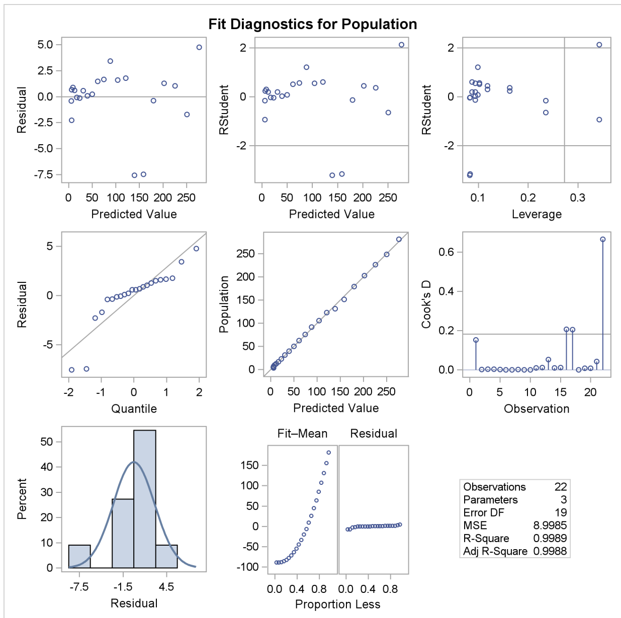
Figure 73.12 Diagnostics Panel
