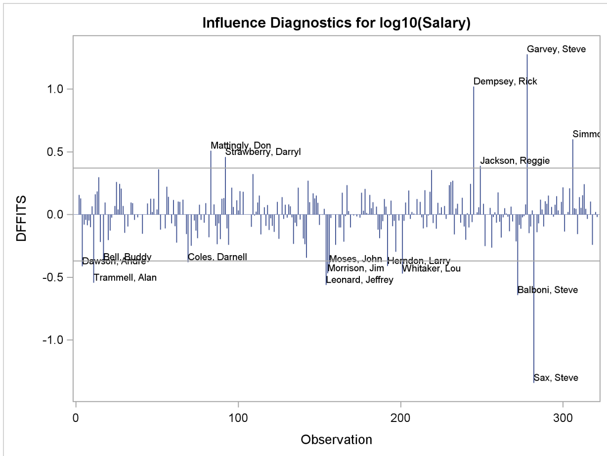
Output 73.1.14 DFFITS
