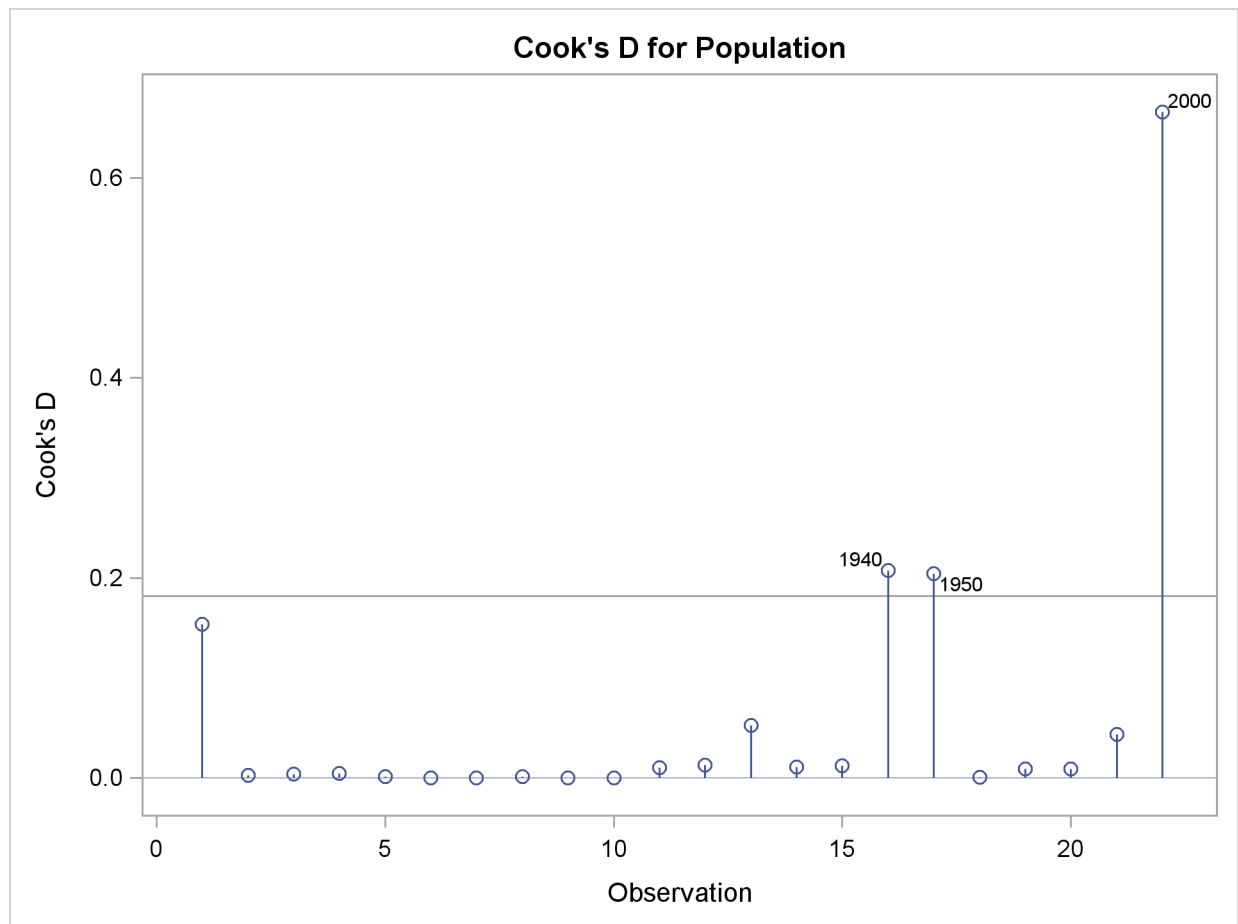
Figure 73.52 Influence Diagnostics
