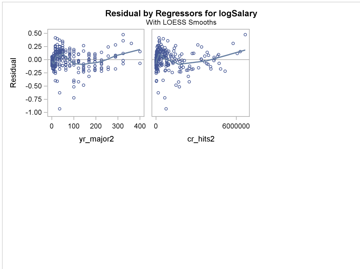
Output 73.1.9 Residuals by Regressors
