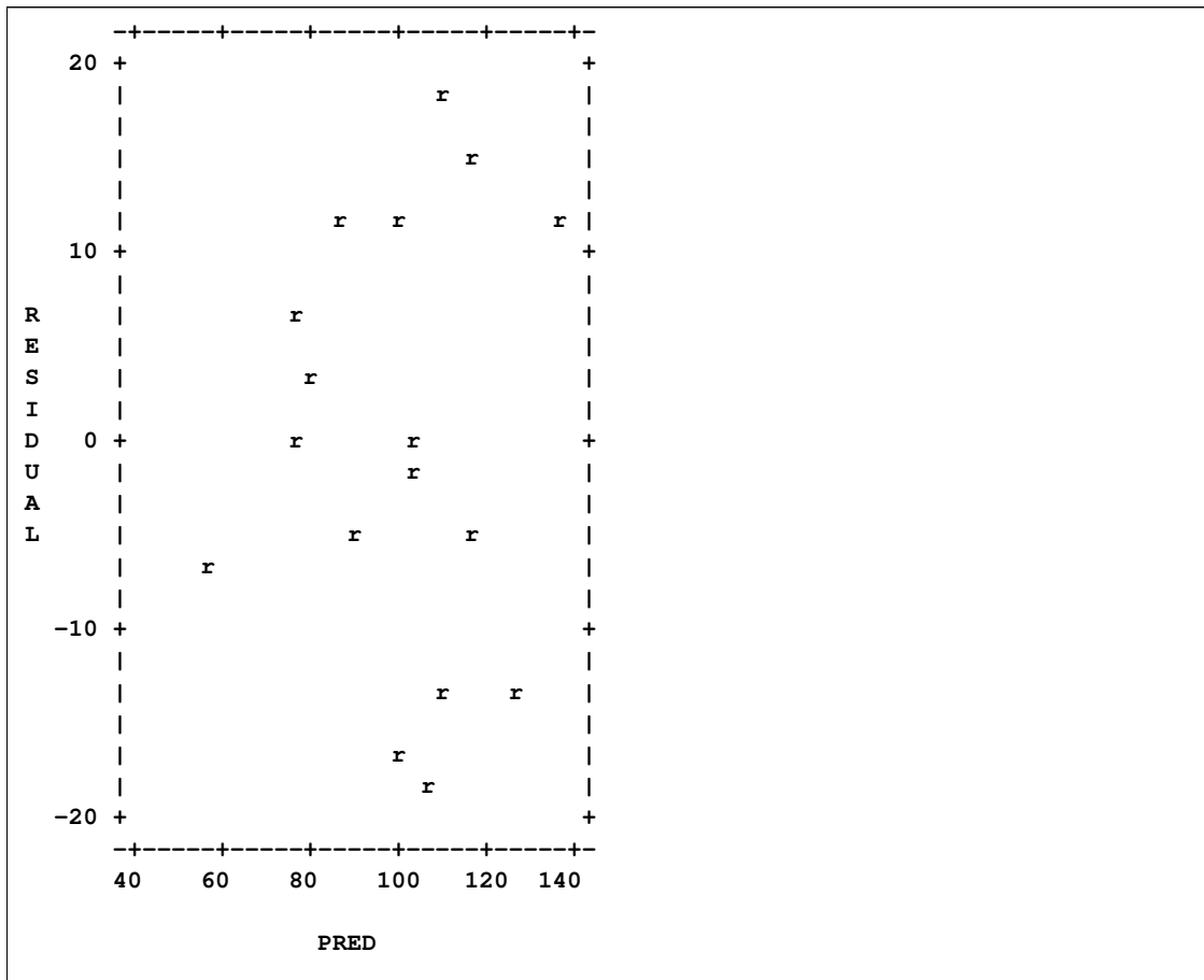
Figure 73.37 Residual Plot for Reduced Model Only
