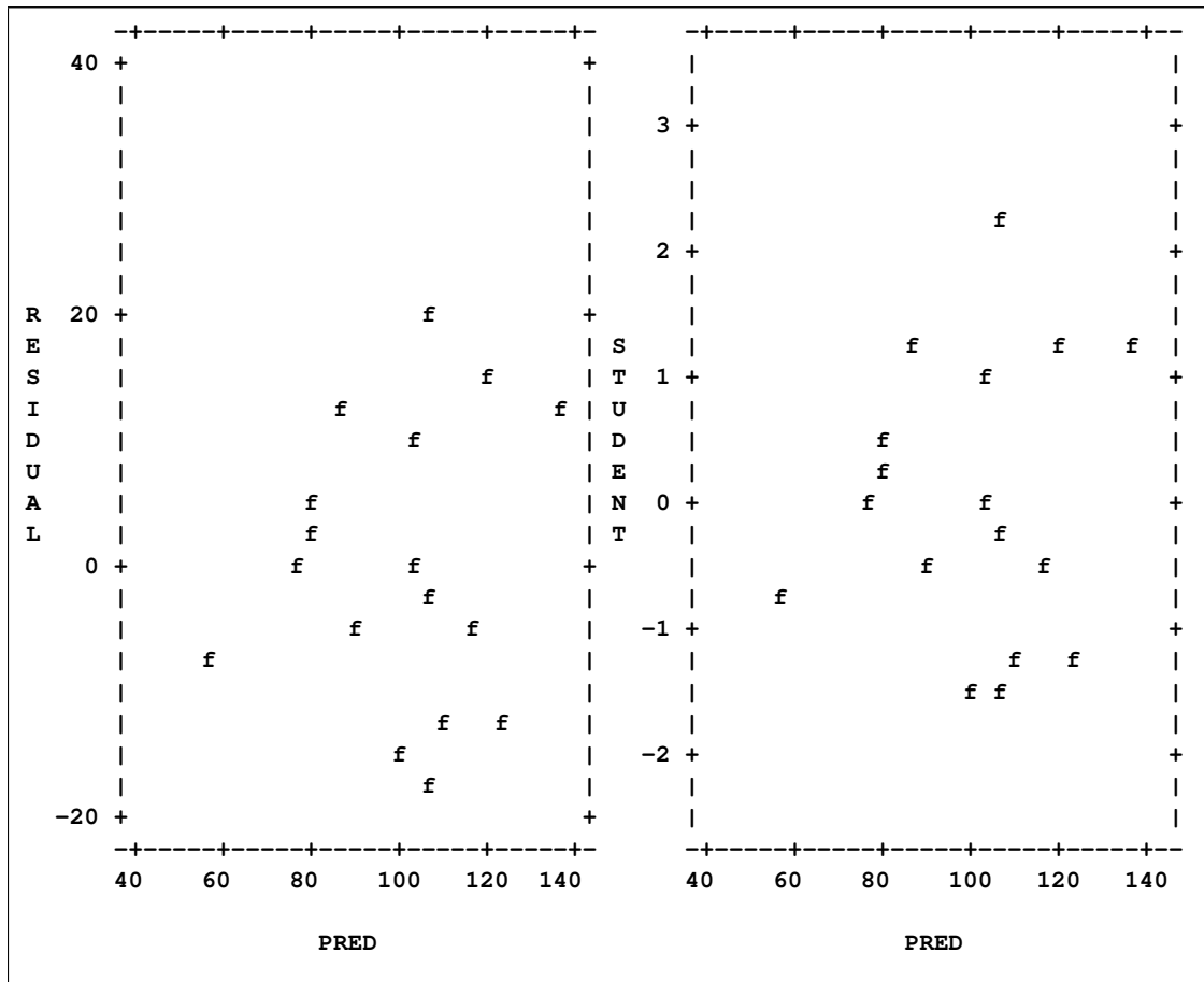
Figure 73.38 continued
