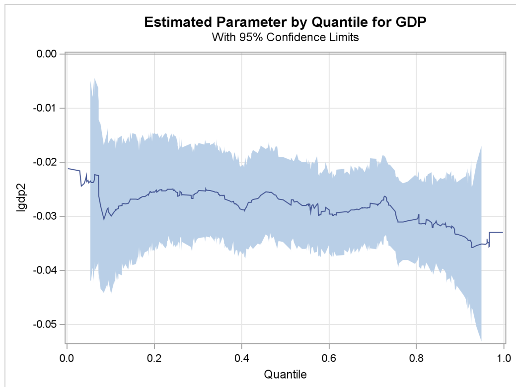
Output 72.2.9 Quantile Process Plot for LGDP2
