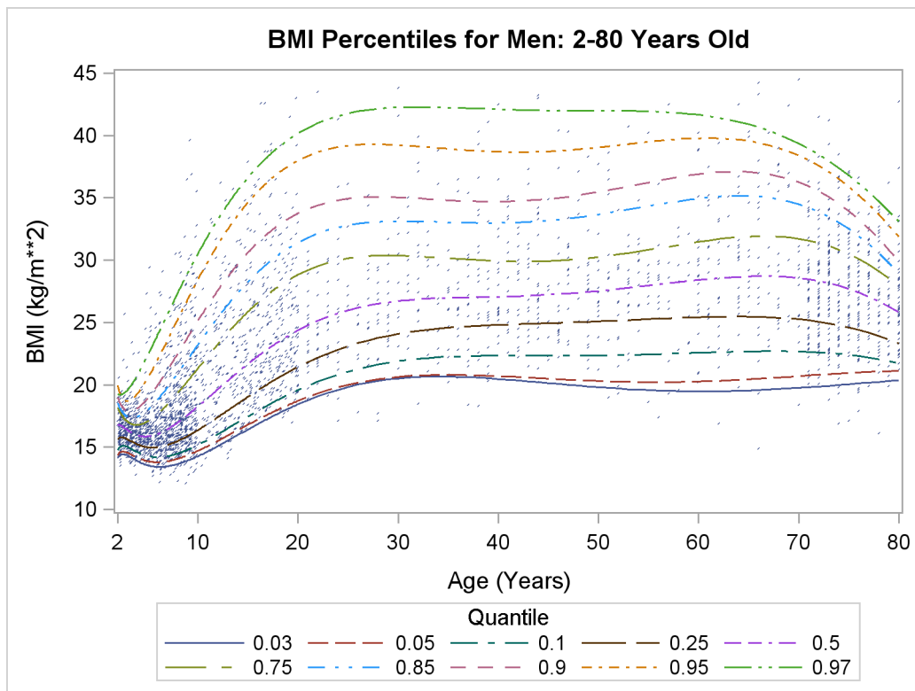
Figure 72.2 Quantiles for Body Mass Index
