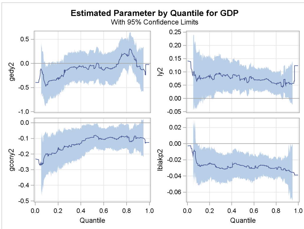
Output 72.2.8 Quantile Processes with 95% Confidence Bands
