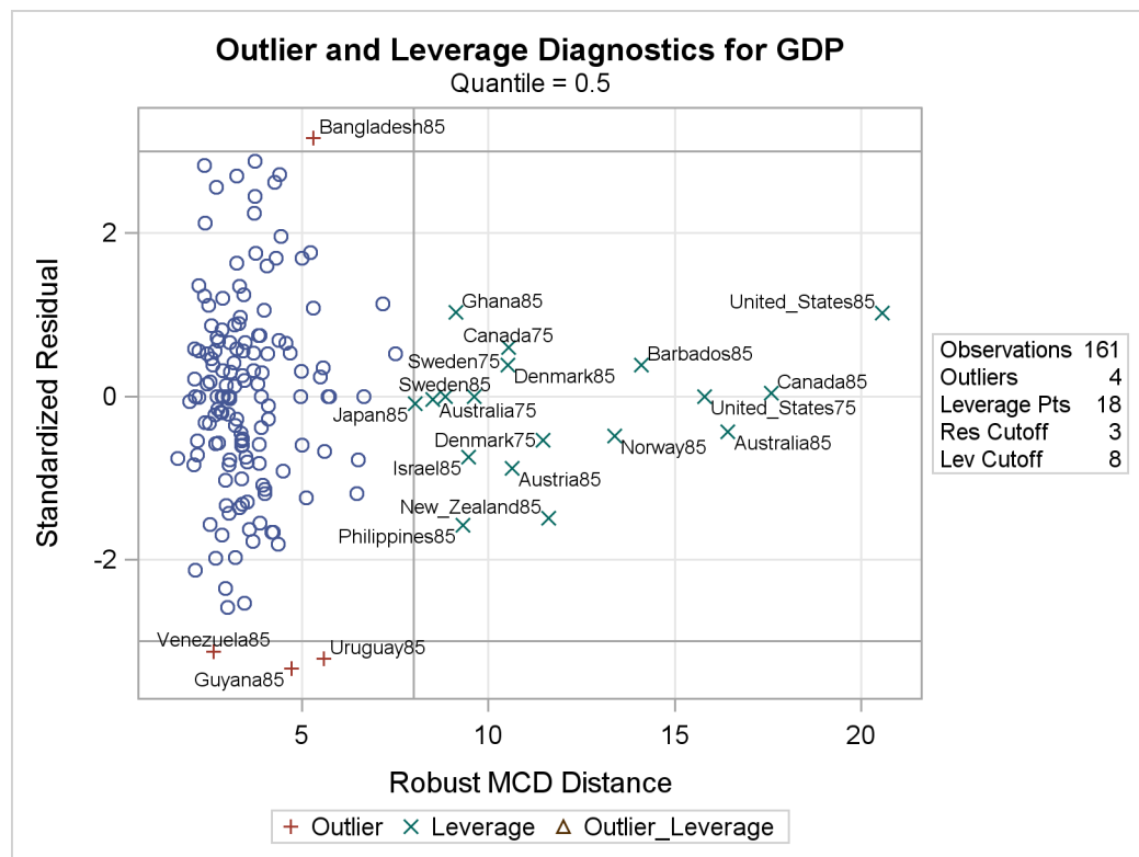
Output 72.2.3 Residual-Robust Distance Plot
