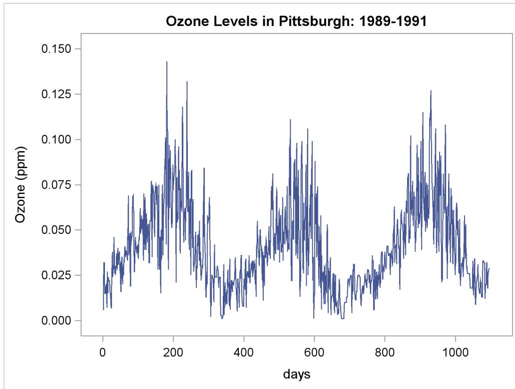
Output 72.4.1 Time Series of Ozone Levels in Pittsburgh, Pennsylvania
