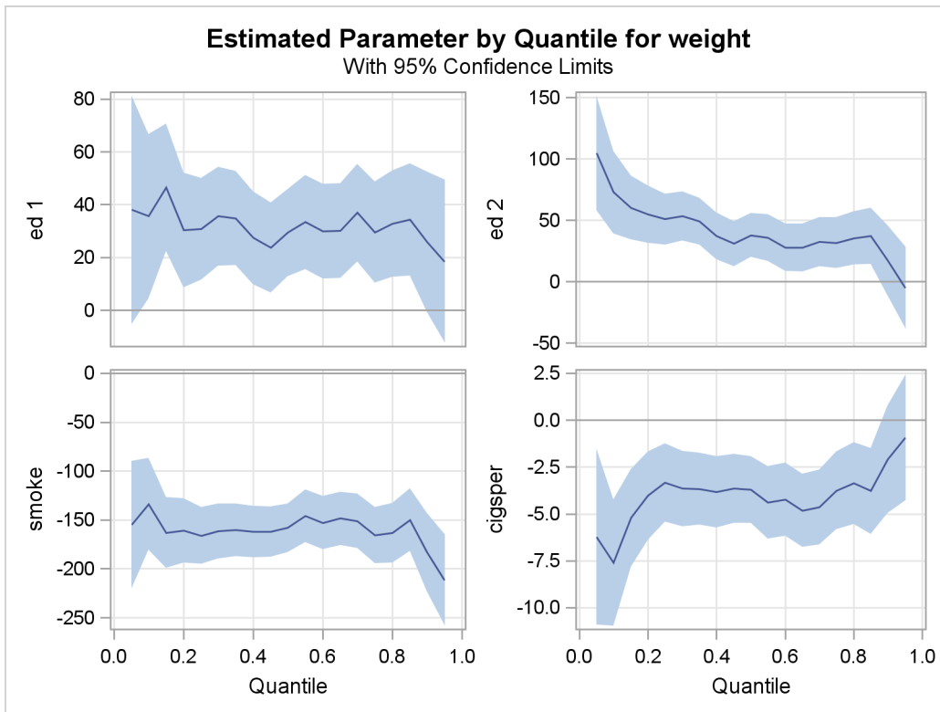
Output 72.3.4 Quantile Processes with 95% Confidence Bands
