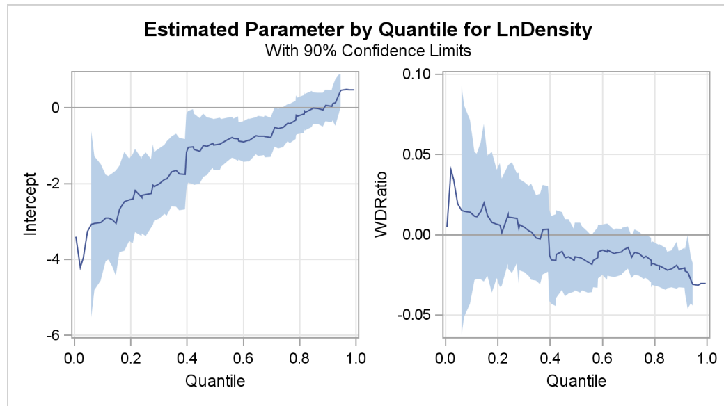
Figure 72.9 Quantile Processes for Intercept and Slope
