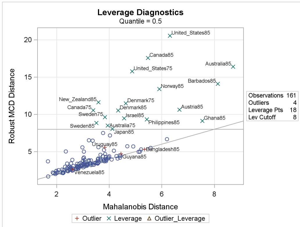
Output 72.2.4 Robust Distance-Mahalanobis Distance Plot
