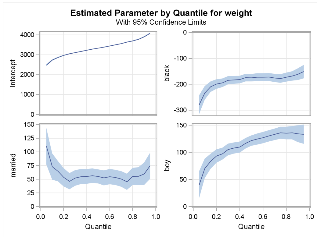
Output 72.3.2 Quantile Processes with 95% Confidence Bands
