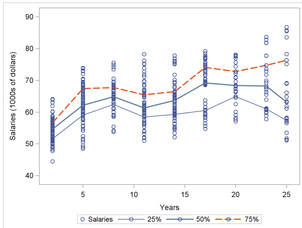
Output 72.5.2 Salary with Years as Professor: Sample Quantiles
