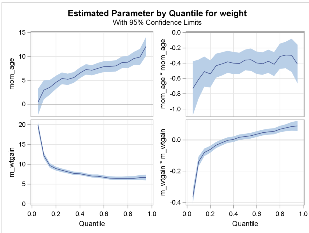
Output 72.3.5 Quantile Processes with 95% Confidence Bands
