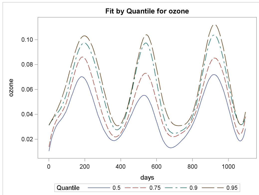
Output 72.4.2 Quantiles of Ozone Levels in Pittsburgh, Pennsylvania
