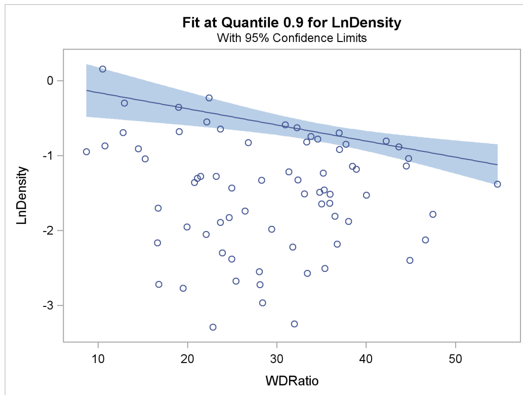
Figure 72.13 Fit Plot with Confidence Limits
