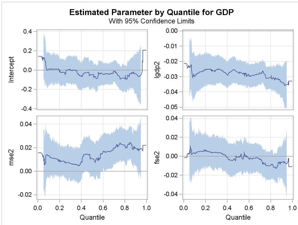
Output 72.2.7 Quantile Processes with 95% Confidence Bands
