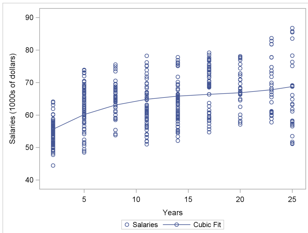
Output 72.5.1 Salary with Years as Professor: Cubit Fit
