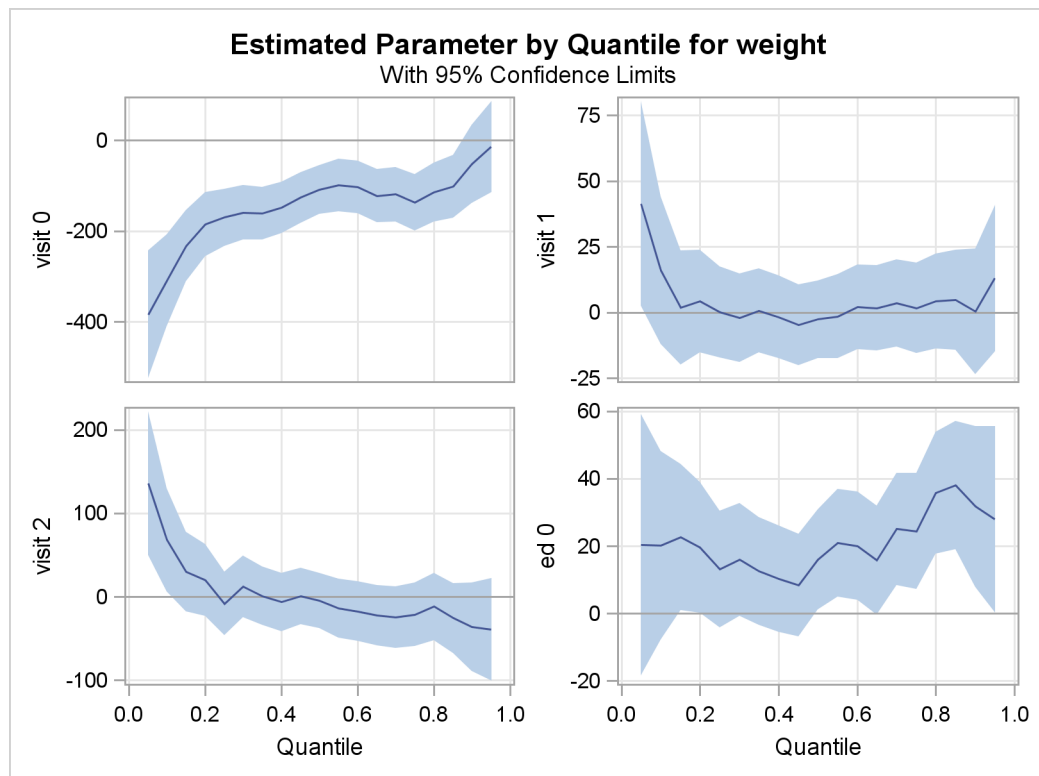
Output 72.3.3 Quantile Processes with 95% Confidence Bands
