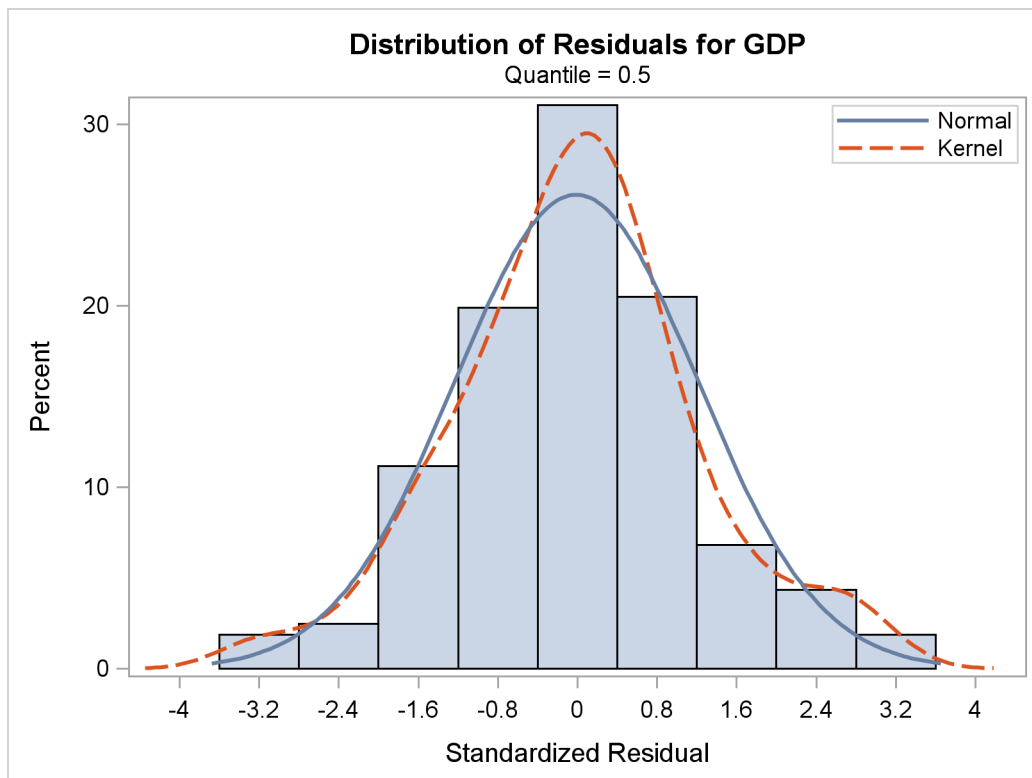
Output 72.2.5 Histogram for Residuals
