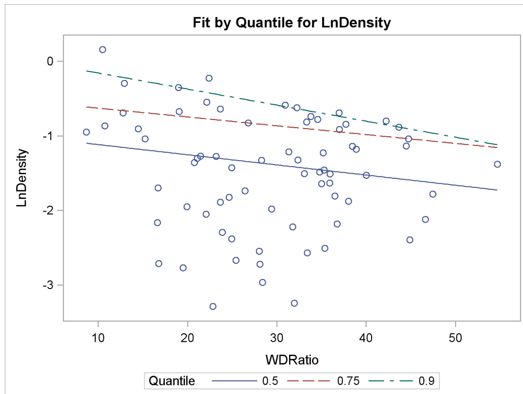
Figure 72.14 Fit Plot for Multiple Quantiles
