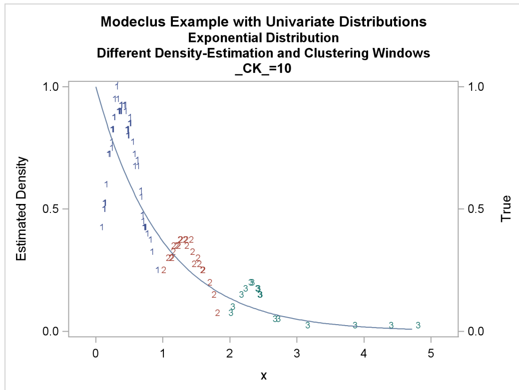
Output 57.1.10 True Density, Estimated Density, and Cluster Membership by \_R_=0.2 with Various \_CK\_ Values
