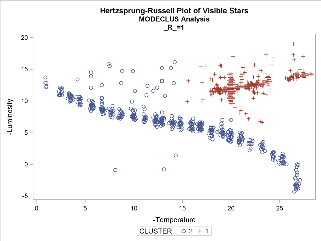
Output 57.4.3 Scatter Plots of Cluster Memberships by _R_ = 1
