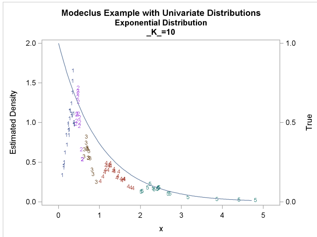
Output 57.1.6 True Density, Estimated Density, and Cluster Membership by Various _K_ Values
