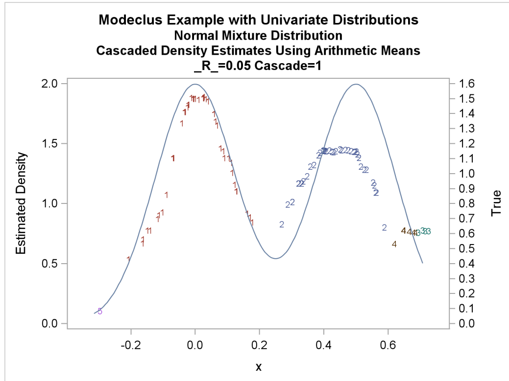
Output 57.1.18 True Density, Estimated Density, and Cluster Membership by \_R_=0.05 with Various \_CASCAD\_ Values
