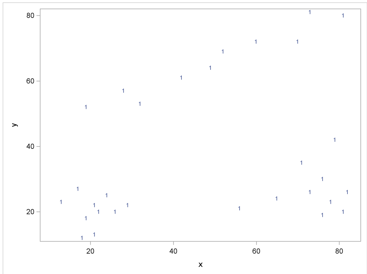
Figure 57.8 Scatter Plots of Cluster Memberships with _R_=35
