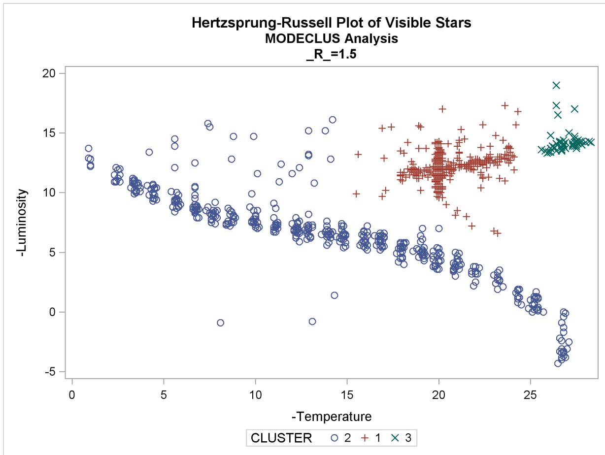
Output 57.4.4 Scatter Plots of Cluster Memberships by \_R\_ = 1.5
