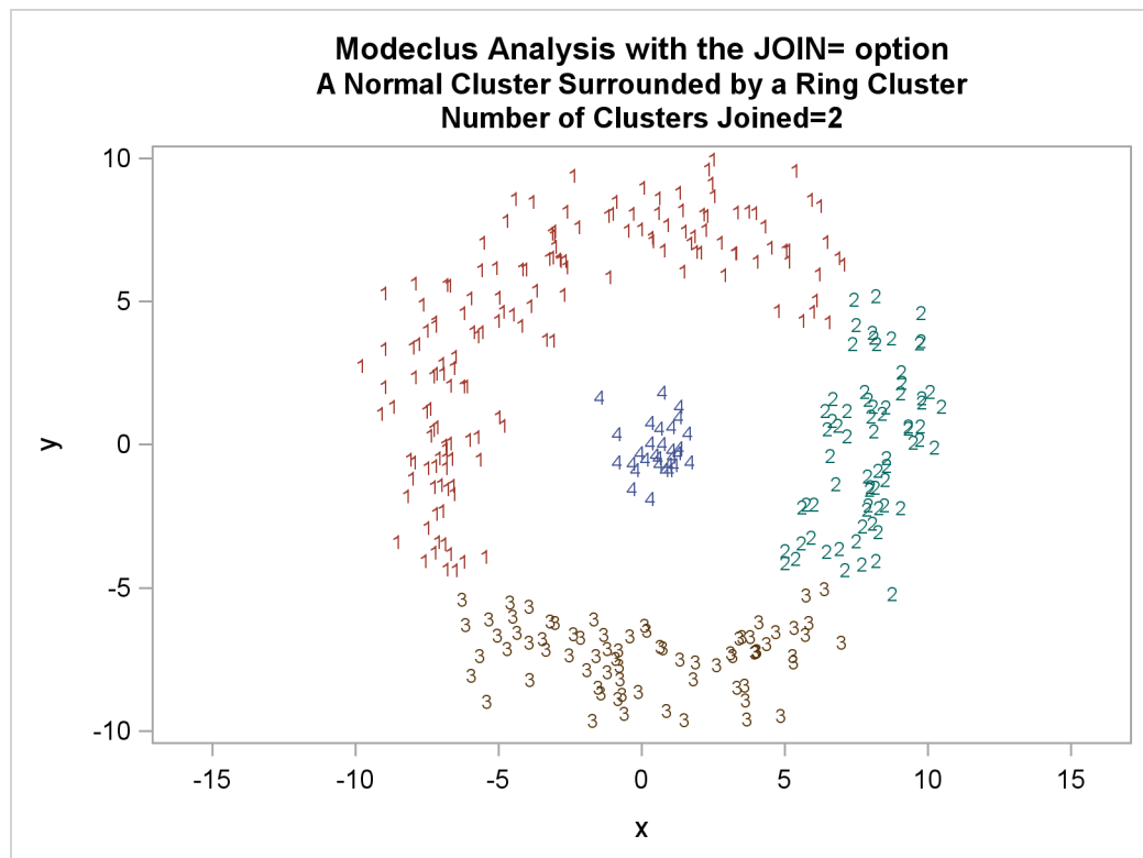
Output 57.3.5 Cluster Memberships When Number of Clusters Joined=2
