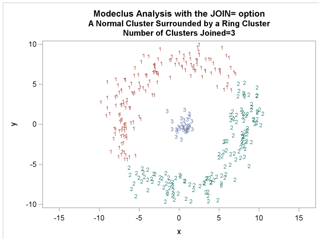
Output 57.3.6 Cluster Memberships When Number of Clusters Joined=3
