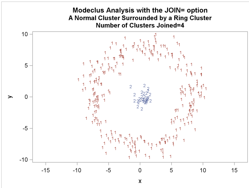
Output 57.3.7 Cluster Memberships When Number of Clusters Joined=4
