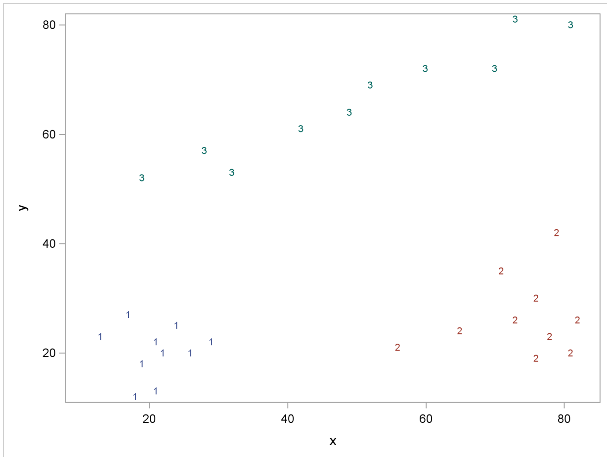
Figure 57.7 Scatter Plots of Cluster Memberships with _R_=15
