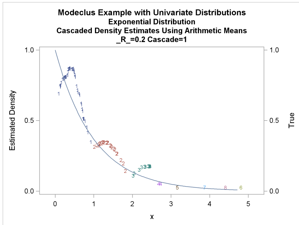
Output 57.1.12 True Density, Estimated Density, and Cluster Membership by \_R_=0.2 with Various \_CASCAD\_ Values
