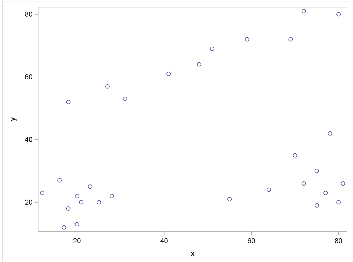
Figure 57.1 Scatter Plot of Data
