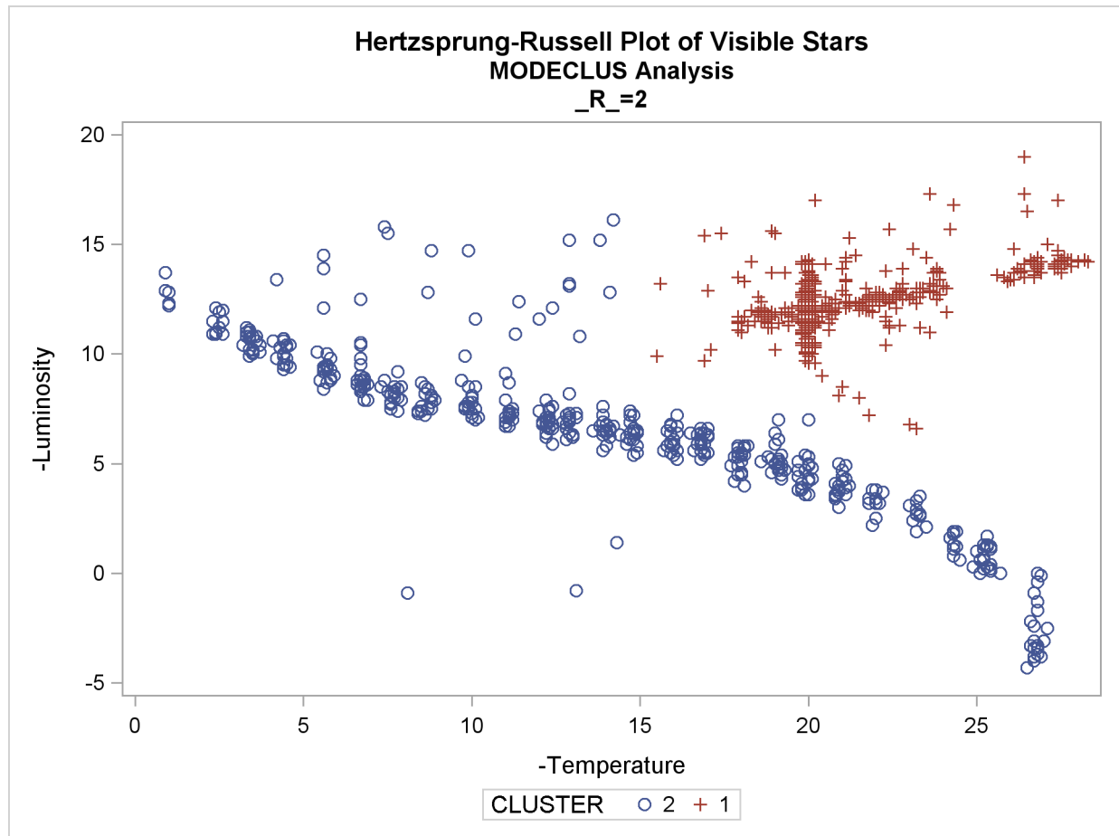
Output 57.4.5 Scatter Plots of Cluster Memberships by _R_=2
