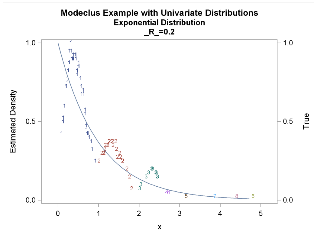
Output 57.1.8 True Density, Estimated Density, and Cluster Membership by Various \_R\_ Values
