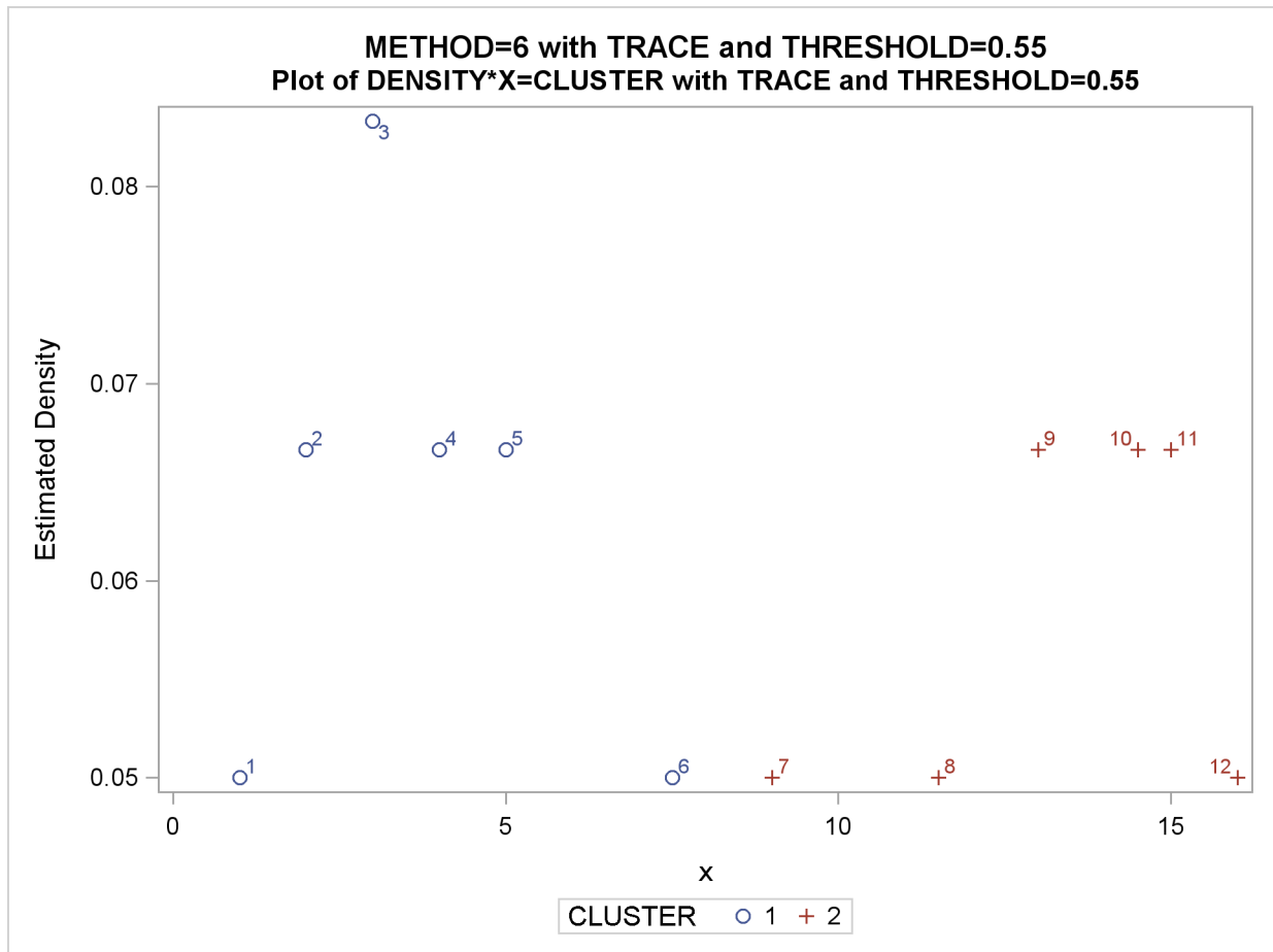
Output 57.5.4 Density Plot
