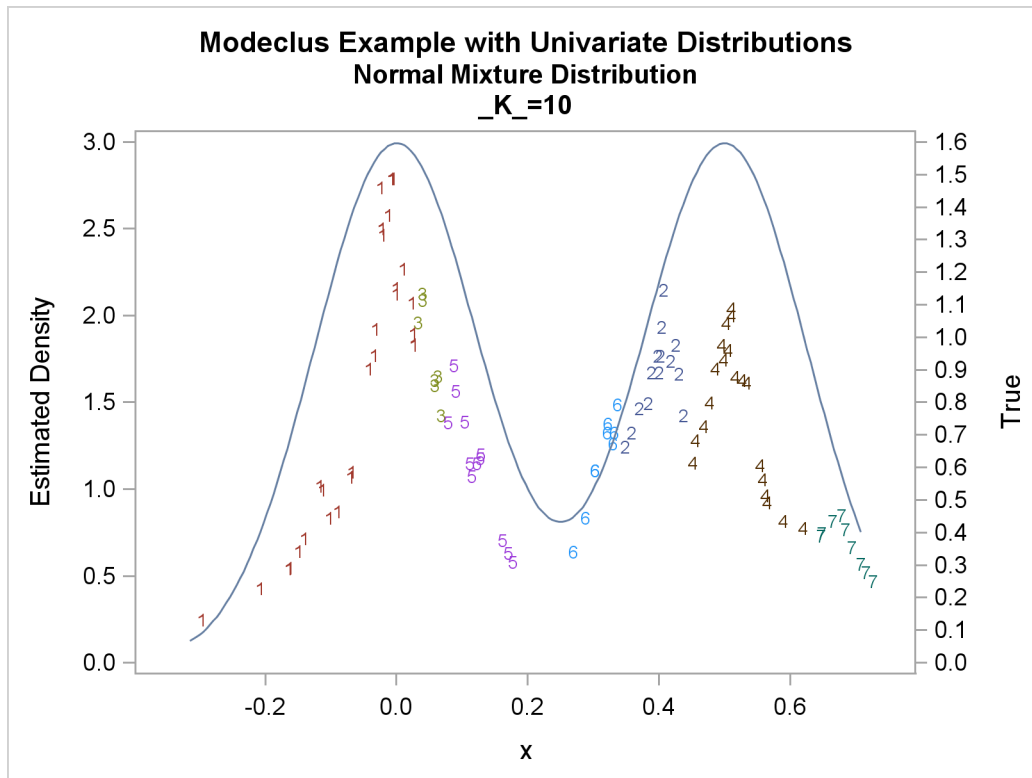
Output 57.1.14 True Density, Estimated Density, and Cluster Membership by Various _K Values
