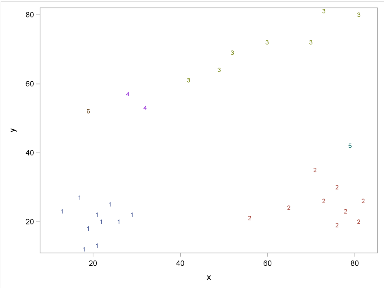
Figure 57.6 Scatter Plots of Cluster Memberships with _R_=10
