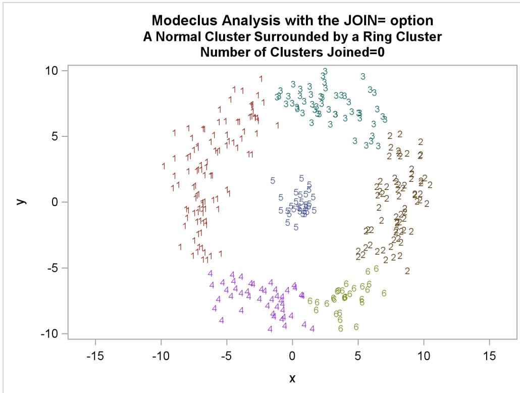
Output 57.3.3 Cluster Memberships When Number of Clusters Joined=0
