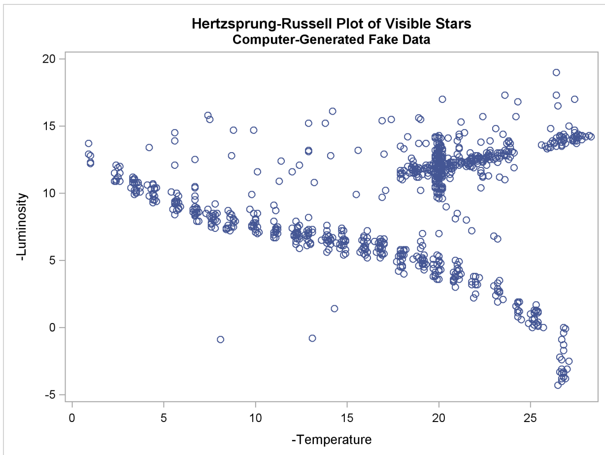
Output 57.4.1 Scatter Plot of Data
