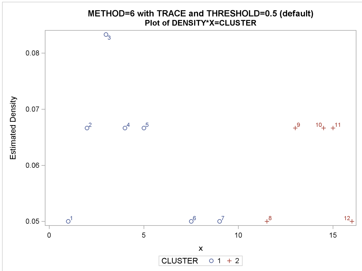
Output 57.5.2 Density Plot
