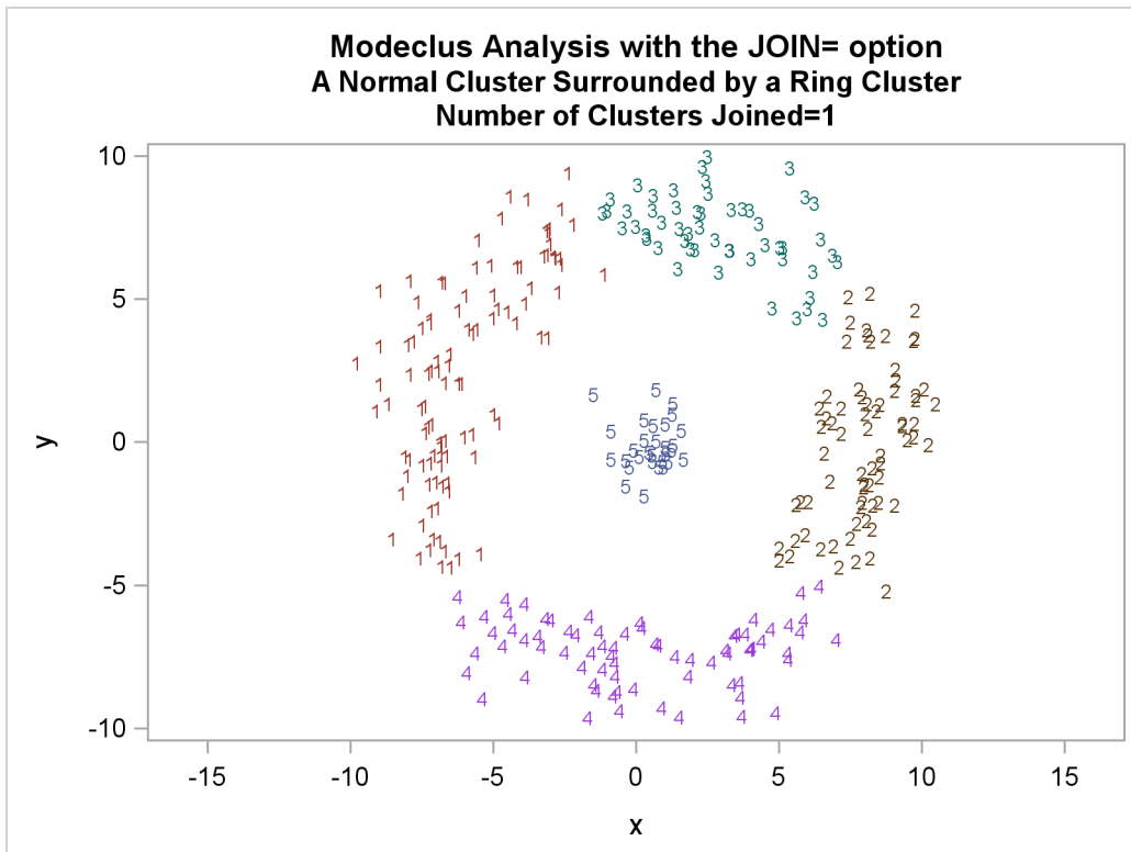
Output 57.3.4 Cluster Memberships When Number of Clusters Joined=1
