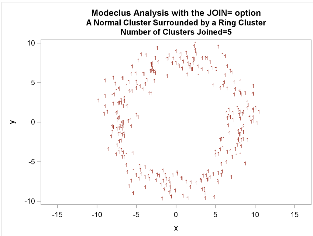
Output 57.3.8 Cluster Memberships When Number of Clusters Joined=5
