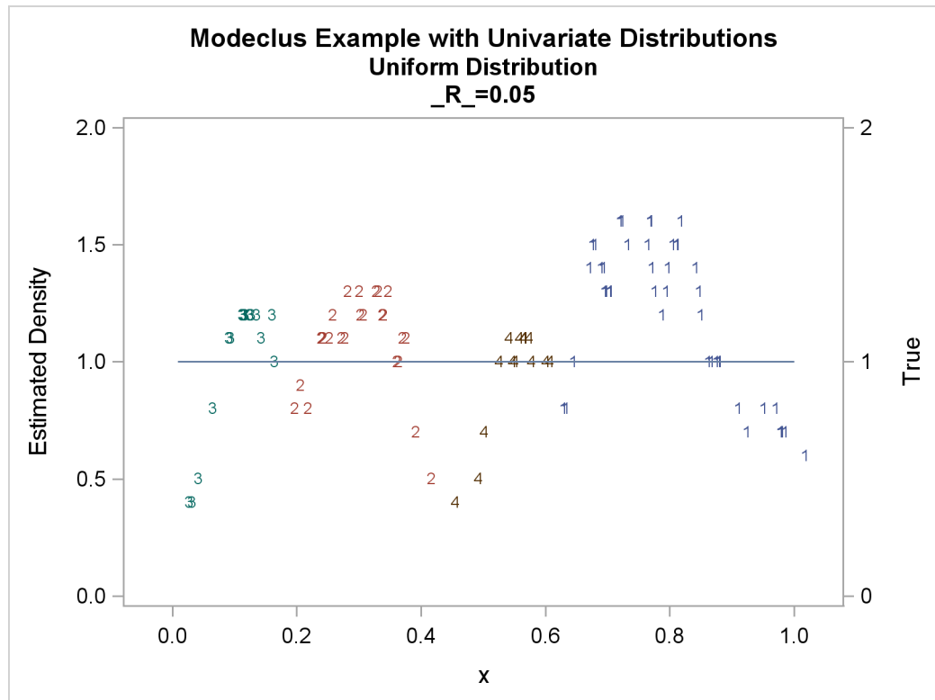
Output 57.1.4 True Density, Estimated Density, and Cluster Membership by Various _R_ Values
