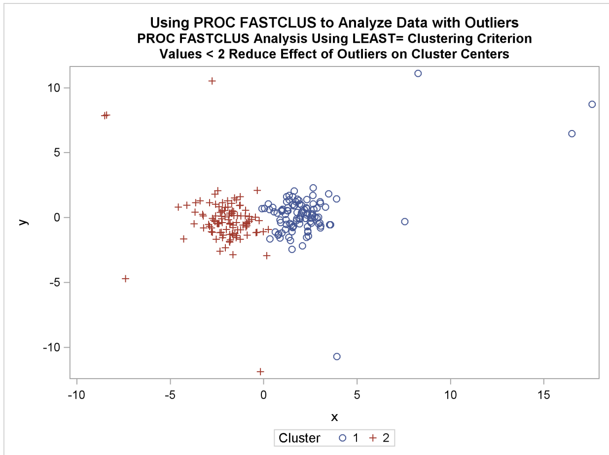
Output 34.2.4 Analysis Plot of Data with Outliers
