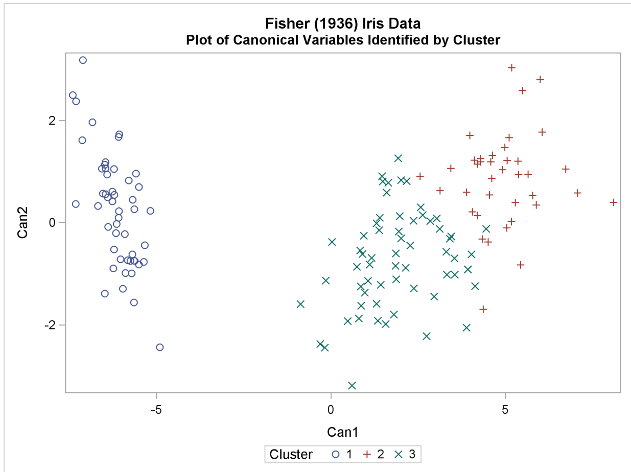
Output 34.1.4 Plot of Fisher's Iris Data using PROC CANDISC
