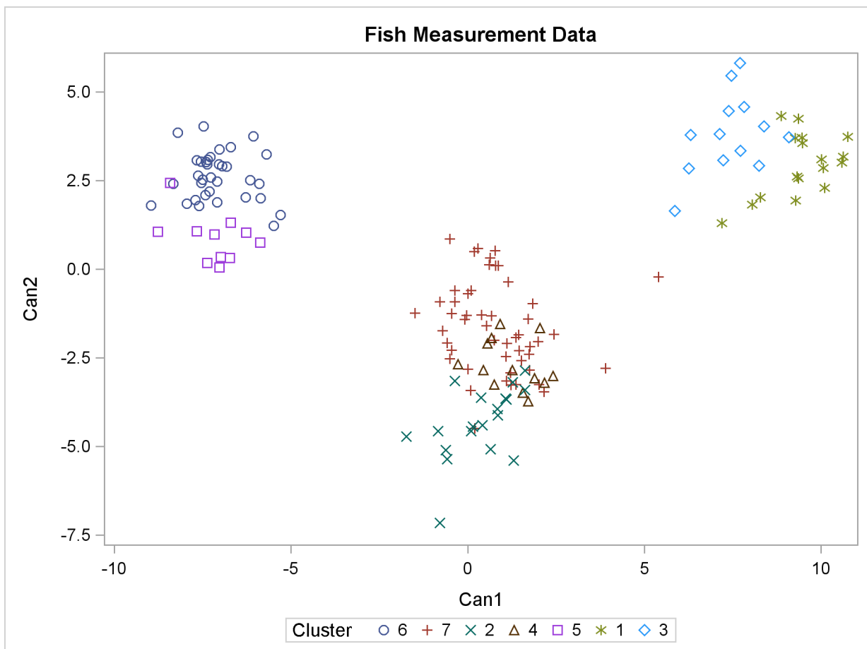
Figure 34.6 Plot of Canonical Variables and Cluster Value
