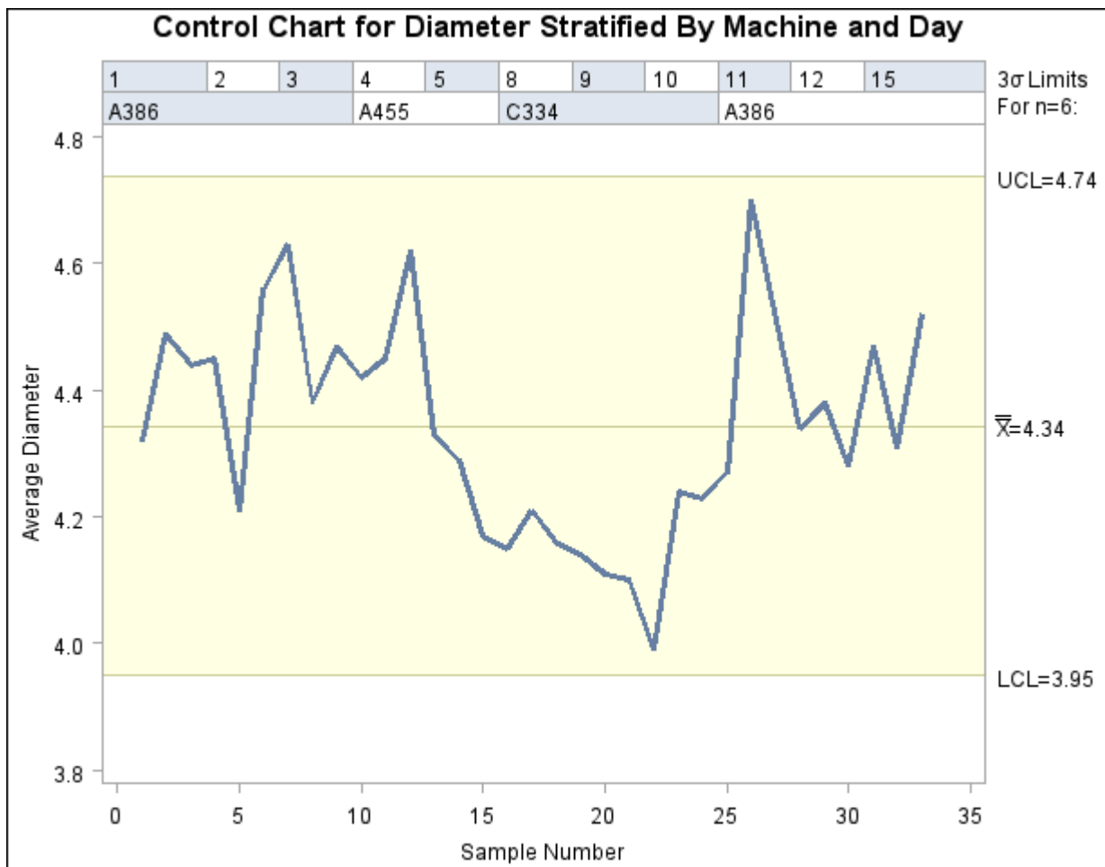
Output 13.43.28 Stratified Control Chart Using Multiple Block Variables
