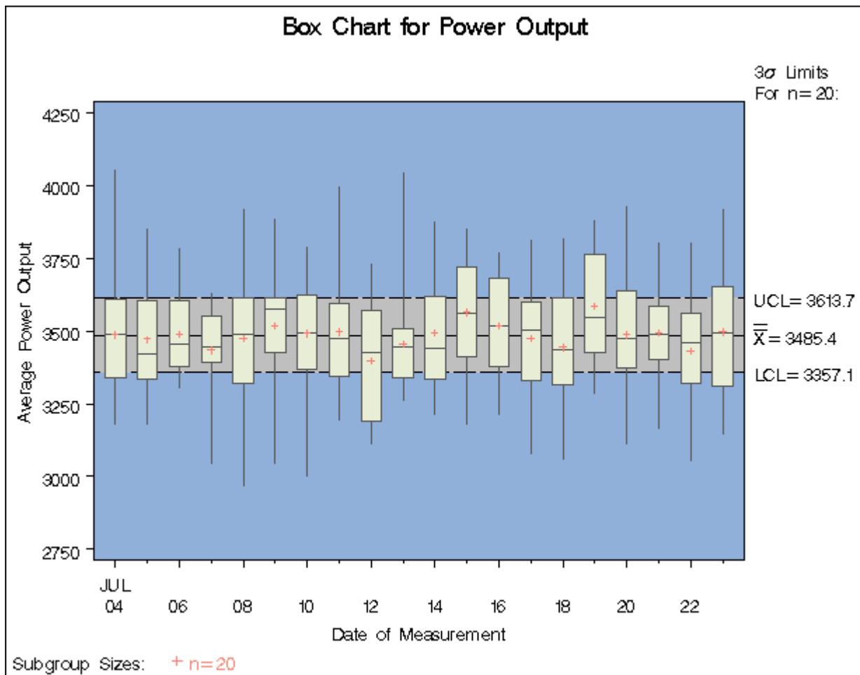
Figure 13.7 Box Chart for Power Output Data (Traditional Graphics with NOGSTYLE)
