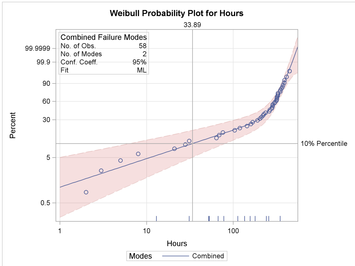
Figure 12.29 Weibull Plot for Failure Modes D and E
