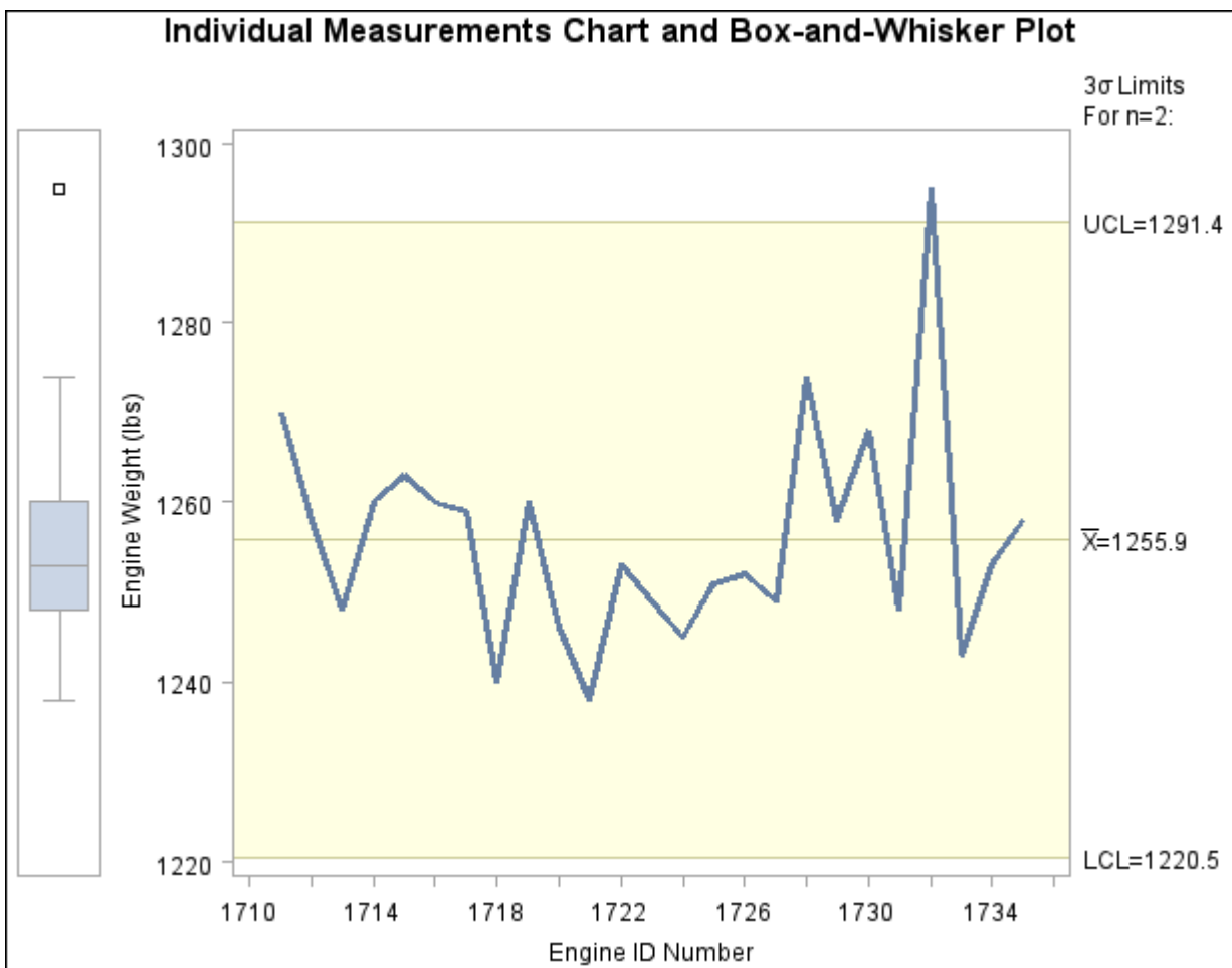
Output 13.13.2 Box-and-Whisker Plot in Left Margin
