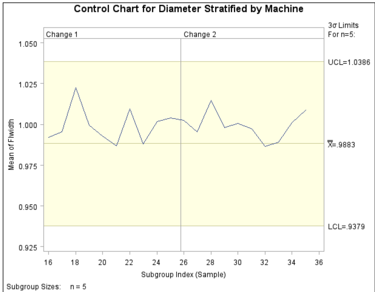
Output 13.43.34 A Single Set of Control Limits for Multiple Phases
