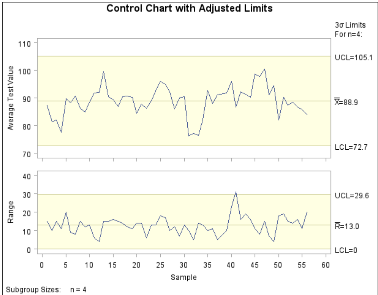
Output 13.43.85 \bar{X} and R Chart with Derived Control Limits
