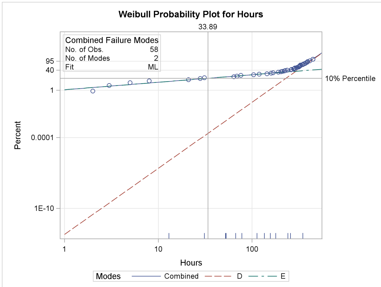
Figure 12.30 Weibull Plot for Failure Modes D and E with Individual Modes
