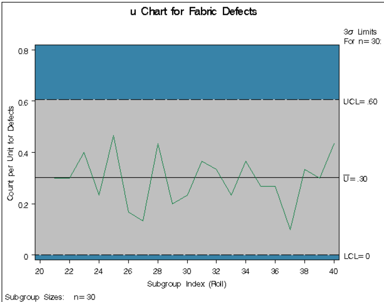
Output 13.30.7 A u Chart for Second Set of Fabric Rolls (Traditional Graphics with NOGSTYLE)
