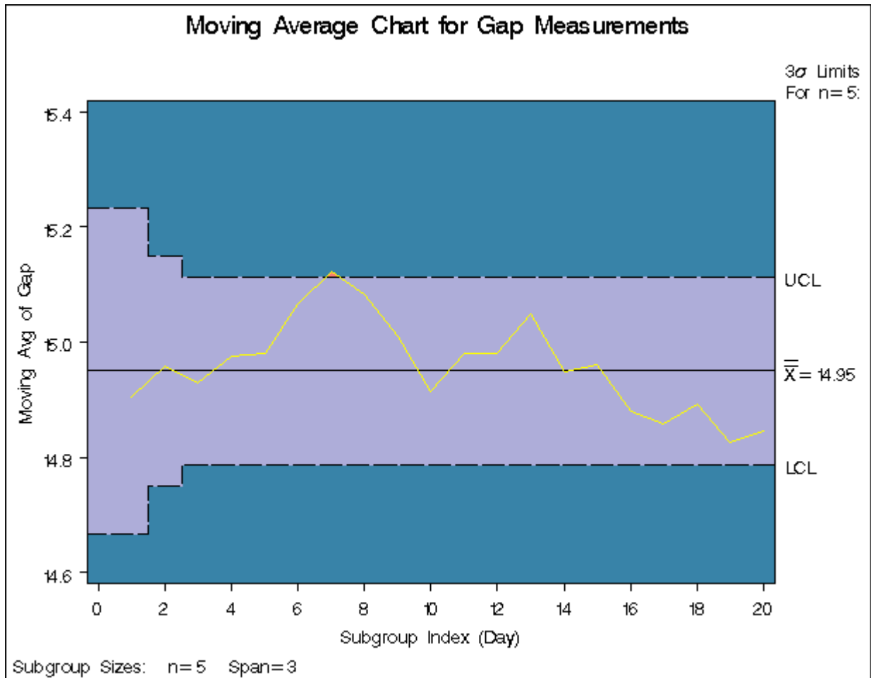
Output 9.5.6 Uniformly Weighted Moving Average Chart from Summary Data
