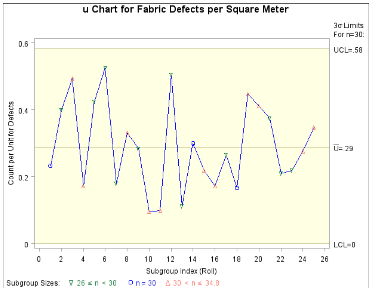
Output 13.33.4 Control Limits Based on Fixed Subgroup Sample Size
