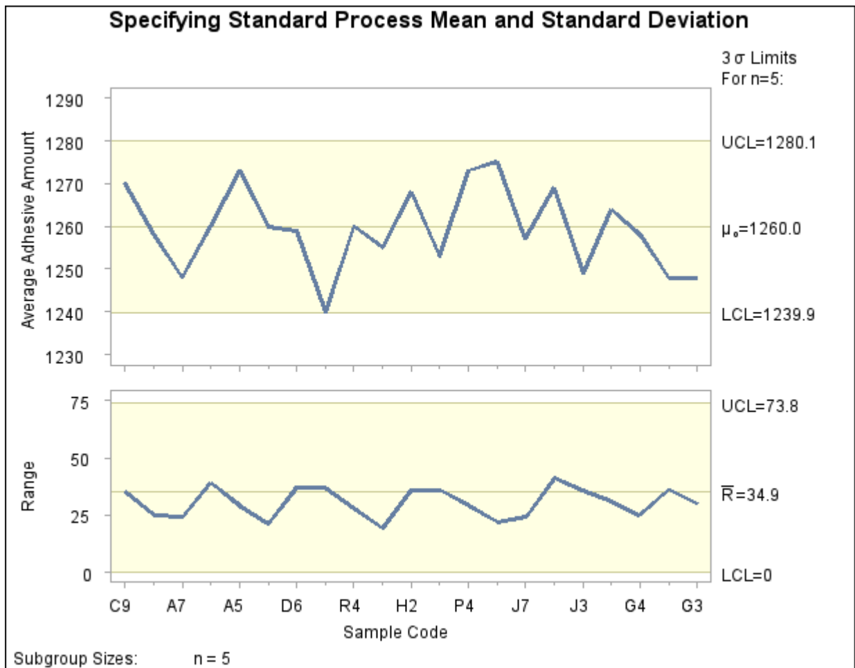
Output 13.39.1 Specifying Standard Values with MU0= and SIGMA0=
