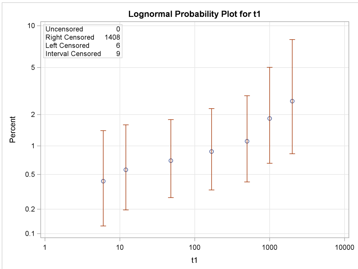
Figure 12.46 Lognormal Probability Plot for the Microprocessor Data
