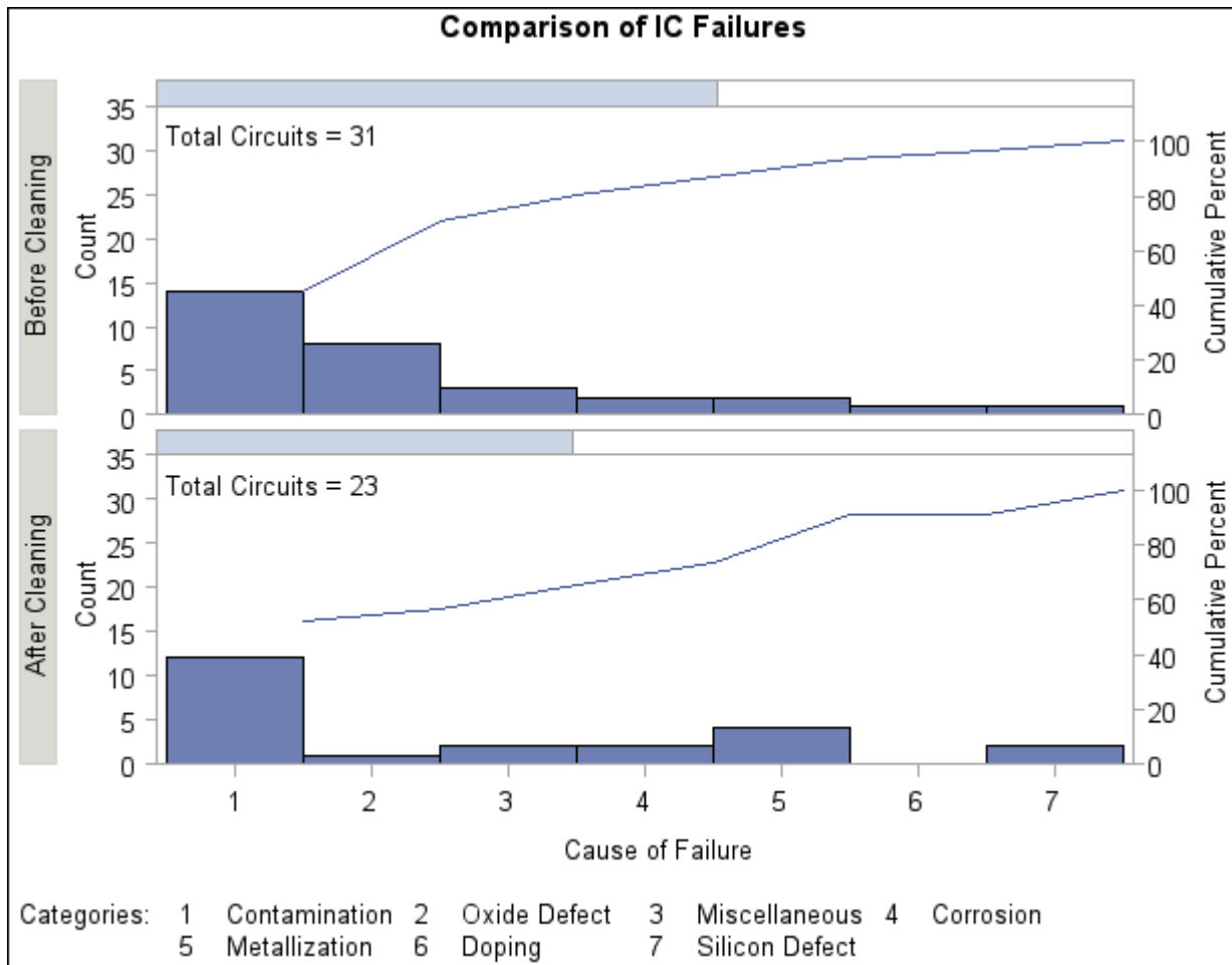
Output 11.1.4 Before-and-After Analysis Using Comparative Pareto Chart
