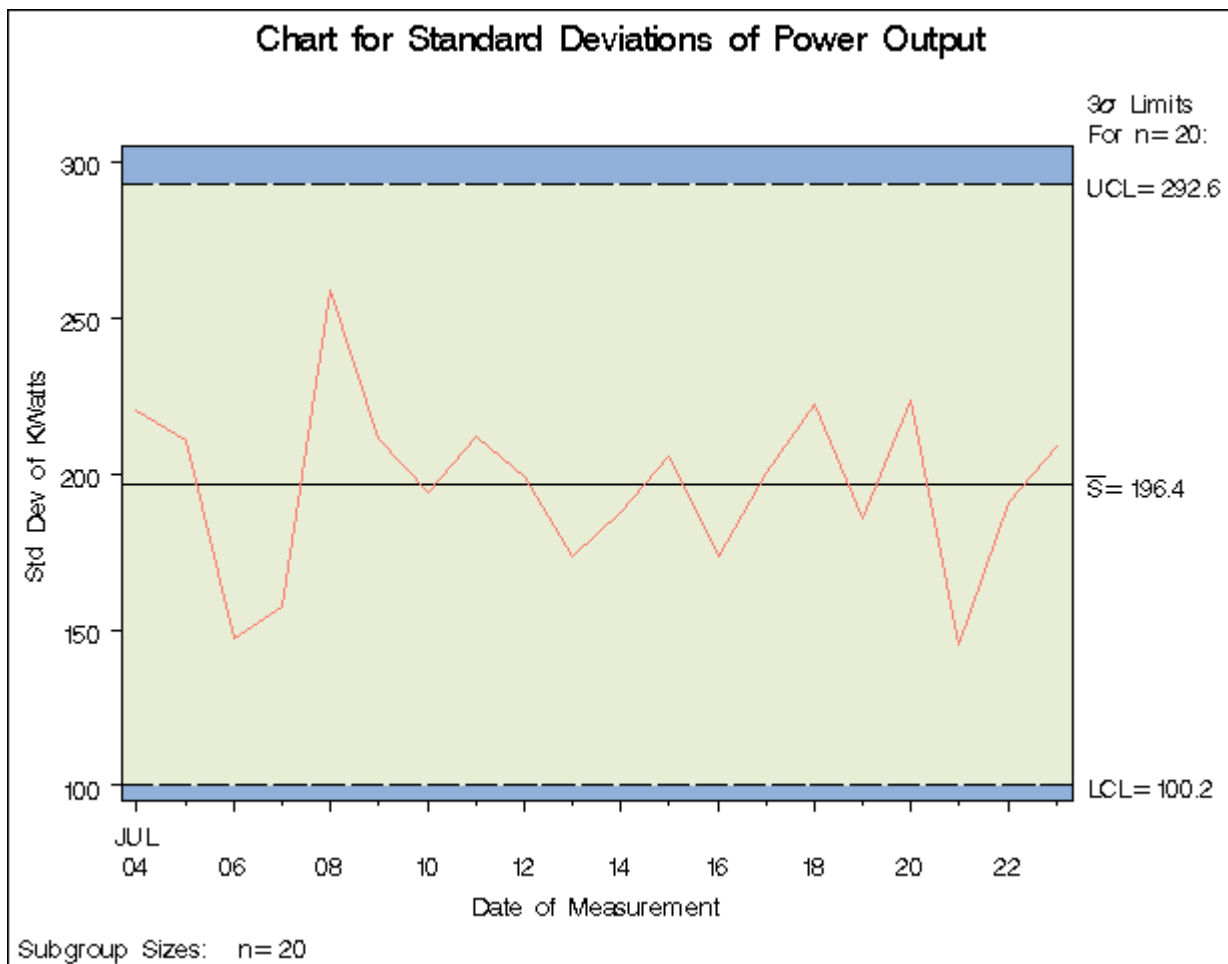
Output 13.28.6 s Chart for Power Output Data (Traditional Graphics with NOGSTYLE)
