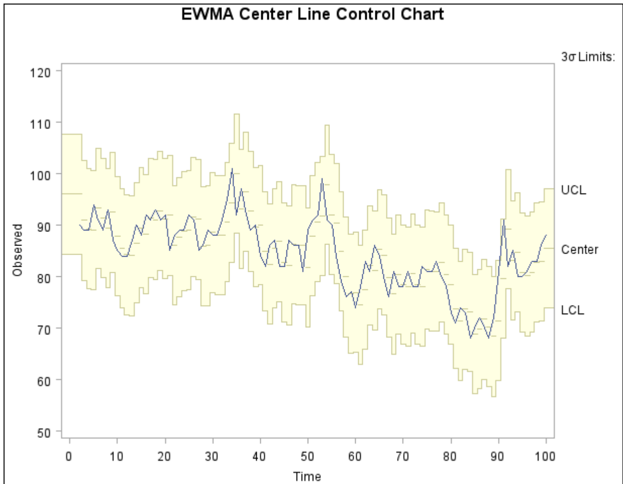
Output 13.43.79 EWMA Center Line Chart
