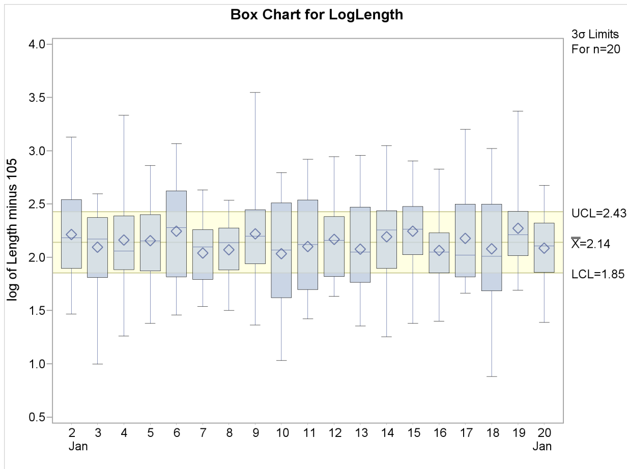
Output 13.43.3 Box Chart for Transformed Data
