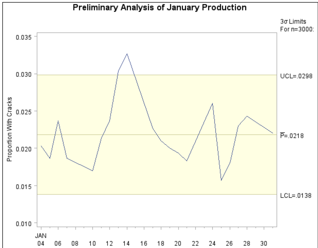
Output 13.43.57 Preliminary p Chart for January Data
