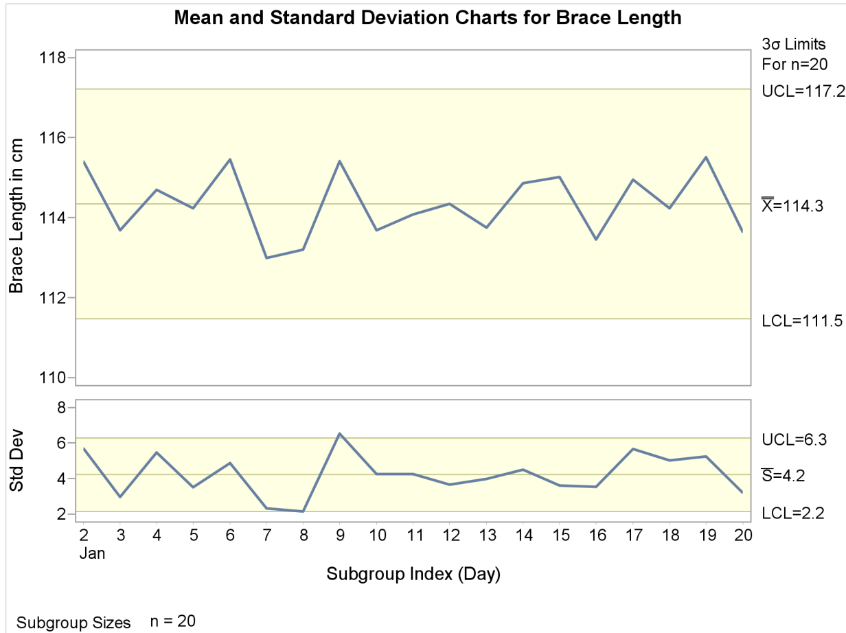
Output 13.43.1 \bar{X} and s Charts
