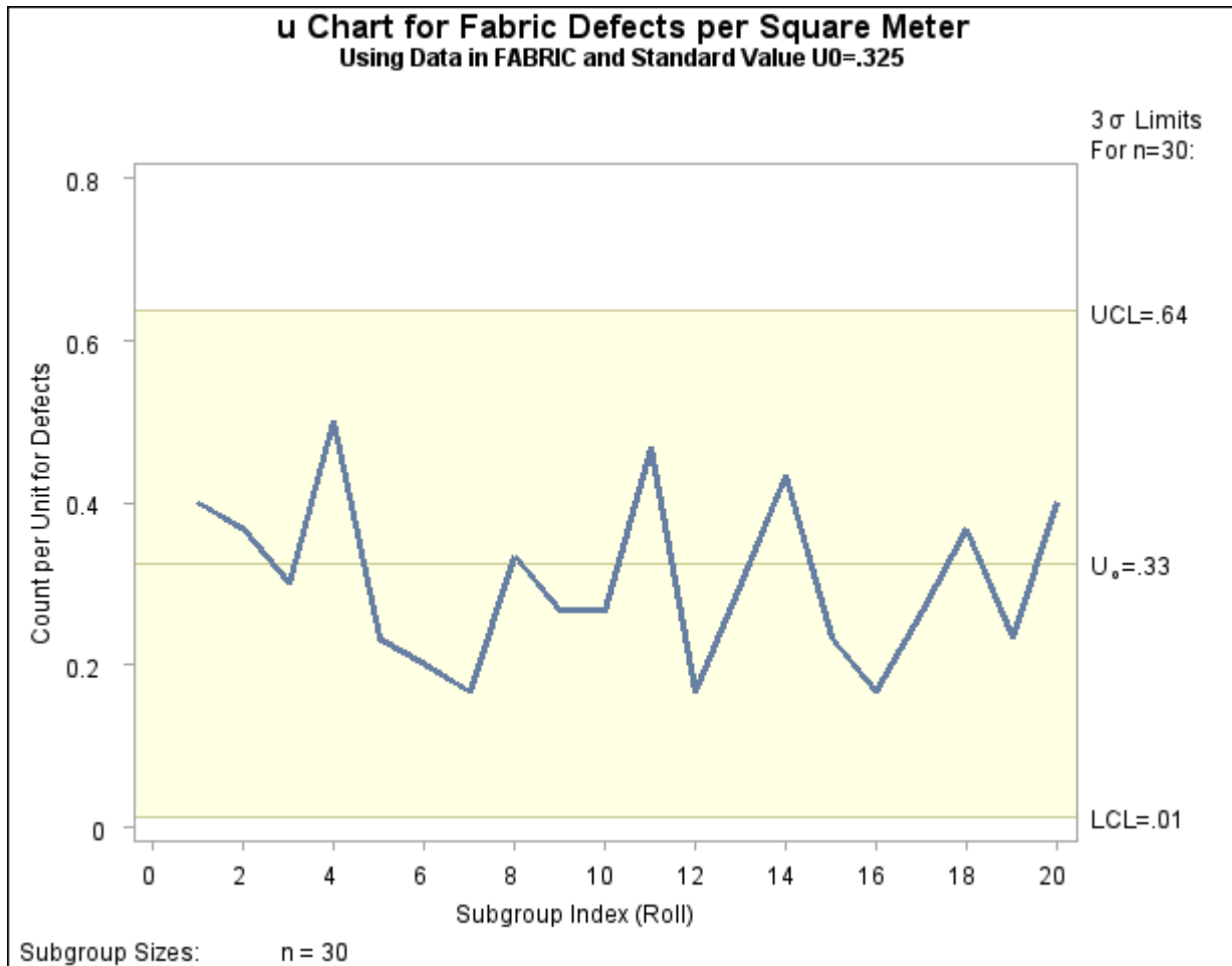
Output 13.32.1 A u Chart with Standard Value u_0
