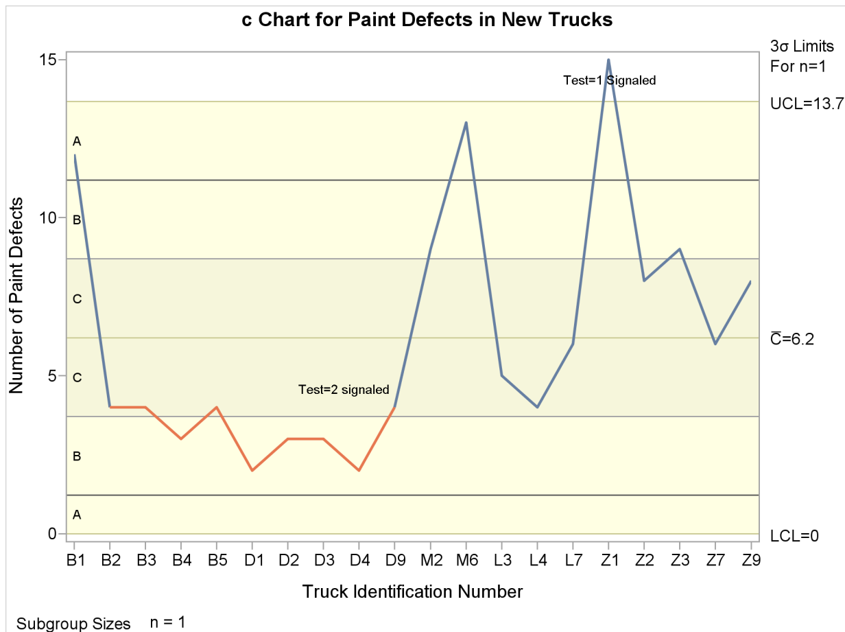
Output 13.8.1 Tests for Special Causes Displayed on c Chart
