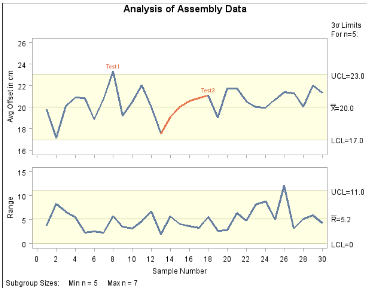
Output 13.43.63 Standard Tests Using the TESTS= Option
