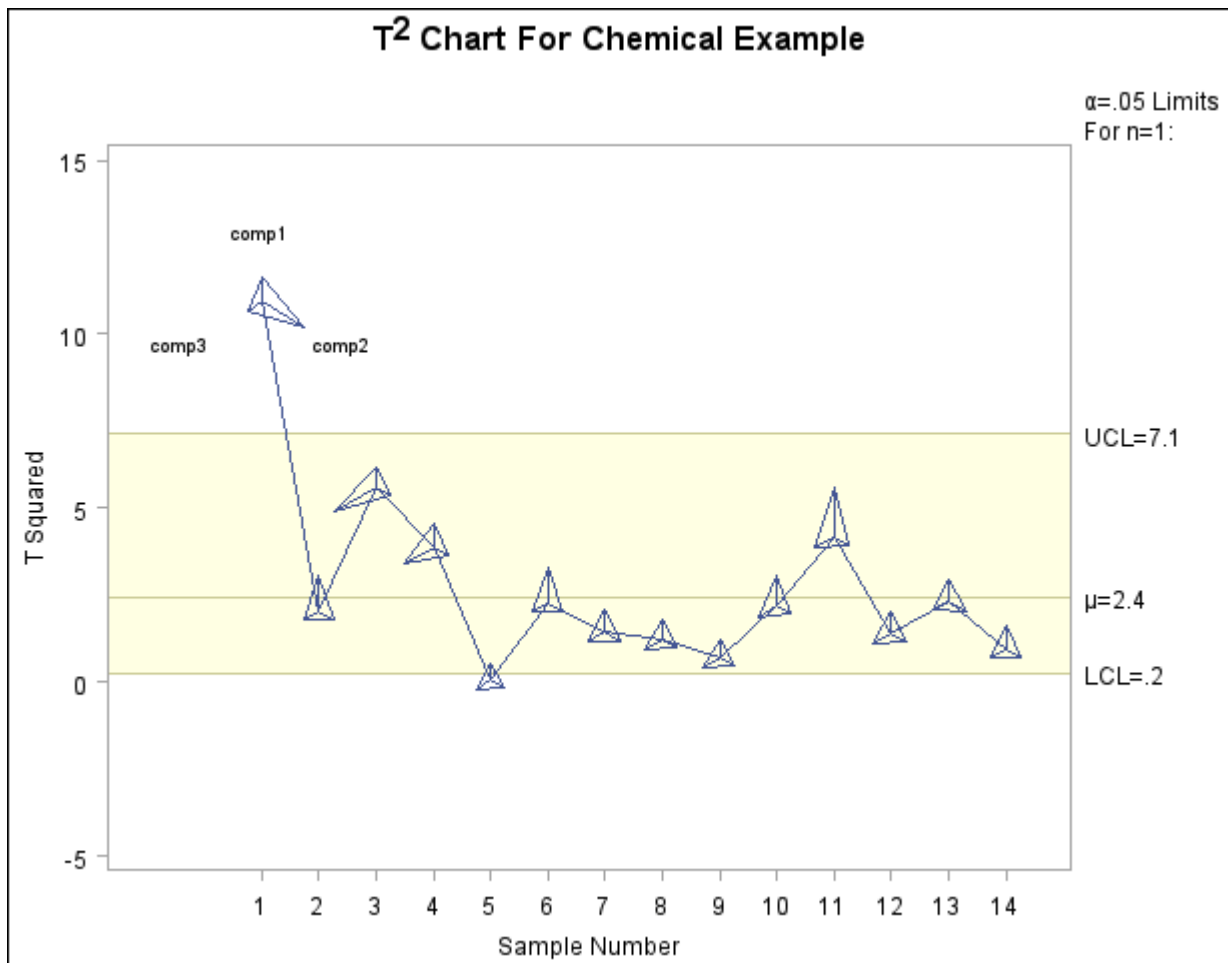
Output 13.43.105 Multivariate Control Chart Displaying Principal Components
