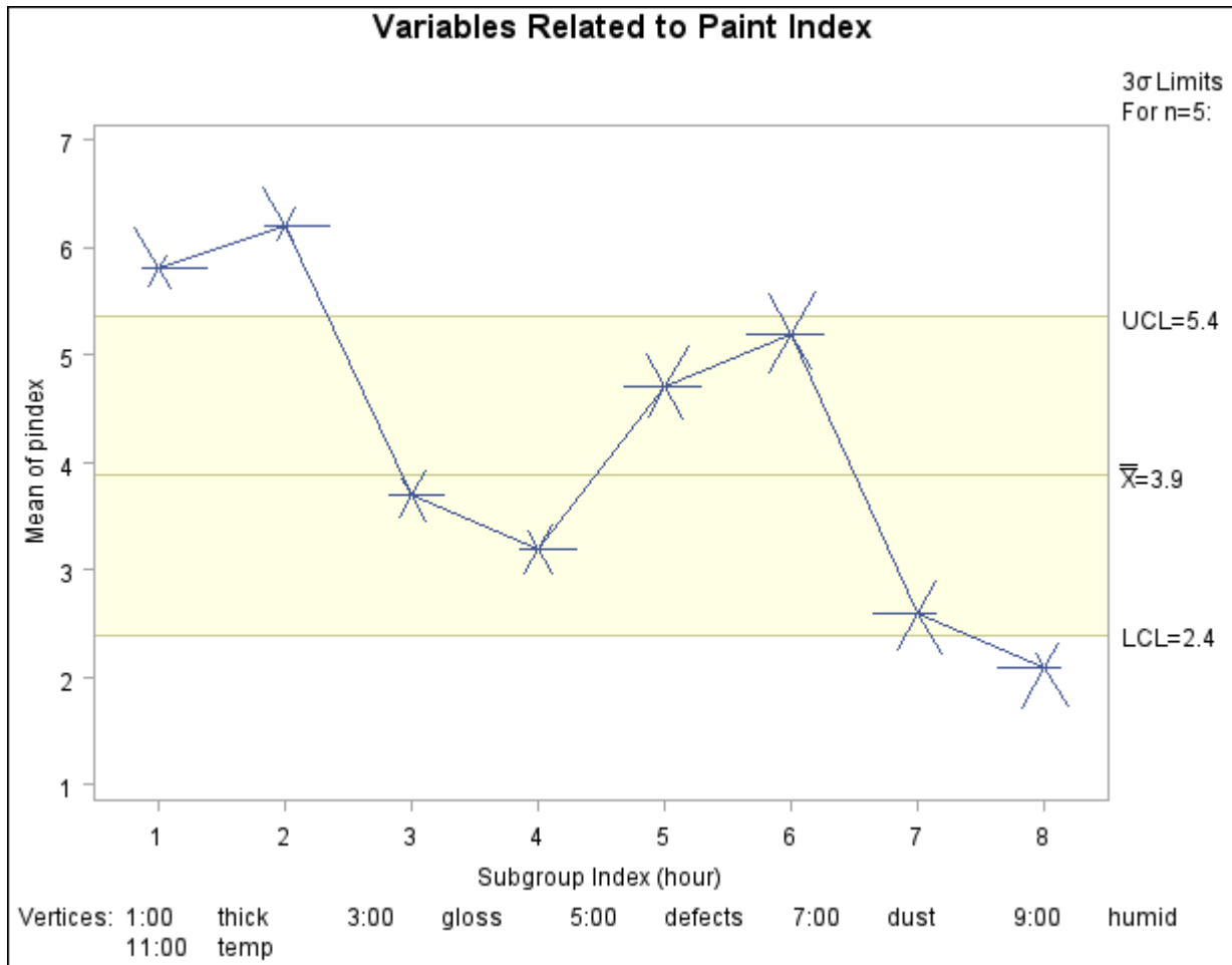
Output 13.43.44 Star Chart Using STARTYPE=RADIAL
