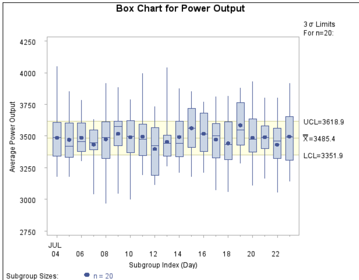
Figure 13.4 Box Chart for Power Output Data (Traditional Graphics)
