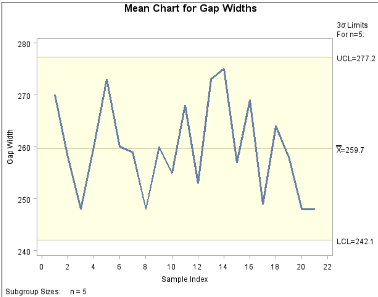
Output 13.33.7 \bar{X} Chart for Gap Width Data (Traditional Graphics)
