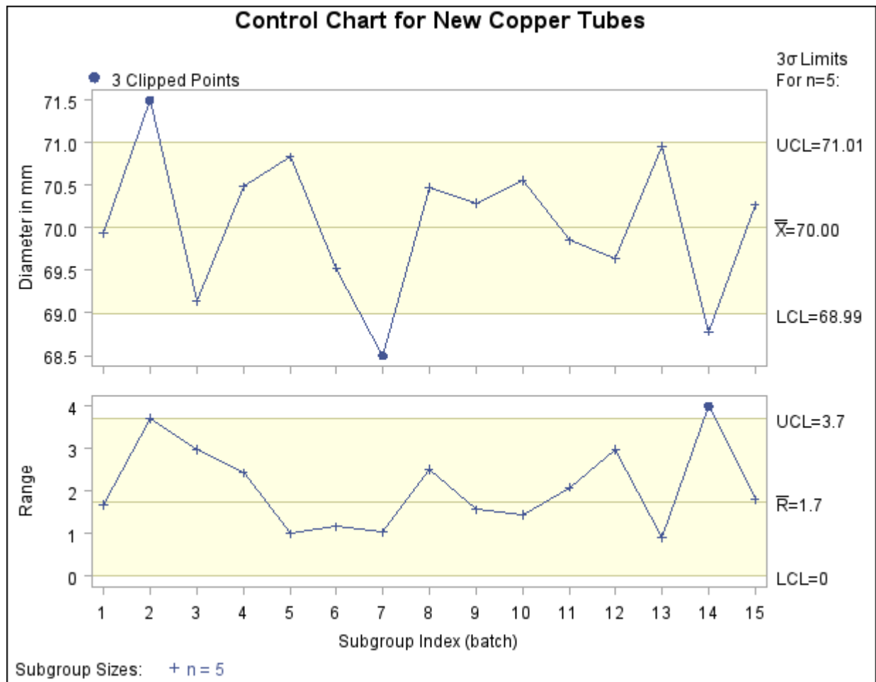
Output 13.43.54 \bar{X} and R Charts Using Clipping Options
