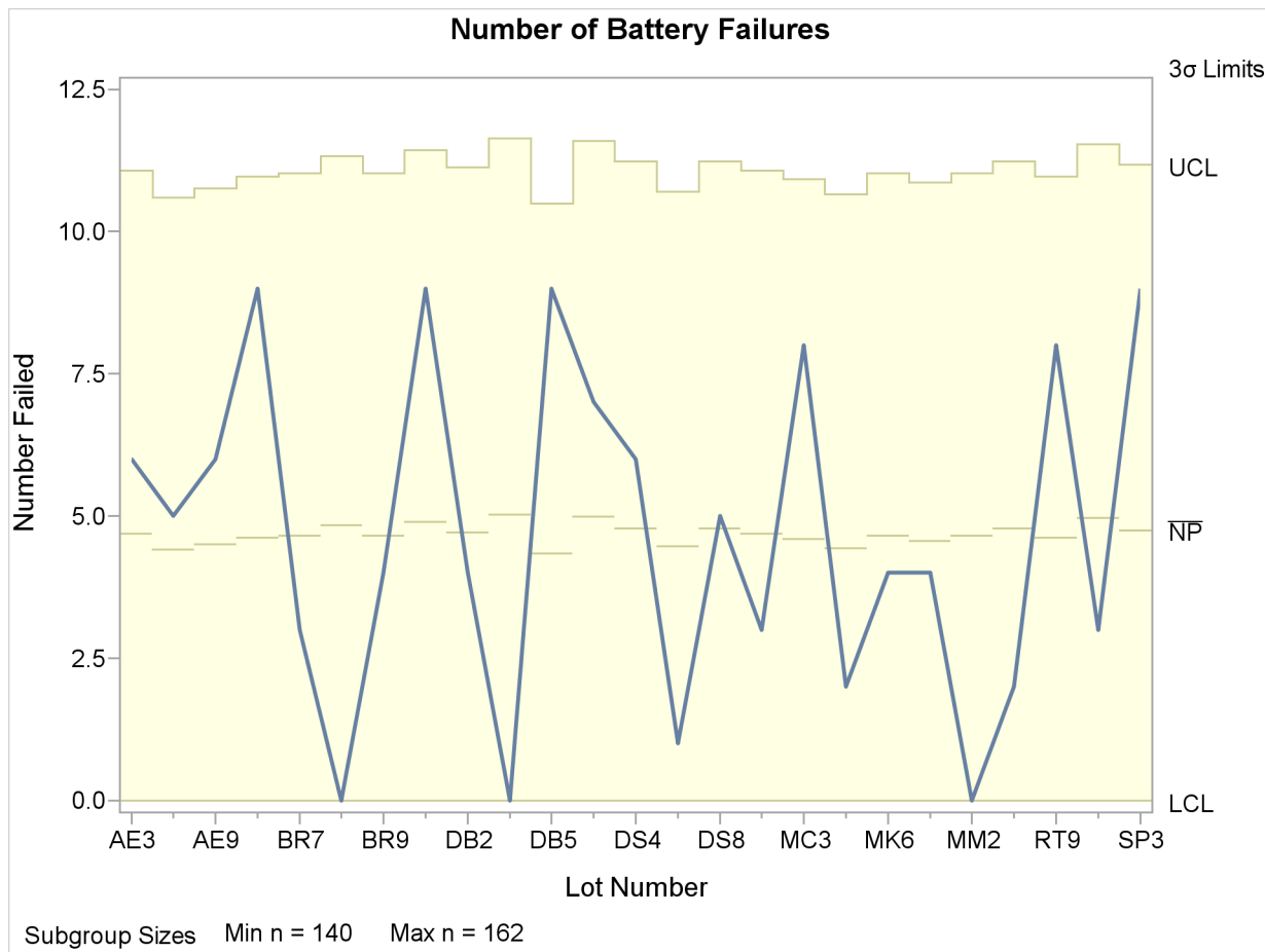
Output 13.20.1 An np Chart with Varying Subgroup Sample Sizes
