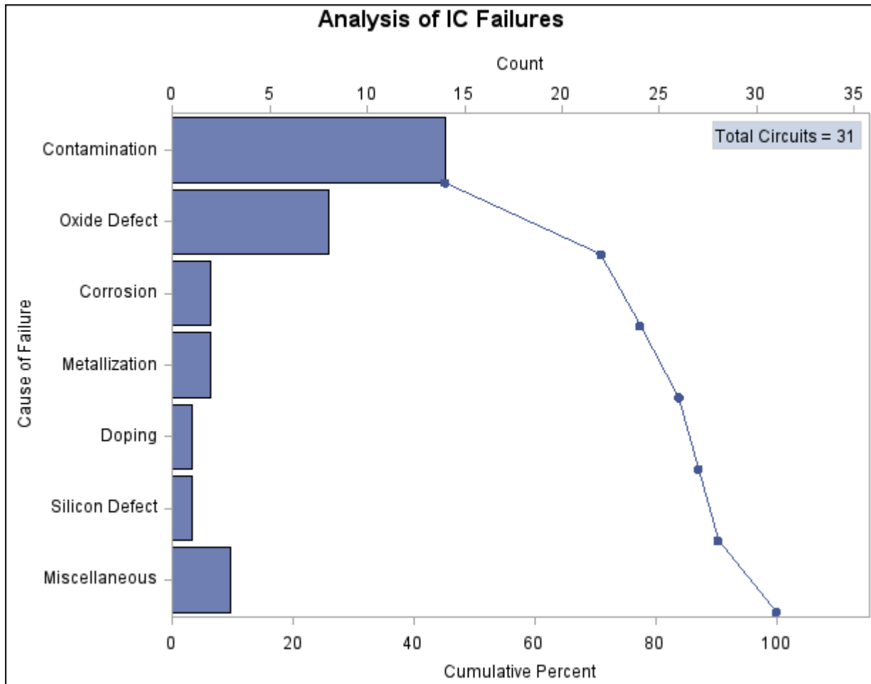
Figure 11.3 Pareto Chart with Frequency Scale
