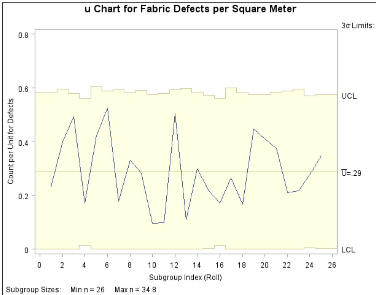
Output 13.33.2 A u Chart with Varying Number of Units per Subgroup
