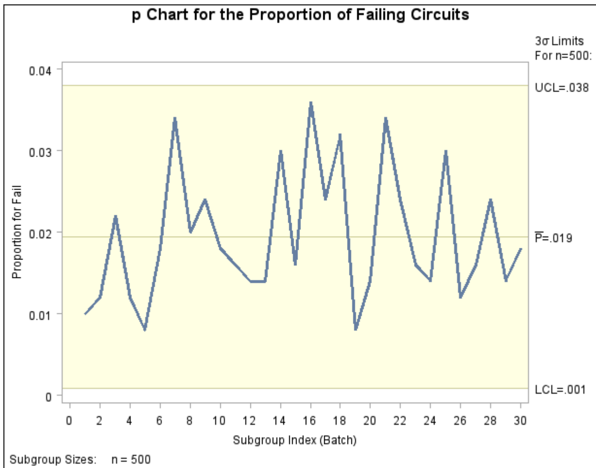
Output 13.21.4 p Chart for Circuit Failures (Traditional Graphics)
