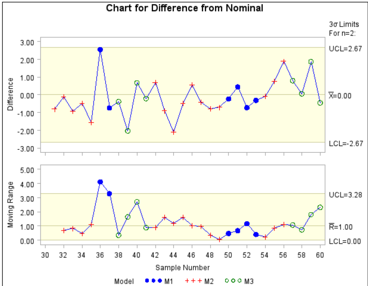
Output 13.43.92 Short Run Control Chart
