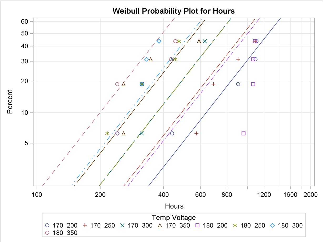
Figure 12.25 Probability Plot for Glass Capacitor Regression Model
