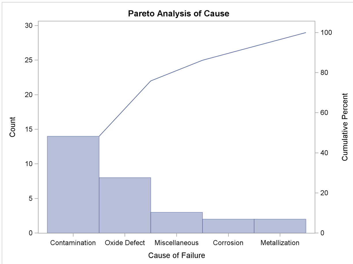
Figure 11.10 Restricted Pareto Chart
