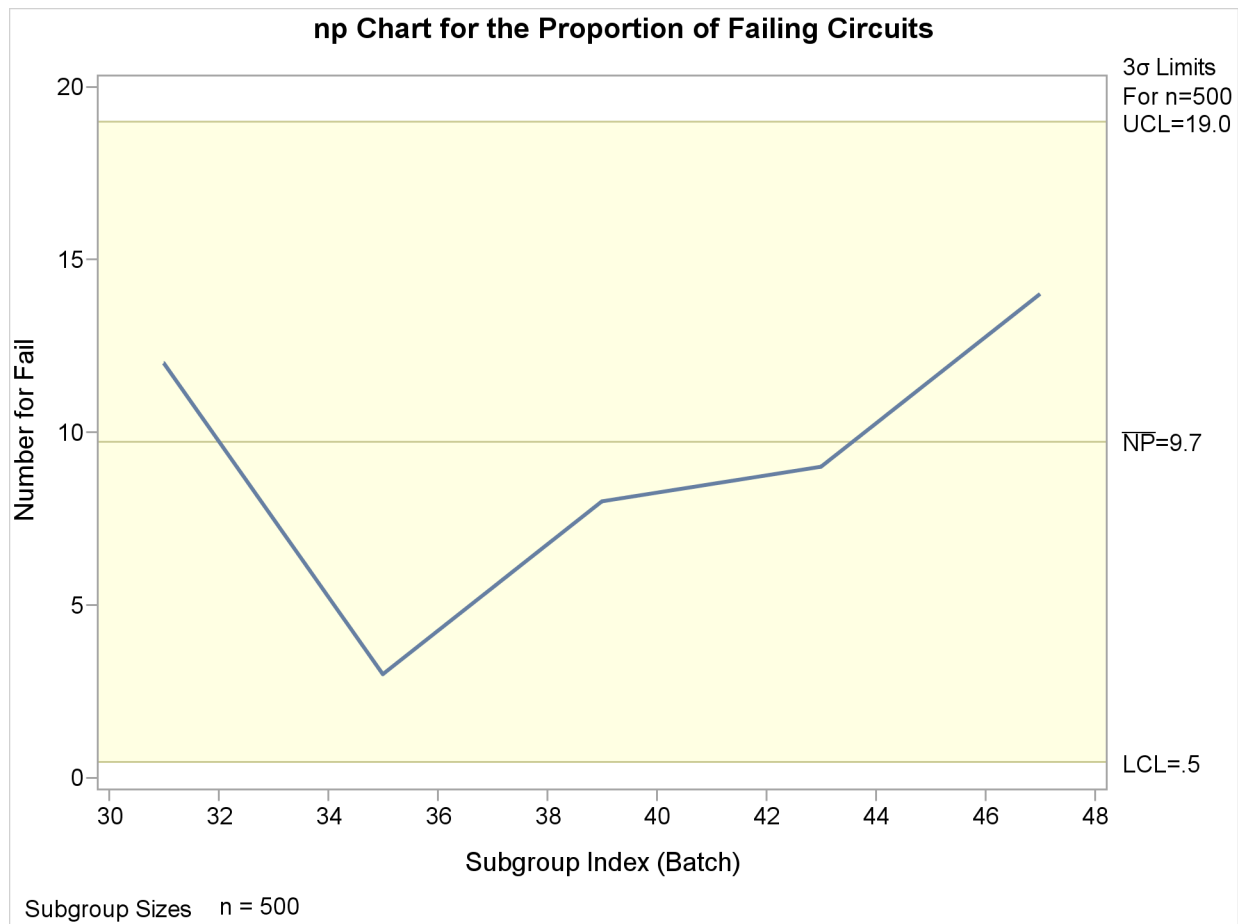
Output 13.17.10 np Chart for Second Set of Circuit Failures (ODS Graphics)
