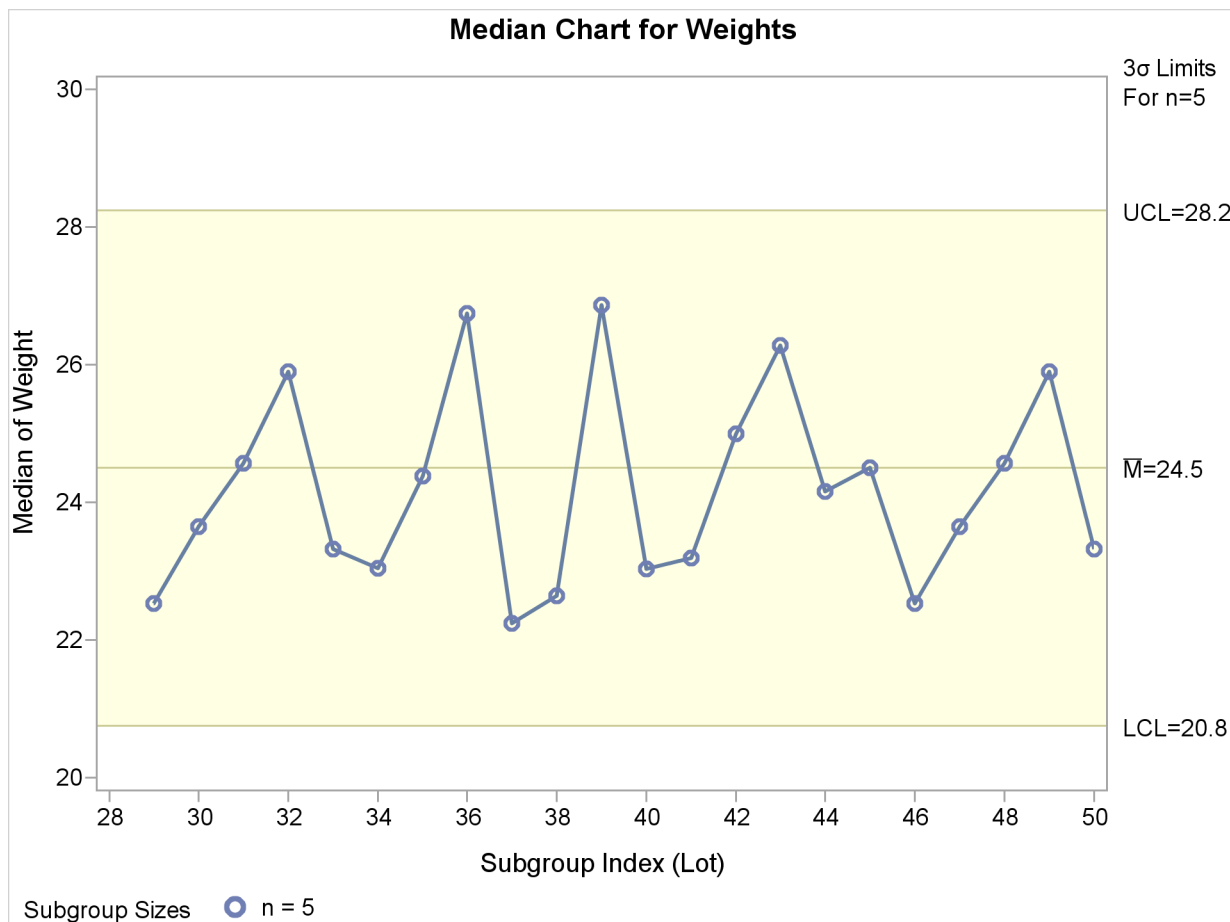
Output 13.13.11 Median Chart for Second Set of Detergent Box Weight Data (ODS Graphics)
