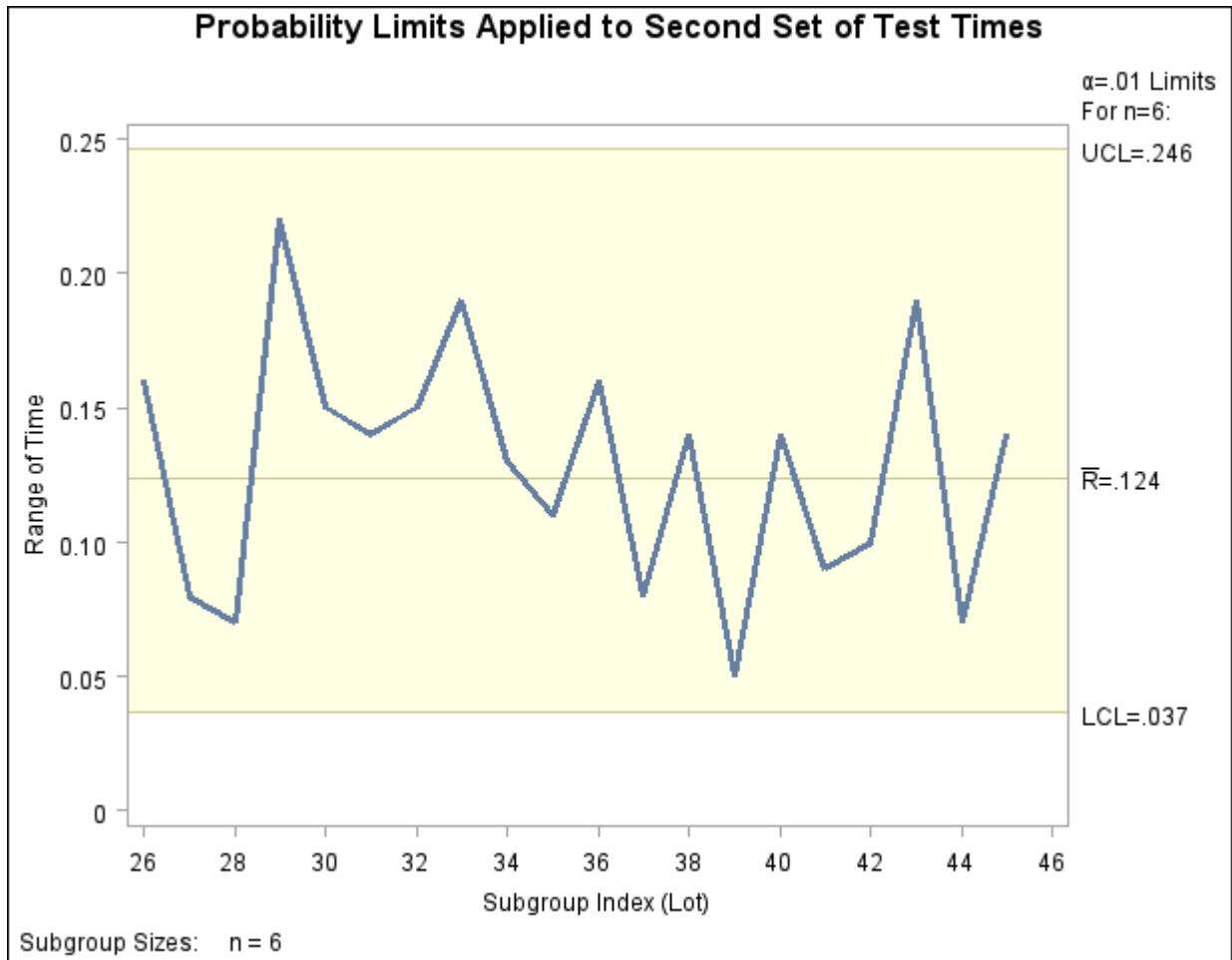
Output 13.27.3 Reading Probability Limits from a LIMITS= Data Set
