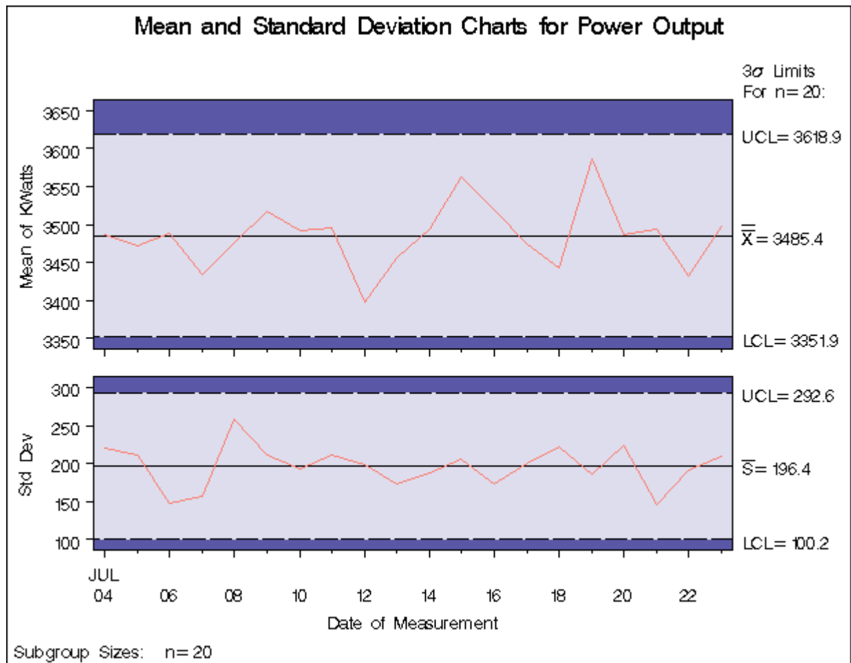
Output 13.40.8 \bar{X} and s Charts for Power Output Data (Traditional Graphics with NOGSTYLE)
