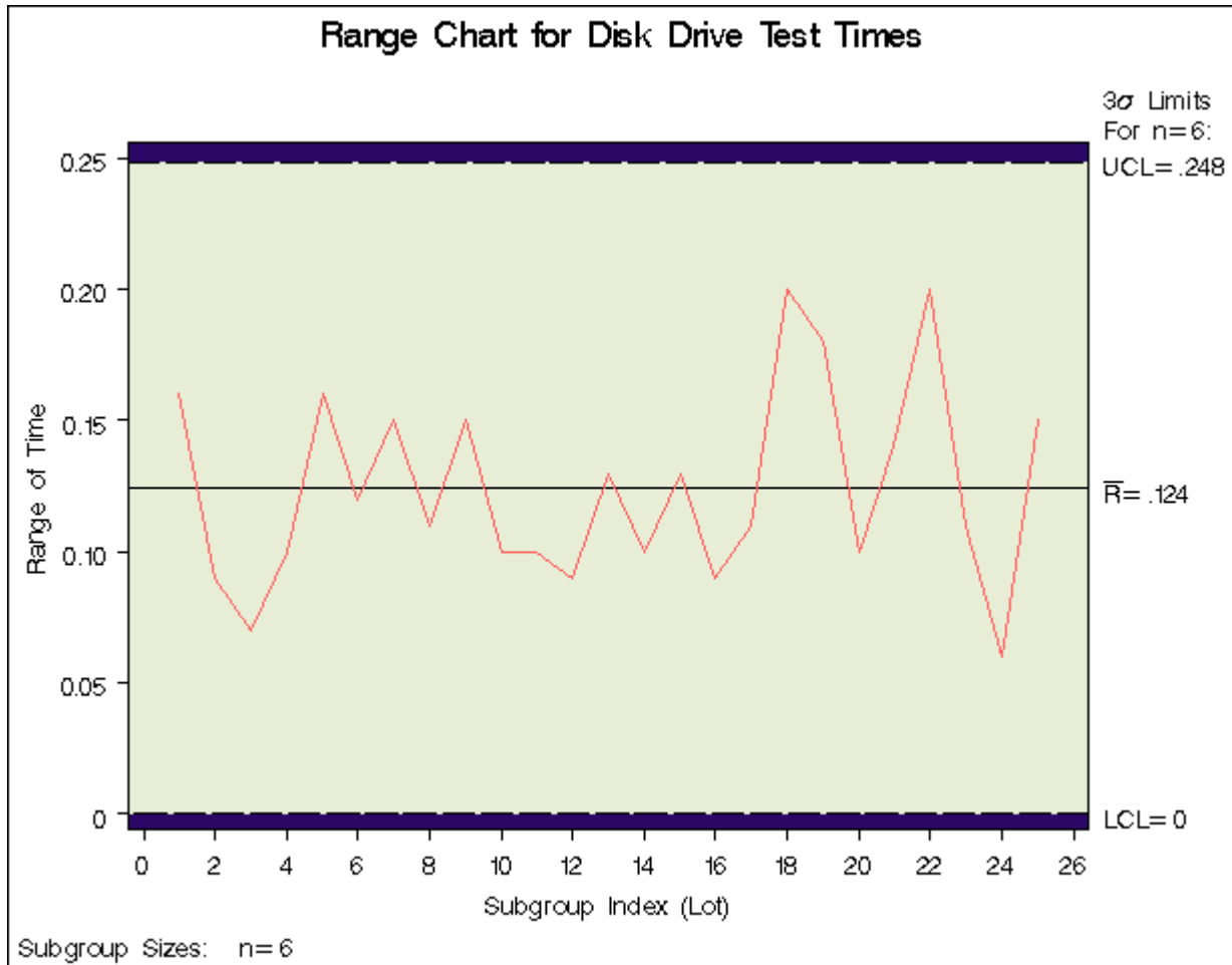
Output 13.26.5 R Chart from the Summary Data Set Disksum (Traditional Graphics with NOGSTYLE)
