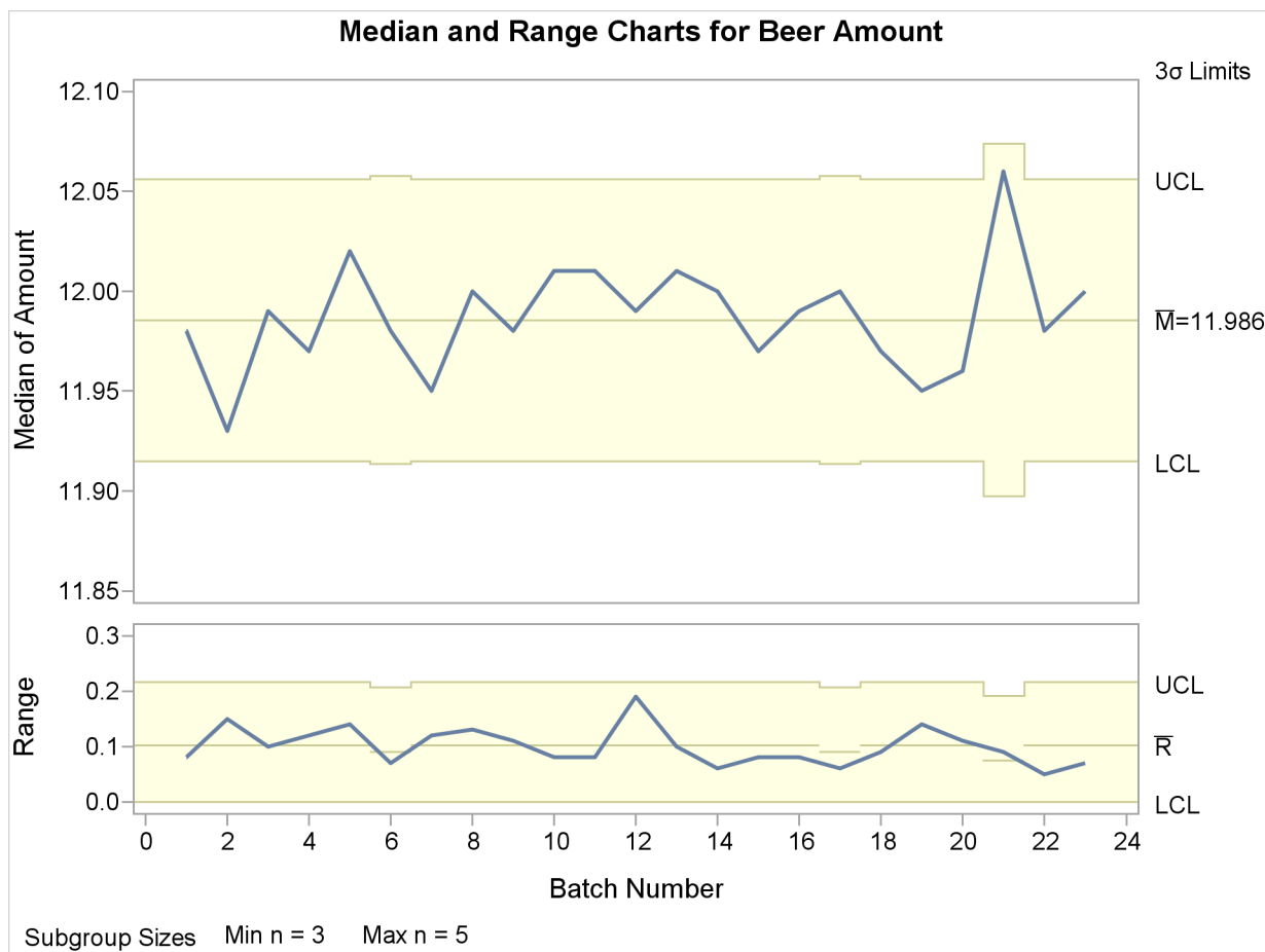
Output 13.16.1 Median and Range Charts with Varying Sample Sizes
