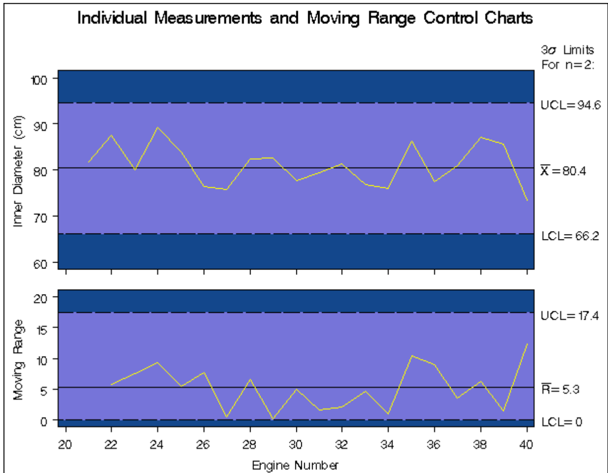
Output 13.10.9 Charts for Second Set of Engine Noise Levels (Traditional Graphics with NOGSTYLE)
