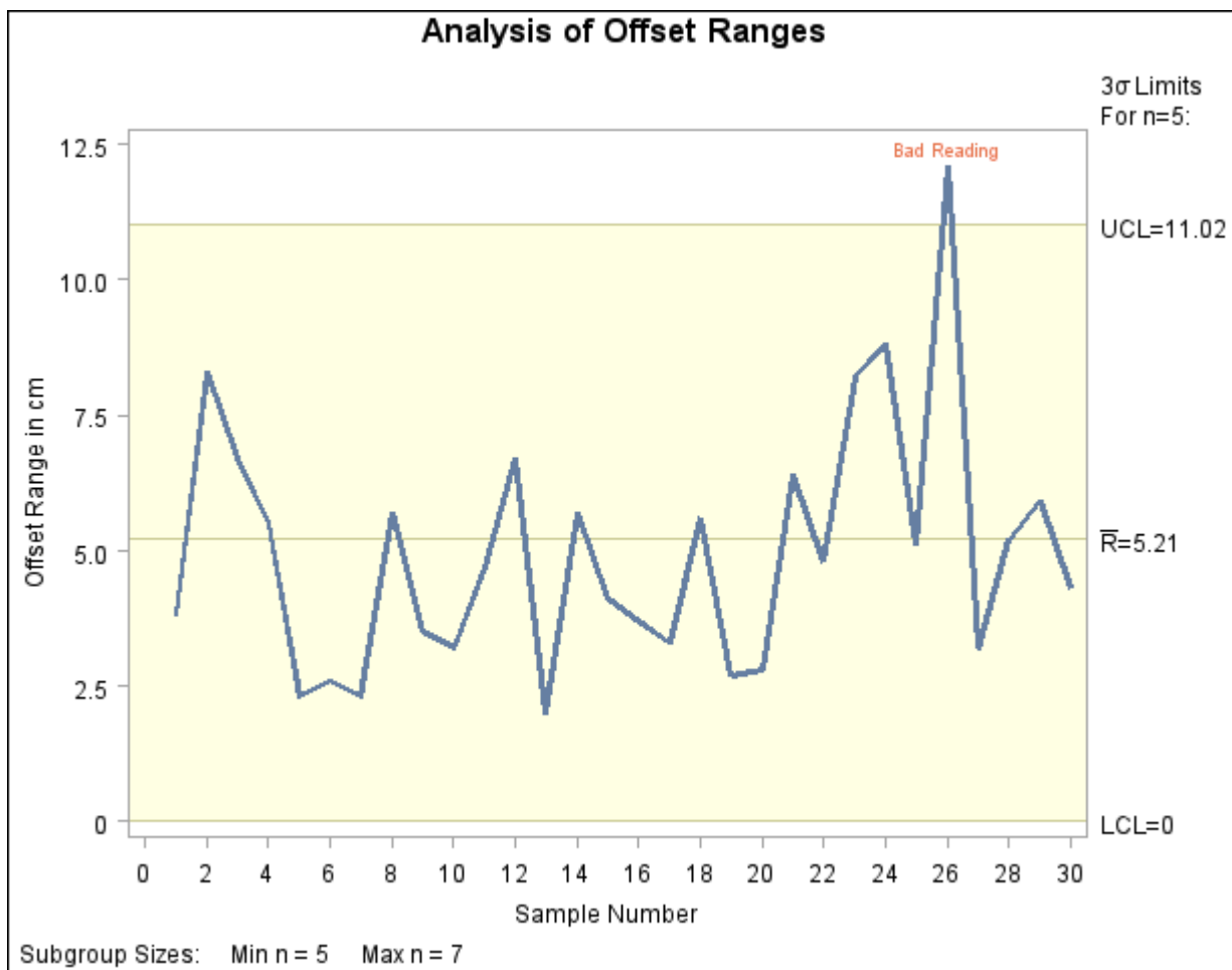
Output 13.43.70 Range Chart with Test 1
