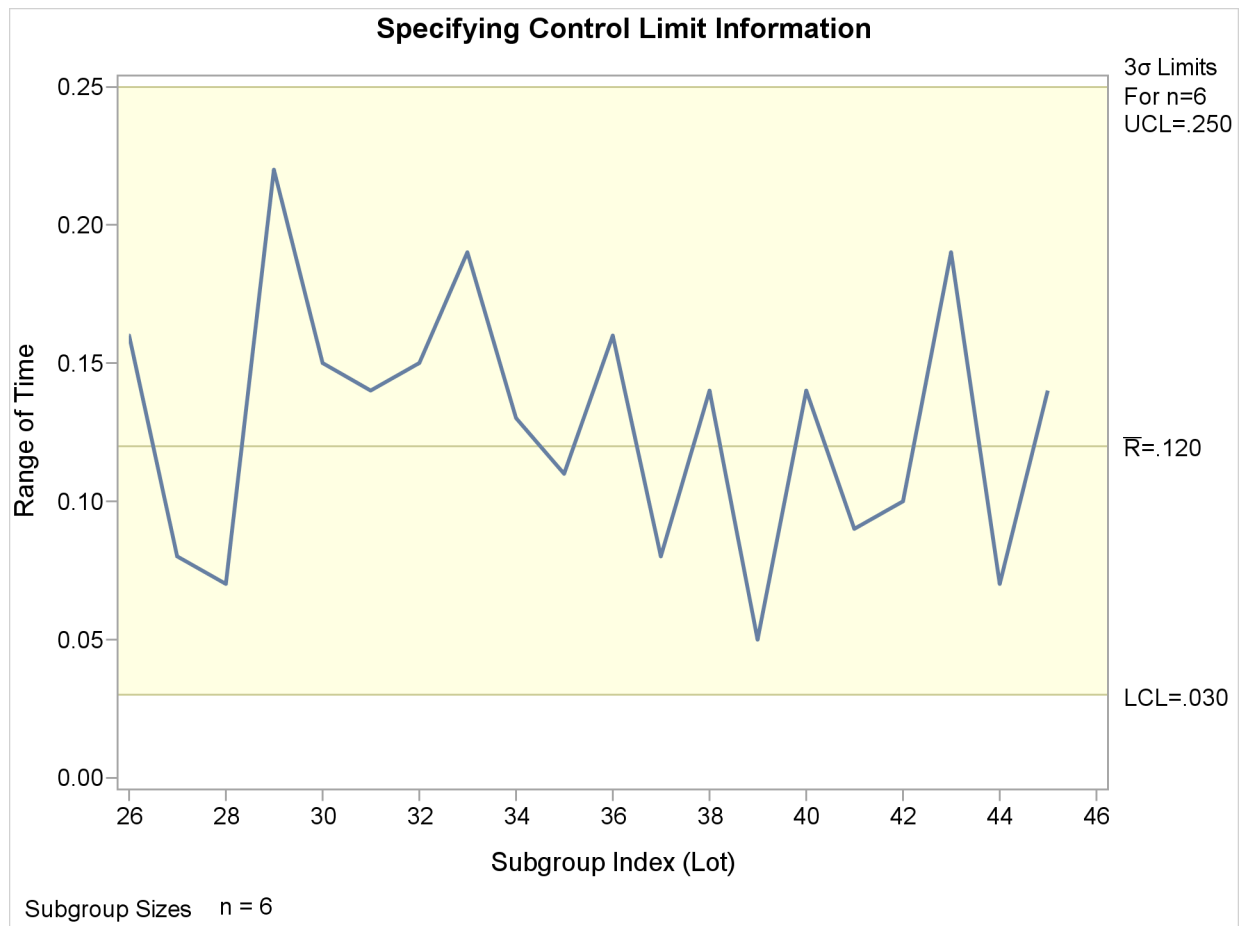
Output 13.28.1 Reading Control Limits from Dlimits2
