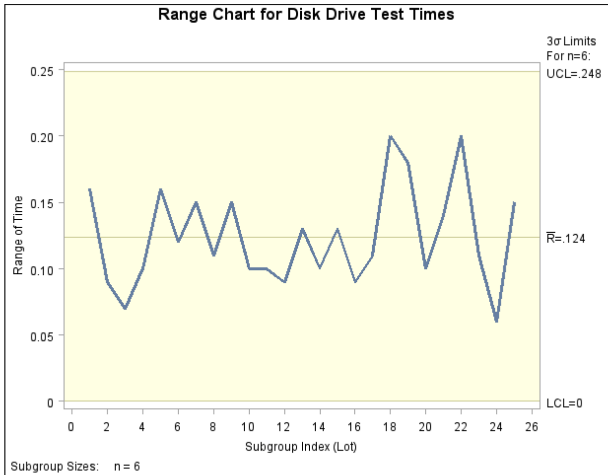
Output 13.26.3 R Chart for the Data Set Disks (Traditional Graphics)
