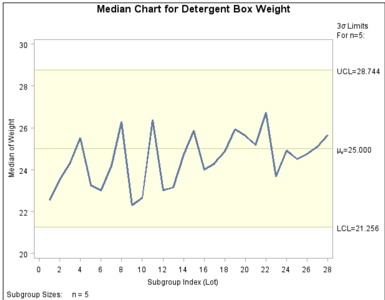
Output 13.14.4 Median Chart for Detergent Box Weight Data
