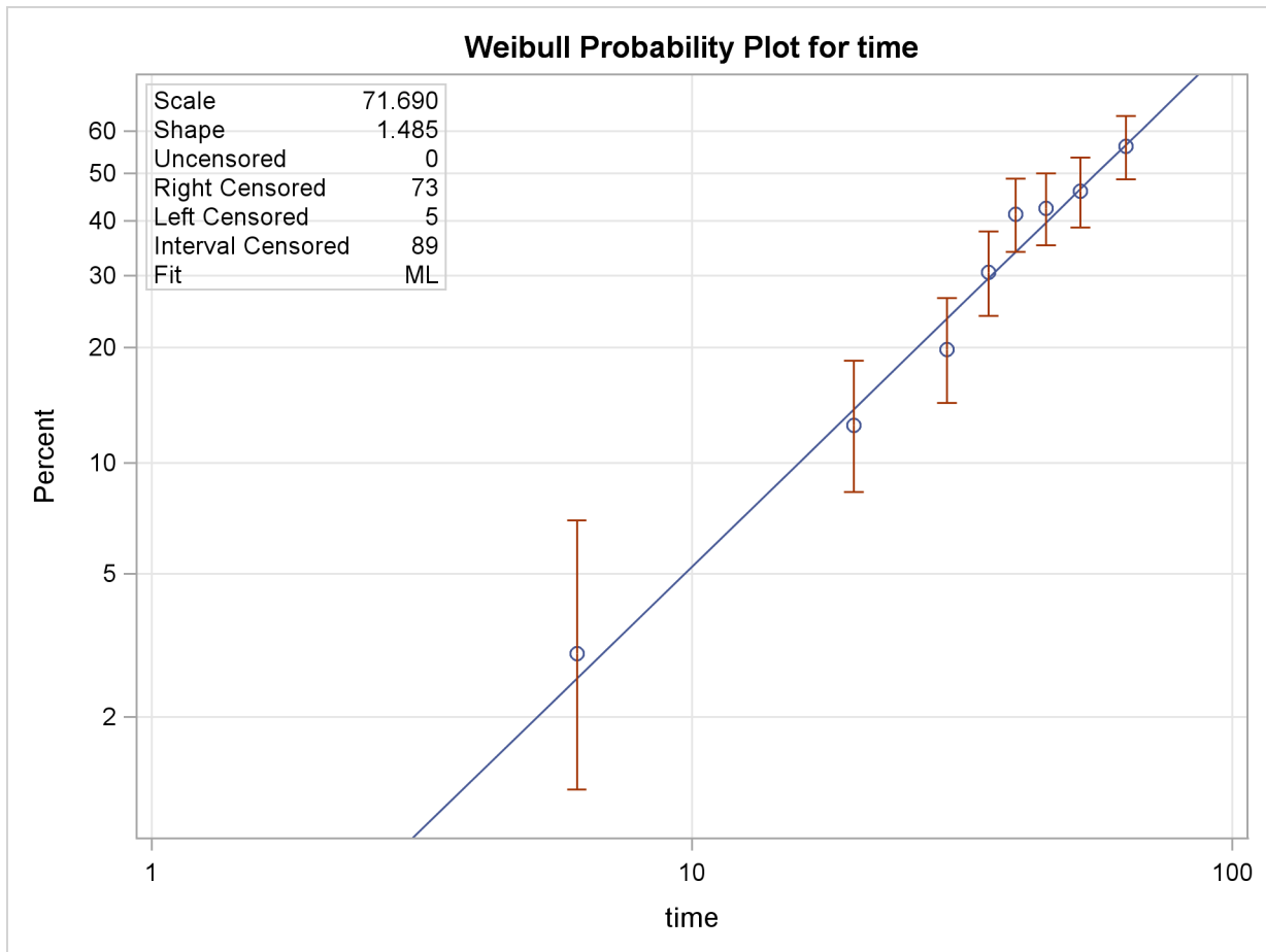
Figure 12.12 Weibull Probability Plot for the Part Cracking Data
