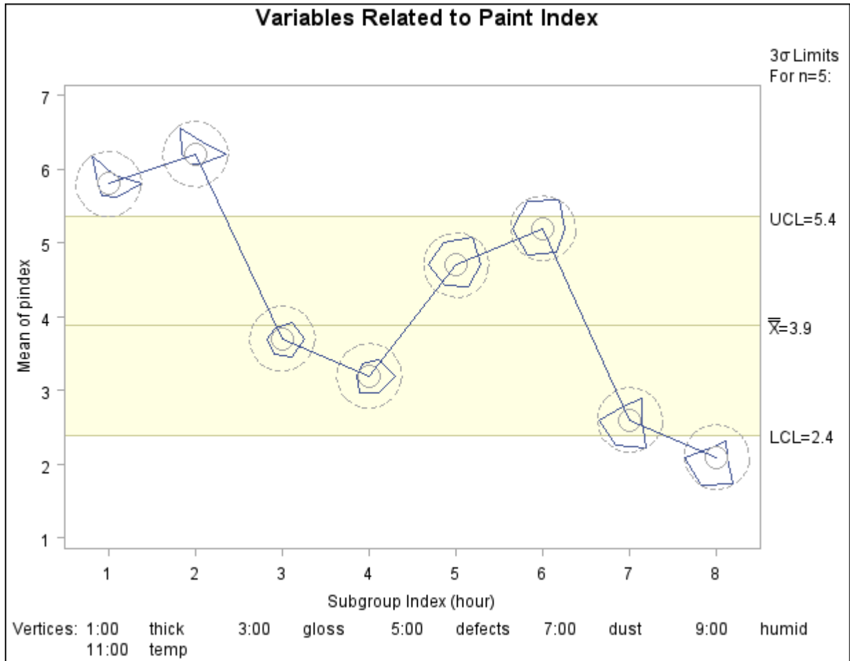
Output 13.43.42 Star Chart with Inner and Outer Circles Added
