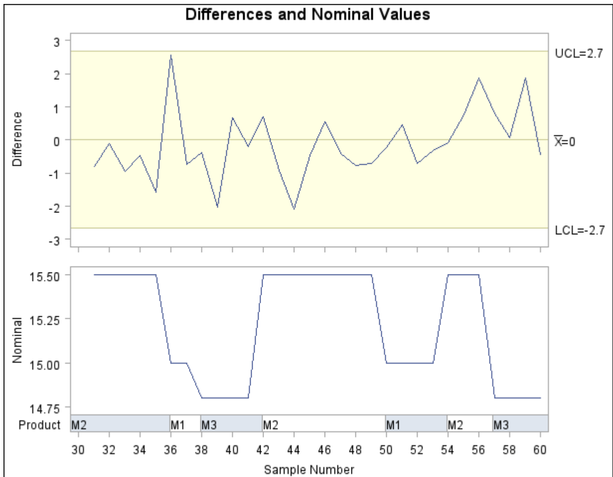
Output 13.43.94 Short Run Control Chart with Nominal Values
