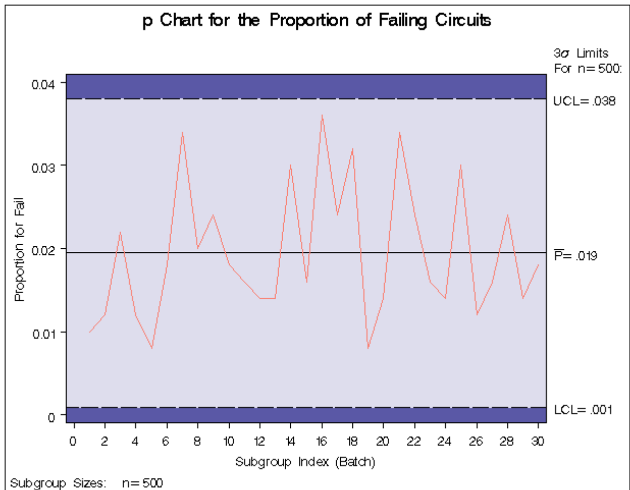
Output 13.21.7 p Chart from Subgroup Proportions (Traditional Graphics with NOGSTYLE)
