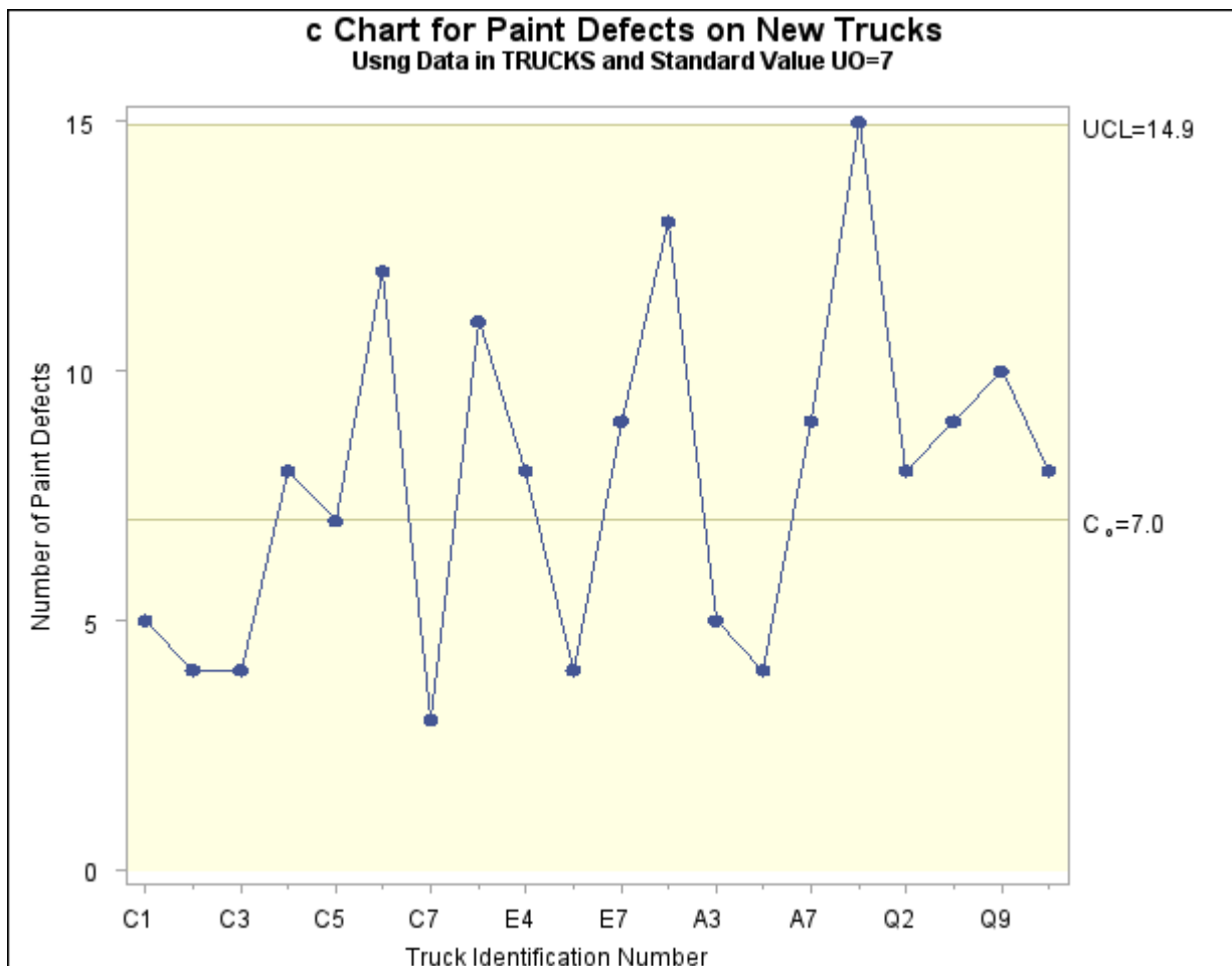
Output 13.9.1 A c Chart with Standard Value u_0
