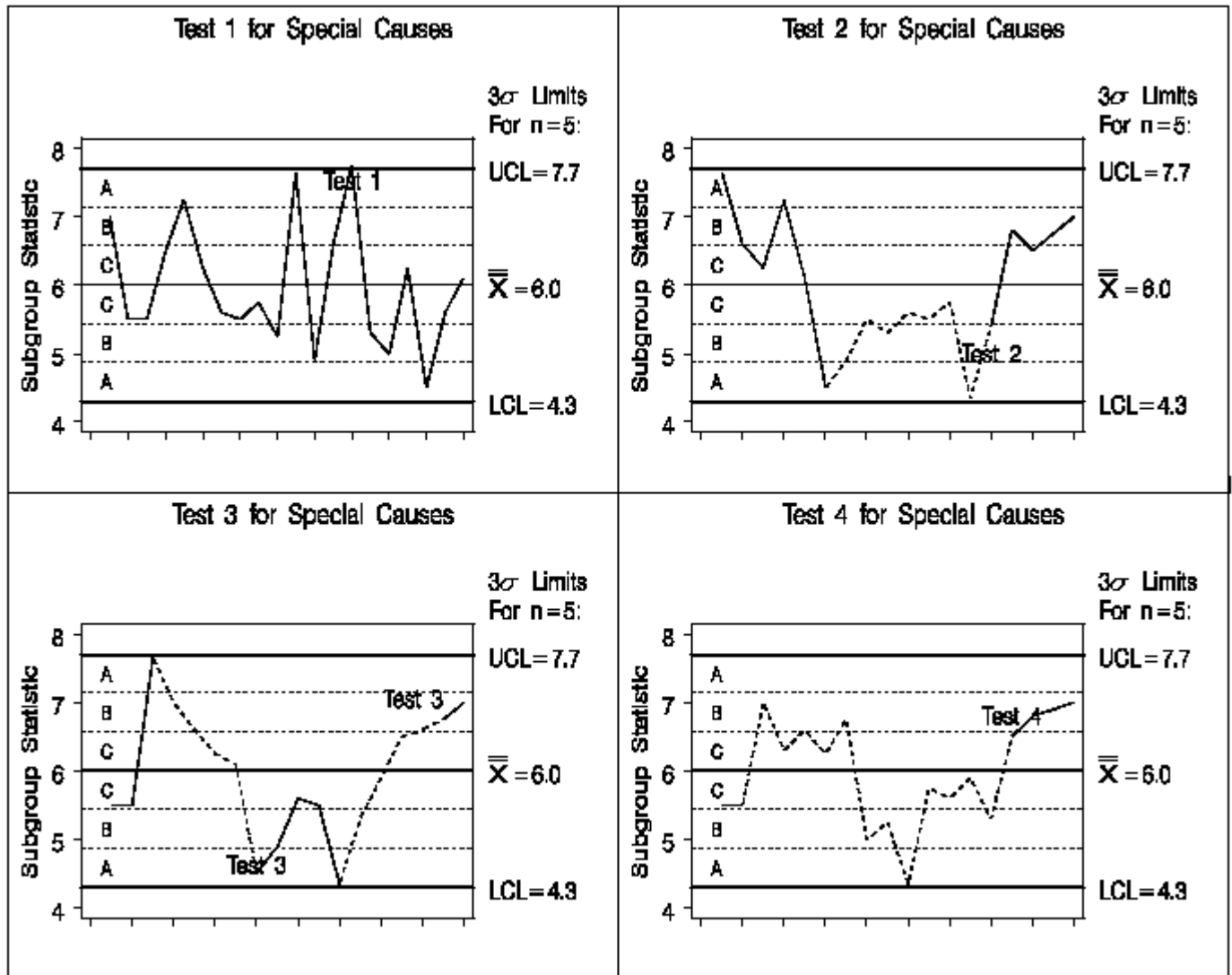
Output 13.43.61 Examples of Tests 1 to 4
