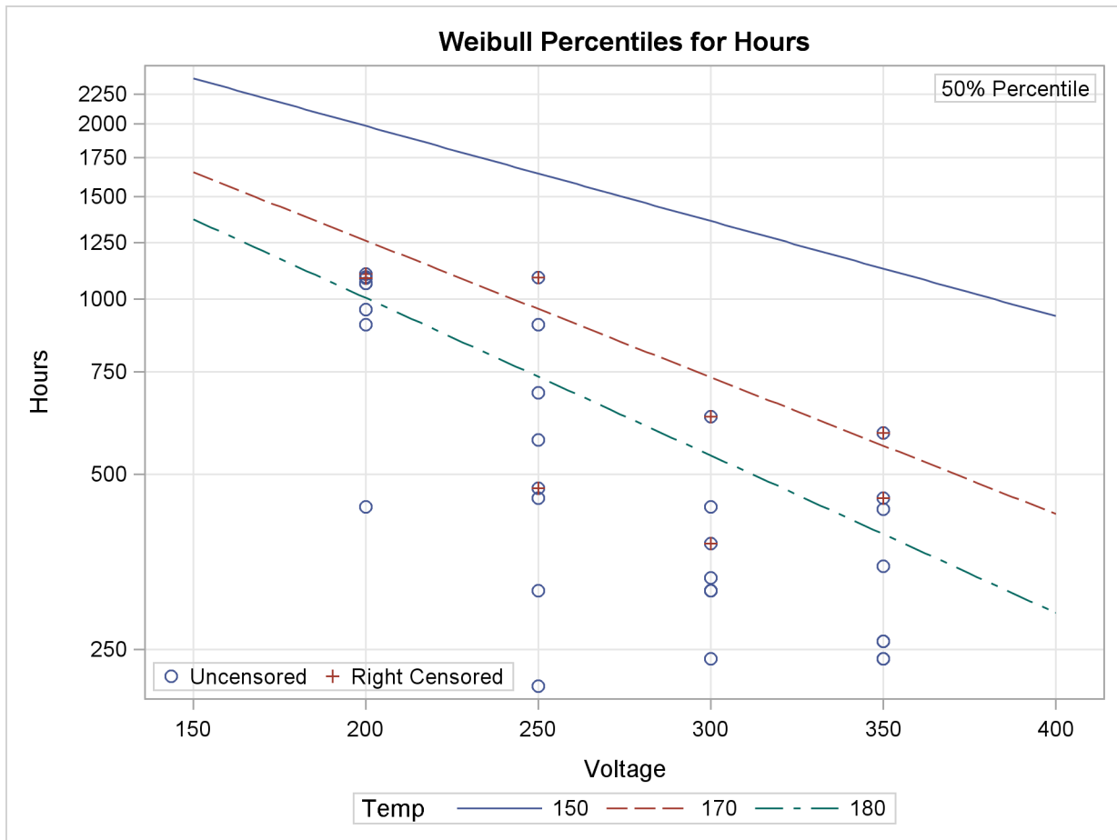
Figure 12.26 Plot of Data and Fitted Weibull Percentiles for Glass Capacitor Regression Model
