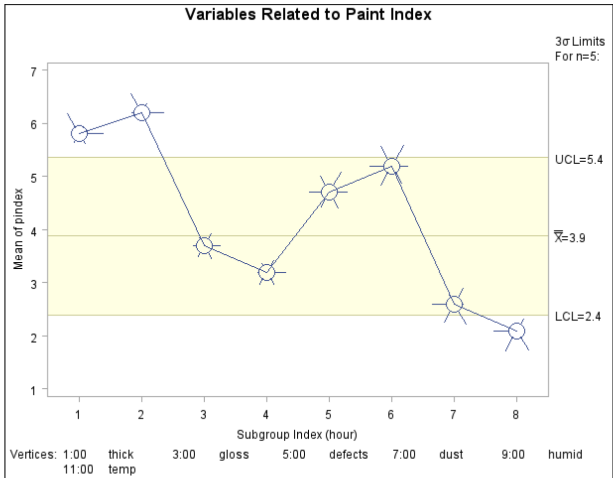
Output 13.43.45 Star Chart Using STARTYPE=SPOKE
