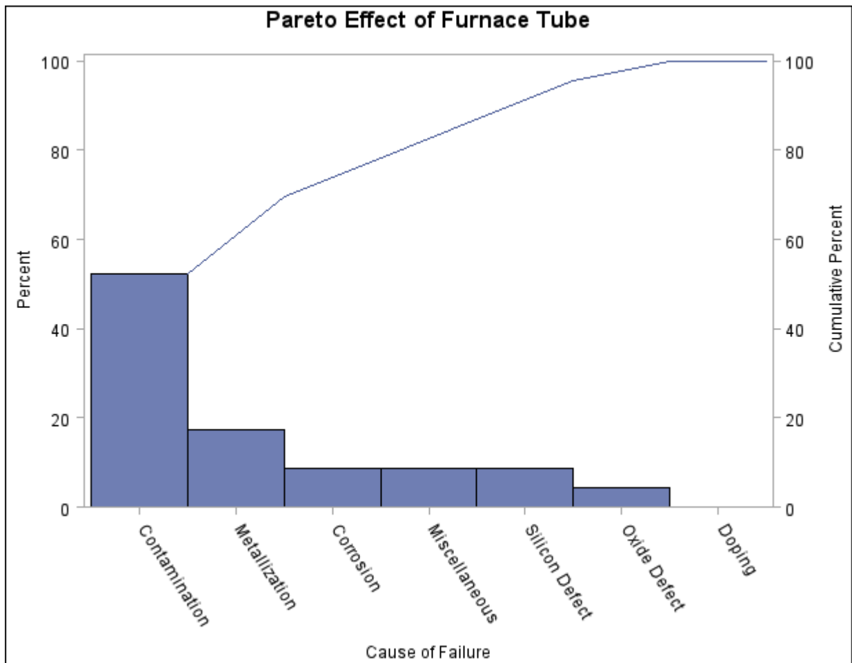
Output 11.1.1 “After” Analysis Using Stage as a BY Variable
