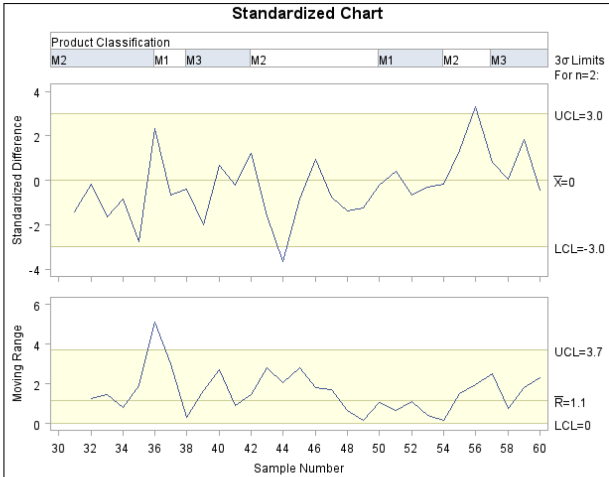
Output 13.43.96 Standardized Difference Chart
