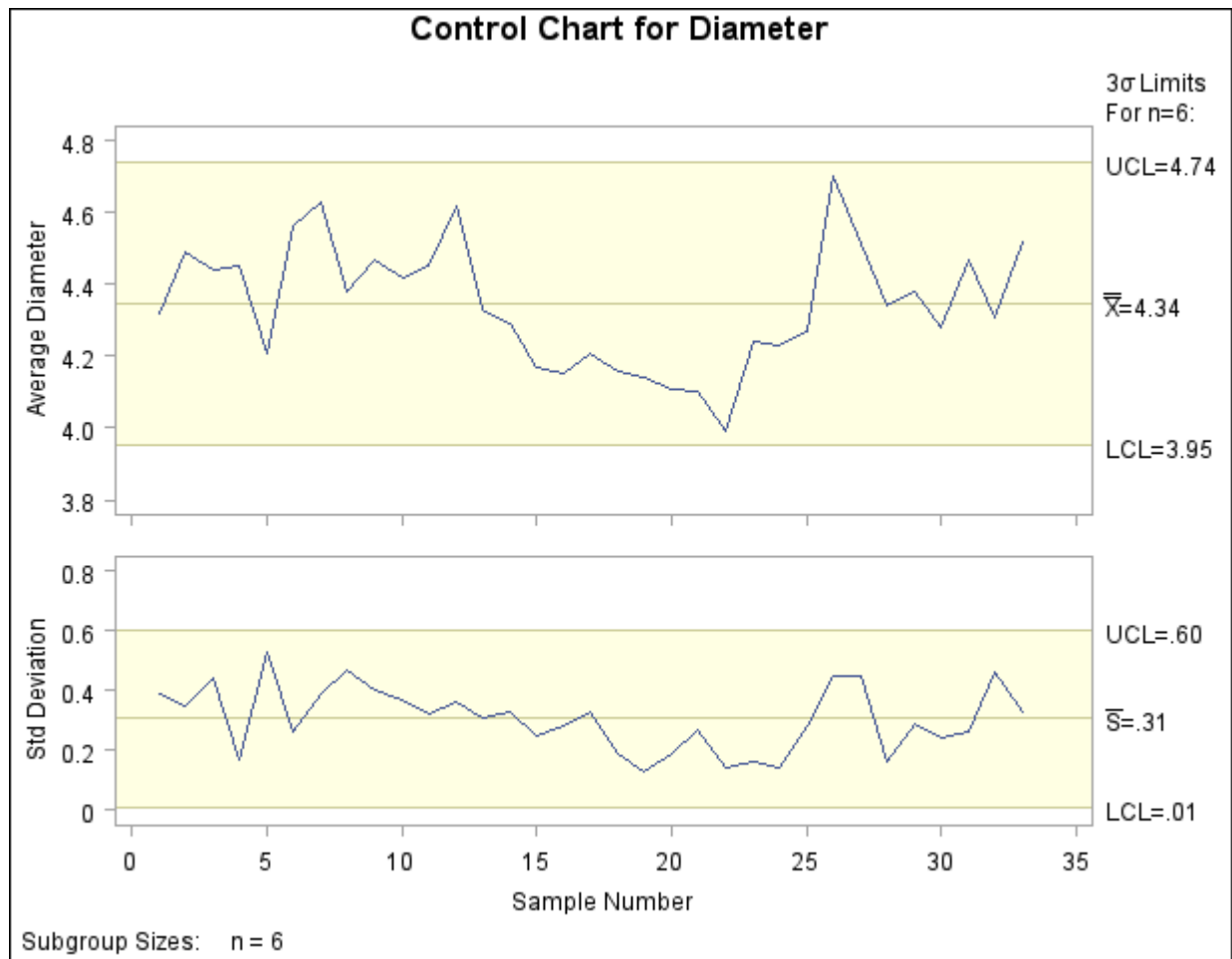
Output 13.43.56 Control Charts with Axis Labels Specified
