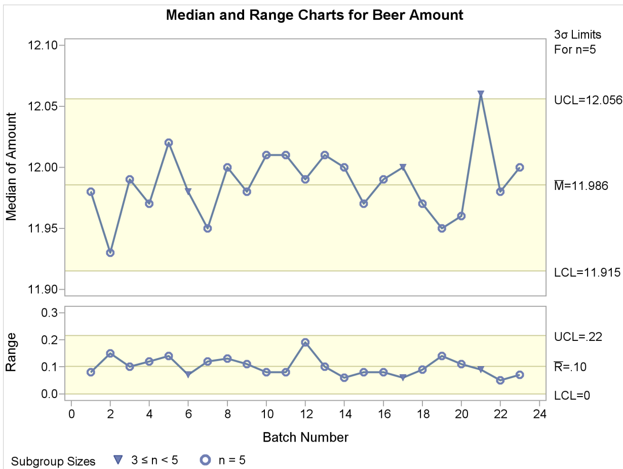
Output 13.16.3 Displaying All Subgroups Regardless of Sample Size
