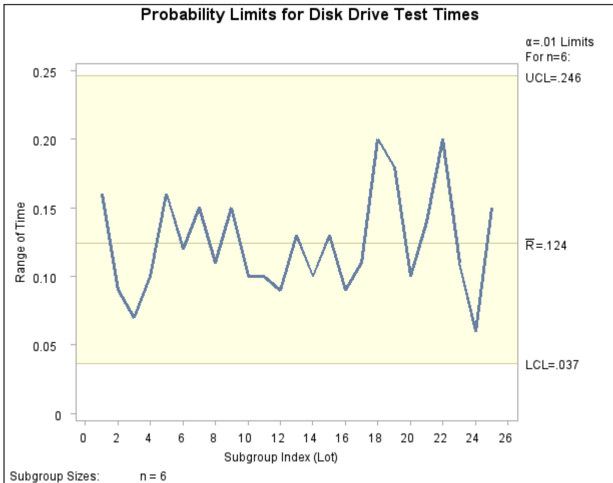
Output 13.27.1 R Chart with Probability Limits
