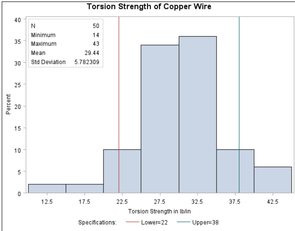
Output 5.14.5 A Histogram with an Inset
