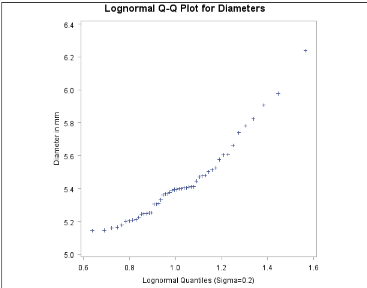
Output 5.22.1 Lognormal Quantile-Quantile Plot ( \sigma = 0.2 )
