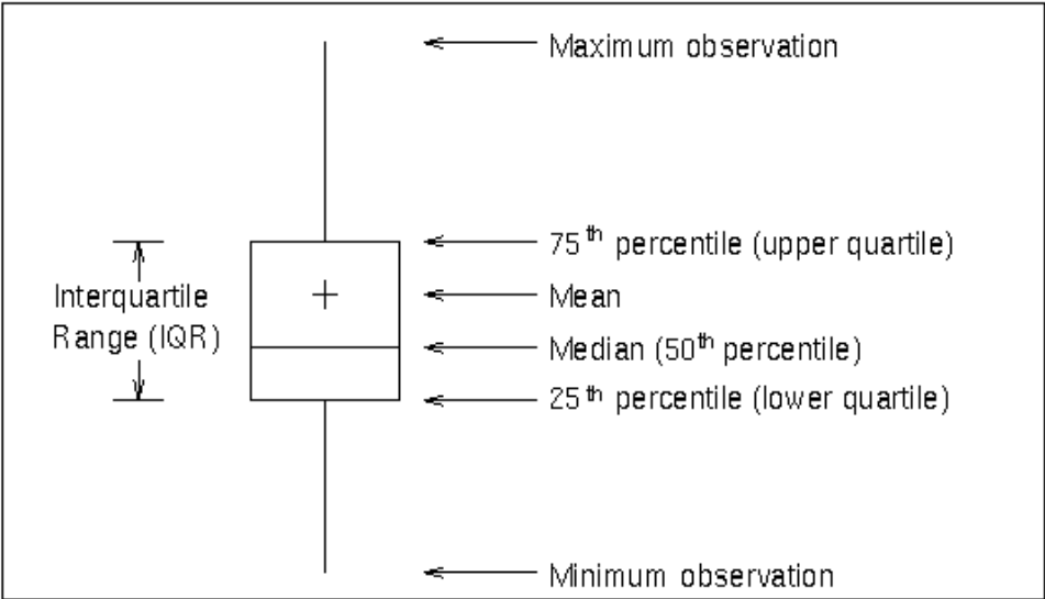
Figure 13.14 Box-and-Whisker Plot
