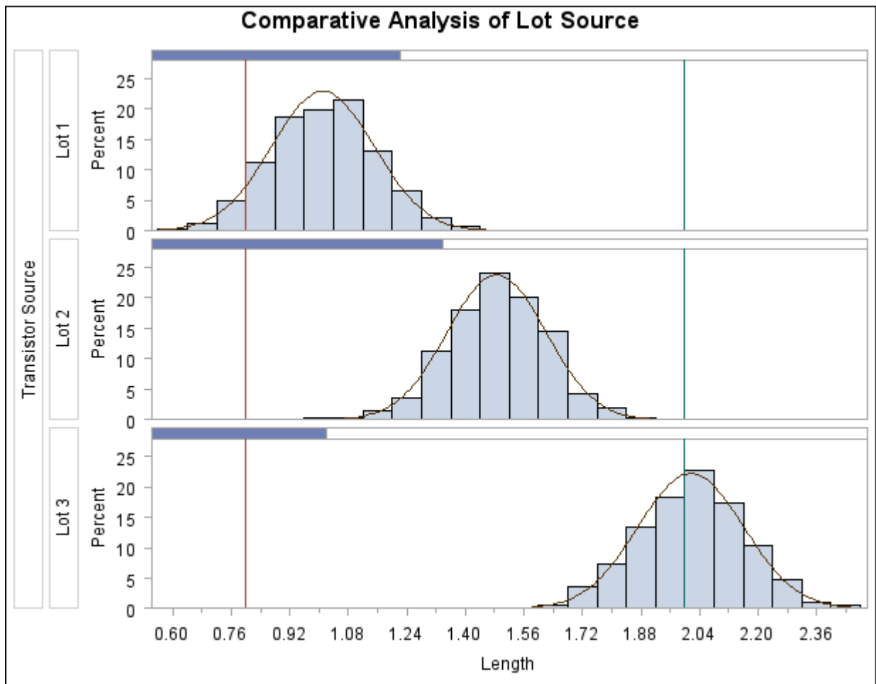
Output 5.5.3 Fitting Normal Curves
