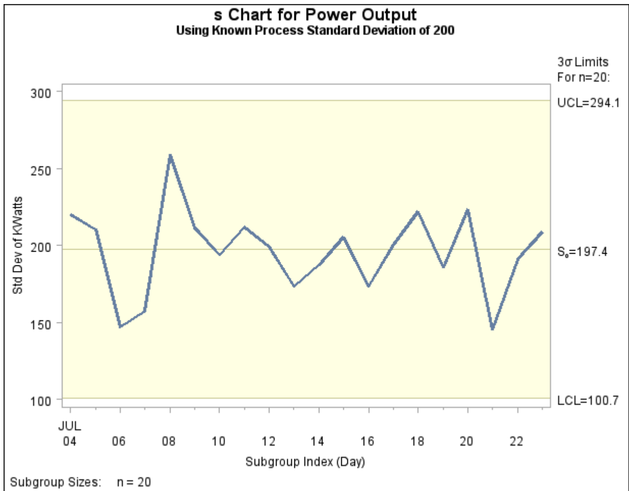
Output 13.29.1 Reading in Standard Value for Process Standard Deviation
