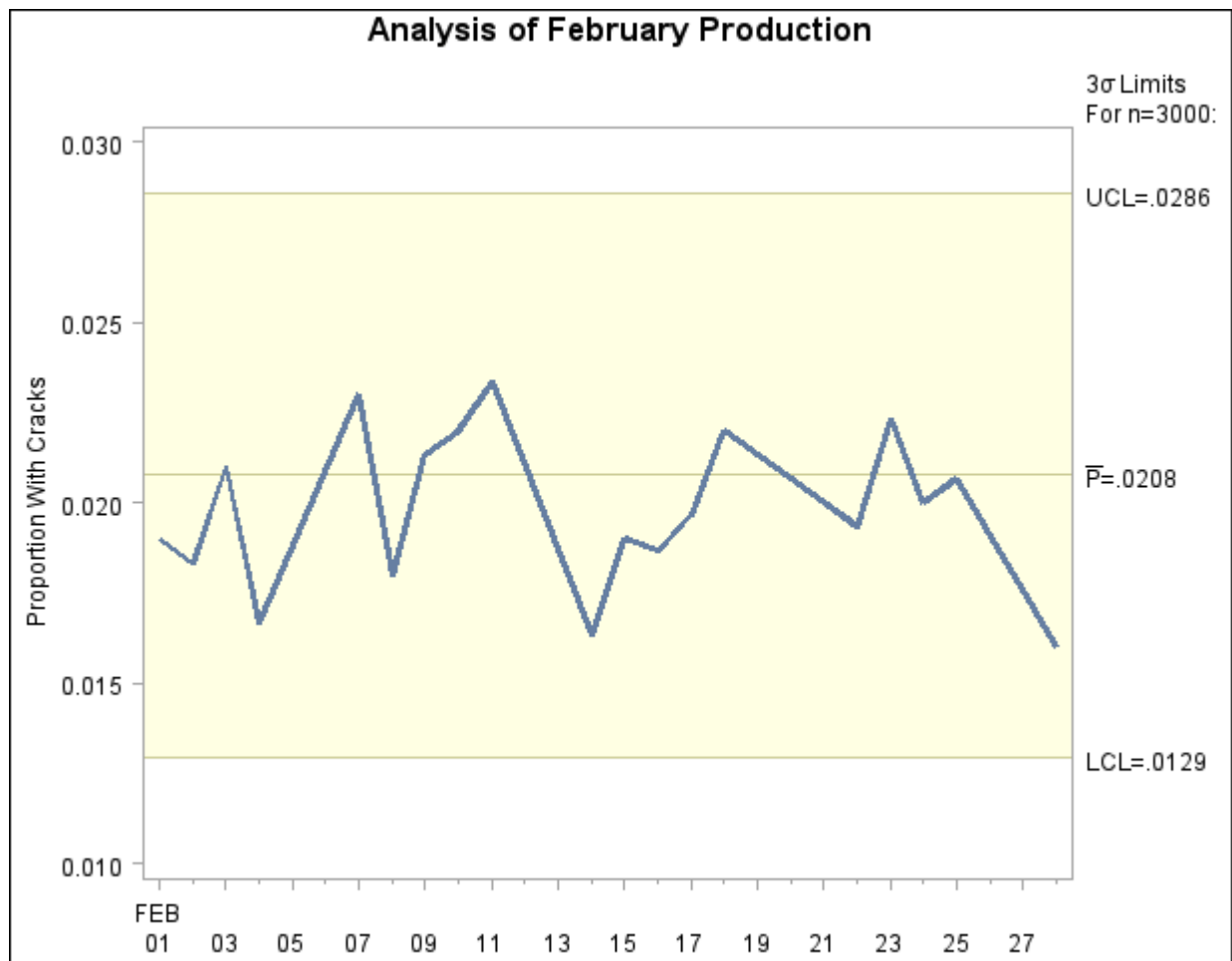
Output 13.43.60 p Chart for February Data
