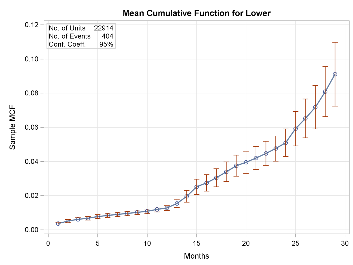
Figure 12.39 MCF Plot for the Defrost Controls
