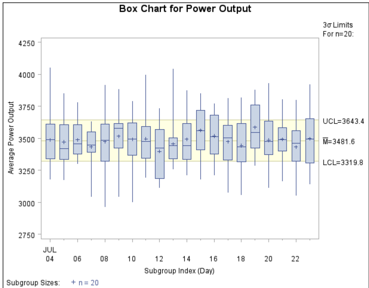
Figure 13.5 Box Chart for Power Output Data (Traditional Graphics)
