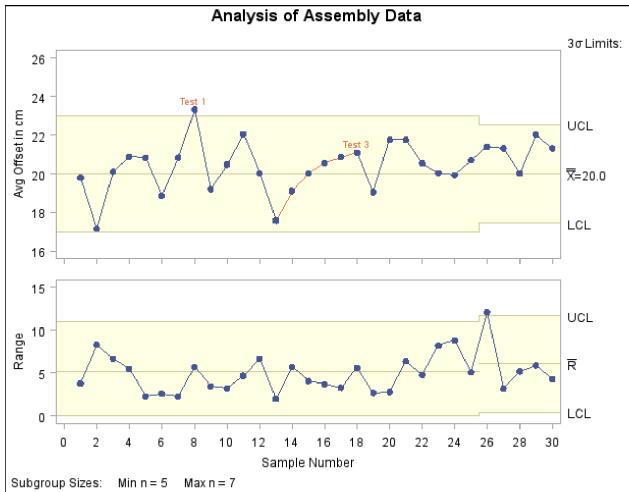
Output 13.43.64 The TESTNMETHOD= Option for Varying Subgroup Sizes
