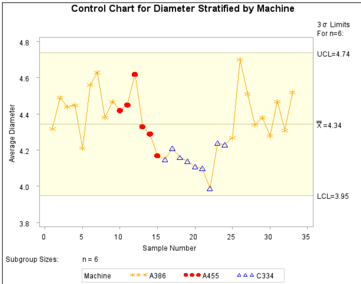
Output 13.43.26 Control Chart Stratified into Levels Using Symbols
