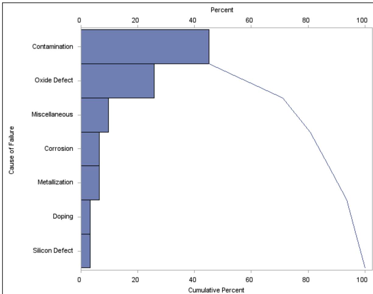
Figure 11.1 Pareto Chart for IC Failures in the Data Set Failure1
