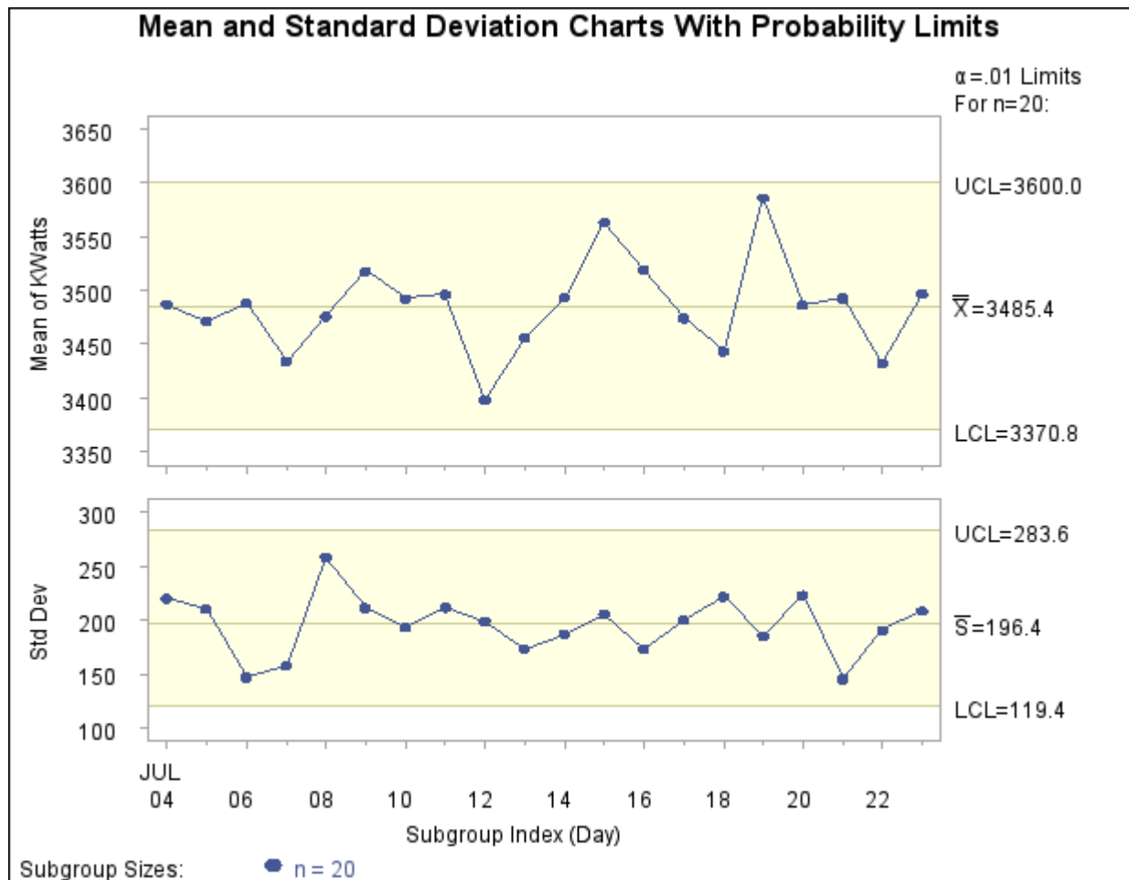
Output 13.41.1 Probability Limits on \bar{X} and s Charts
