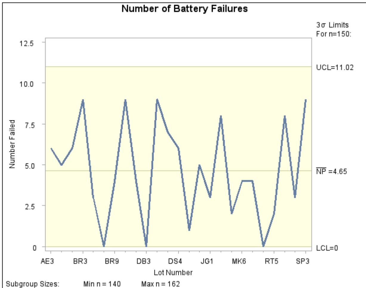
Output 13.20.3 Control Limits Based on Fixed Subgroup Sample Size
