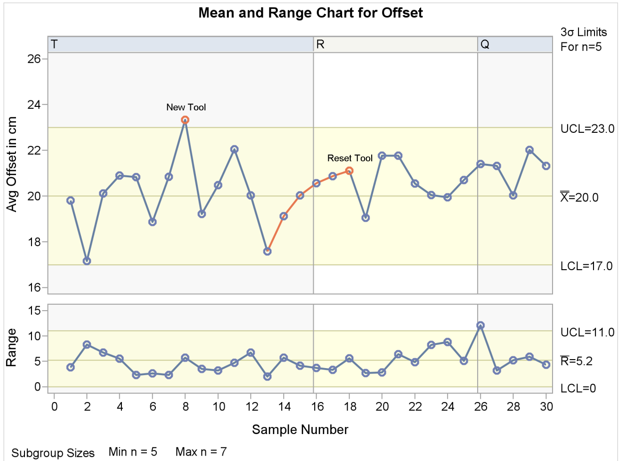
Output 13.43.67 Single Set of Limits with Multiple Phases
