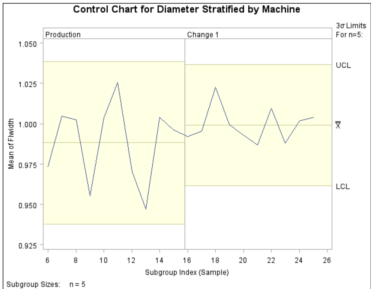
Output 13.43.36 Multiple Phases with Mismatched Control Limits
