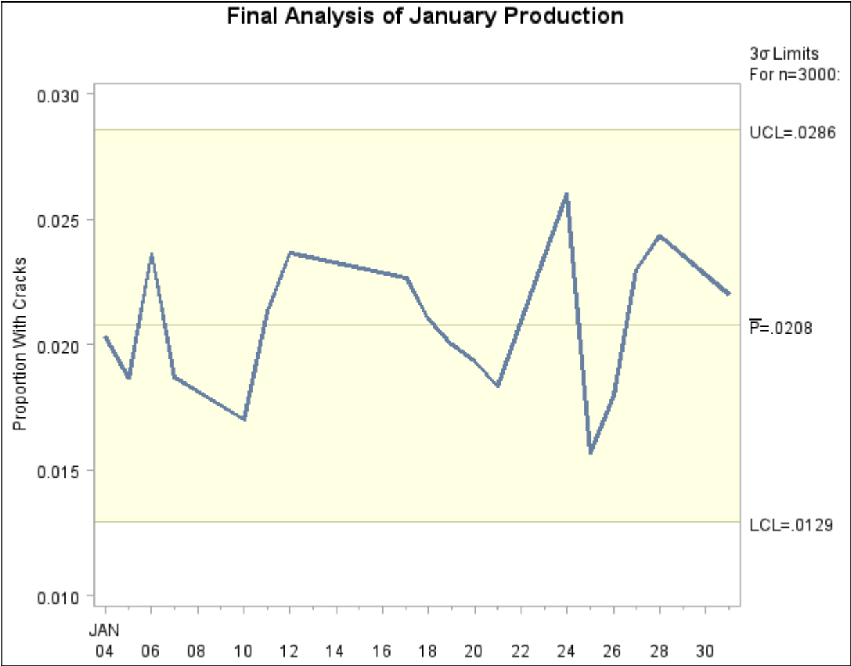
Output 13.43.58 Final p Chart for January Data
