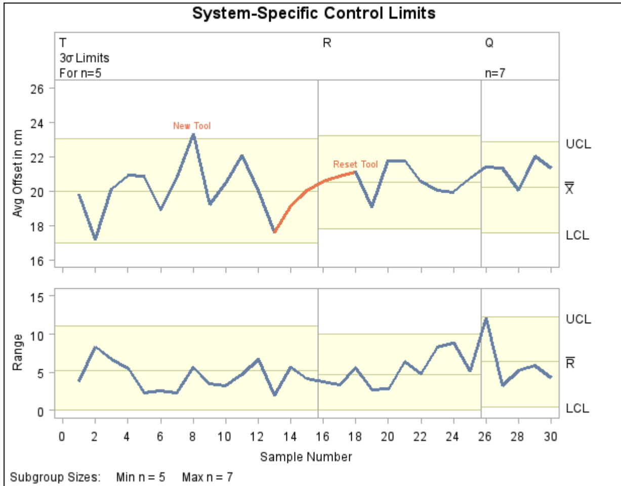
Output 13.43.69 Multiple Sets of Control Limits with the TESTACROSS Option
