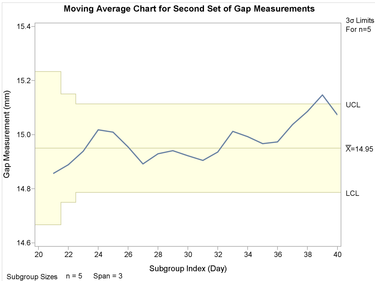
Output 9.5.10 Using Control Limit Parameters from a LIMITS= Data Set
