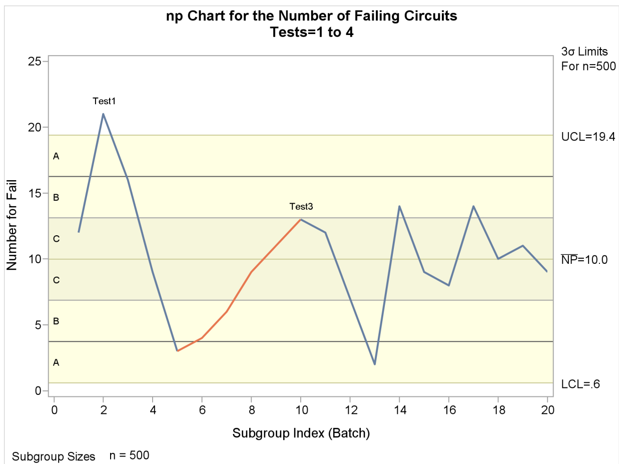
Output 13.18.1 Tests for Special Causes Displayed on np Chart
