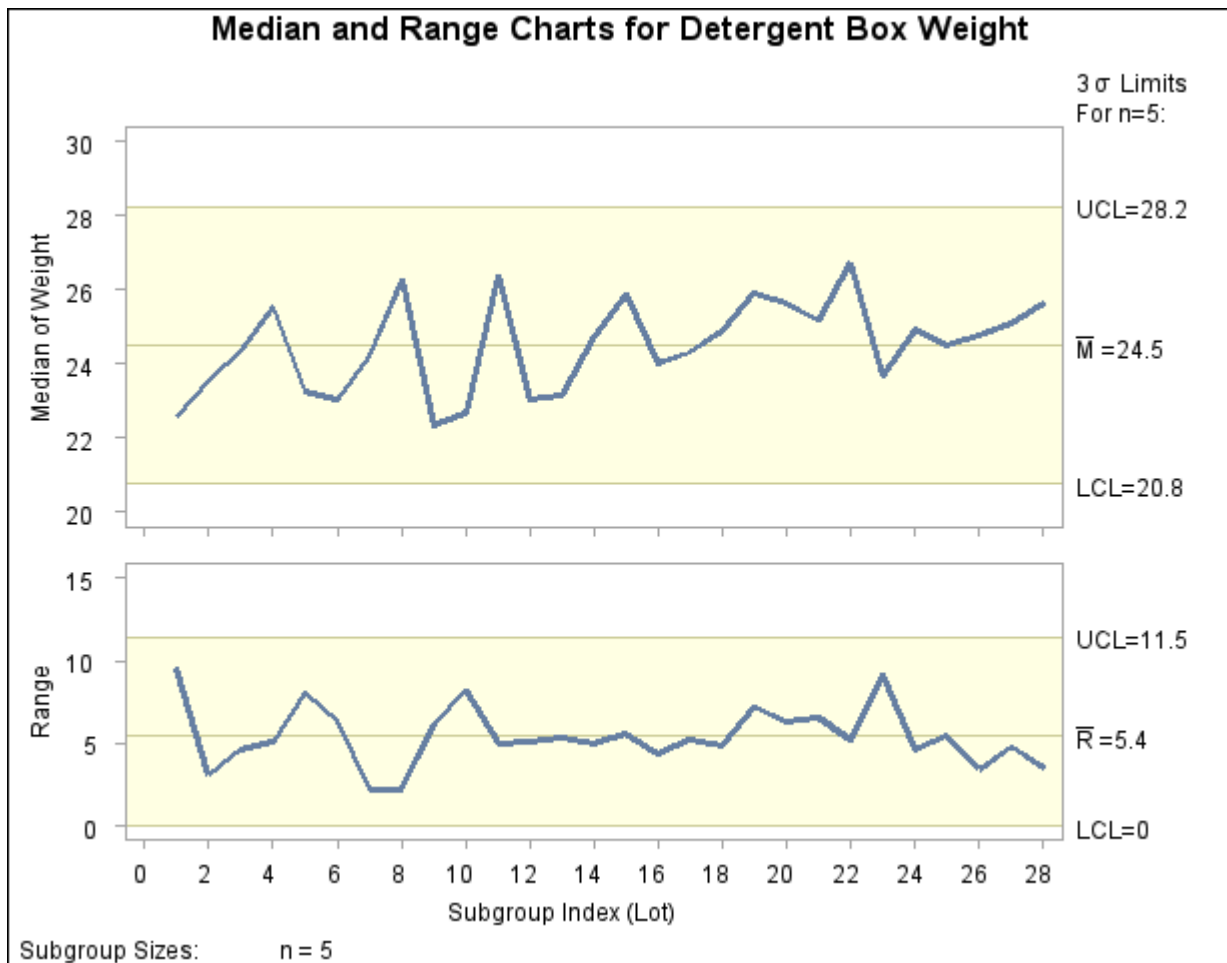
Output 13.15.4 Median and Range Charts (Traditional Graphics)
