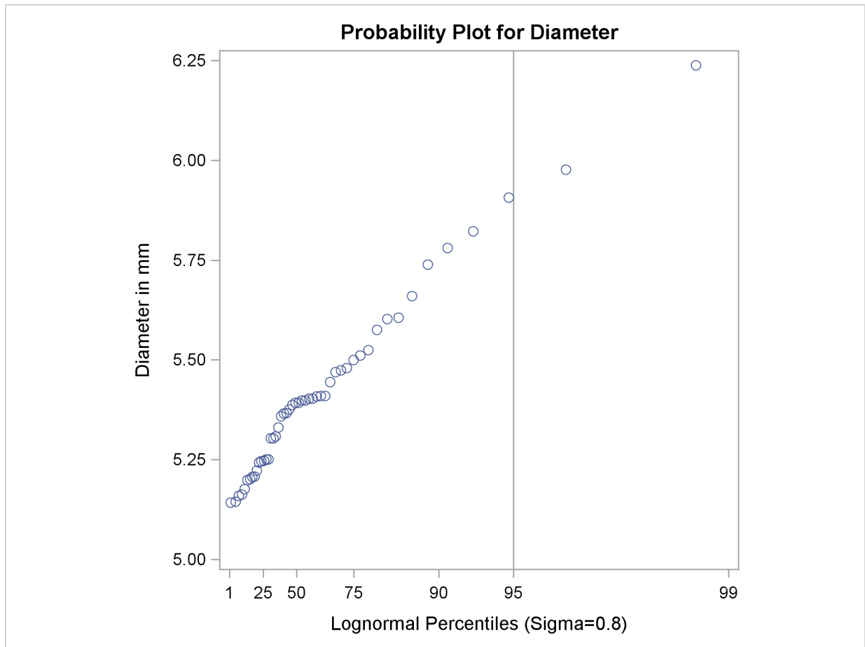
Output 5.18.9 Probability Plot Based on Lognormal Distribution with \sigma = 0.8
