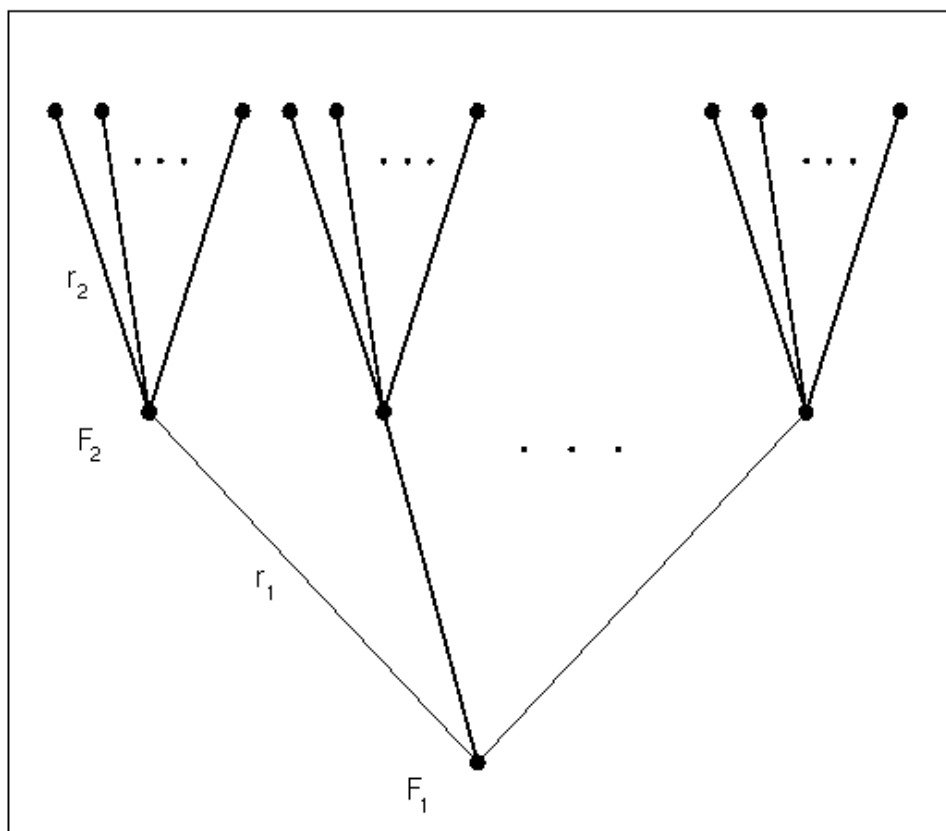
Output 7.16.3 Search Tree
