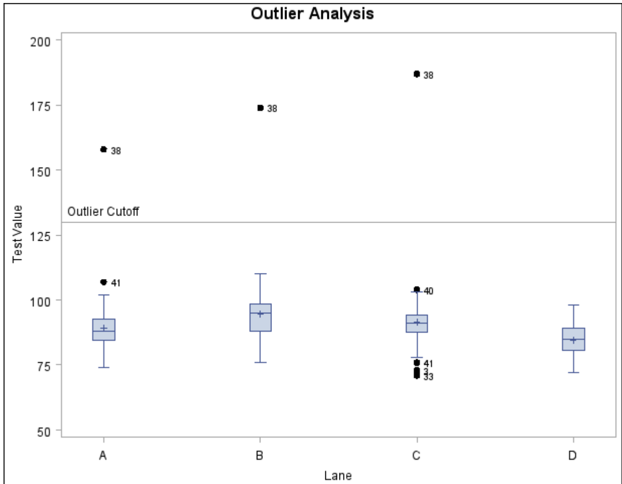
Output 13.43.81 Outlier Analysis for the Data Set Film
