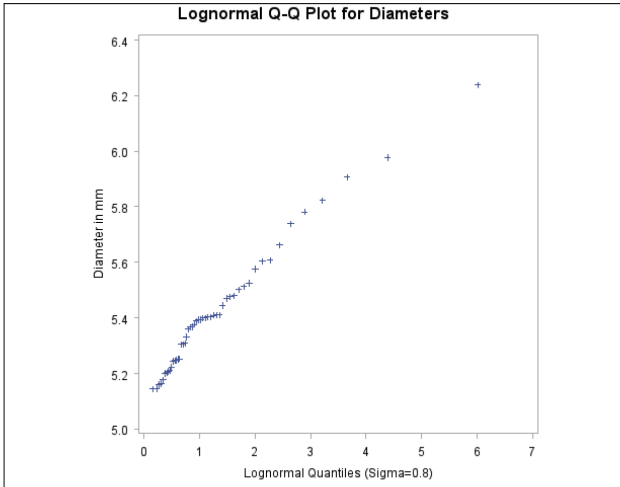
Output 5.22.3 Lognormal Quantile-Quantile Plot ( \sigma = 0.8 )
