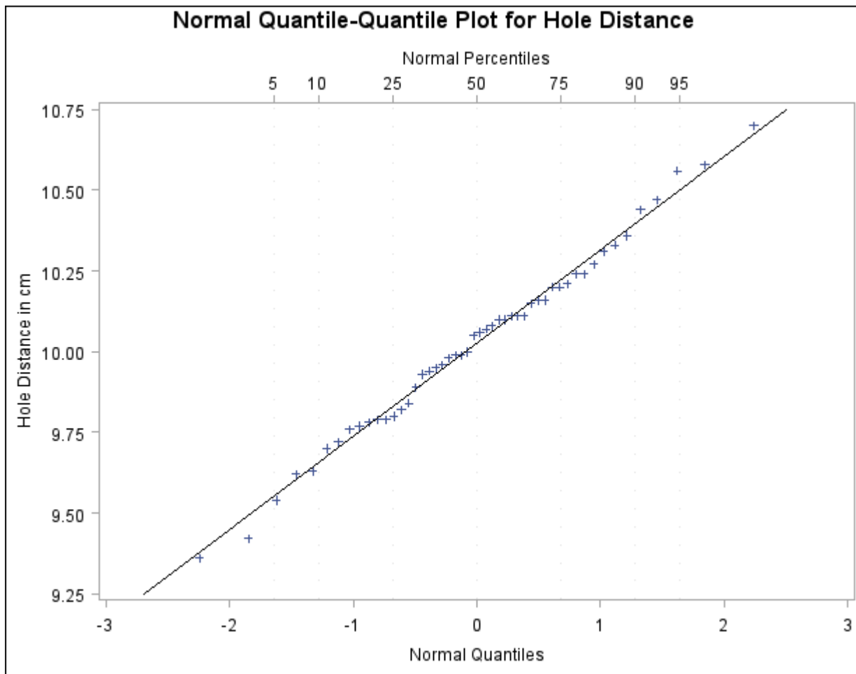
Output 5.20.4 Normal Q-Q Plot with Percentile Axis
