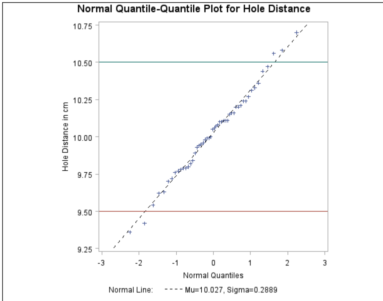
Output 5.20.3 Adding a Distribution Reference Line to a Q-Q Plot
