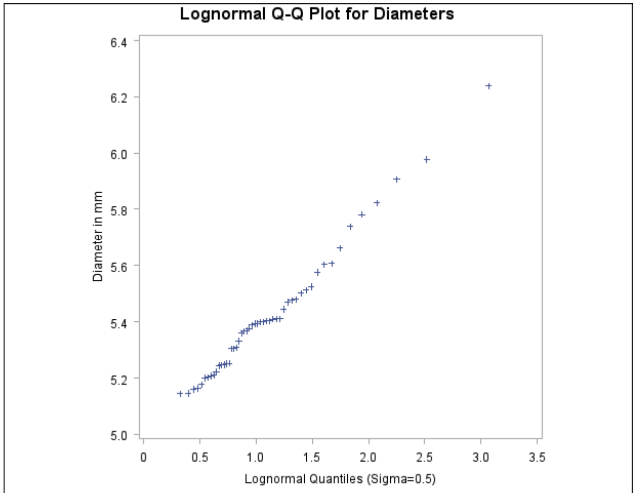
Output 5.22.2 Lognormal Quantile-Quantile Plot ( \sigma = 0.5 )
