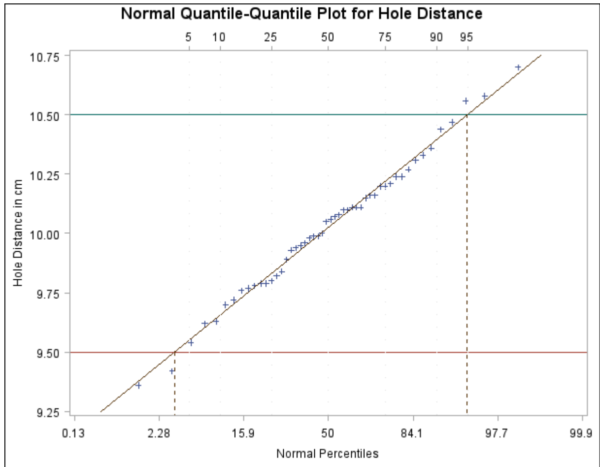
Output 5.20.5 Normal Q-Q Plot for Reading Percentiles of Specification Limits
