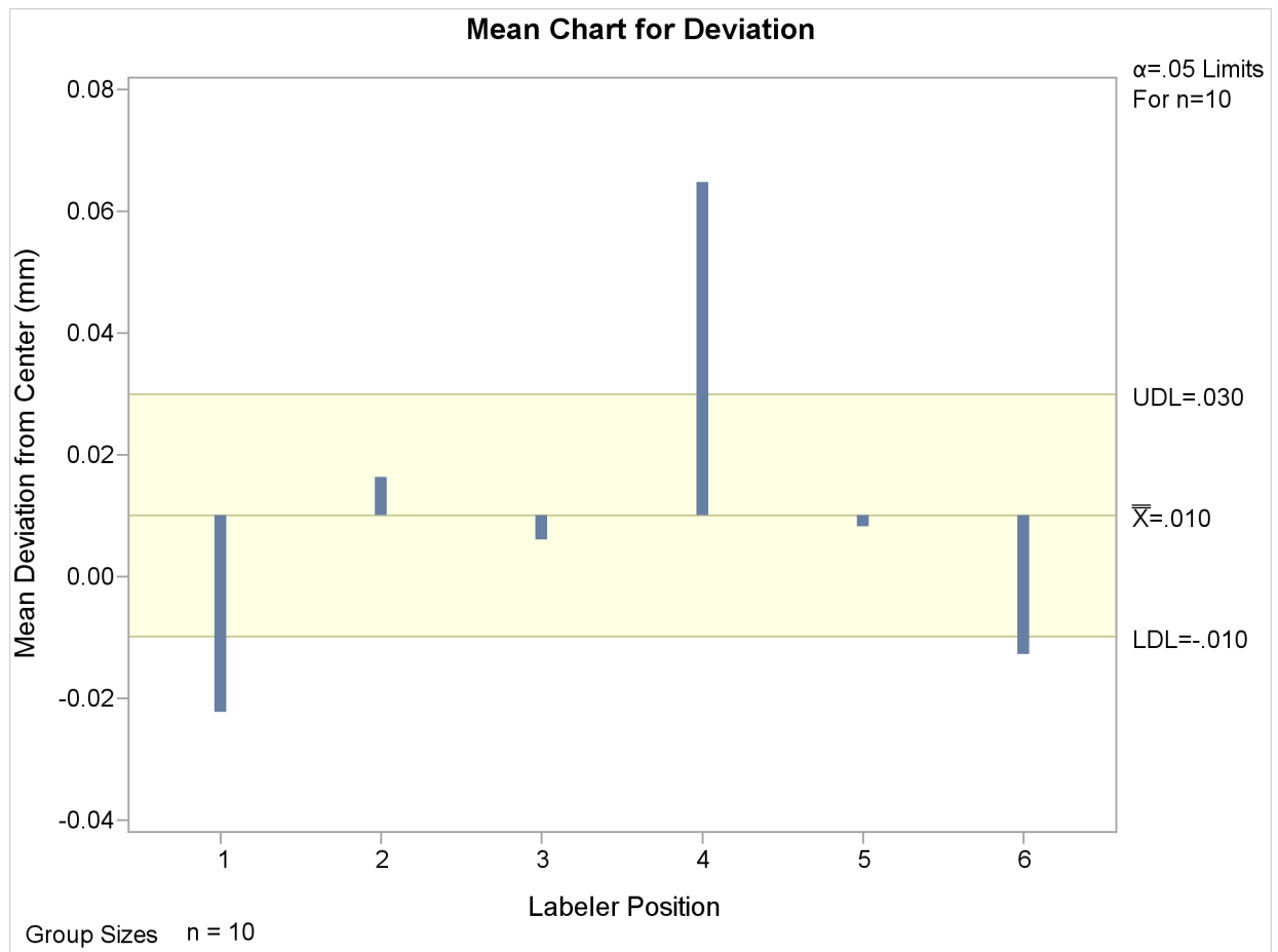
Figure 3.6 ANOM Chart
