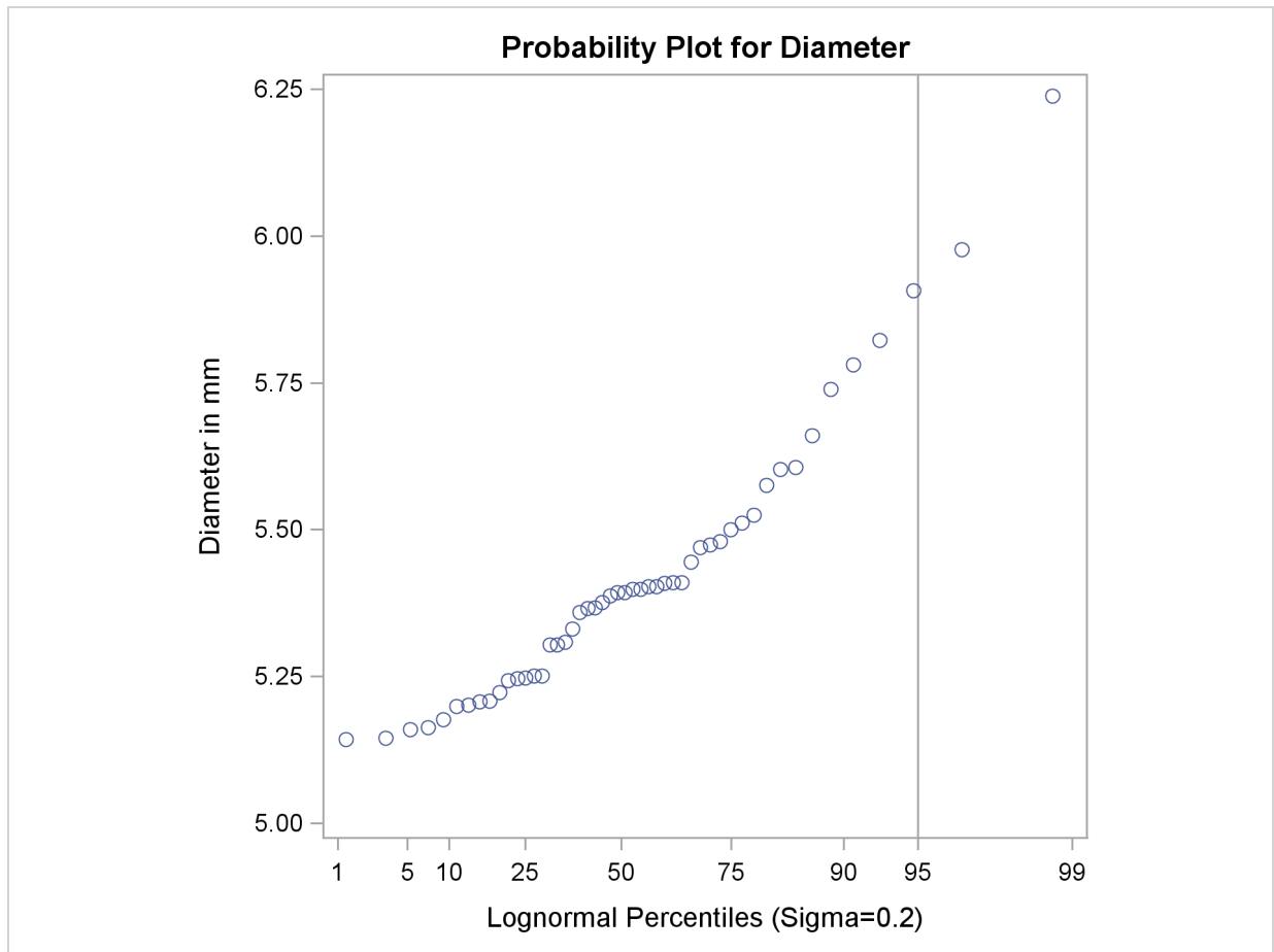
Output 5.18.7 Probability Plot Based on Lognormal Distribution with \sigma = 0.2
