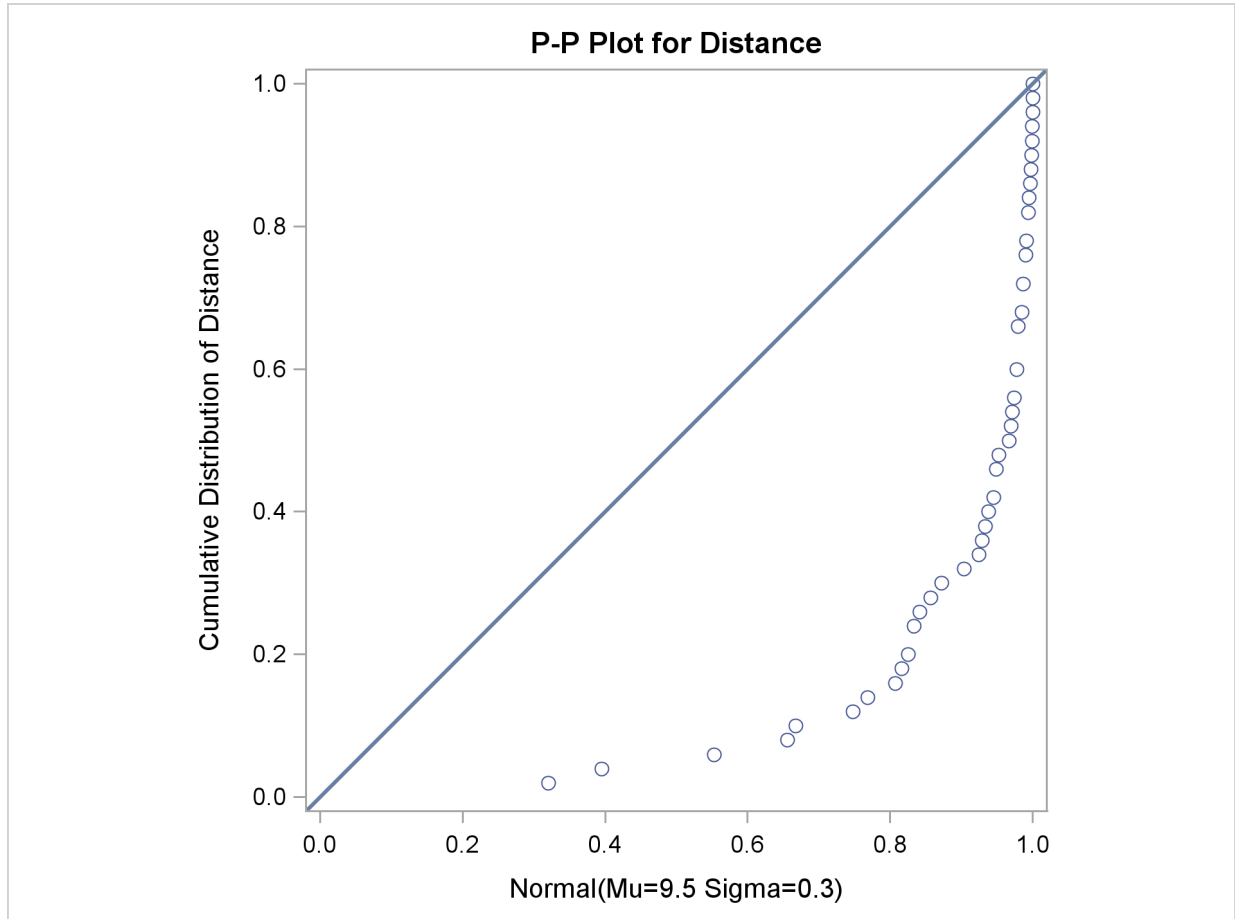
Output 5.18.4 Normal P-P Plot with Mean Specified Incorrectly
