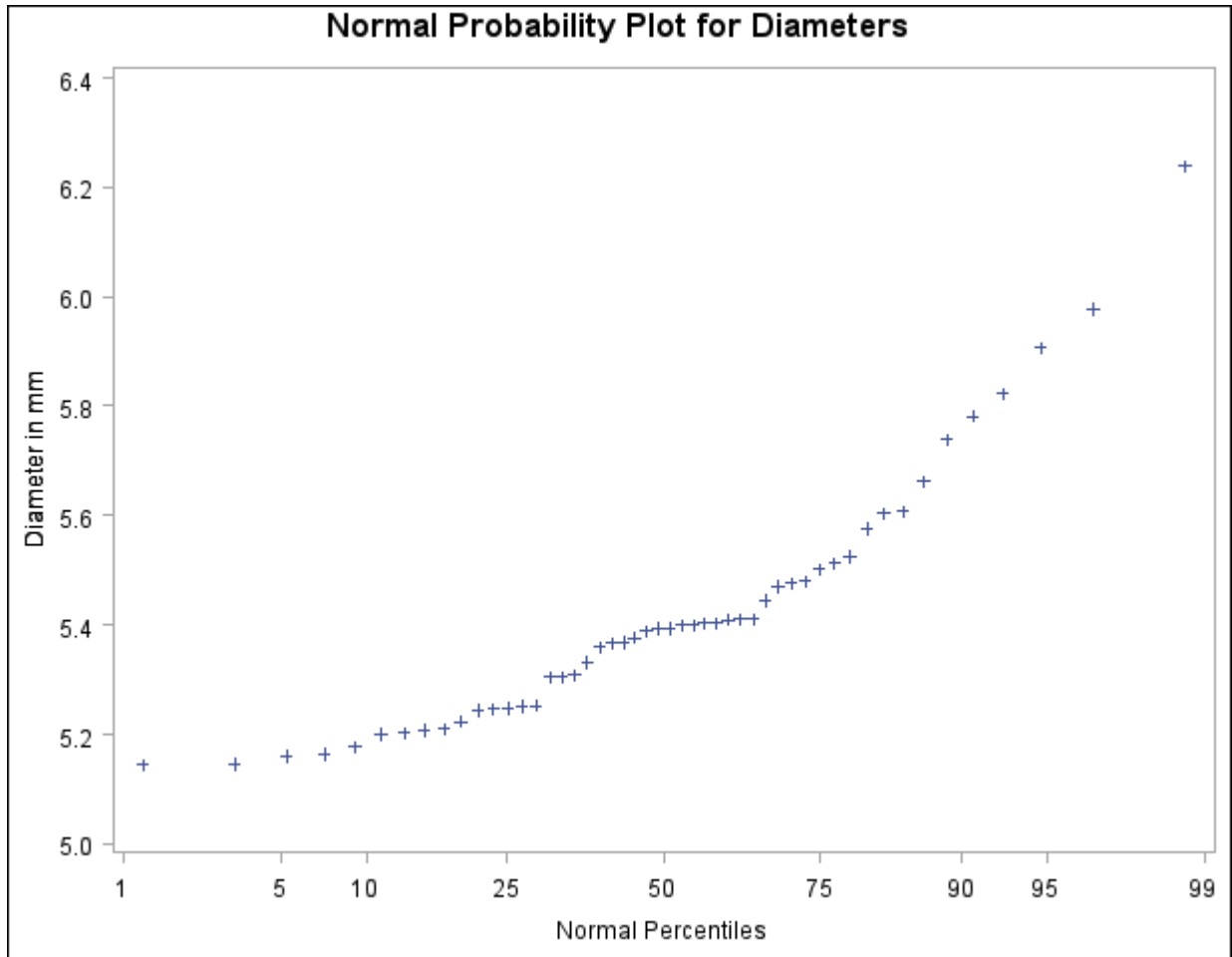
Output 5.18.6 Normal Probability Plot Created with Traditional Graphics
