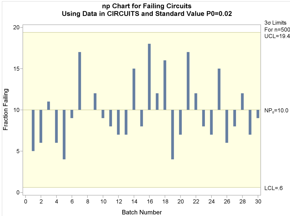
Output 13.19.1 An np Chart with Standard Value of p_0
