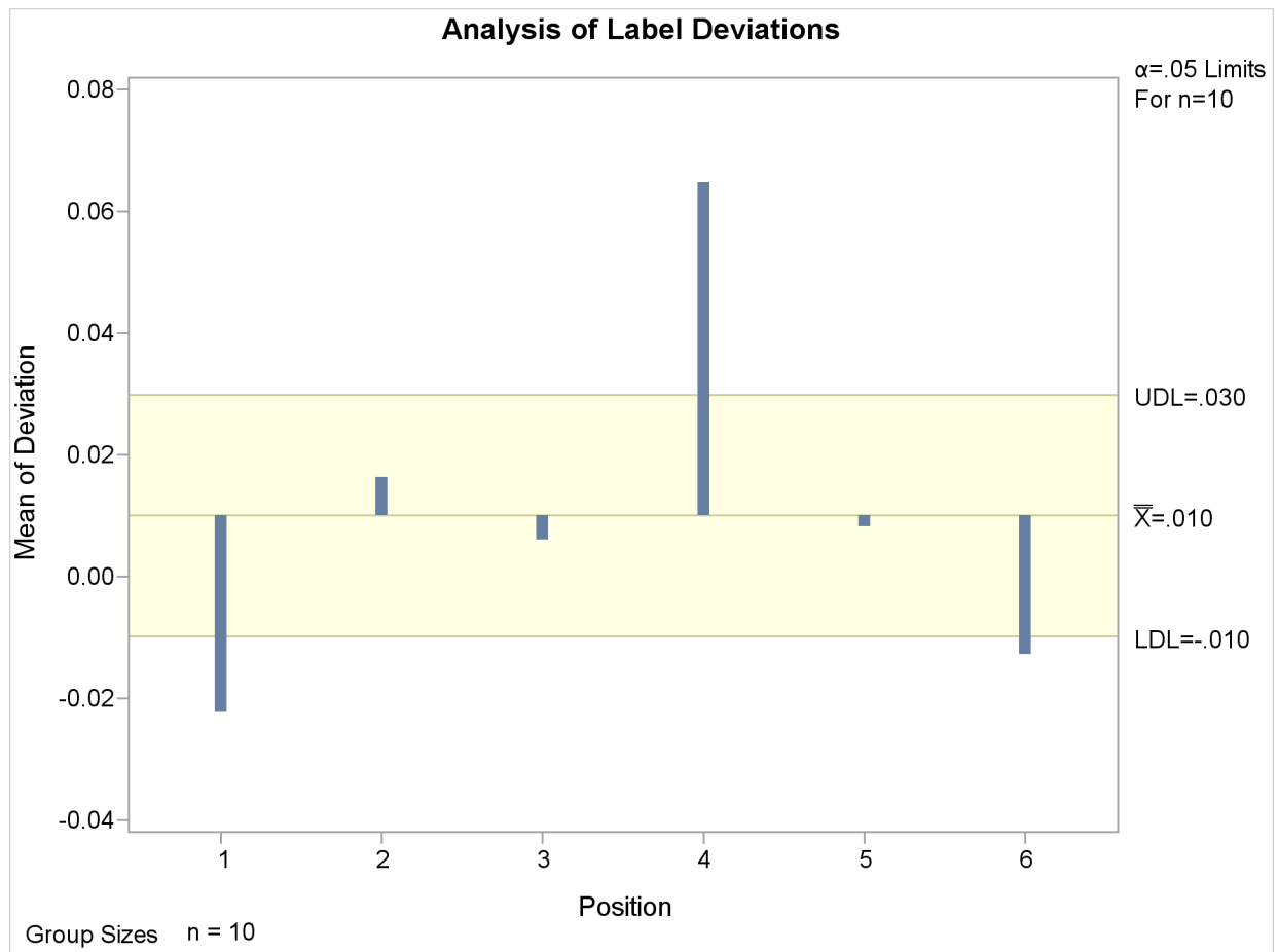
Output 4.3.5 ANOM Chart for Means in Data Set Labels
