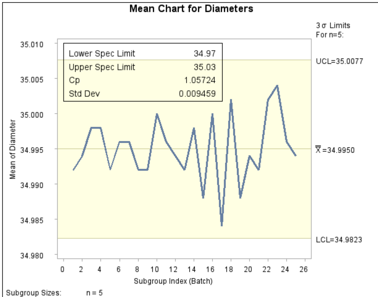
Output 13.43.5 An \bar{X} Chart with an Inset
