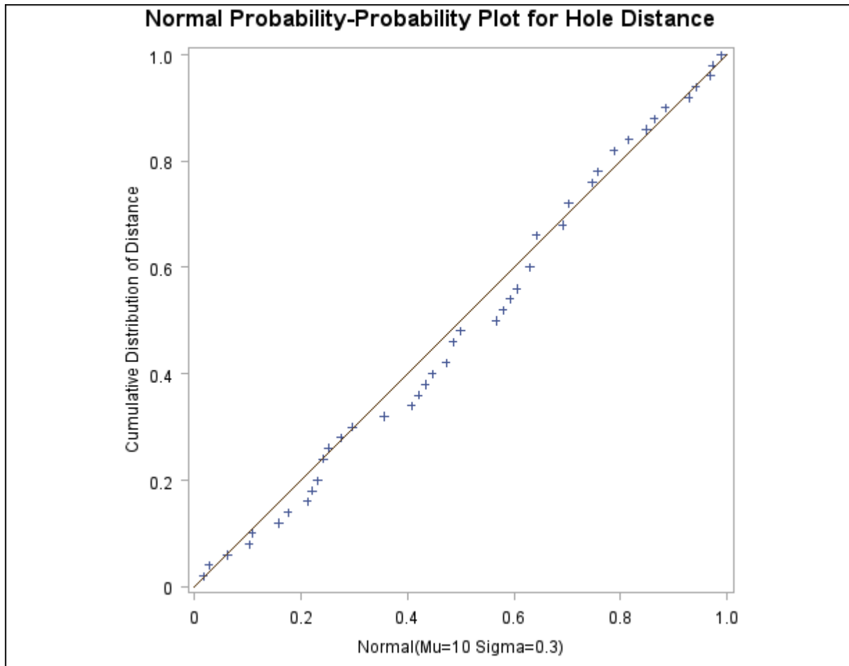
Output 5.18.3 Normal P-P Plot with Diagonal Reference Line
