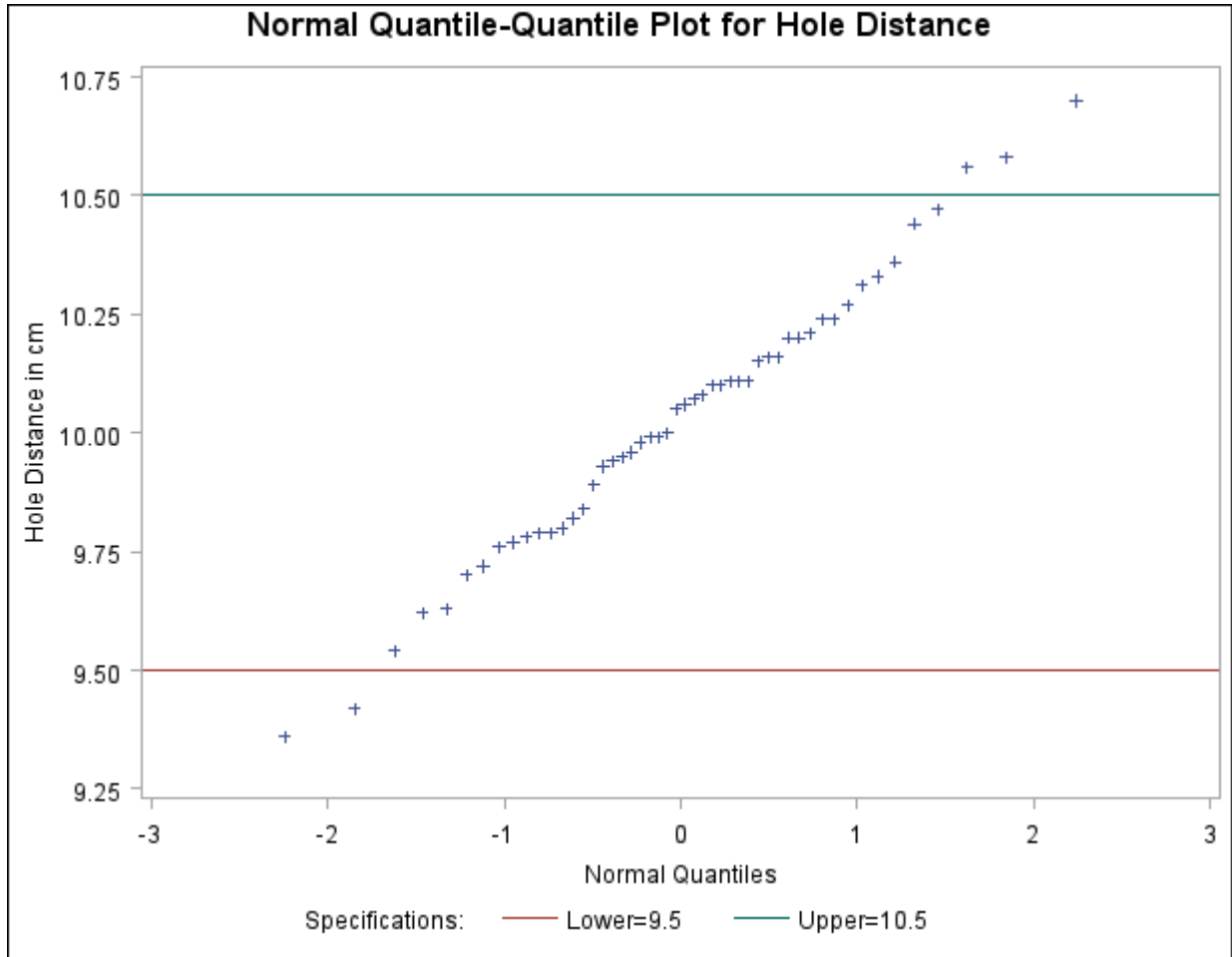
Output 5.20.2 Normal Quantile-Quantile Plot Created with Traditional Graphics
