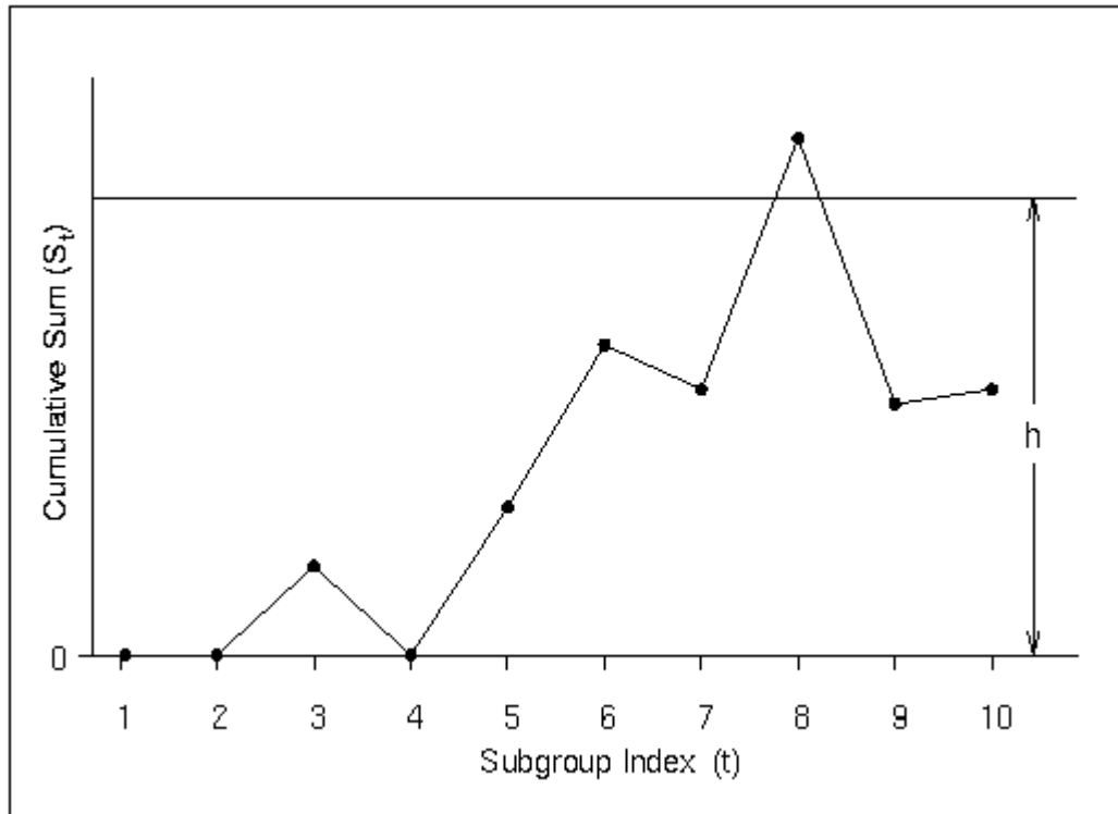
Figure 6.13 Decision Interval
