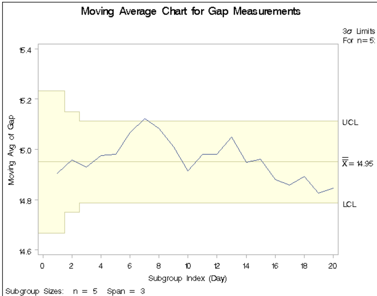
Output 9.5.4 Uniformly Weighted Moving Average Chart for Gap Data
