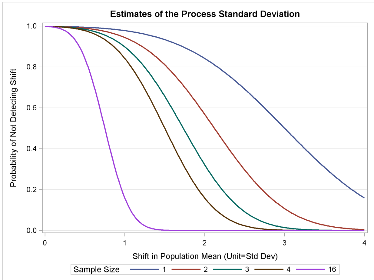
Output 13.36.1 OC Curves for Different Subgroup Sample Sizes
