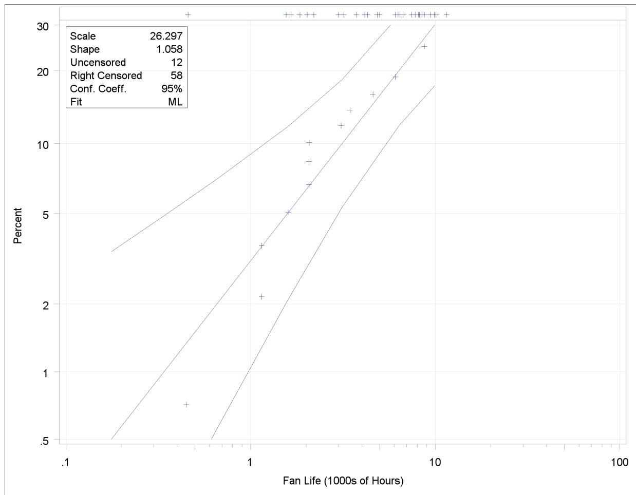
Figure 12.1 Weibull Probability Plot for Engine Fan Data (Traditional Graphics)
