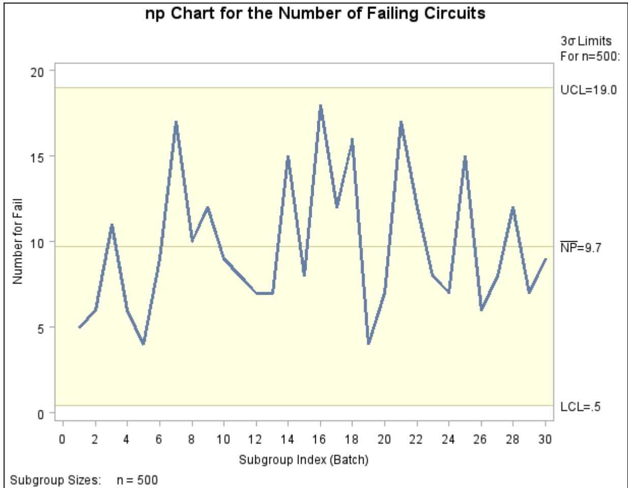
Output 13.17.4 np Chart for Circuit Failures (Traditional Graphics)
