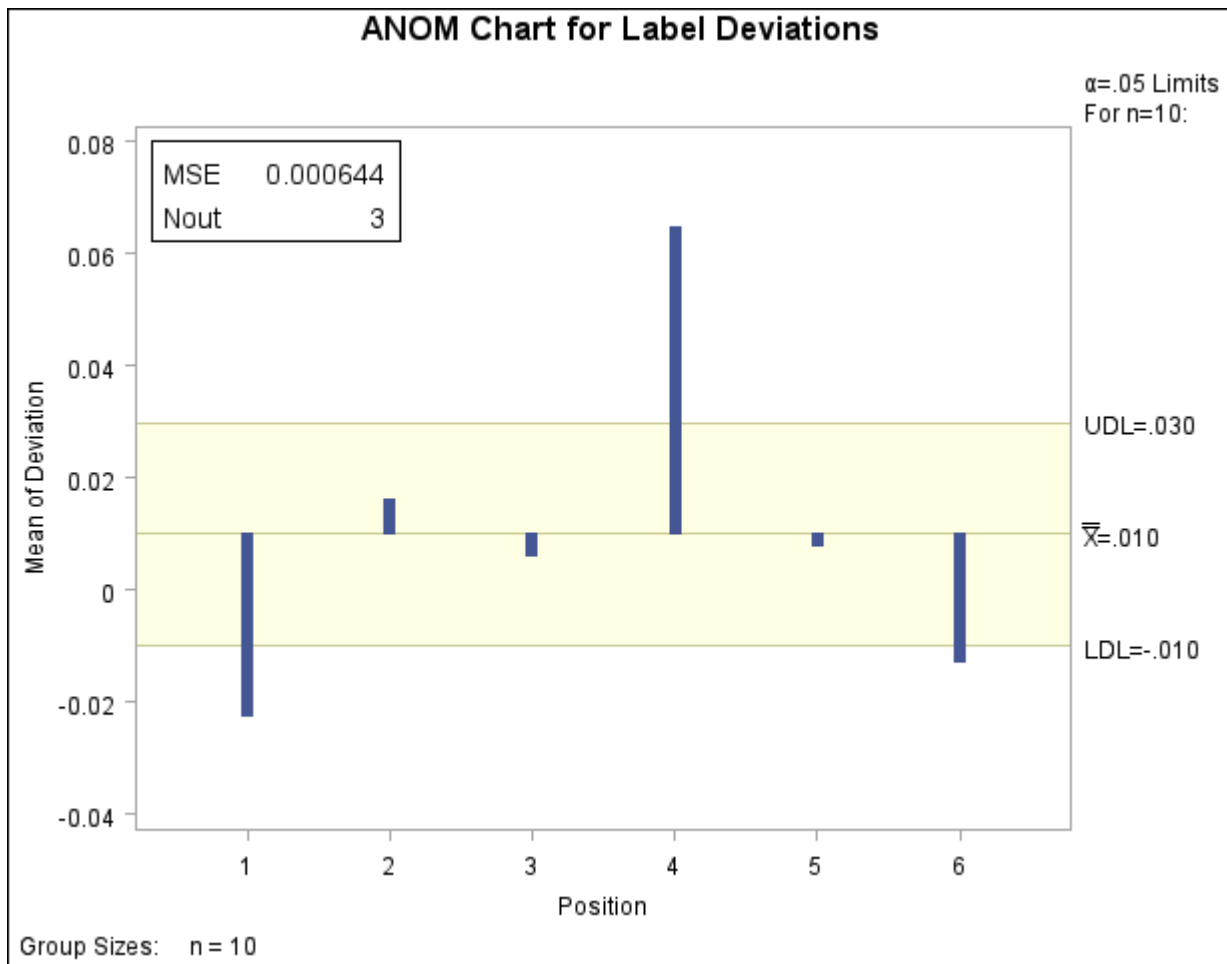
Output 4.7.4 An ANOM Chart with an Inset
