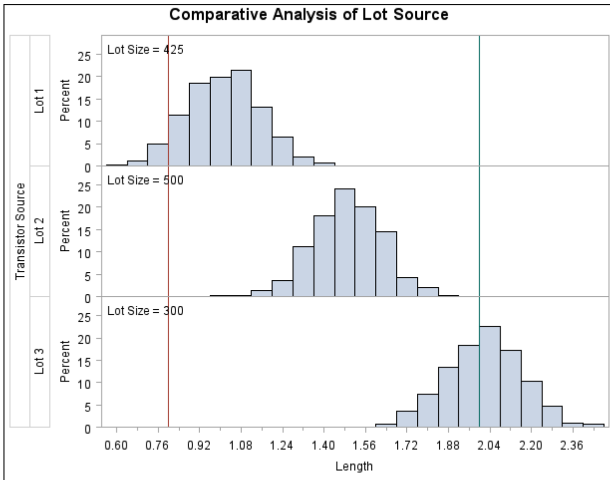
Output 5.5.2 Comparison by Lot Source
