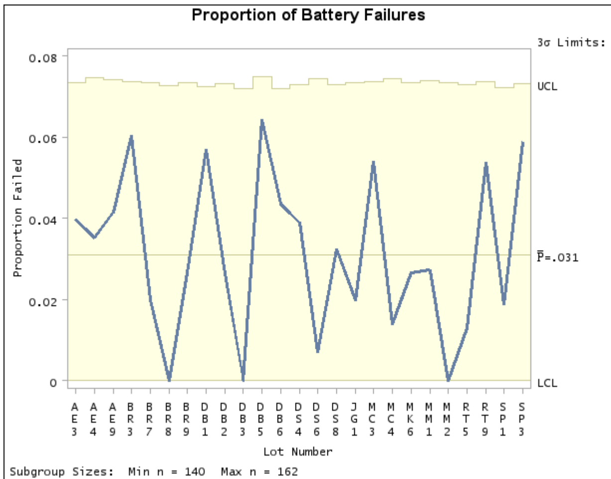
Output 13.24.1 A p Chart with Varying Subgroup Sample Sizes
