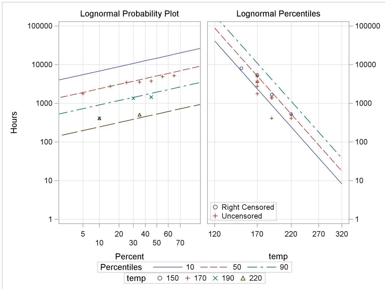
Figure 12.9 Probability and Relation Plots for the Class B Insulation Data
