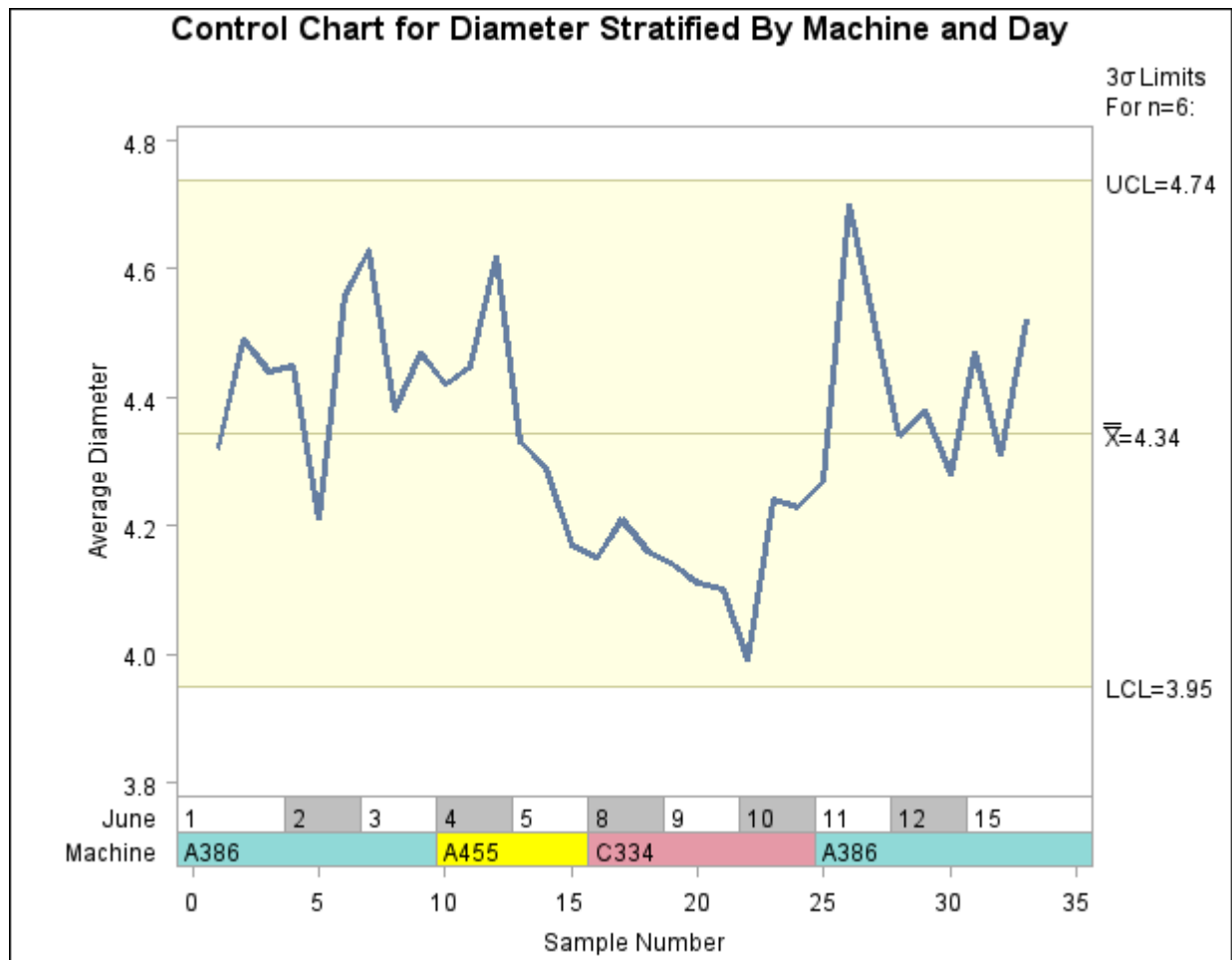
Output 13.43.30 Stratified Control Chart Using Multiple Block Variables
