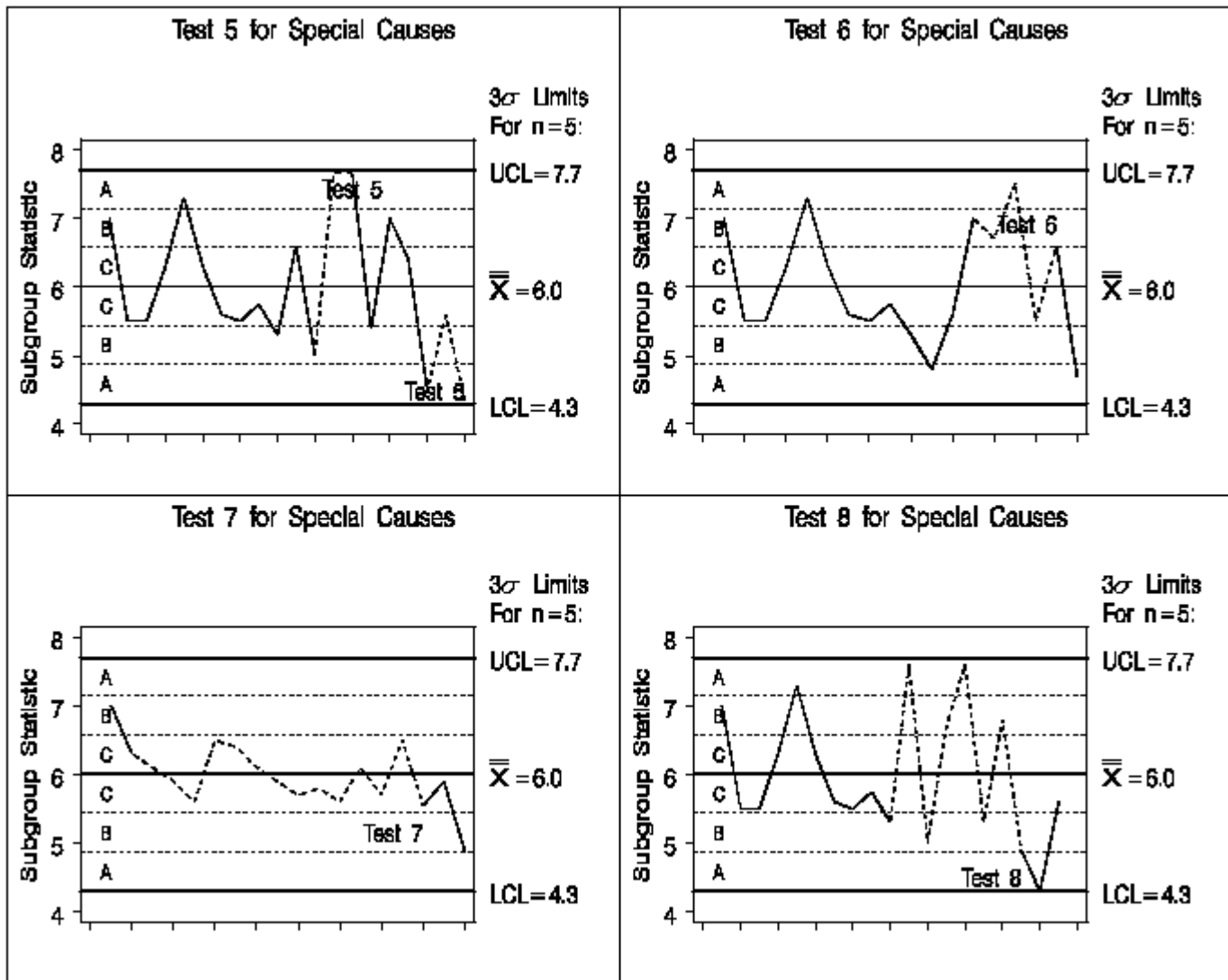
Output 13.43.62 Examples of Tests 5 to 8
