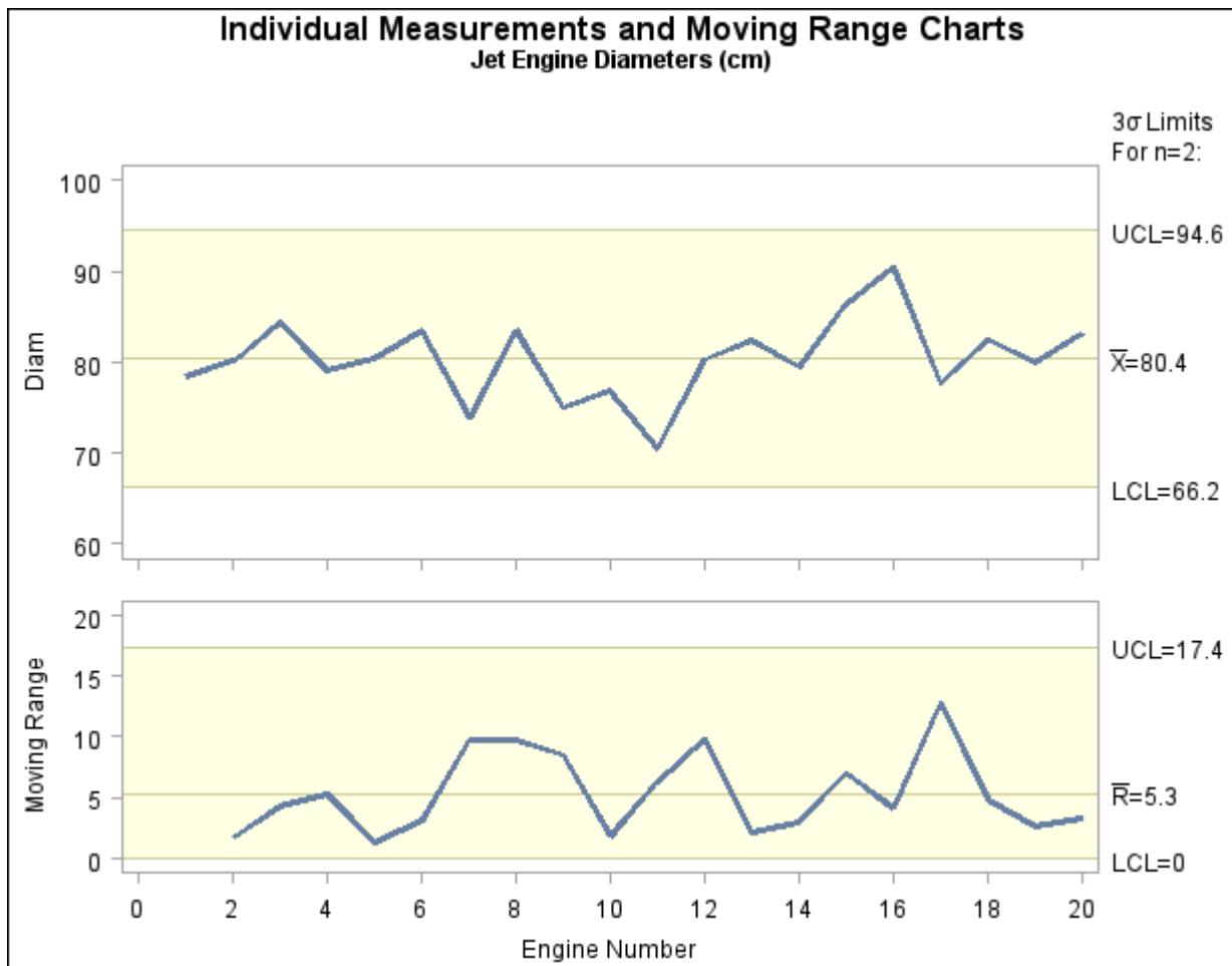
Output 13.10.4 Individual Measurements and Moving Range Charts (Traditional Graphics)
