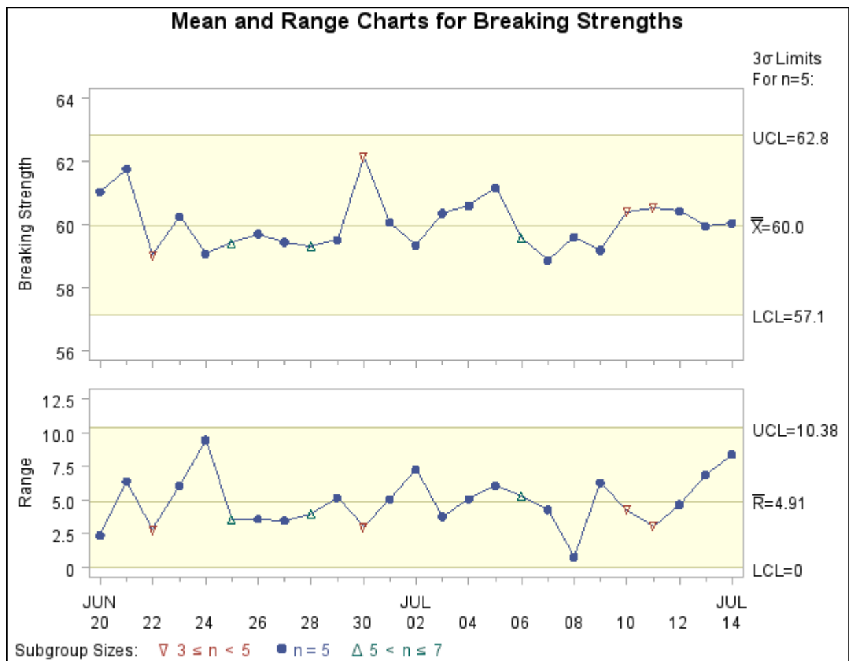
Output 13.40.3 Displaying All Subgroups Regardless of Sample Size
