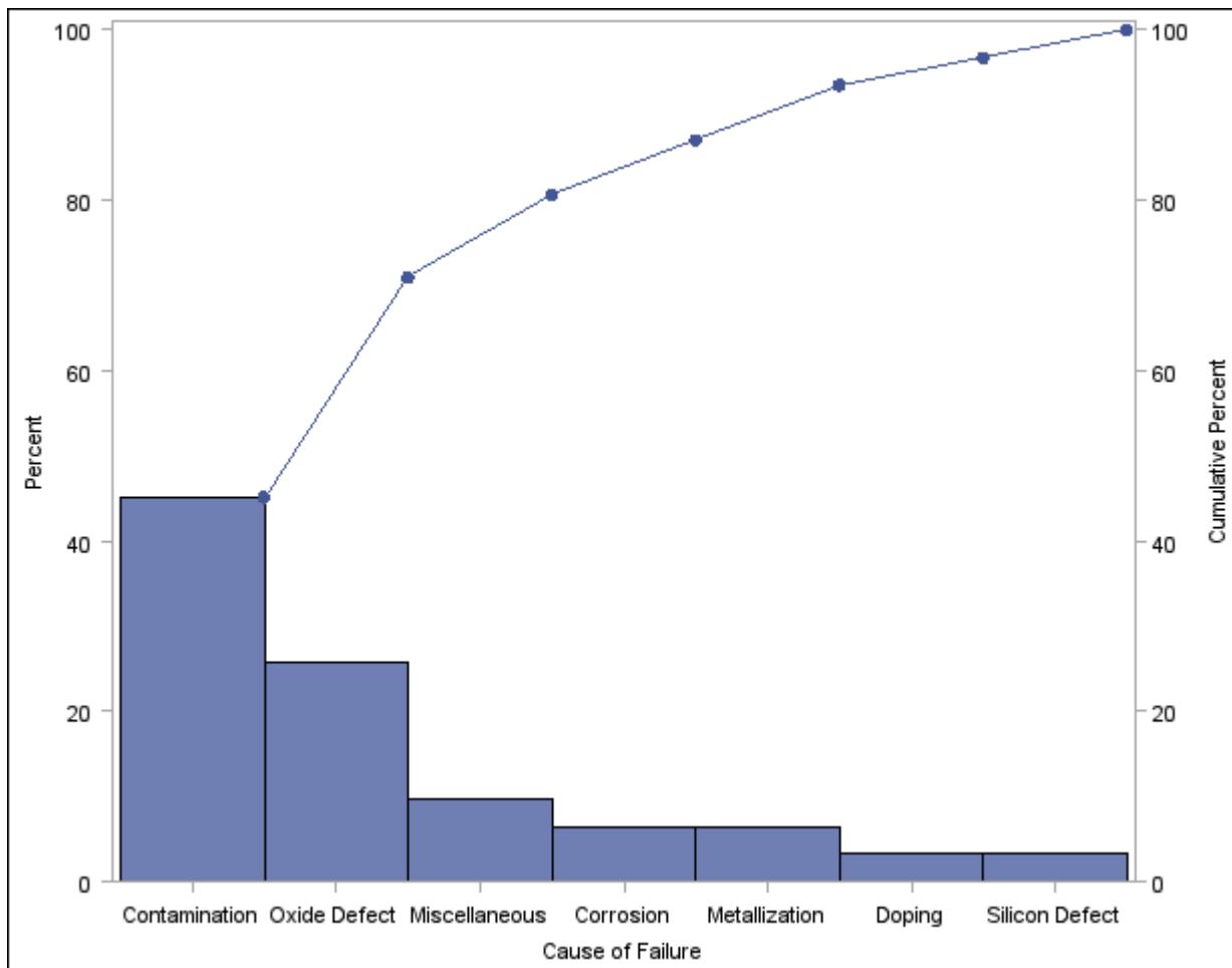
Figure 11.6 Pareto Chart for IC Failures in the Data Set Failure1
