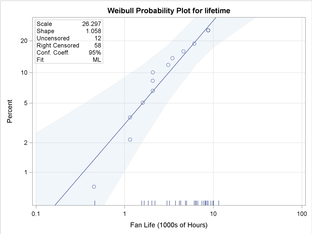
Figure 3.11 Probability Plot (RELIABILITY)
