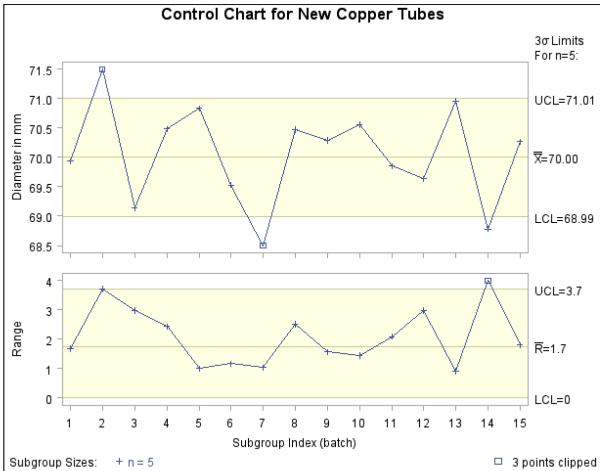
Output 13.43.53 \bar{X} and R Charts with Clip Factor of 1.5
