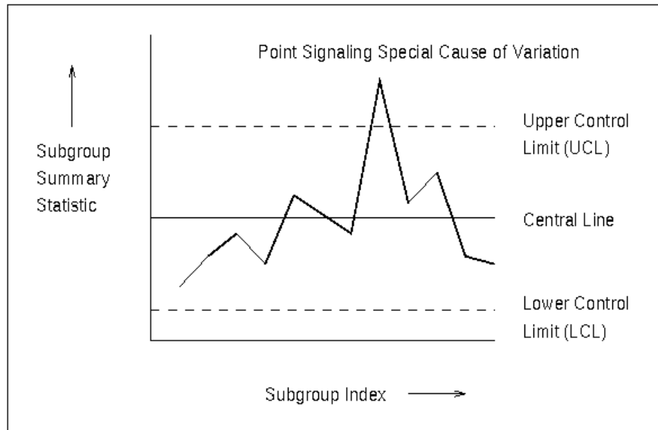
Figure 13.1 A Shewhart Control Chart
