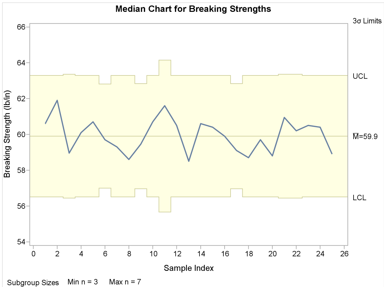
Output 13.15.1 Median Chart with Varying Sample Sizes
