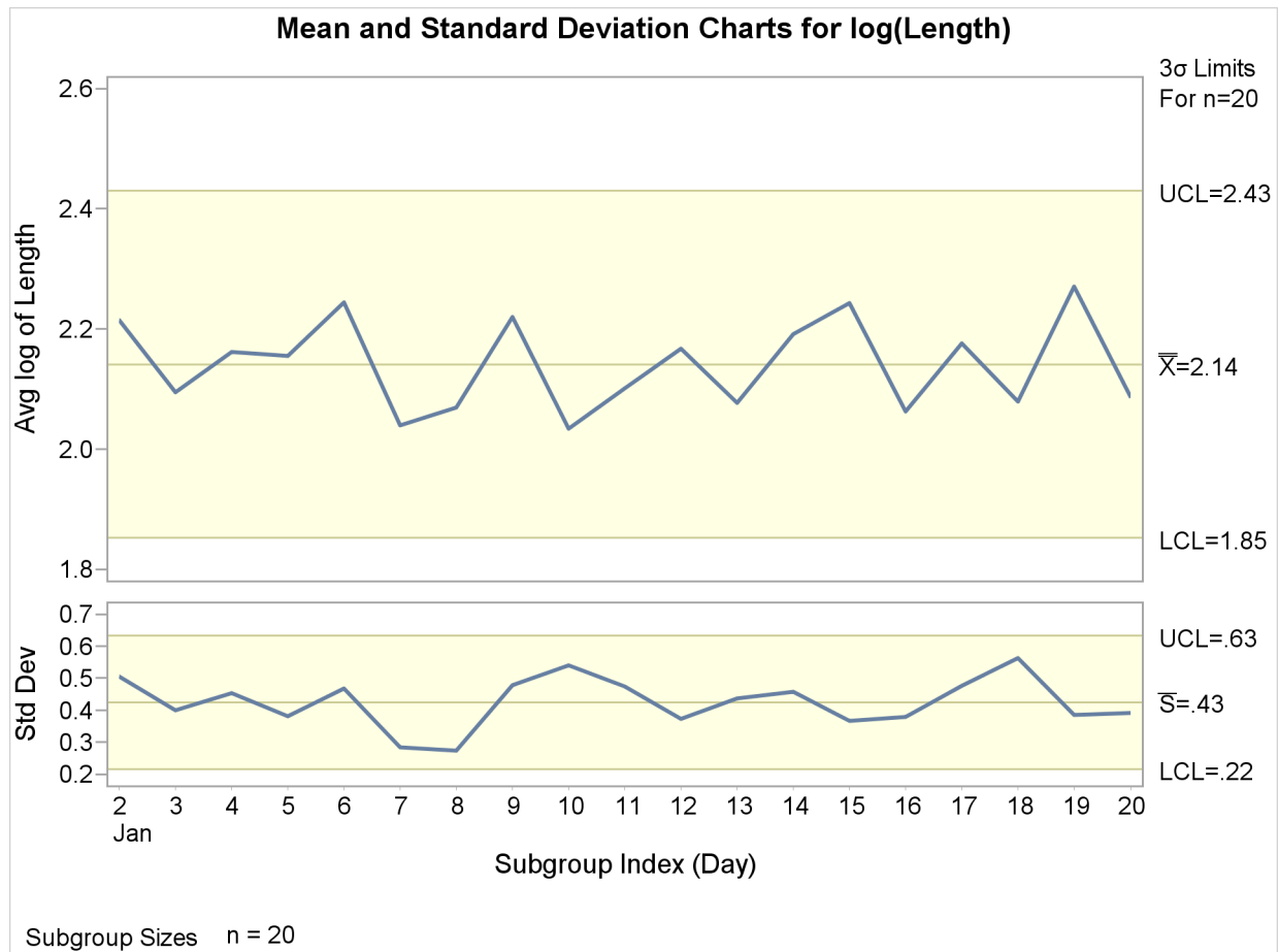
Output 13.43.4 \bar{X} and s Charts for Transformed Length
