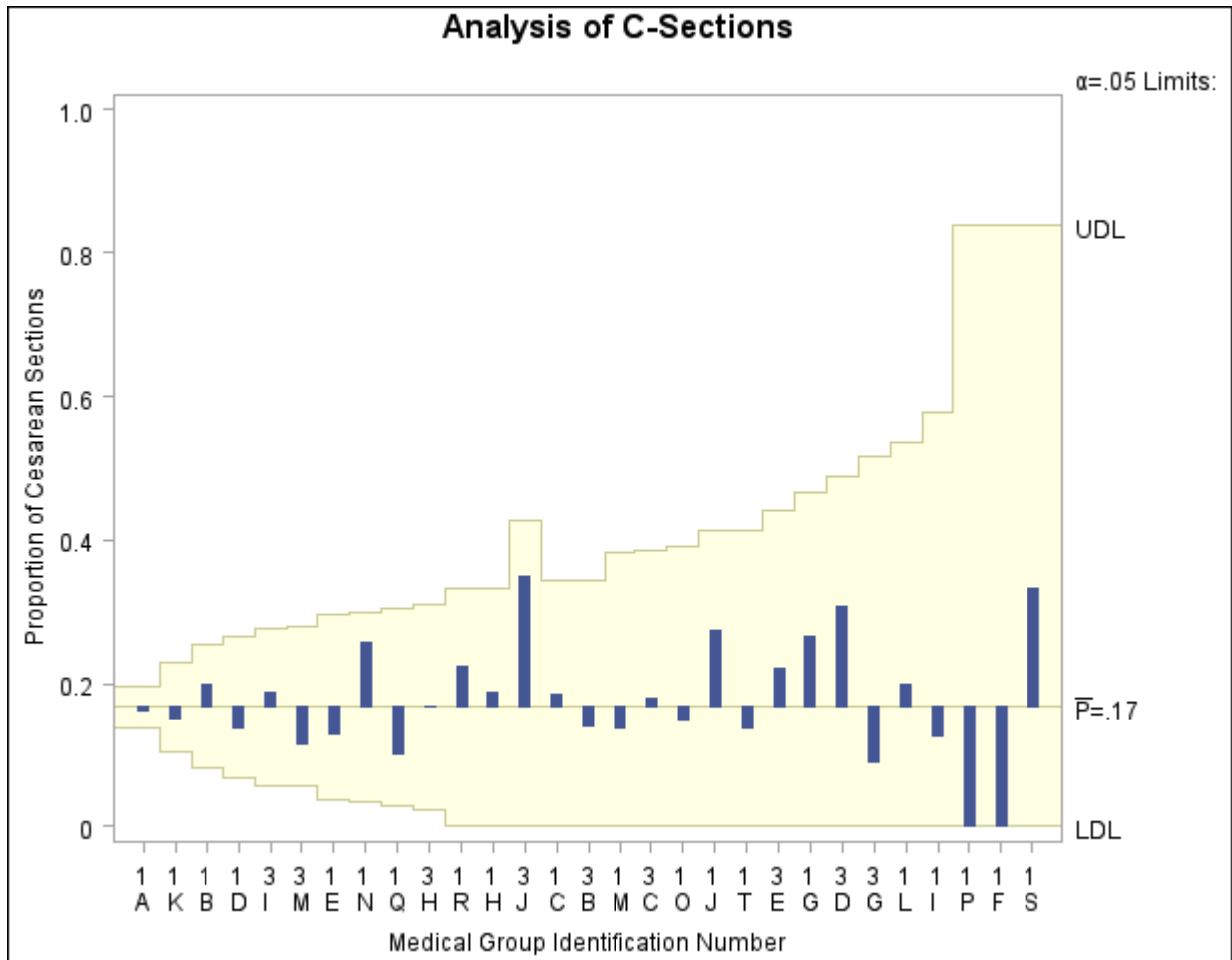
Output 4.1.3 ANOM p Chart for Cesarean Sections
