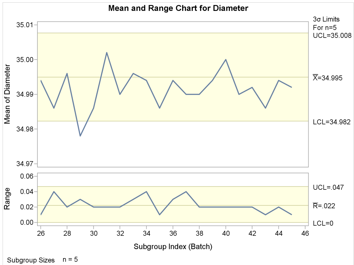
Output 13.37.10 \bar{X} and R Charts for Second Set of Wafer Data (ODS Graphics)
