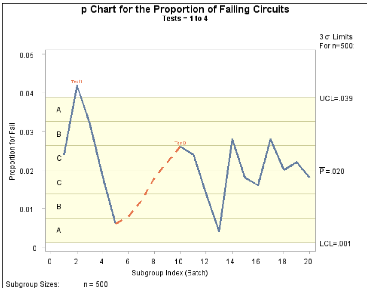
Output 13.22.1 Tests for Special Causes Displayed on p Chart
