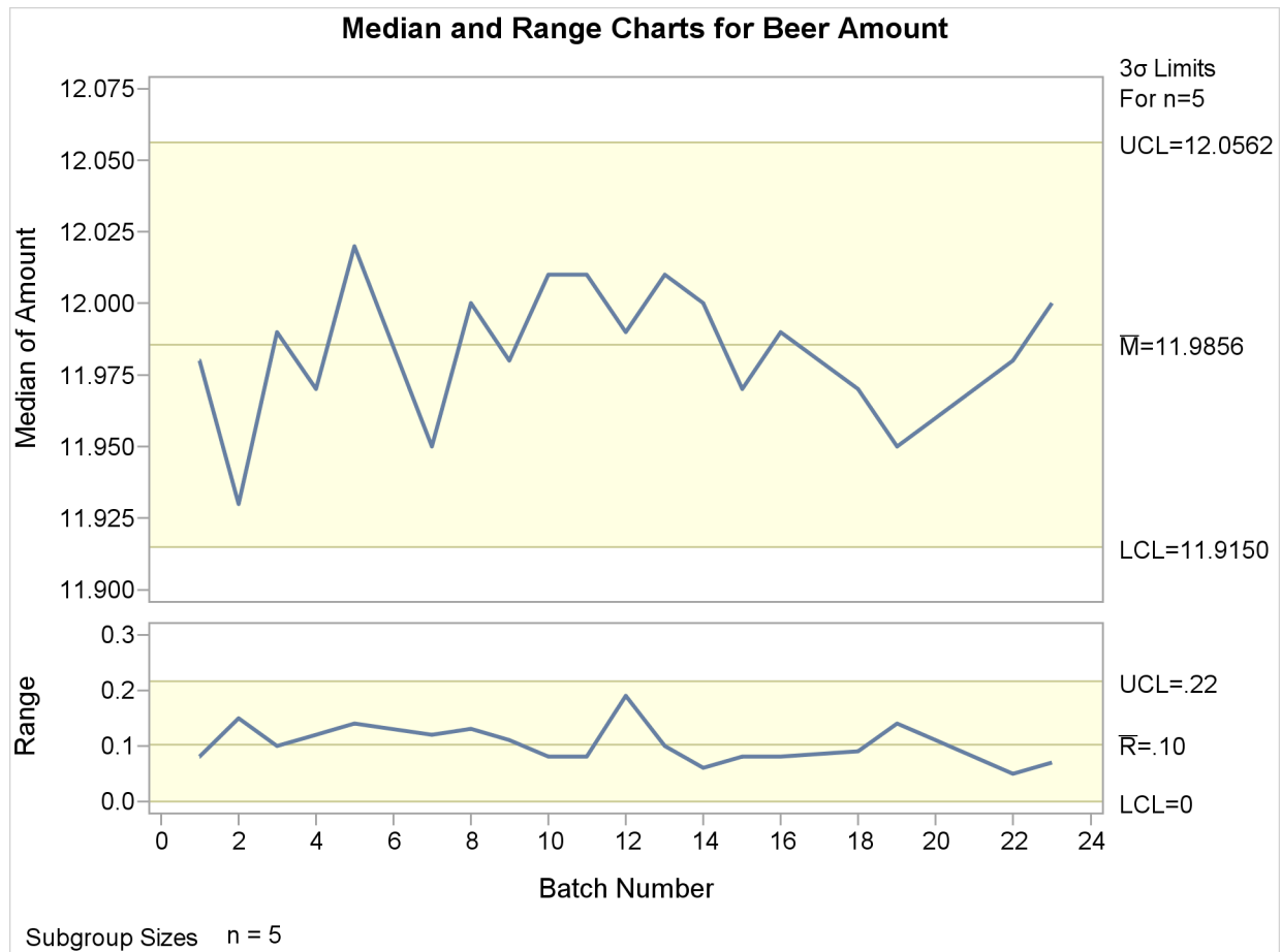
Output 13.16.2 Control Limits Based on Fixed Sample Size
