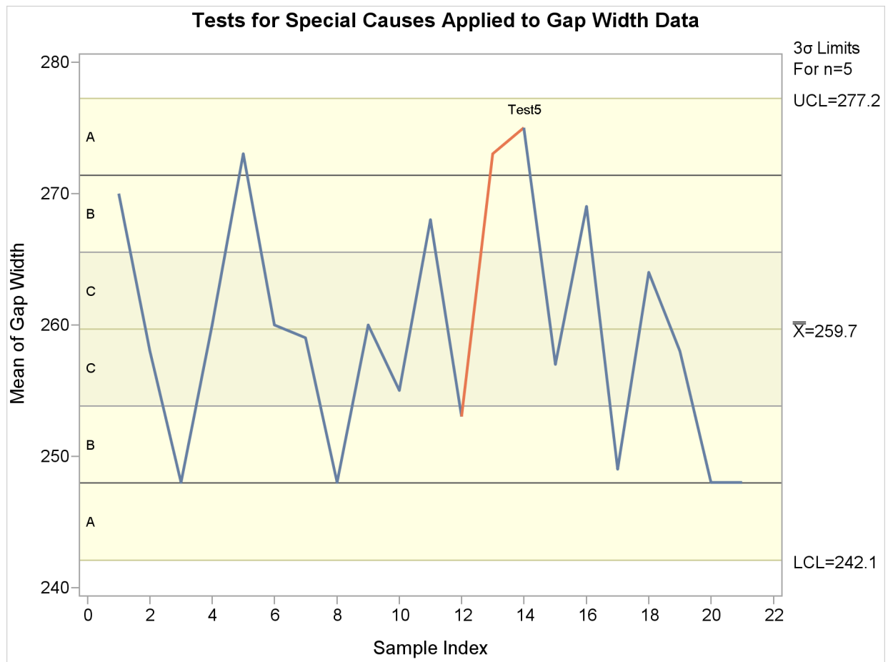
Output 13.34.1 Tests for Special Causes Displayed on an \bar{X} Chart
