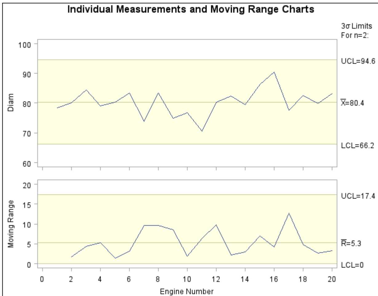
Output 13.10.6 Charts Produced from Summary Data Set Jetinfo
