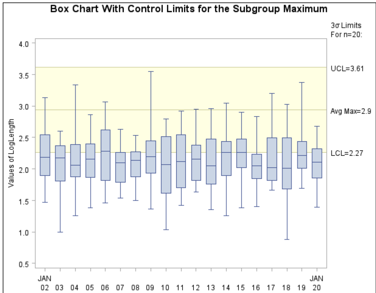
Output 13.6.1 Box Chart for Subgroup Maximum
