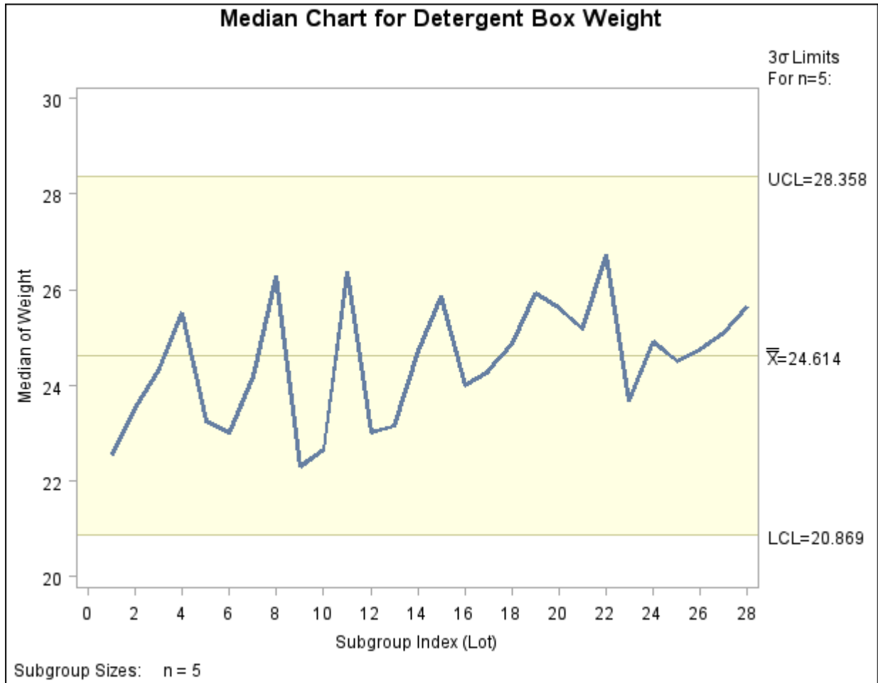
Output 13.14.2 Central Line is Average of Subgroup Means
