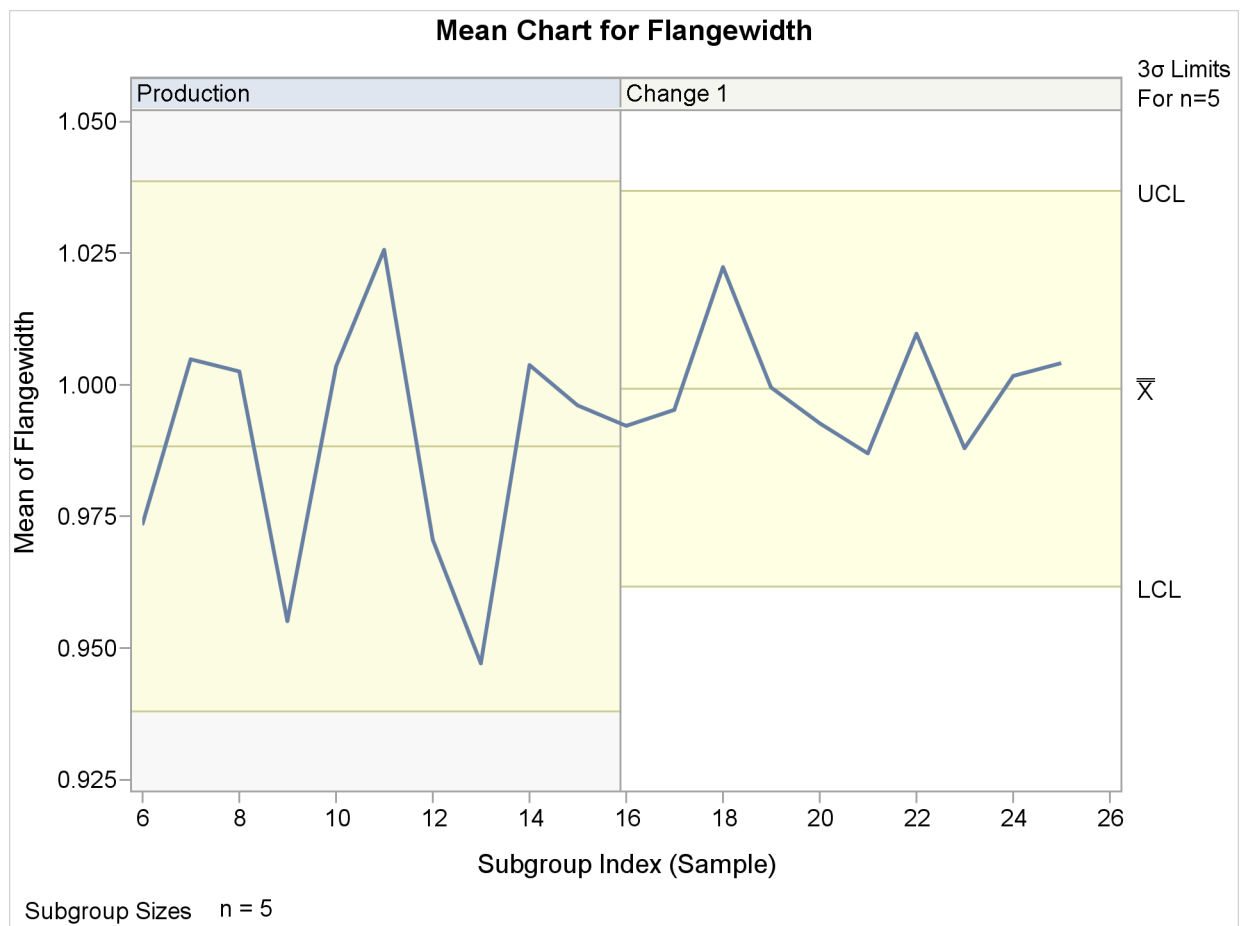
Output 13.43.22 Multiple Control Limits for Multiple Phases
