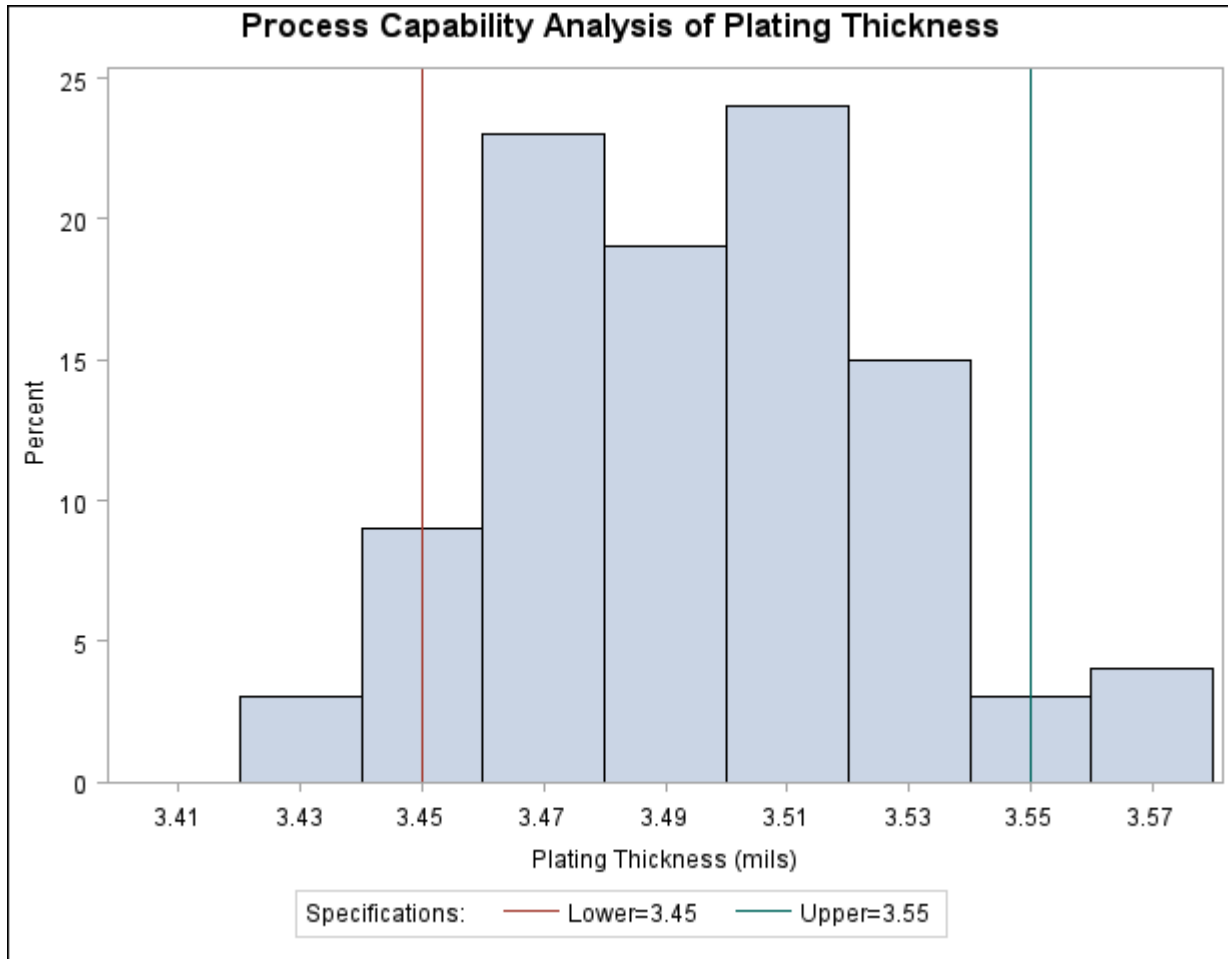
Output 5.7.2 Histogram Created with Traditional Graphics
