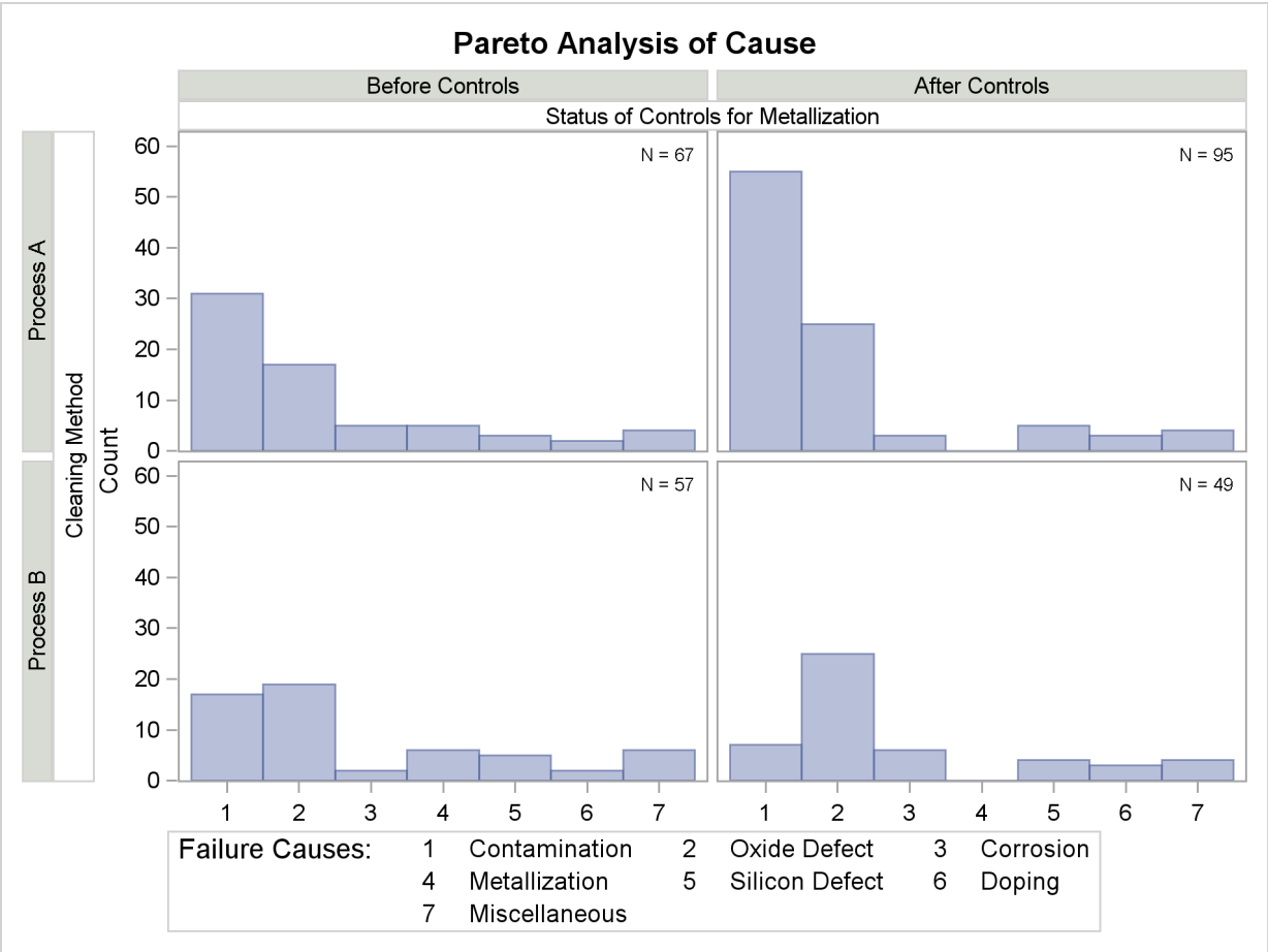
Figure 3.10 Pareto Chart
