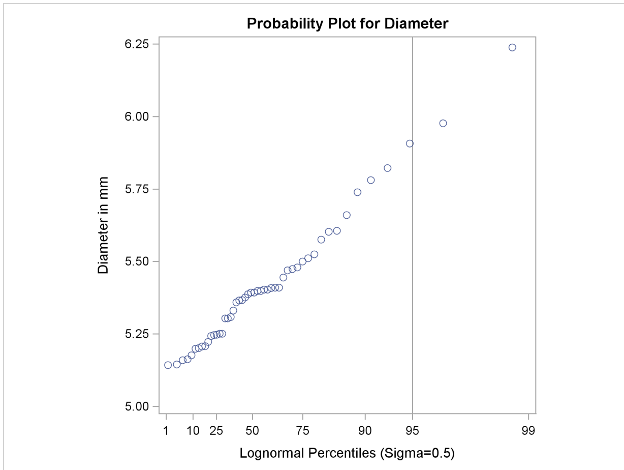
Output 5.18.8 Probability Plot Based on Lognormal Distribution with \sigma = 0.5
