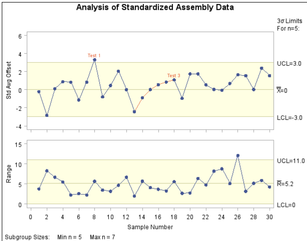
Output 13.43.65 Tests with Standardized Means
