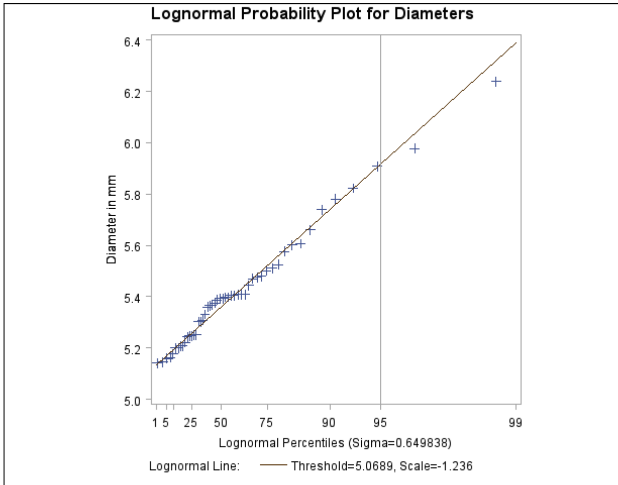
Output 5.18.10 Probability Plot Based on Lognormal Distribution with Estimated \sigma
