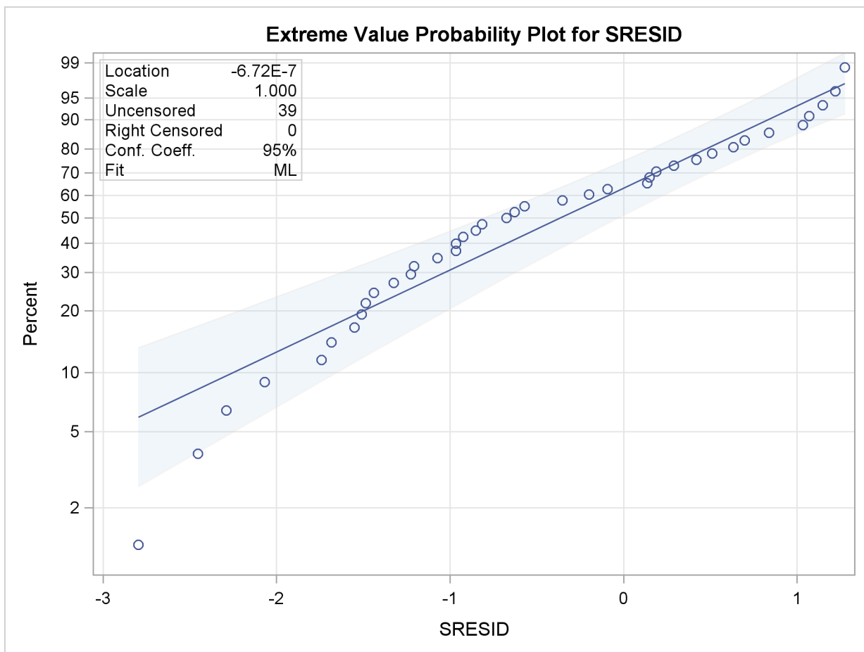
Figure 12.20 Extreme Value Probability Plot for the Standardized Residuals
