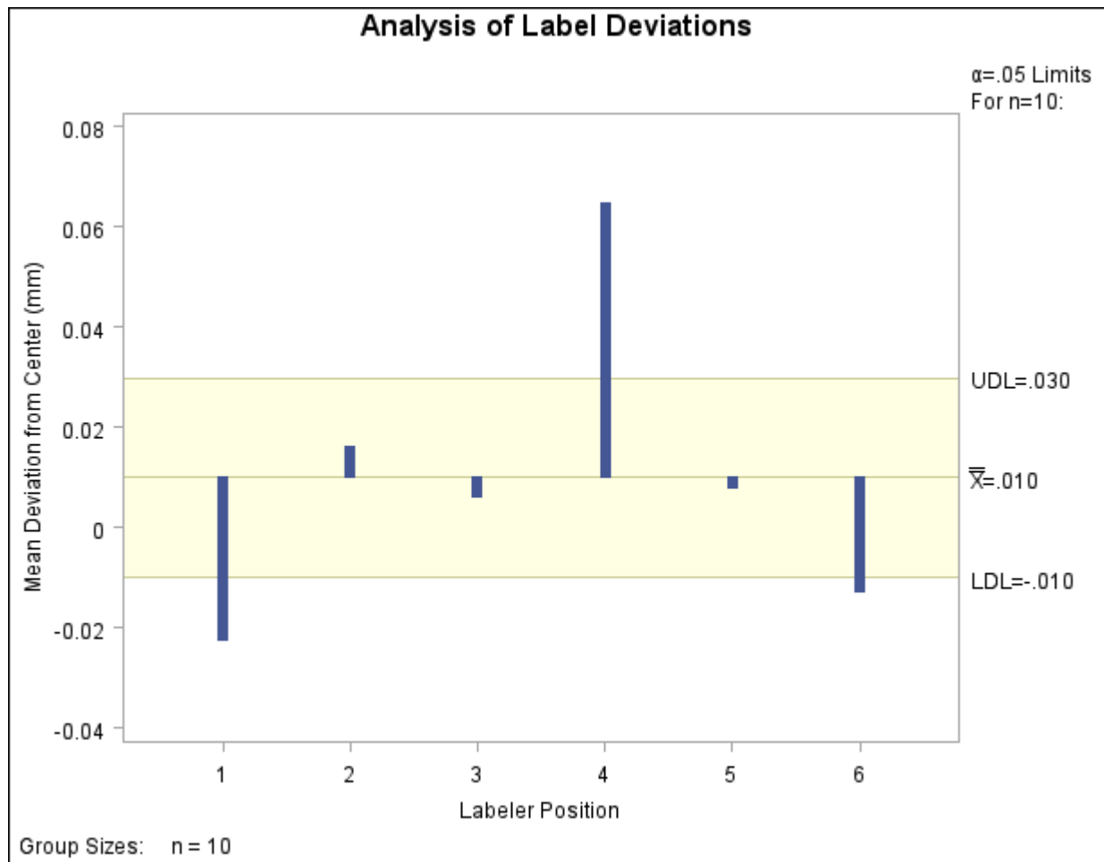
Output 4.3.3 ANOM Chart for Means of Labeler Position Data
