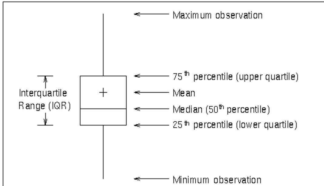
Figure 4.9 Box-and-Whisker Plot
