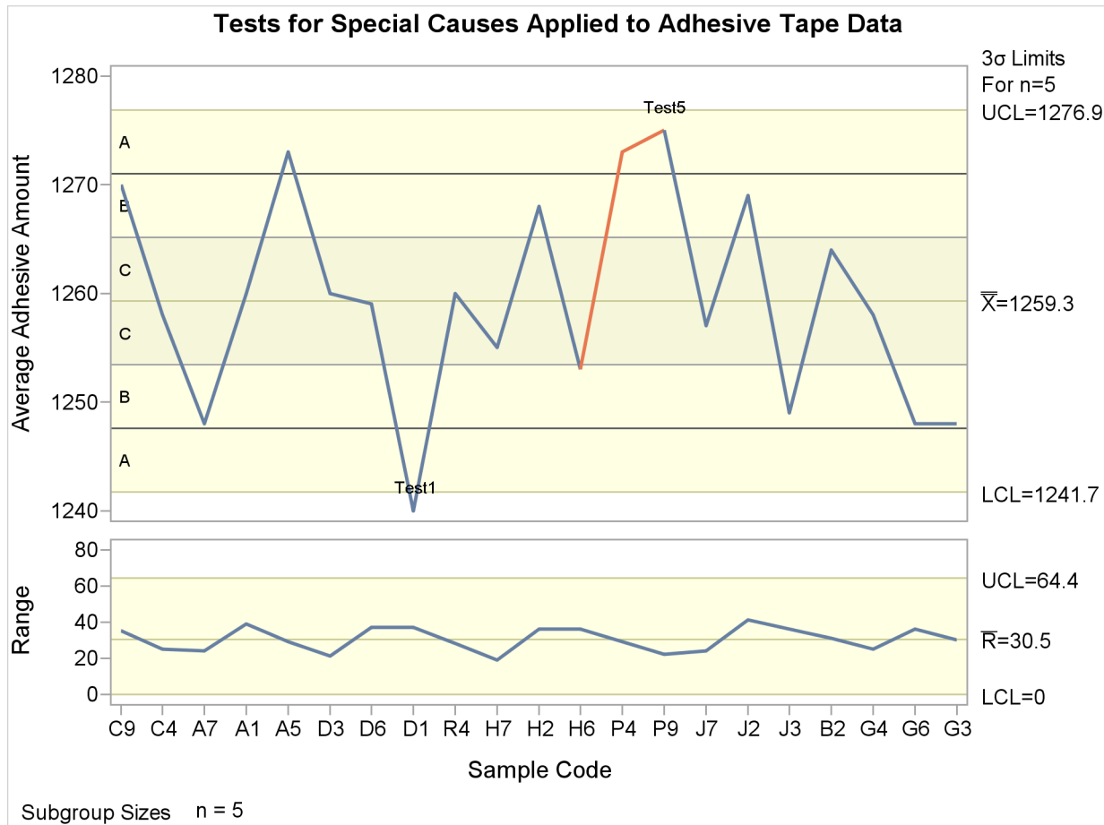
Output 13.38.1 Tests for Special Causes Displayed on \bar{X} and R Charts
