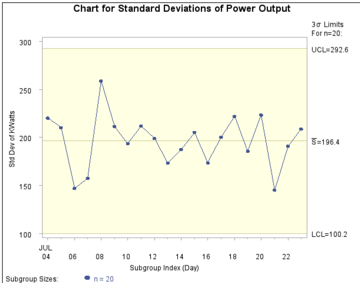
Output 13.28.4 s Chart for Power Output Data (Traditional Graphics)
