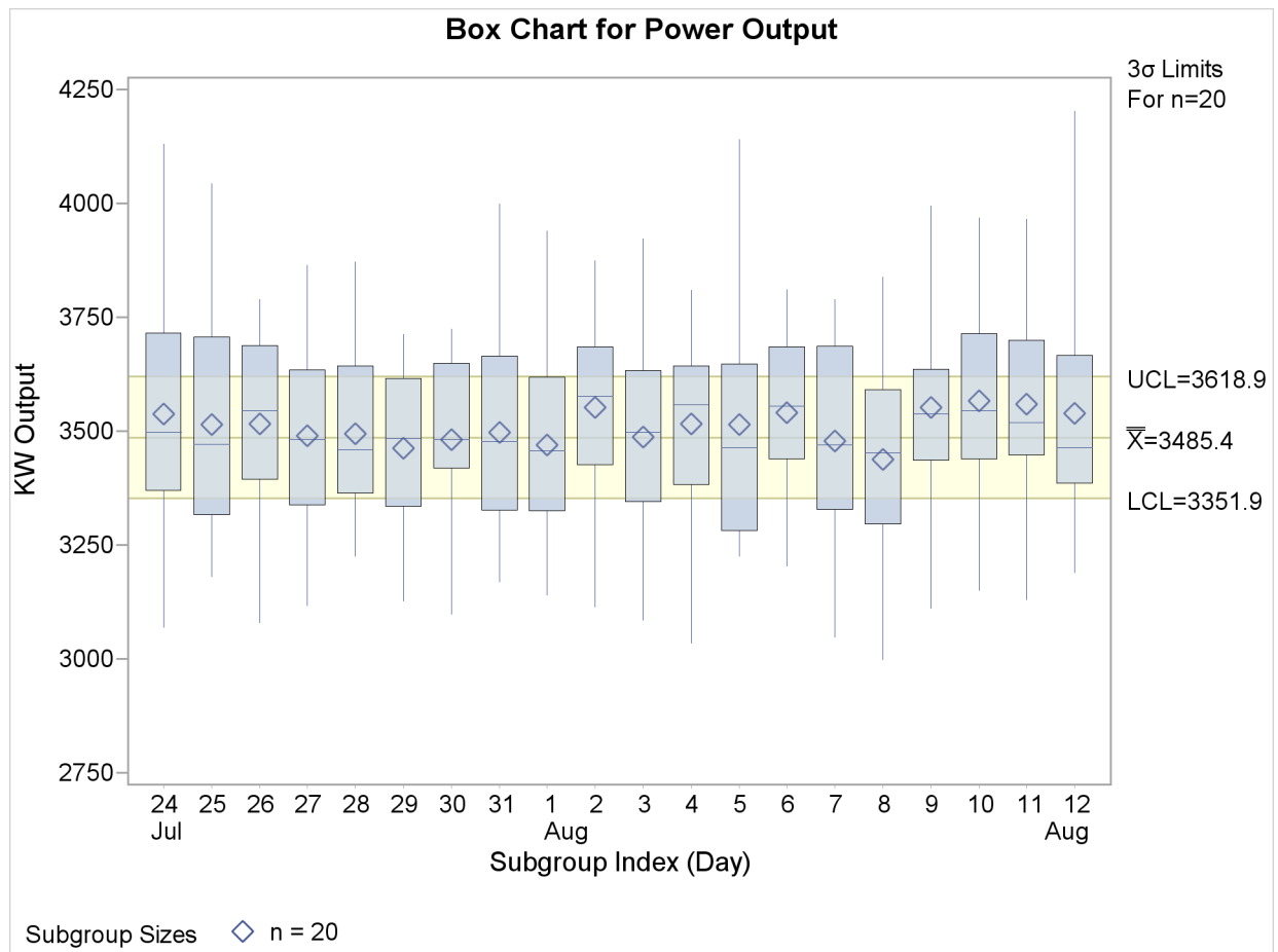
Figure 13.13 Box Chart for Second Set of Power Outputs (ODS Graphics)
