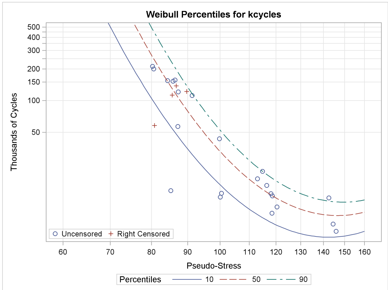
Figure 12.22 Superalloy Fatigue Data with Fitted Regression Model
