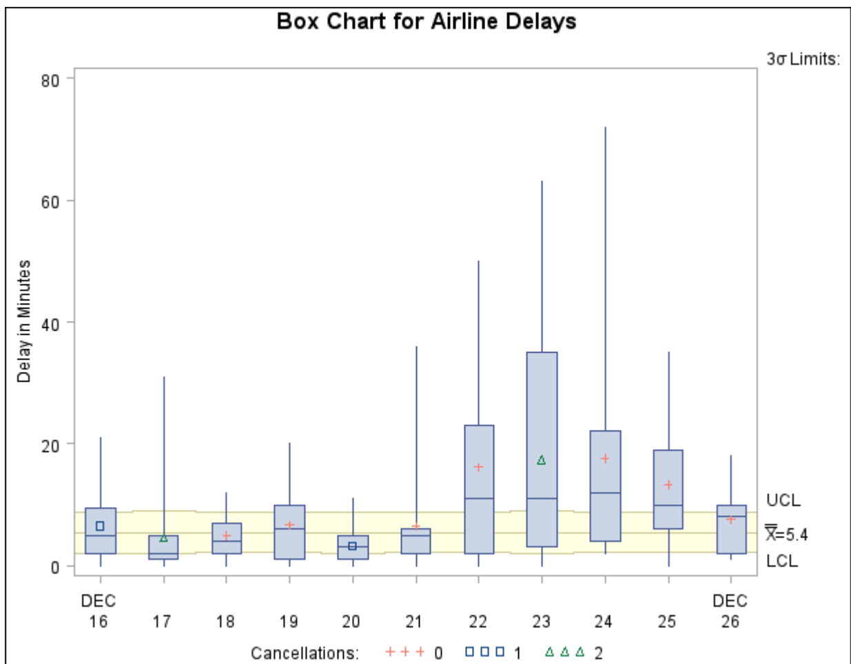
Output 13.1.1 Box Chart for Airline Data
