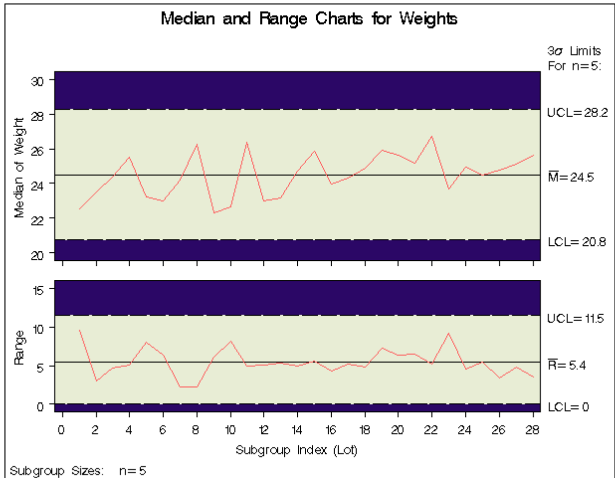
Output 13.15.6 Median and Range Charts from Summary Data Set Detsum (Traditional Graphics with NOGSTYLE)
