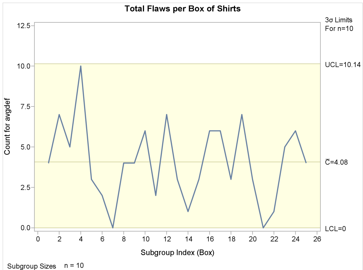
Output 13.7.10 c Chart for Boxes of Shirts (ODS Graphics)
