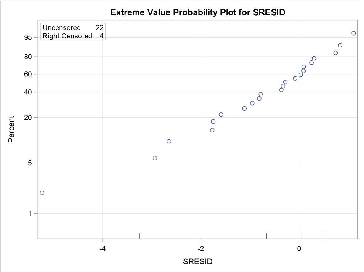
Figure 12.23 Residuals for Superalloy Fatigue Data Regression Model
