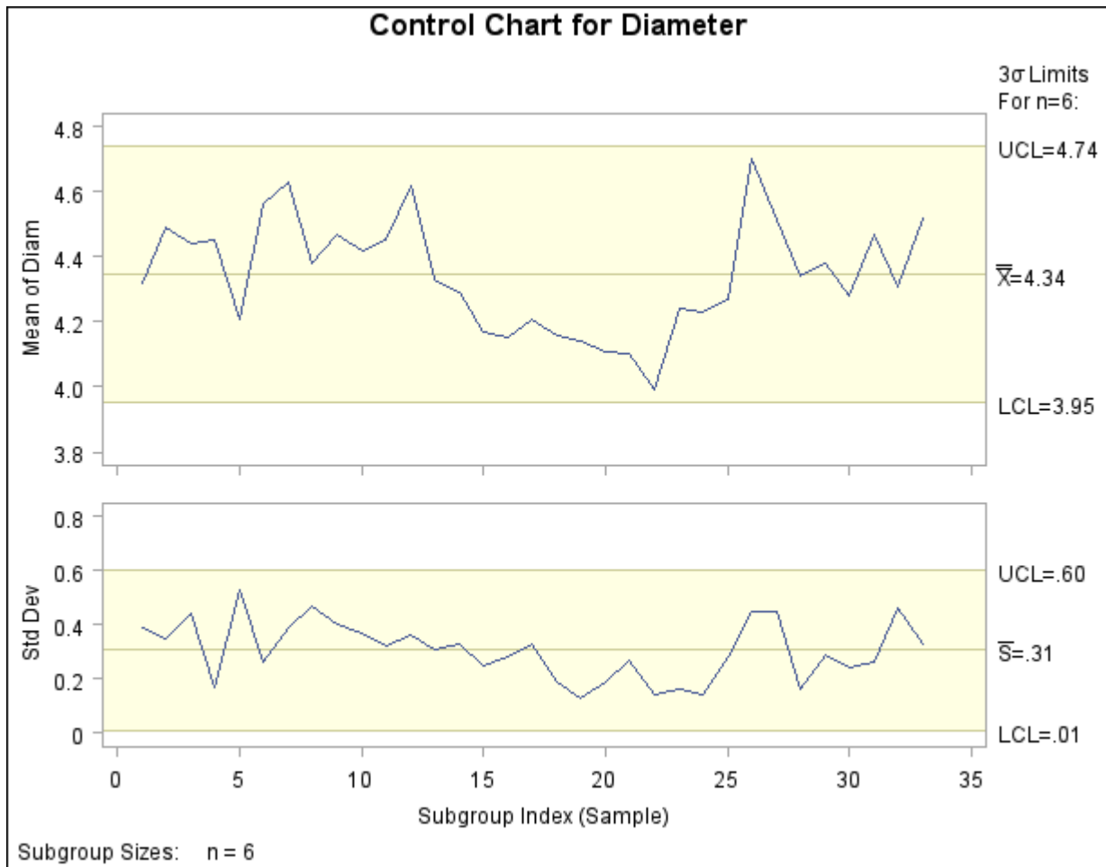
Output 13.43.55 Control Charts with Default Labels
