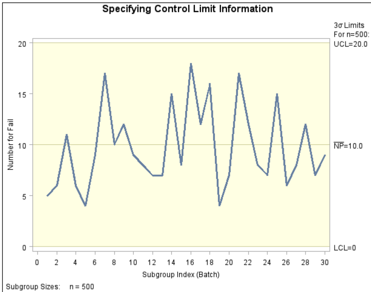
Output 13.21.1 Control Limit Information Read from Climits1
