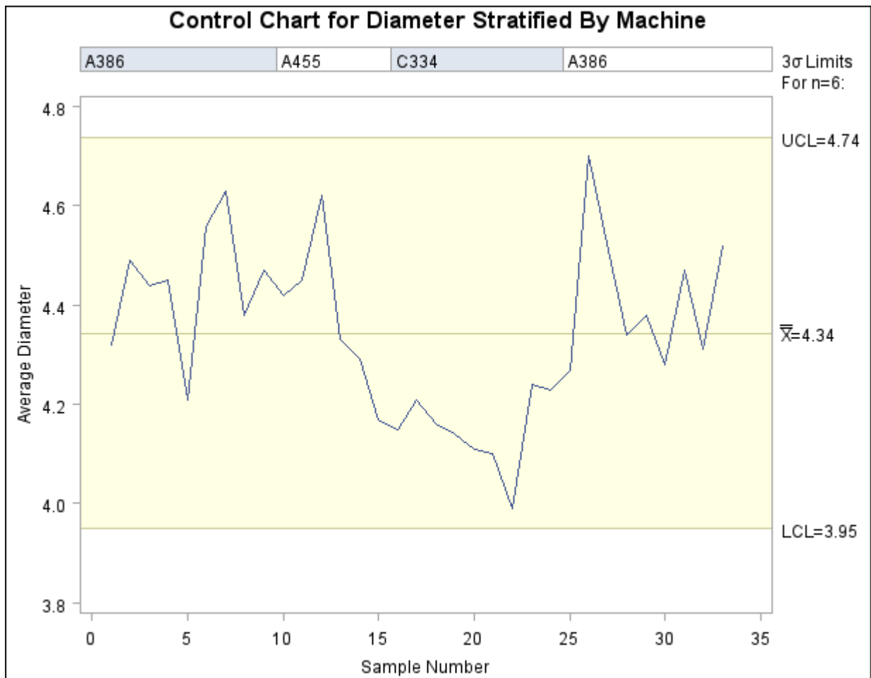
Output 13.43.27 Stratified Control Chart Using a Single Block Variable
