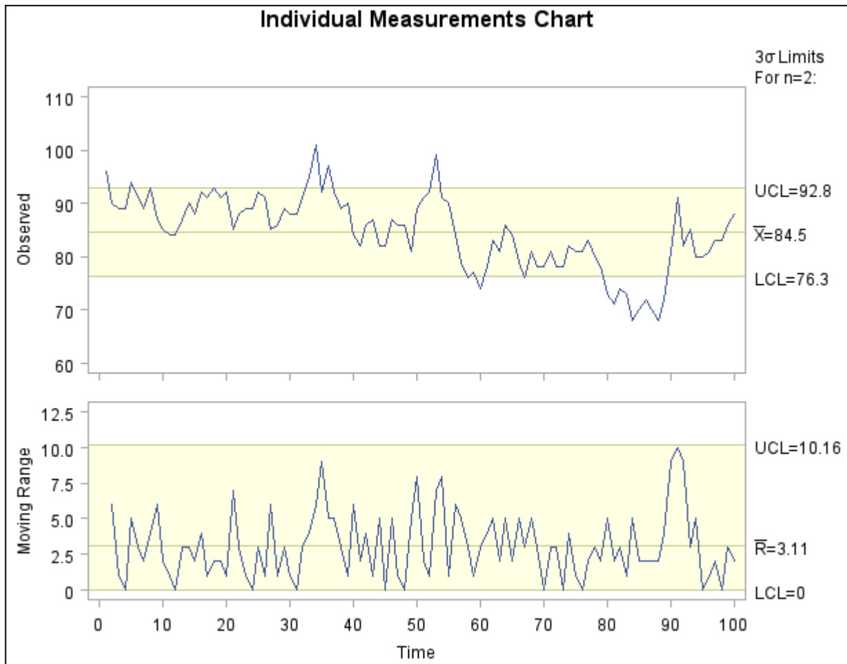
Output 13.43.74 Conventional Shewhart Chart
