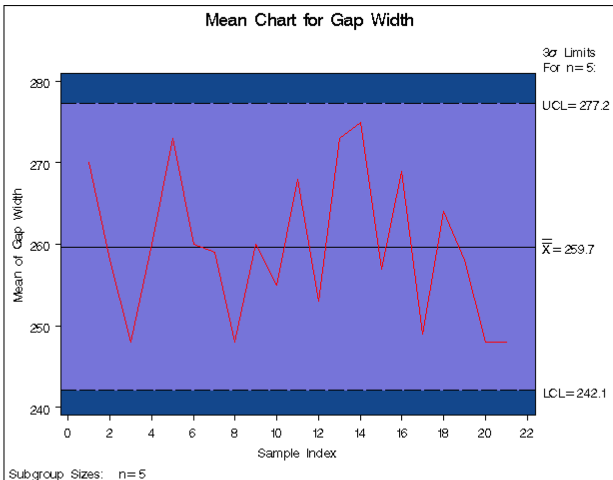
Output 13.33.9 \bar{X} Chart from the Summary Data Set Parts (Traditional Graphics with NOGSTYLE)
