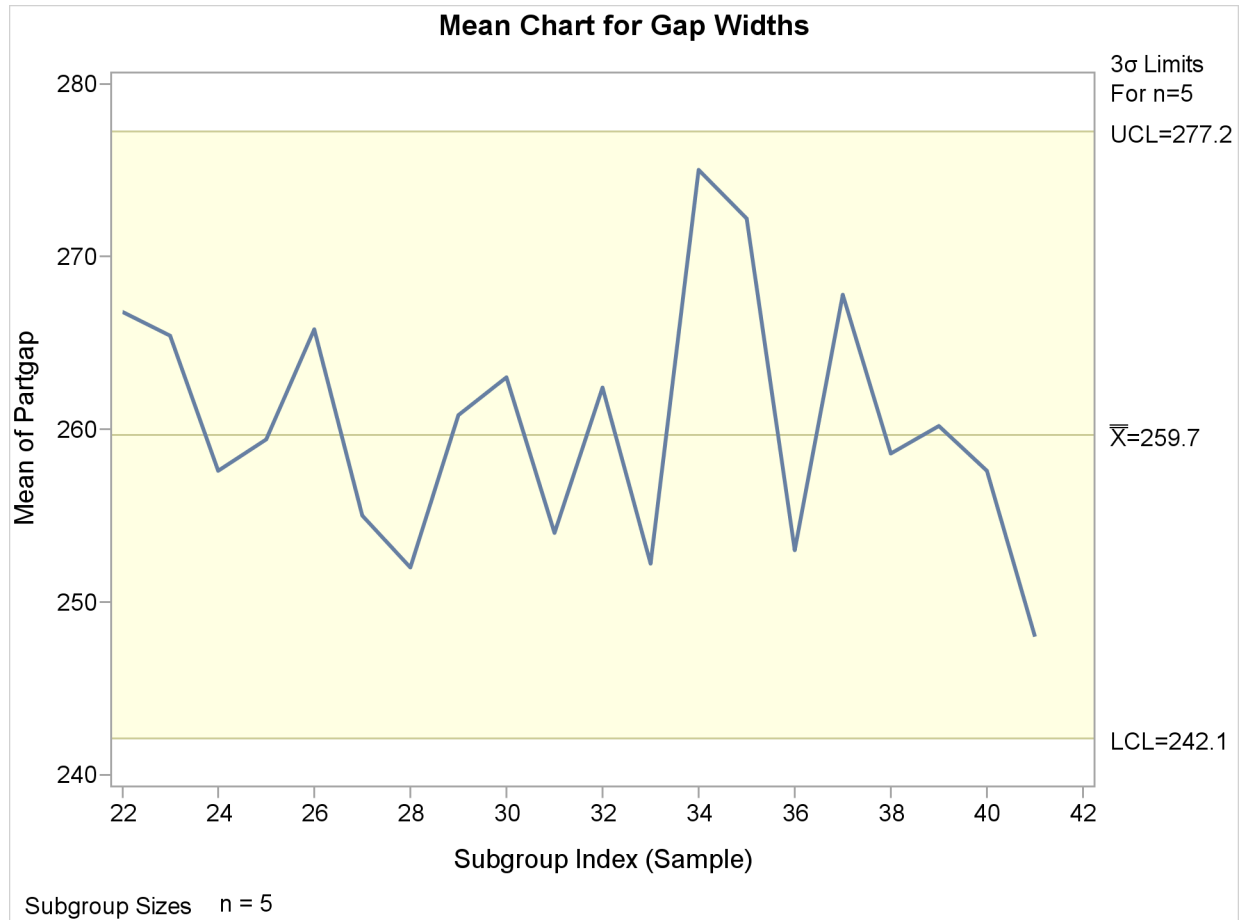
Output 13.33.14 \bar{X} Chart for Second Set of Gap Width Data (ODS Graphics)
