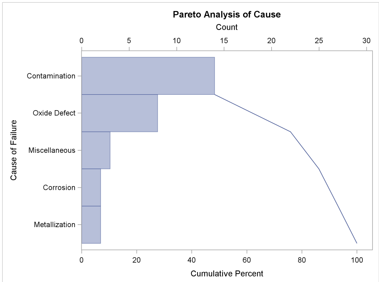
Figure 11.4 Restricted Pareto Chart
