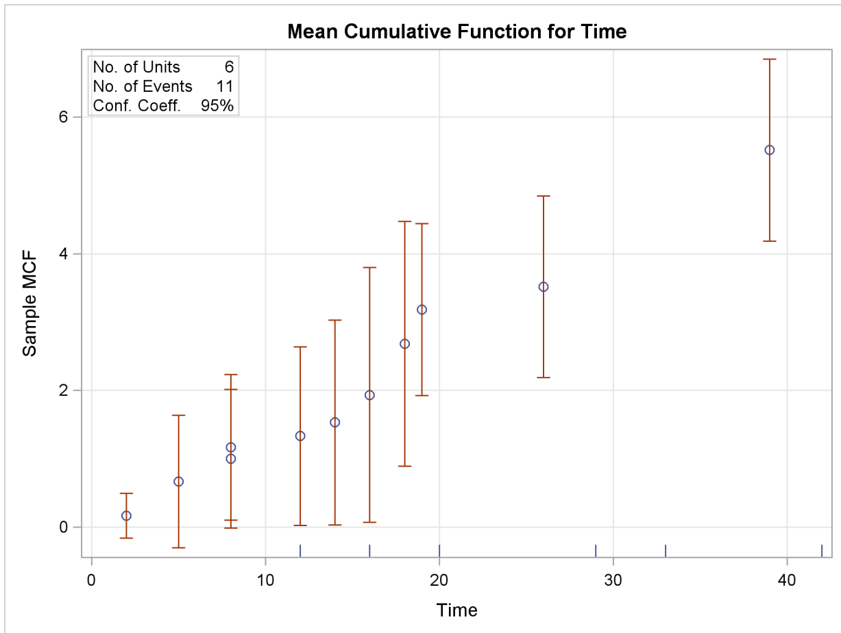
Figure 12.48 MCF Plot for the Artificial Data
