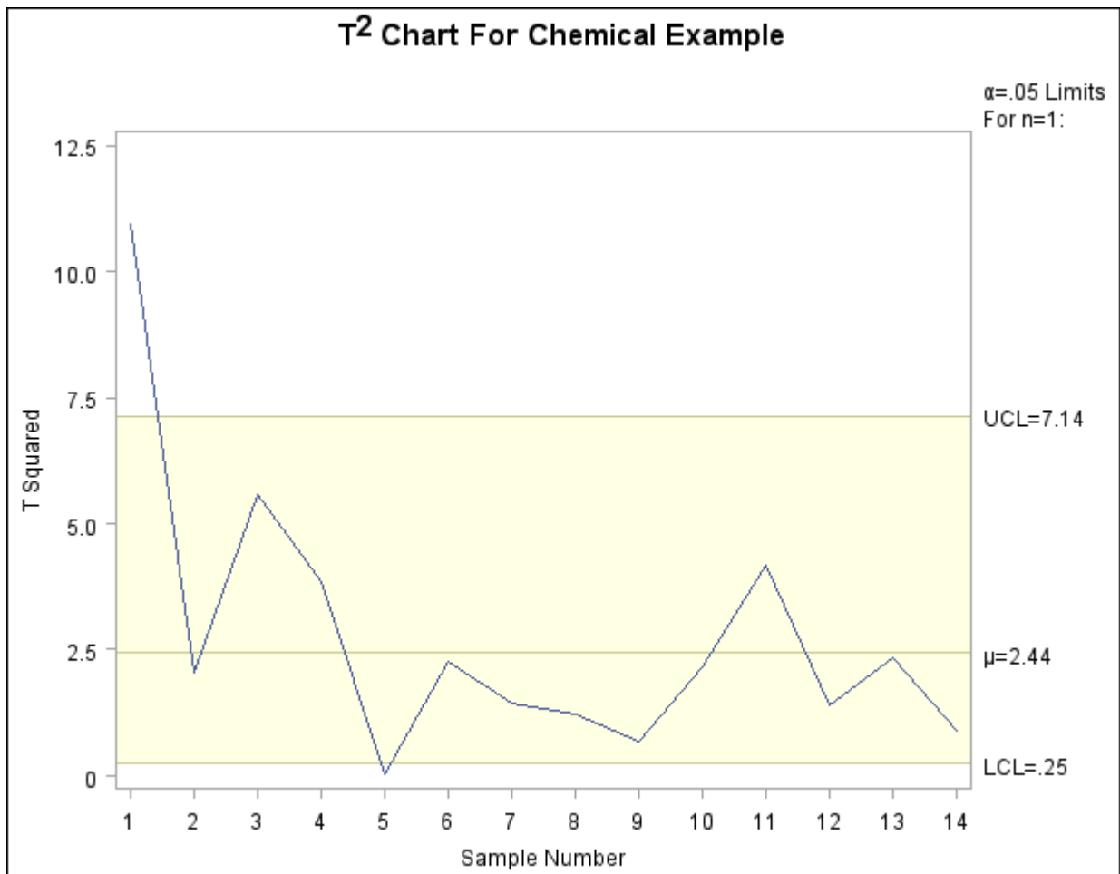
Output 13.43.104 Multivariate Control Chart for Chemical Process
