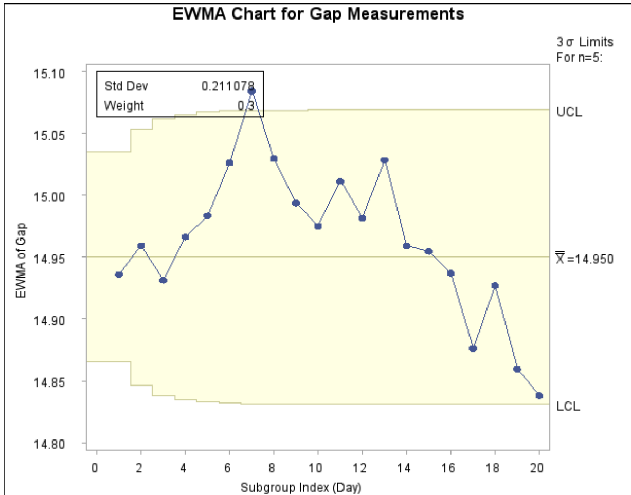
Output 9.7.2 Exponentially Weighted Moving Average Chart with an Inset
