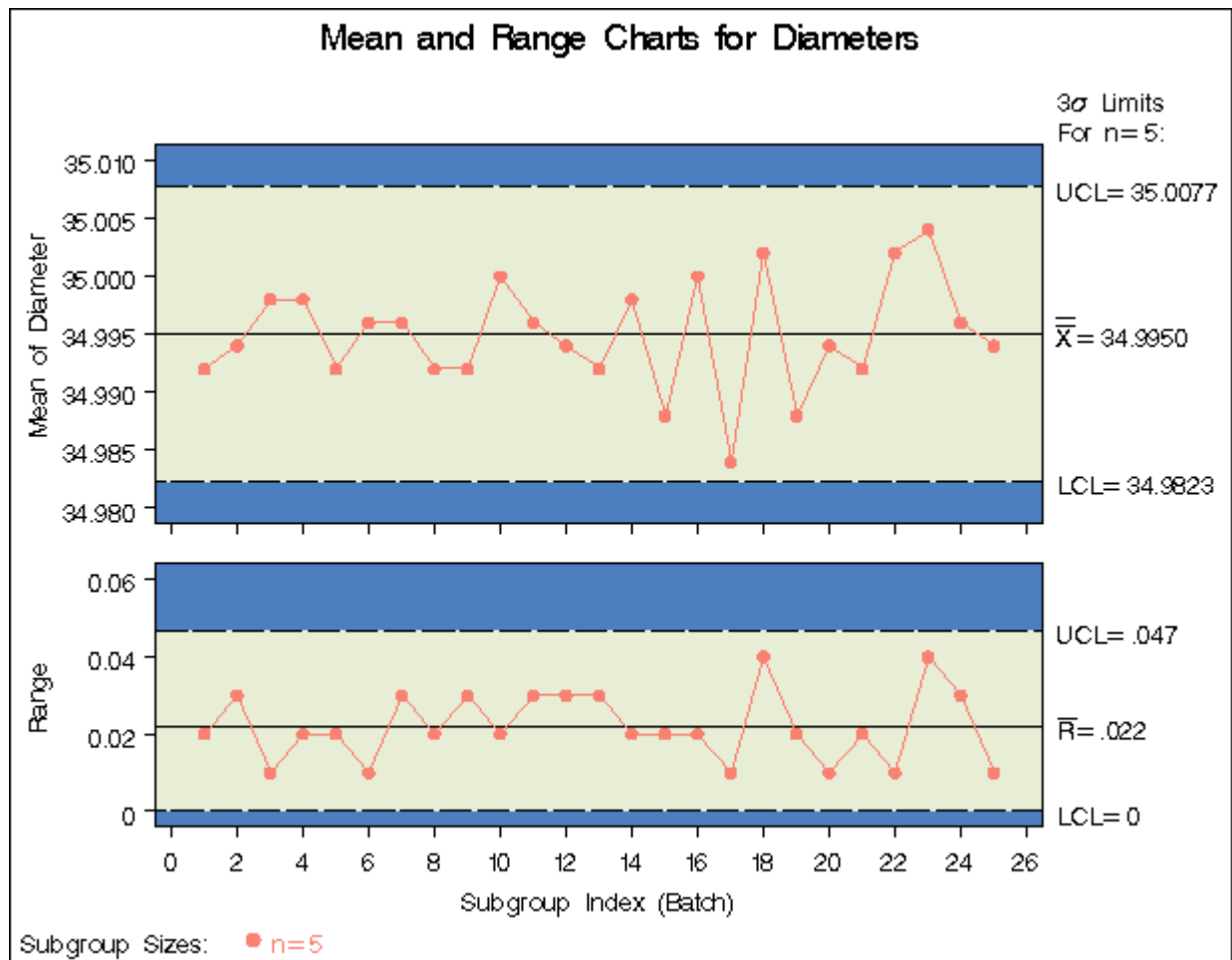
Output 13.37.5 \bar{X} and R Charts from Summary Data (Traditional Graphics with NOGSTYLE)
