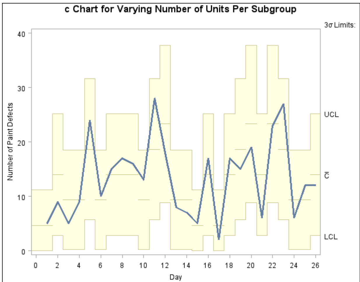
Output 13.10.2 c Chart for Varying Number of Units
