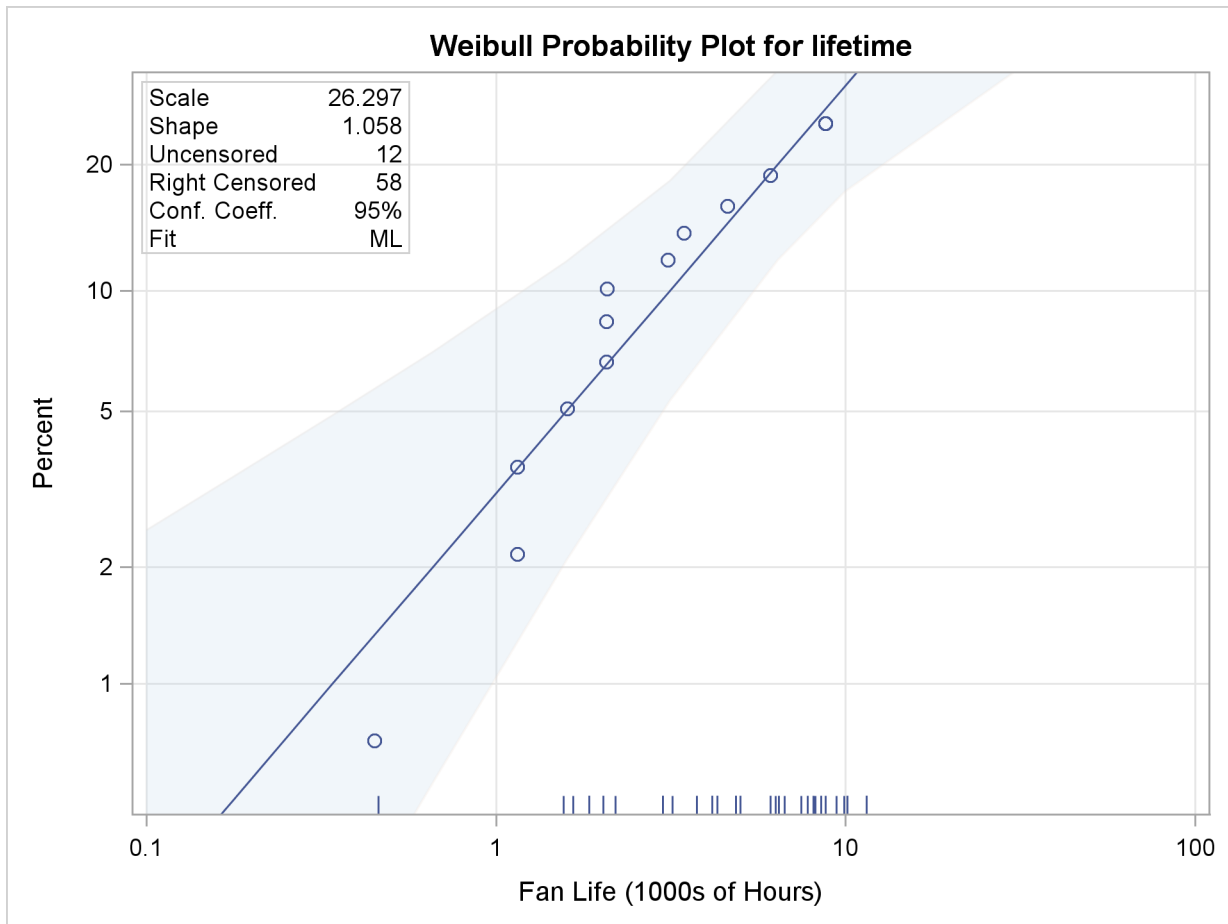
Figure 12.2 Weibull Probability Plot for Engine Fan Data (ODS Graphics)
