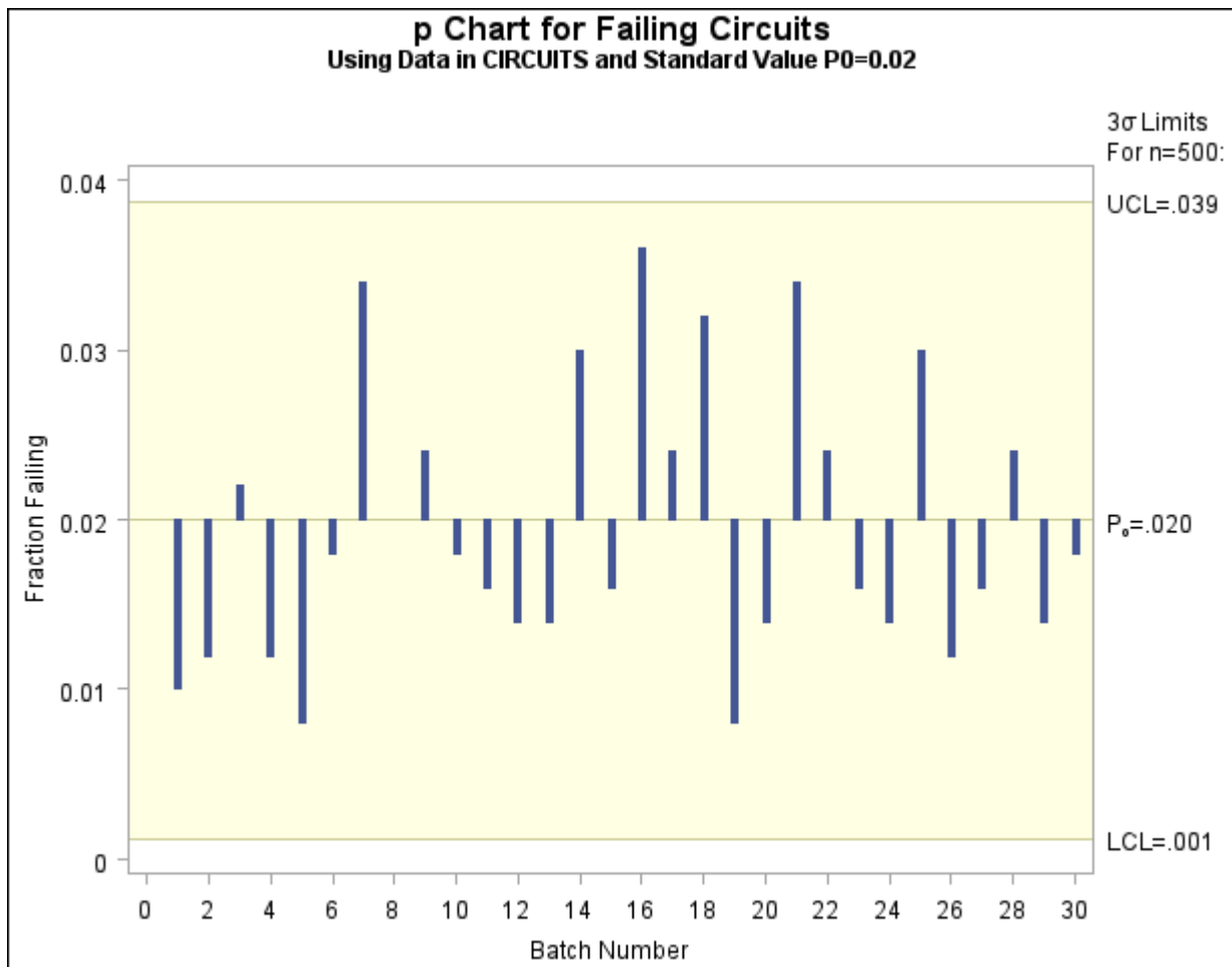
Output 13.23.1 A p Chart with Standard Value p_0
