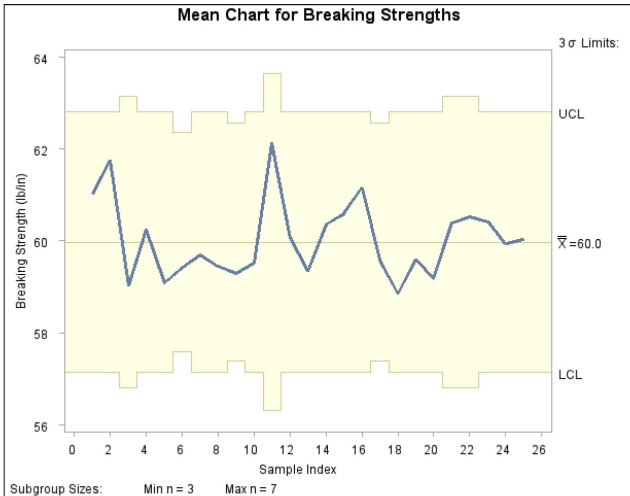
Output 13.35.1 \bar{X} Chart with Varying Subgroup Sample Sizes
