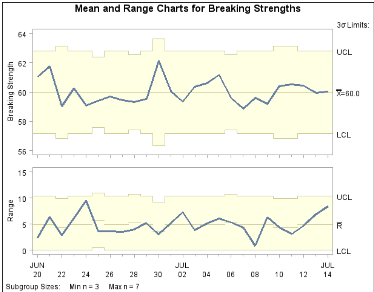
Output 13.40.1 \bar{X} and R Charts with Varying Subgroup Sample Sizes
