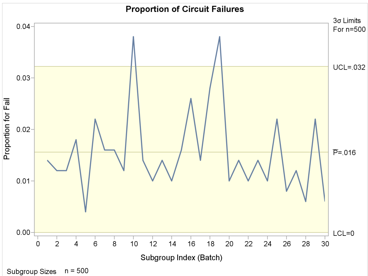
Output 13.25.1 A p Chart for Circuit Failures
