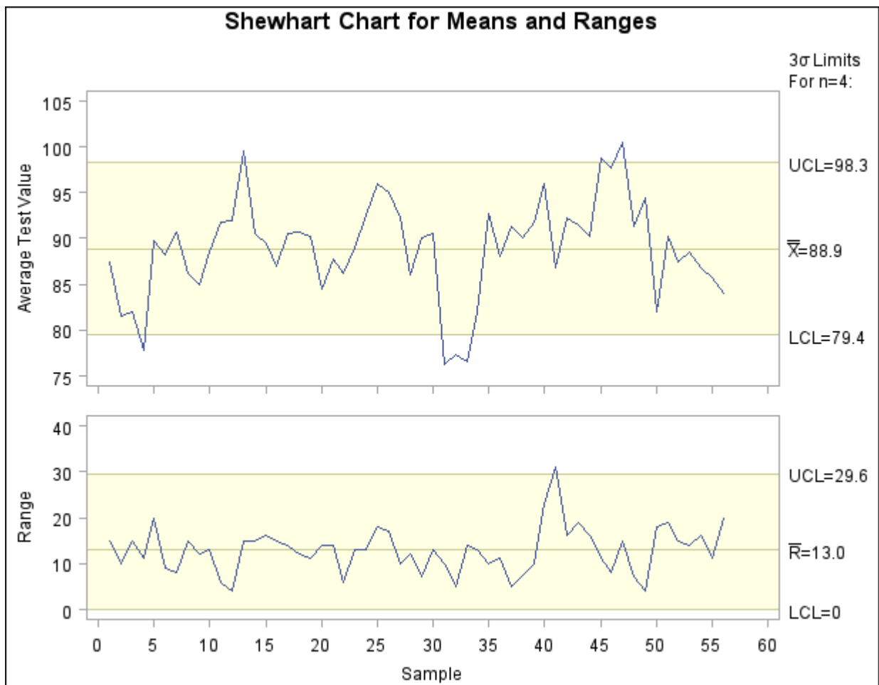
Output 13.43.83 Conventional \bar{X} and R Chart
