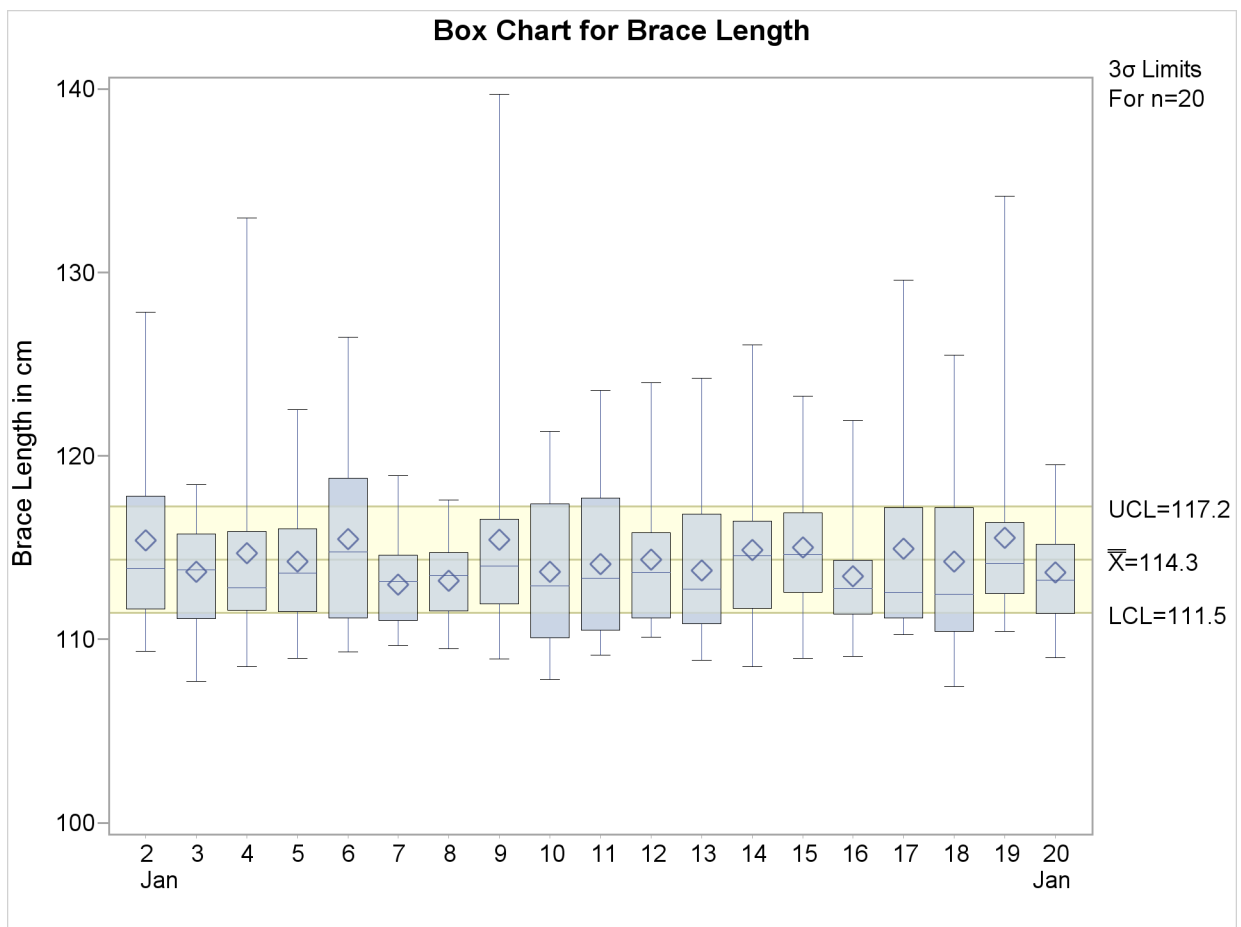
Output 13.43.2 Box Chart
