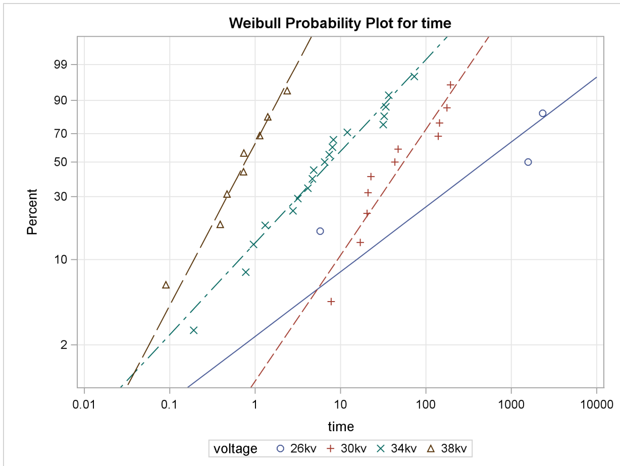
Figure 12.5 Weibull Probability Plot for the Insulating Fluid Data
