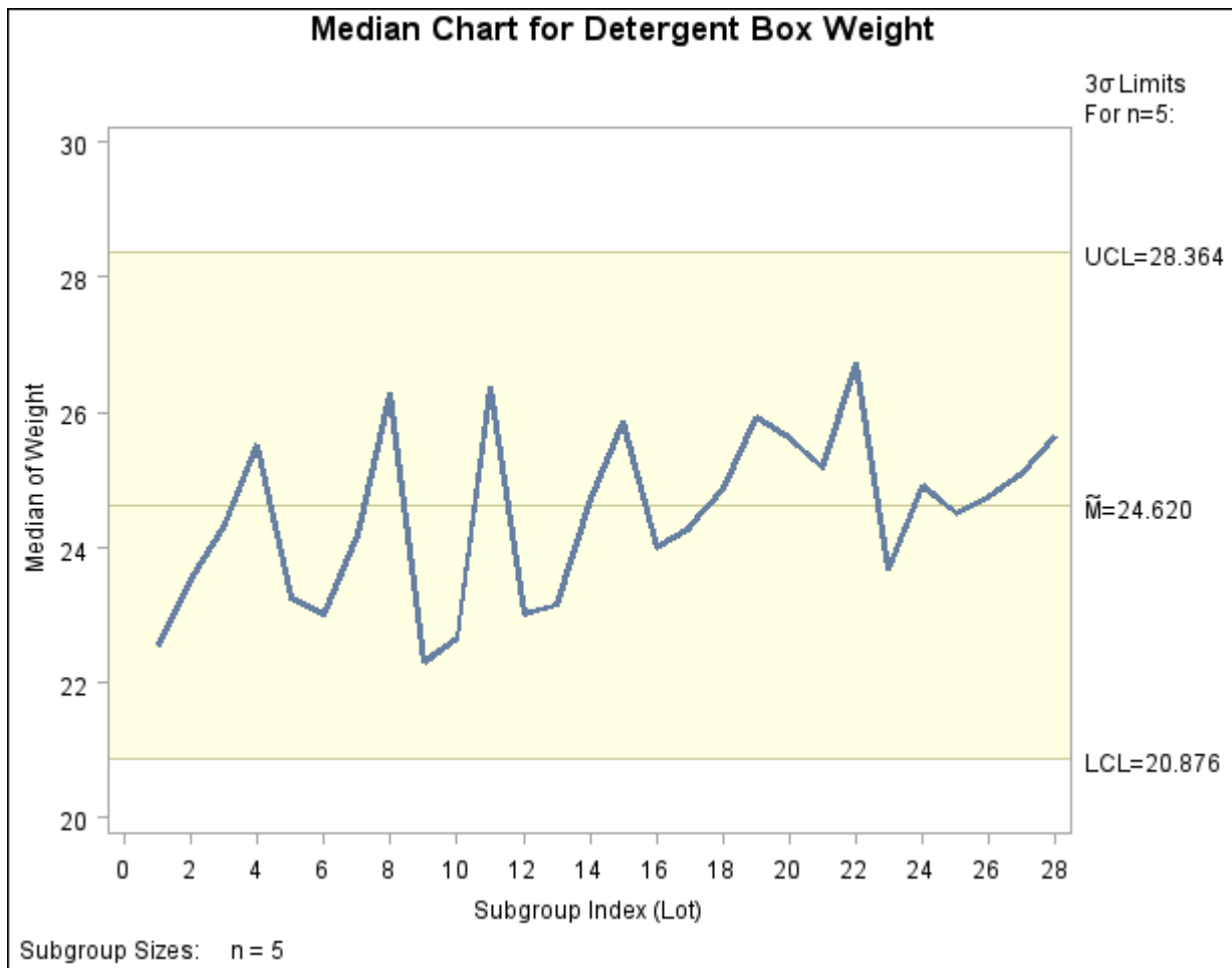
Output 13.14.3 Central Line is Median of Subgroup Medians
