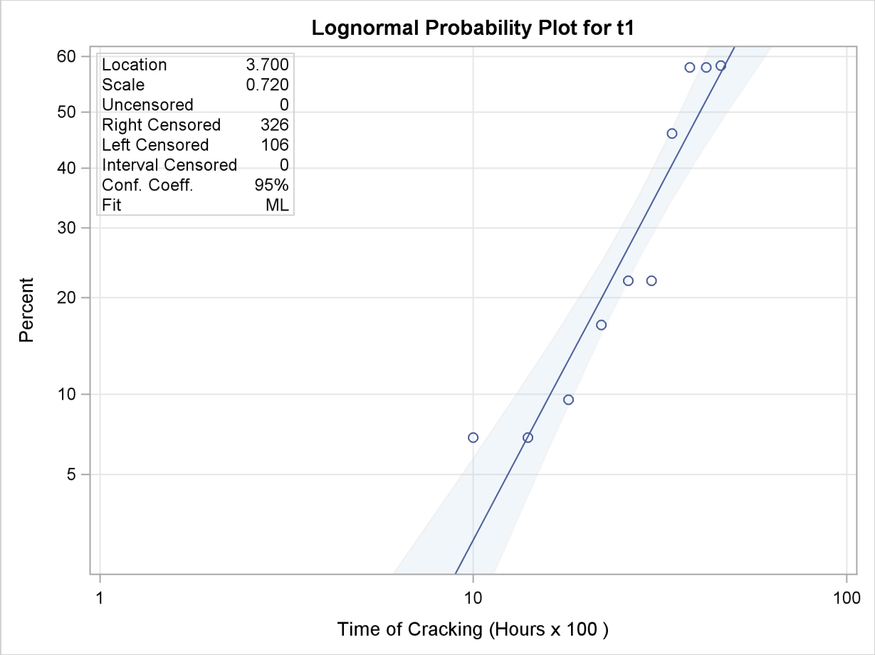
Figure 12.15 Lognormal Probability Plot for the Turbine Wheel Data
