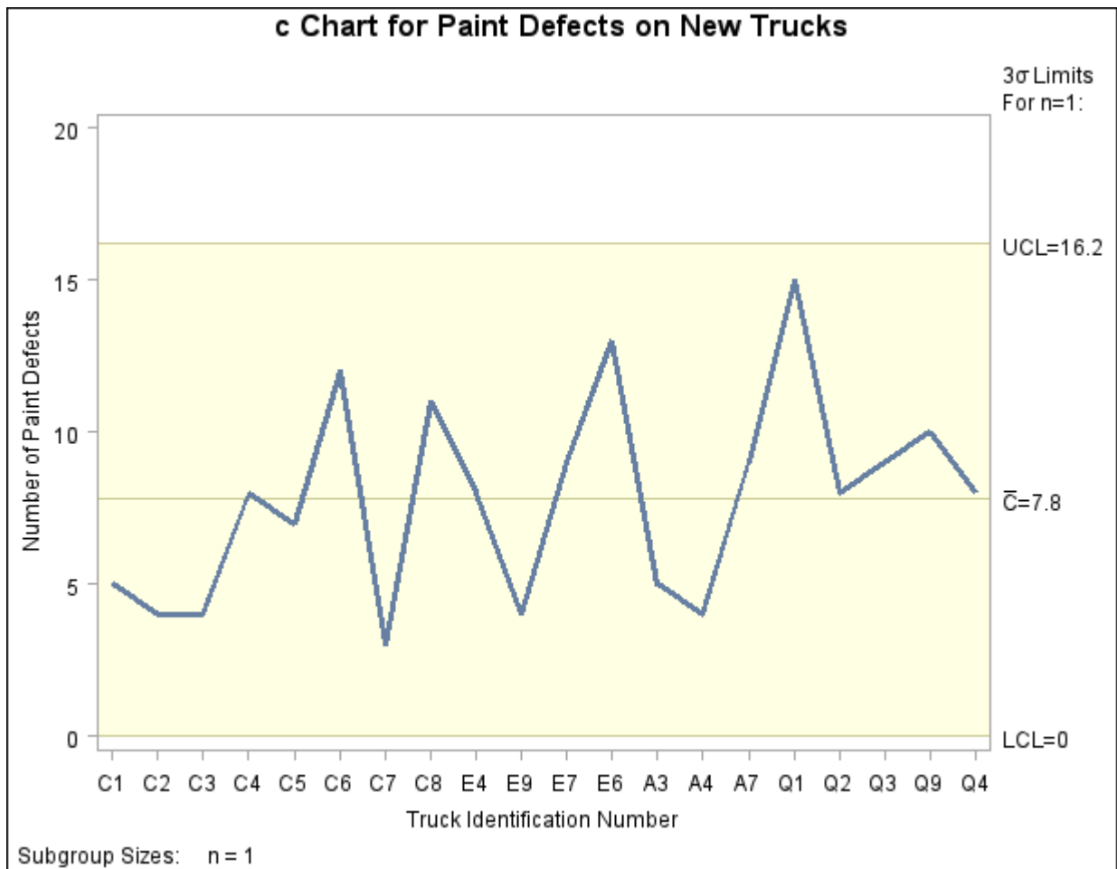
Output 13.7.5 c Chart of Paint Defects (Traditional Graphics)
