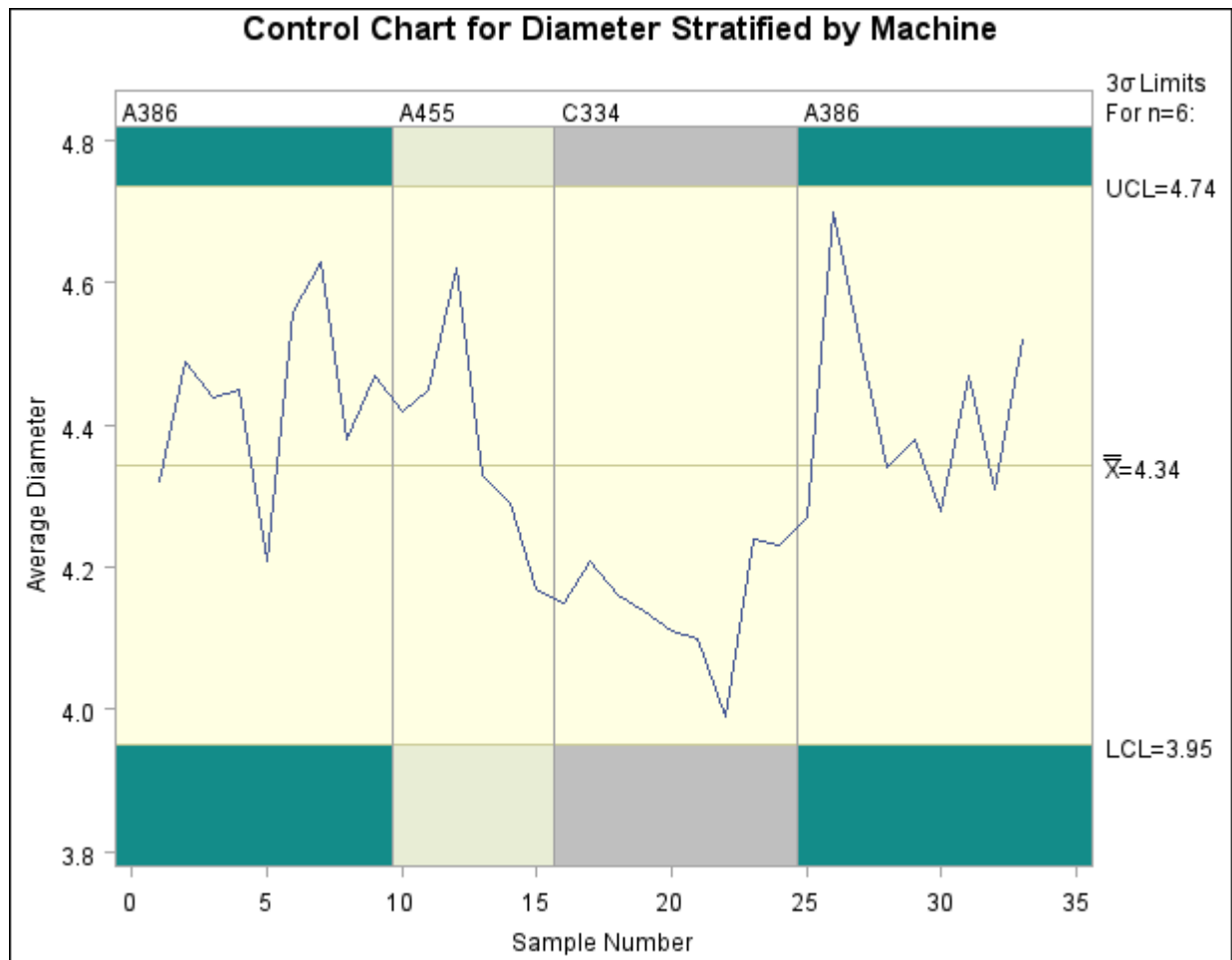
Output 13.43.31 Control Chart Stratified by Phases
