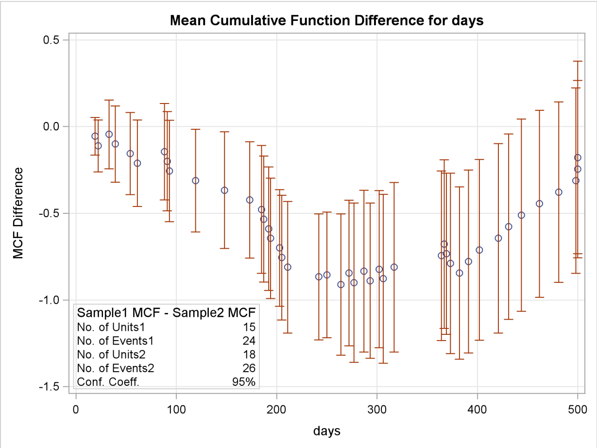
Figure 12.36 Mean Cumulative Function Difference
