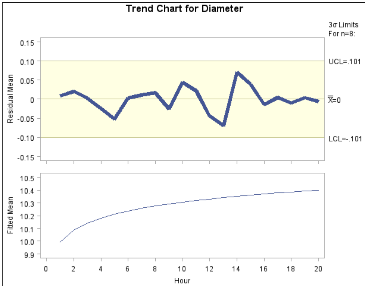
Output 13.43.51 Trend Chart for Diameter Data
