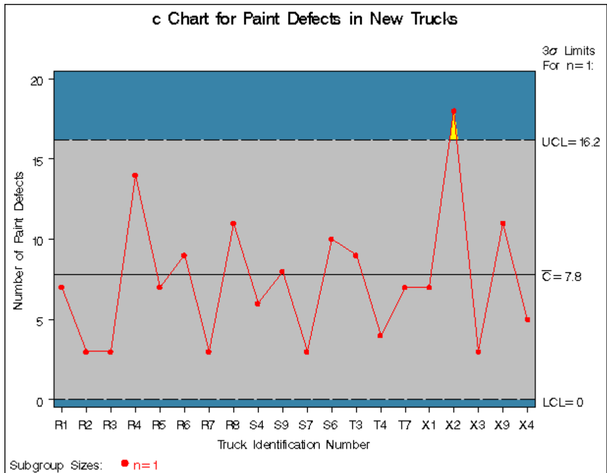
Output 13.7.8 c Chart for Second Set of Trucks (Traditional Graphics with NOGSTYLE)
