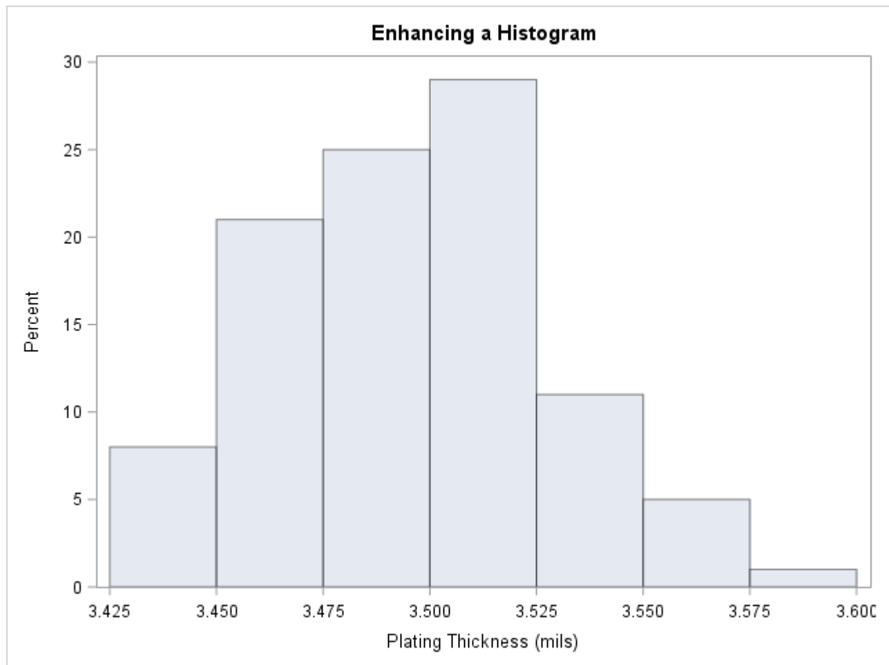
Output 4.18.2 Histogram with ENDPOINTS= Option
