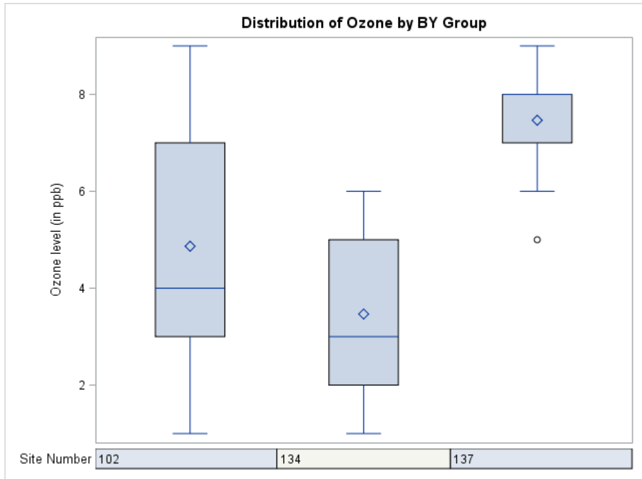
Output 4.5.8 Ozone Side-by-Side Boxplot for All BY Groups
