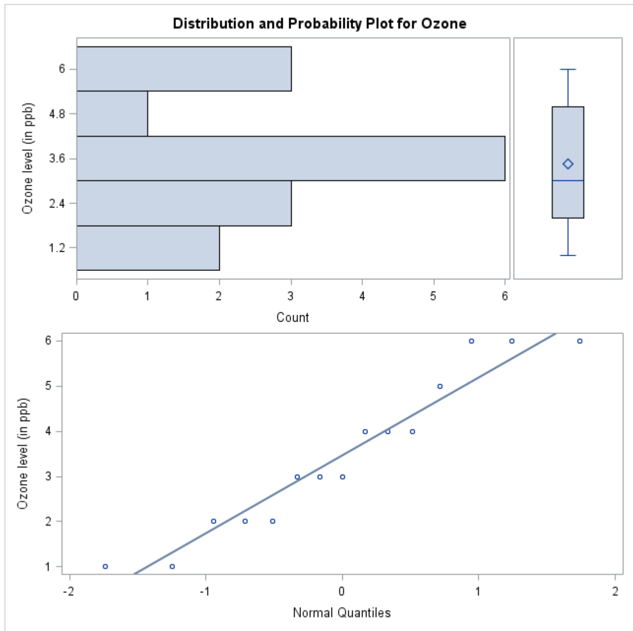
Output 4.5.6 Ozone Plots for BY Group Site = 134
