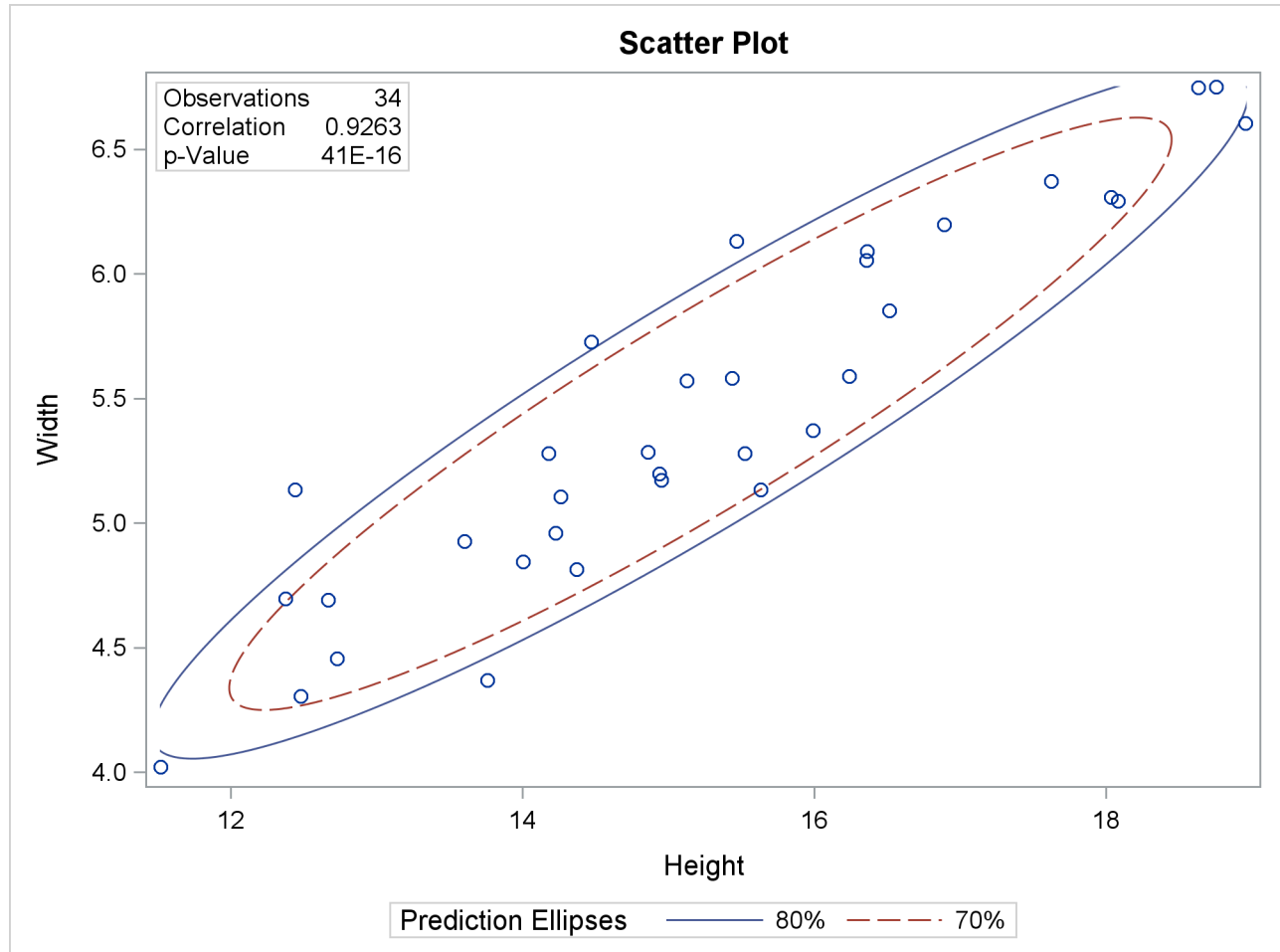
Output 2.8.4 Scatter Plot with Prediction Ellipses
