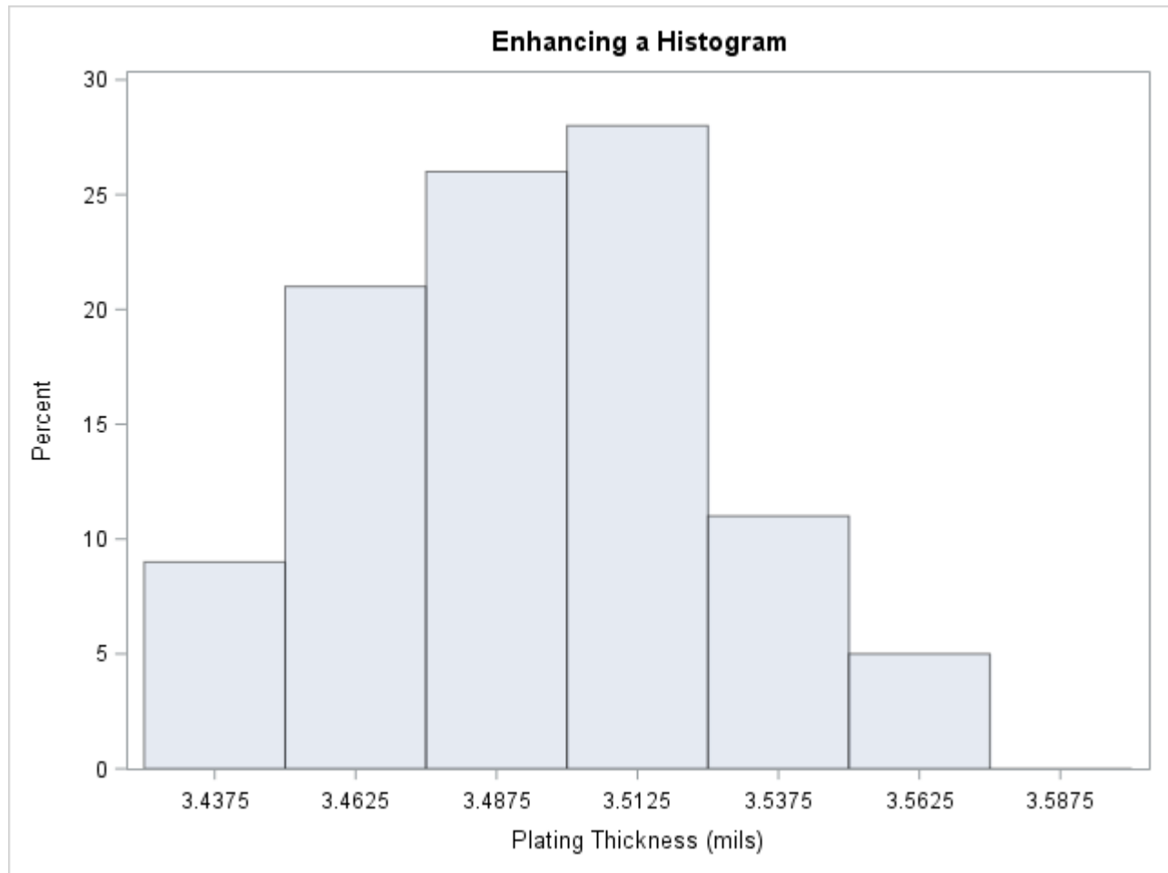
Output 4.18.3 Histogram with MIDPOINTS= and RTINCLUDE Options
