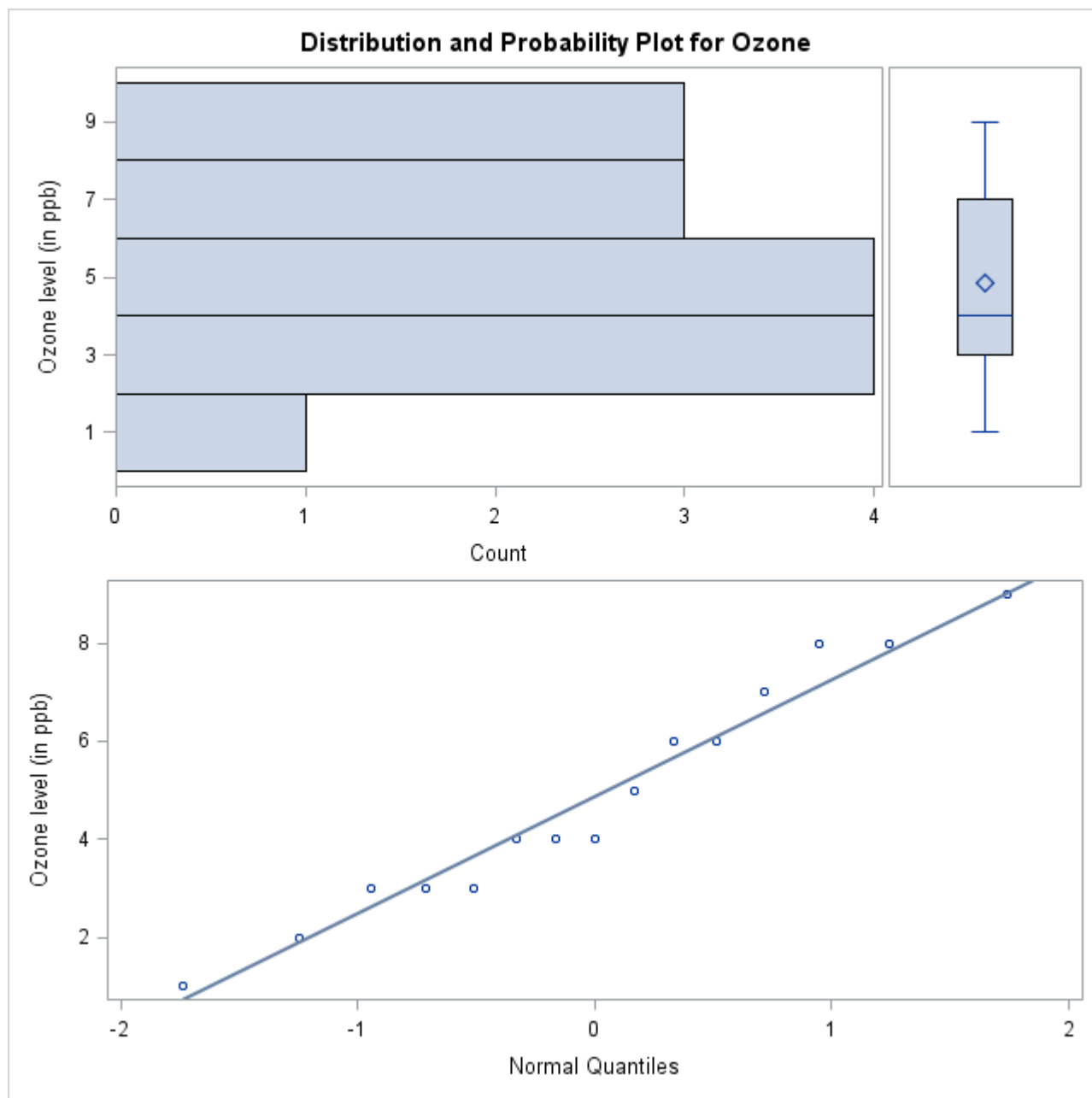
Output 4.5.5 Ozone Plots for BY Group Site = 102
