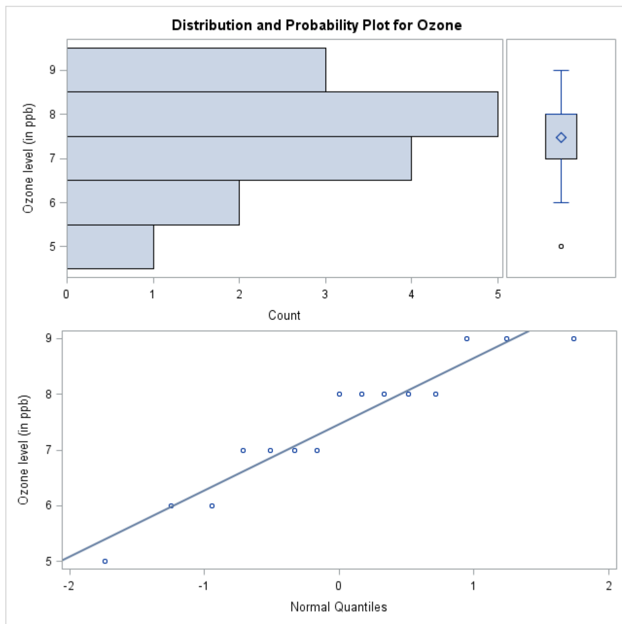
Output 4.5.7 Ozone Plots for BY Group Site = 137
