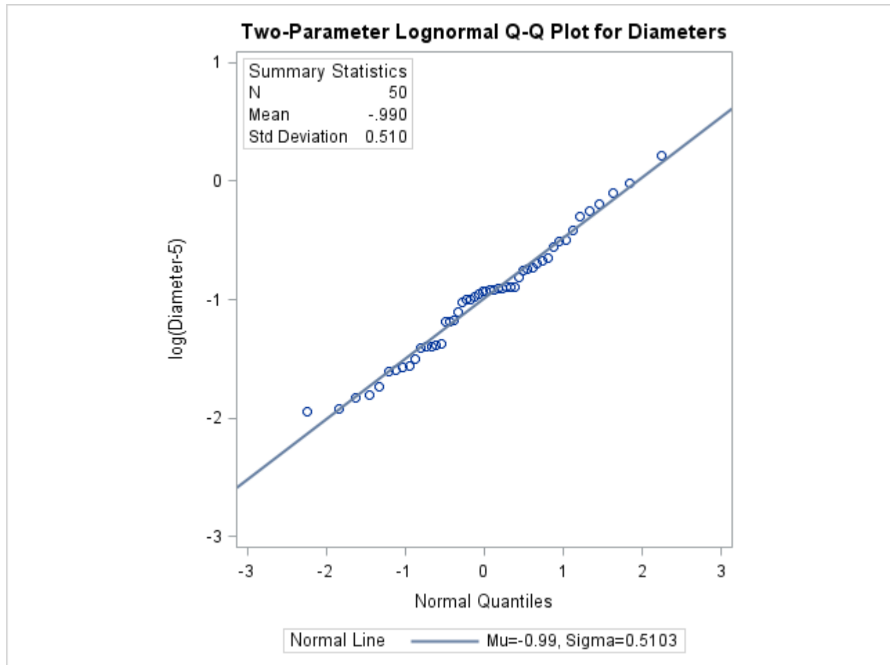
Output 4.33.1 Two-Parameter Lognormal Q-Q Plot for Diameters
