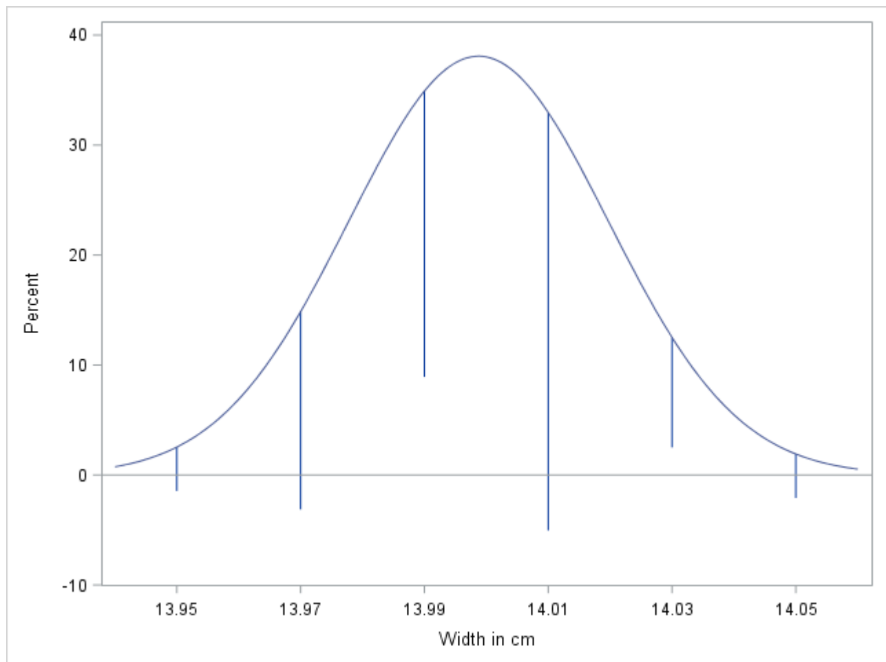
Figure 4.7 Hanging Histogram
