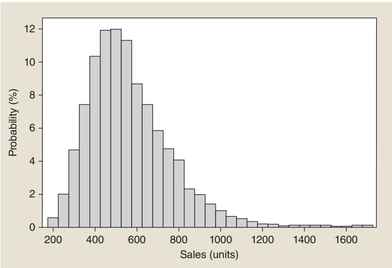
Figure 1.2 A Density Forecast
