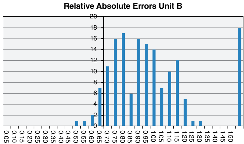
Figure 1.9 The Unavoidability Ratio (Absolute Errors Relative to Those of a Naïve Forecast) for Unit B
