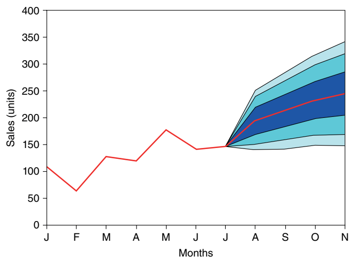
Figure 1.1 A Fan Chart
