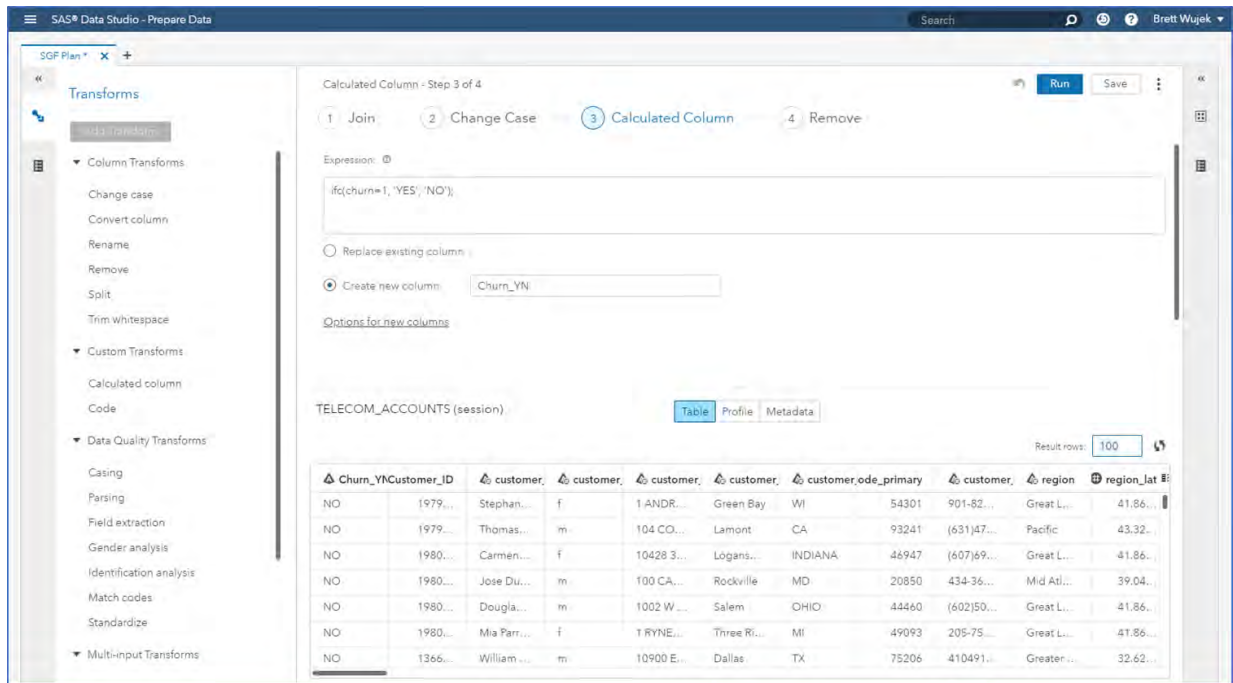
Figure 29. Create Calculated Columns by Using Custom SAS Programming Functions
