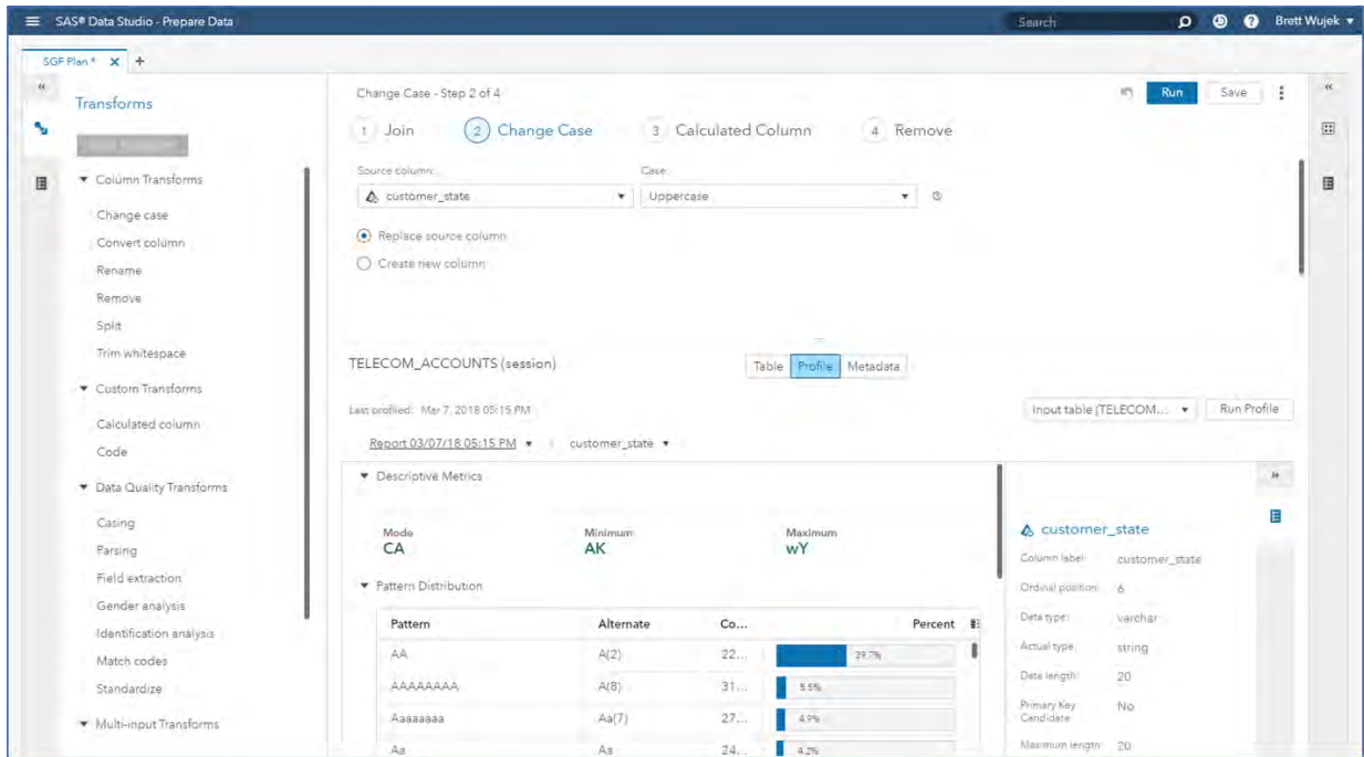
Figure 28. Generate Variable Profiles and Identify and Fix Data Quality Issues
