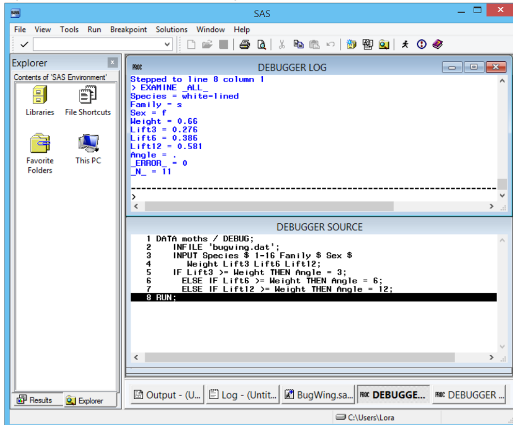
Figure 4 DEBUGGER LOG window showing data values.
