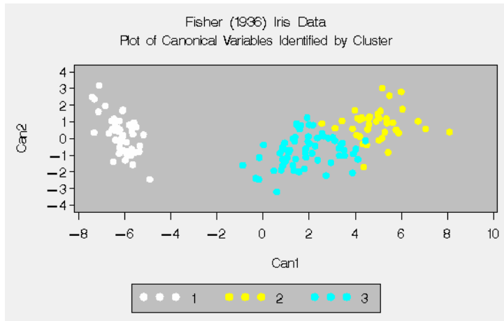
Figure 1: Cluster Analysis of Anderson Iris Data
