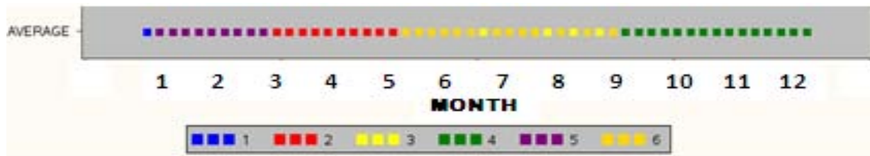
Figure 4: Averaged Seasonal Cluster Analysis of US Gasoline Prices, 1991-2010
