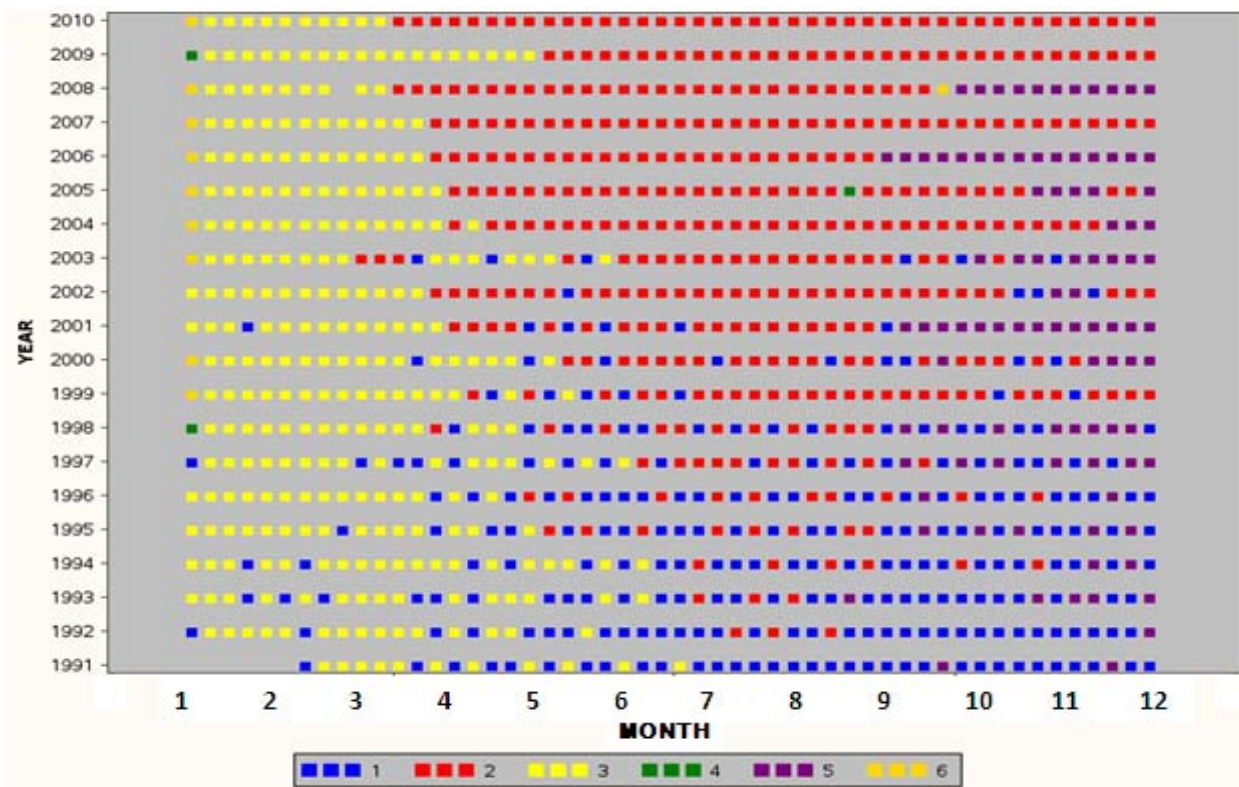
Figure 3: Seasonal Cluster Analysis of US Gasoline Prices, 1991-2010
