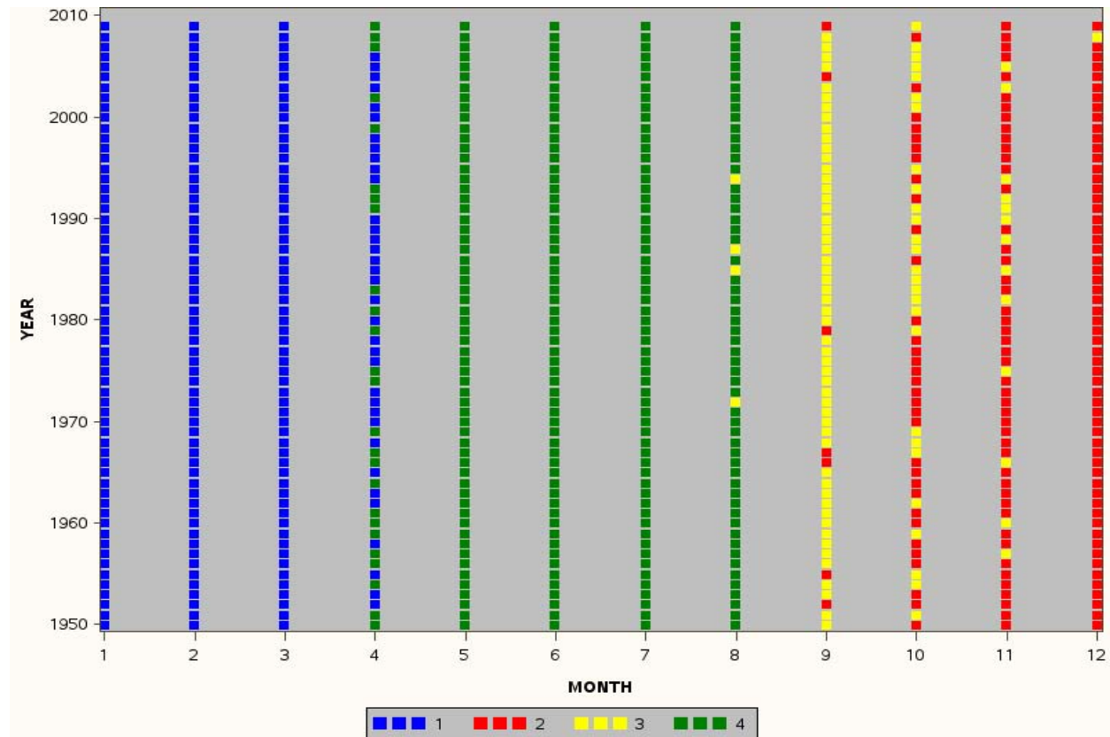
Figure 2: Seasonal Variation in Precipitation in the State of Michigan, 1950-2009 (NOAA Data)
