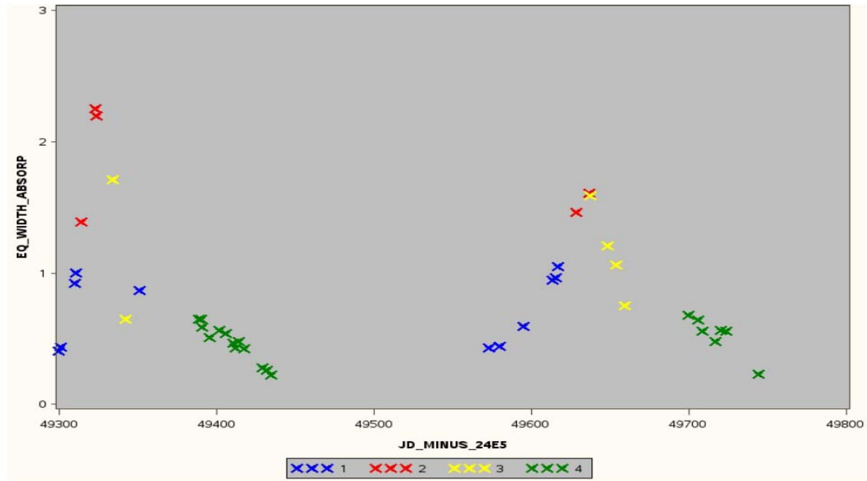
Figure 6: Evolutionary Stages in High Velocity Absorption Events in the A0 Supergiant Star HR 1040
