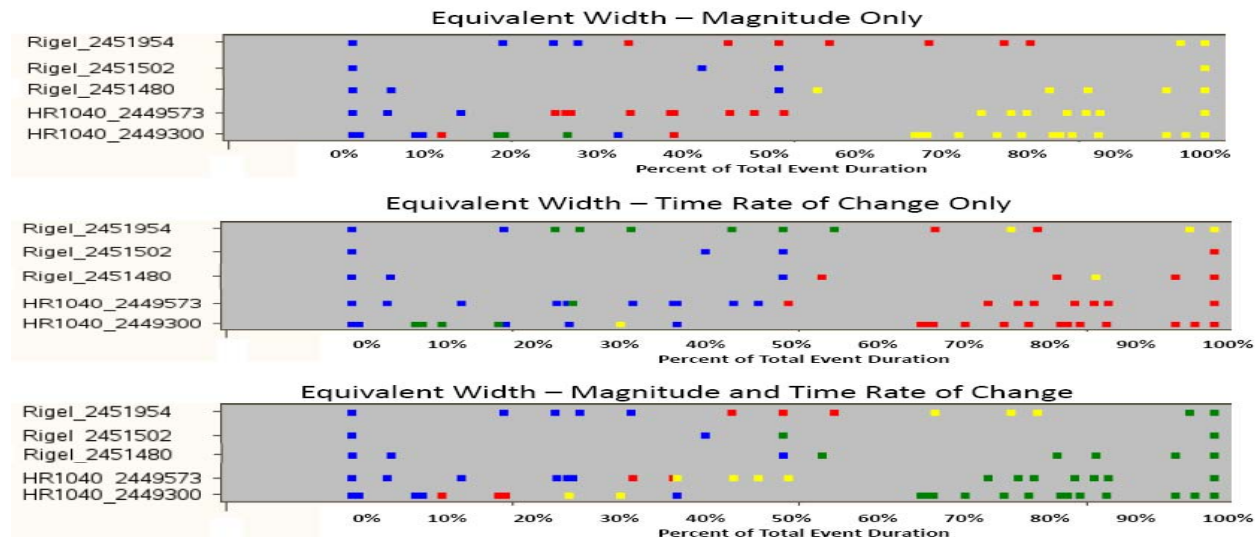
Figure 5: Comparison of Magnitude vs. Time Rate of Change Variables in Cluster Analysis
