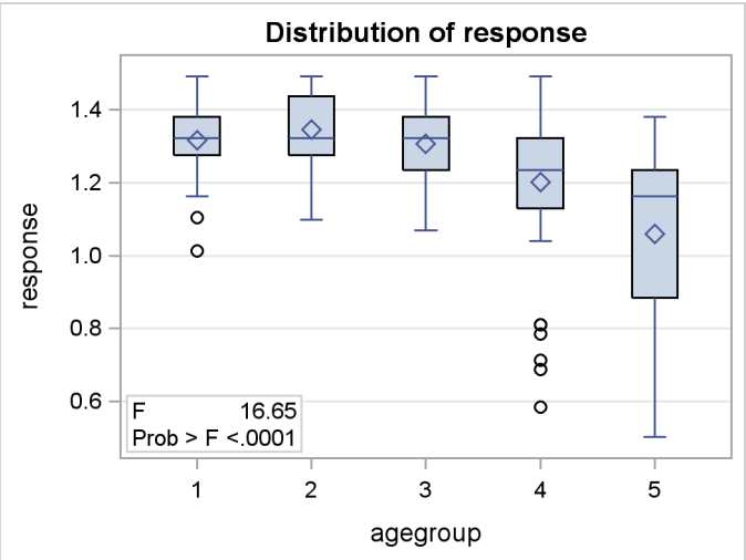
Figure 5 GLM Procedure
