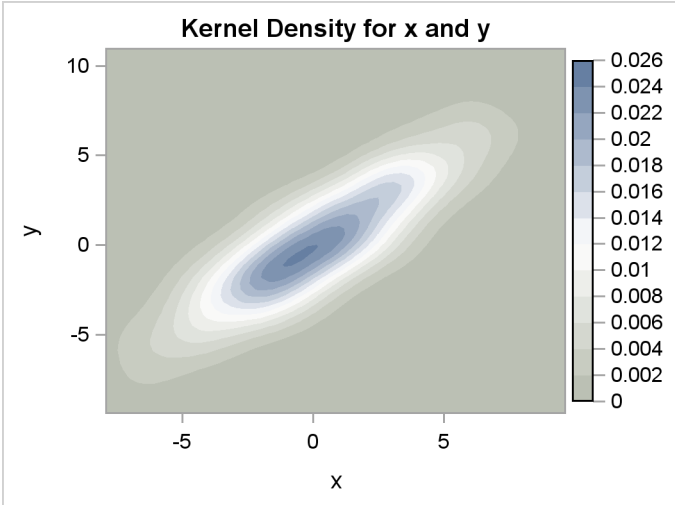
Figure 6 KDE Procedure
