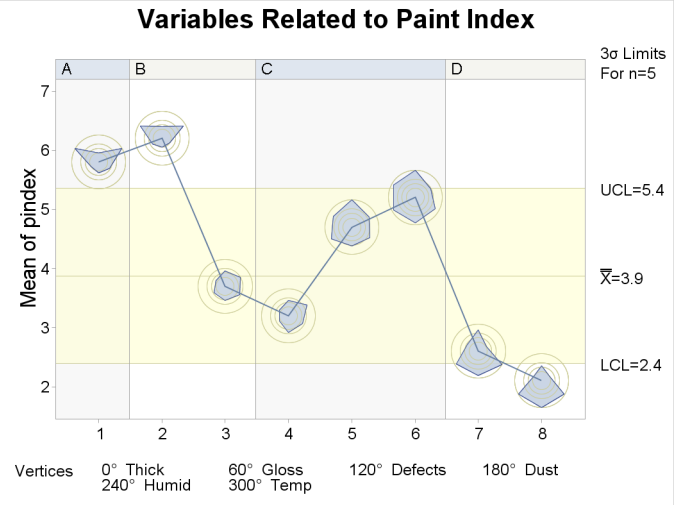
Figure 9 SHEWHART Procedure
