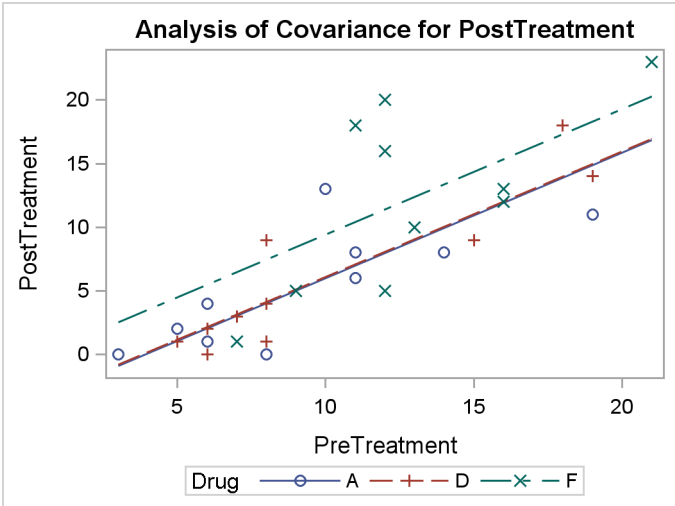
Figure 4 GLM Procedure
