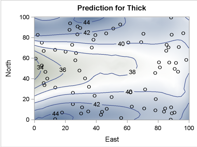
Figure 8 KRIGE2D Procedure
