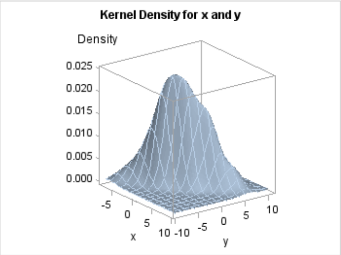
Figure 7 KDE Procedure
