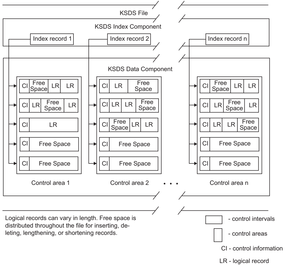
Figure 1.3 KSDS Control Intervals and Control Areas
