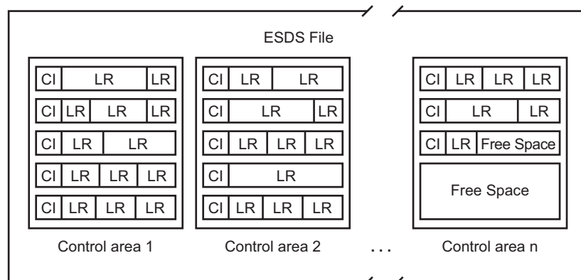
Figure 1.2 ESDS Control Intervals and Control Areas
