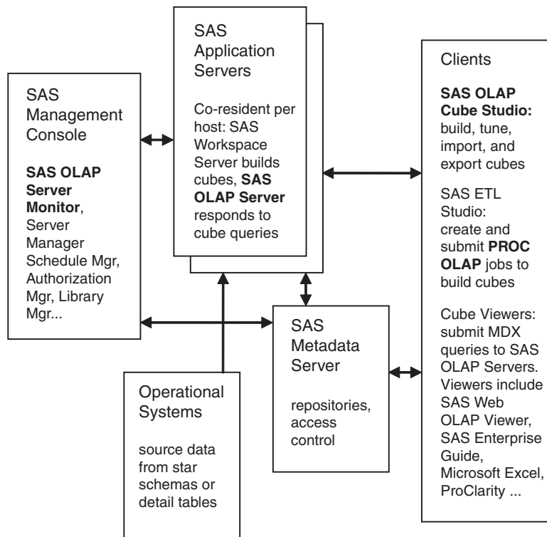
Figure 1.1 SAS OLAP Server Components and Connections
