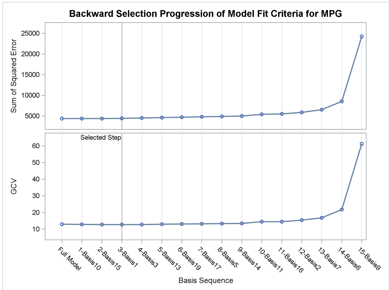
Figure 25.5 Selection Plot
