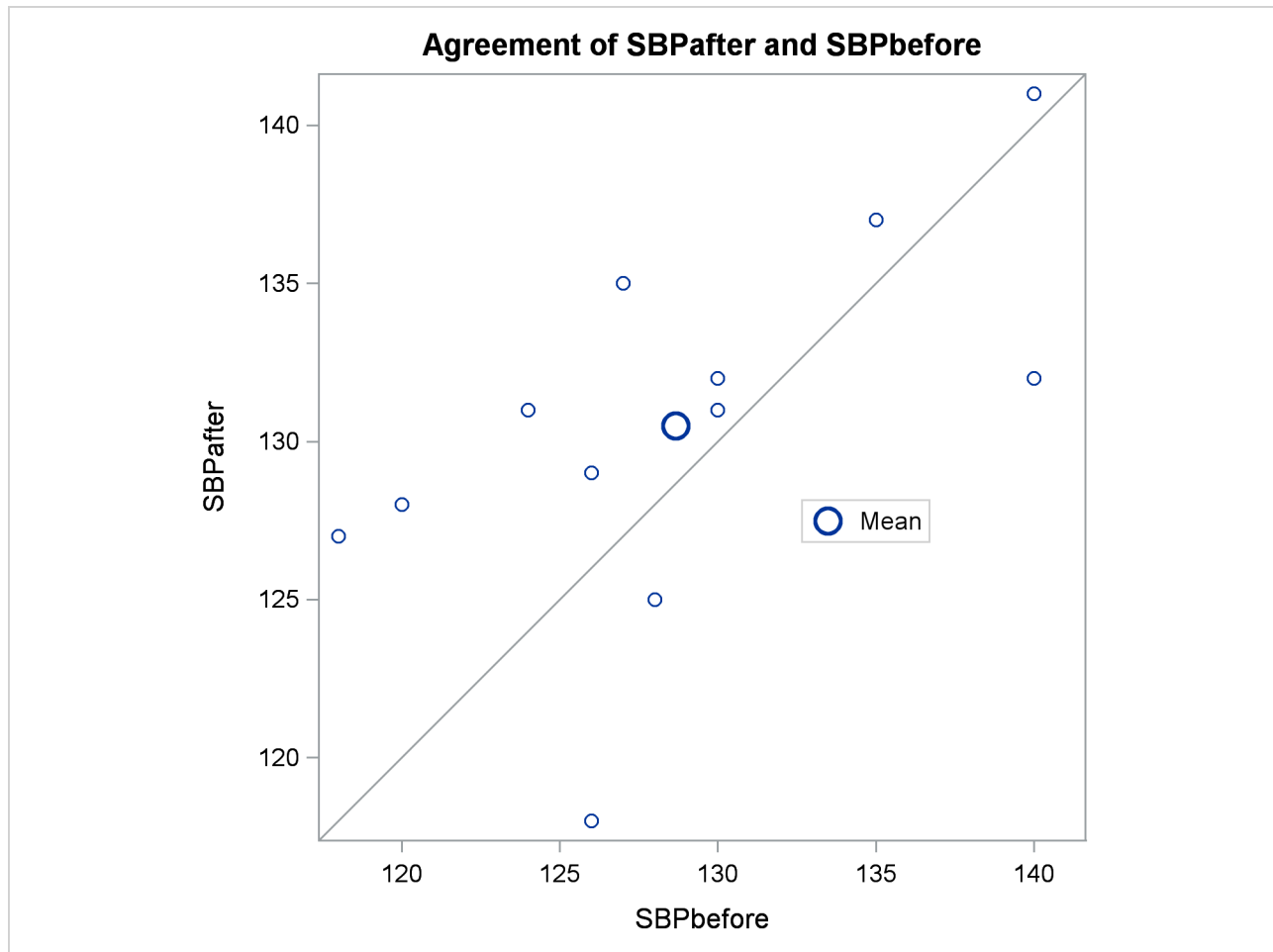
Output 119.3.3 Agreement of Treatments
