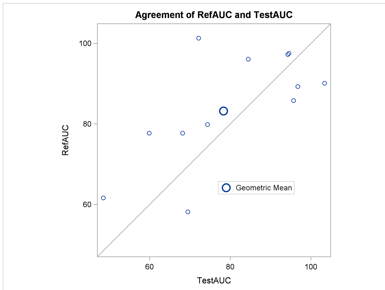
Output 119.5.7 Agreement Plot
