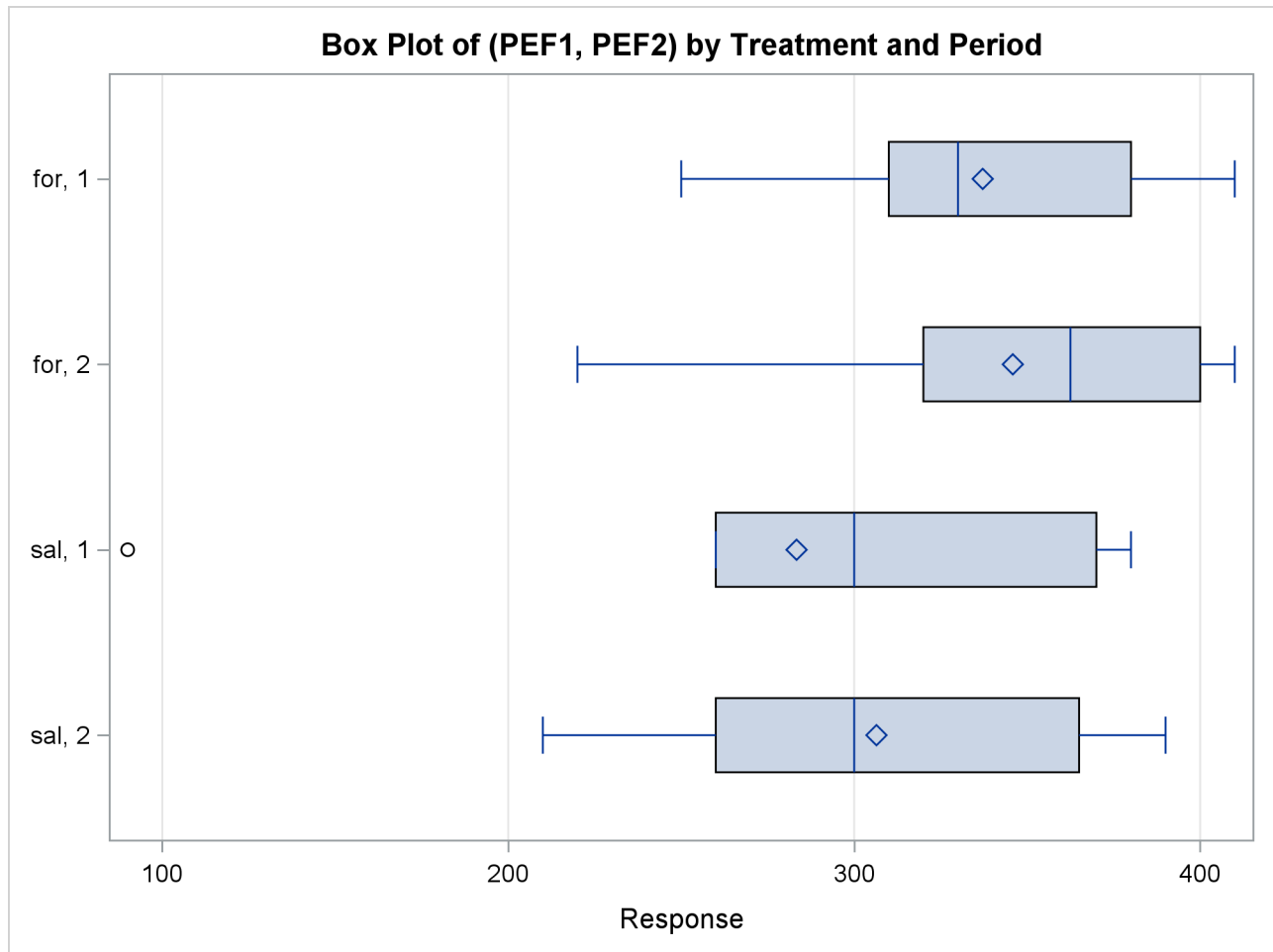
Output 119.4.8 Comparative Box Plots
