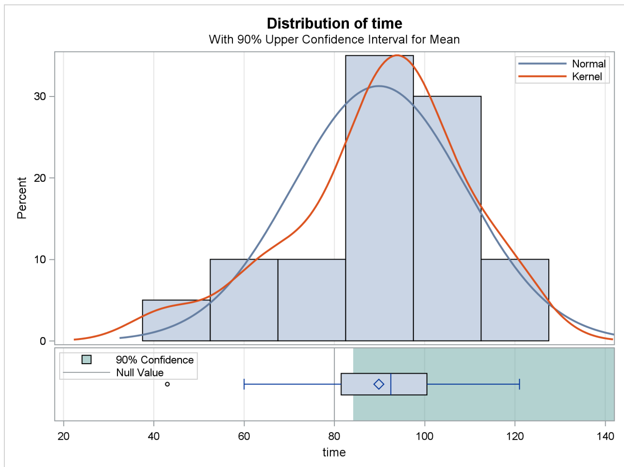
Figure 119.2 Summary Panel
