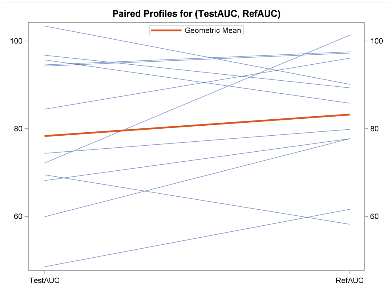
Output 119.5.8 Profiles Plot
