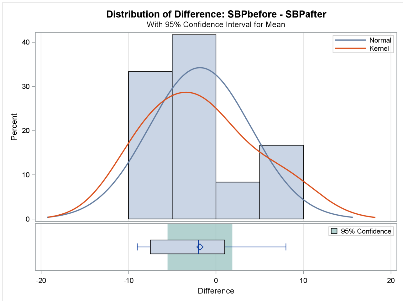
Output 119.3.2 Summary Panel
