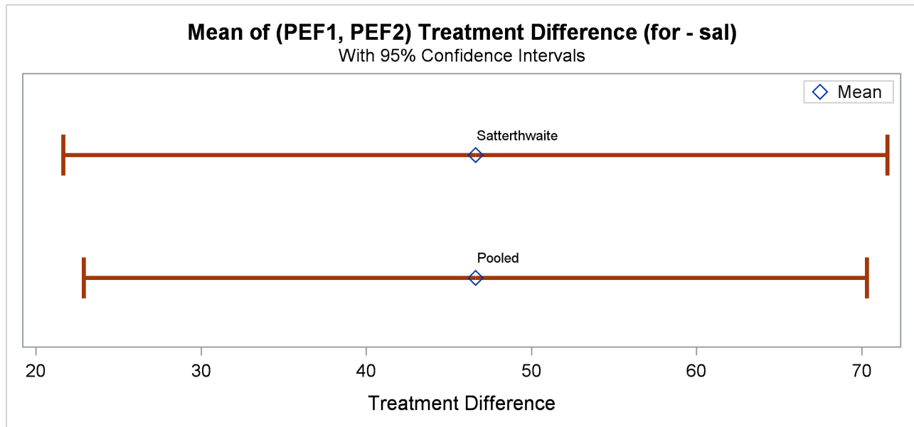
Output 119.4.12 Confidence Intervals for Treatment Difference
