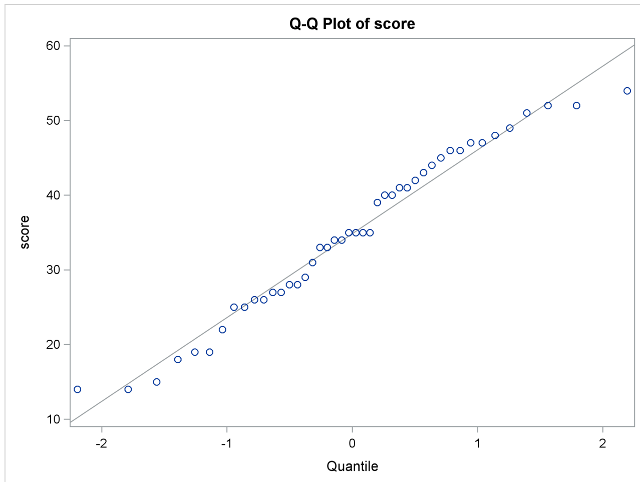
Output 119.2.3 Q-Q Plot
