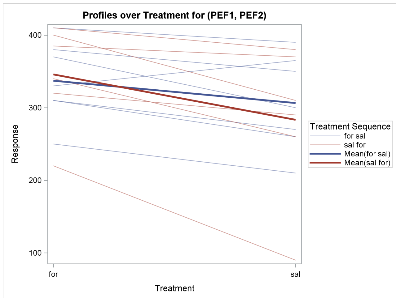
Output 119.4.10 Profiles over Treatment
