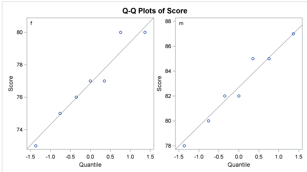
Figure 119.9 Q-Q Plot
