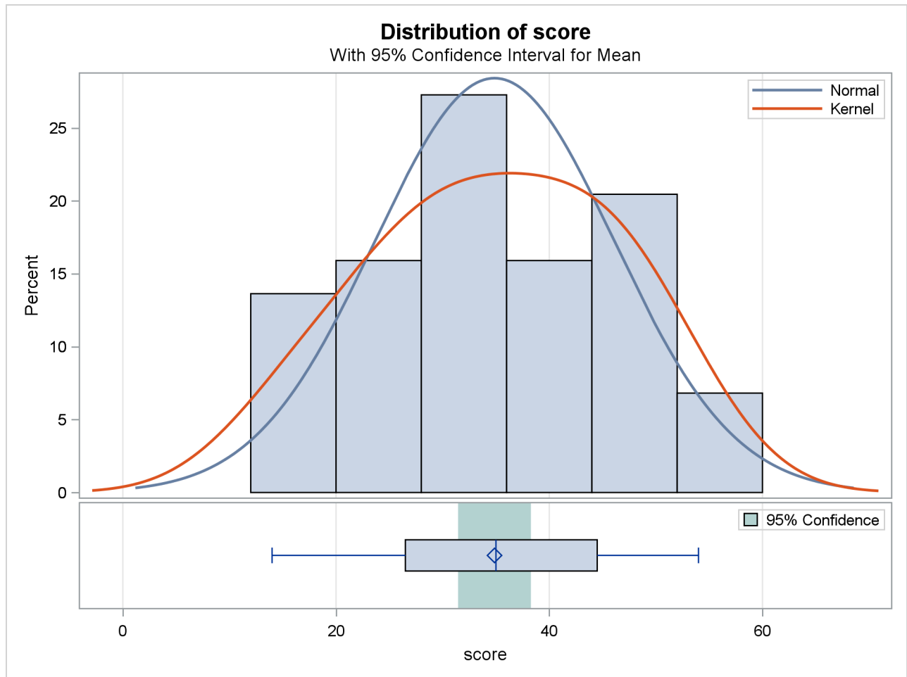
Output 119.2.2 Summary Panel
