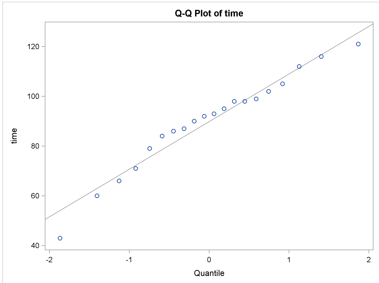
Figure 119.3 Q-Q Plot
