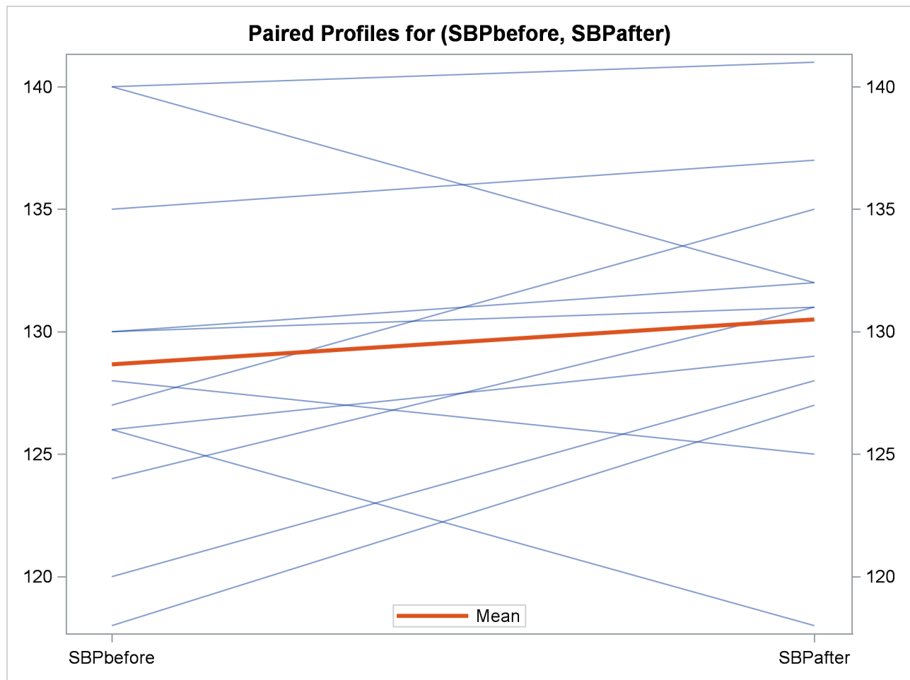
Output 119.3.4 Profiles over Treatments
