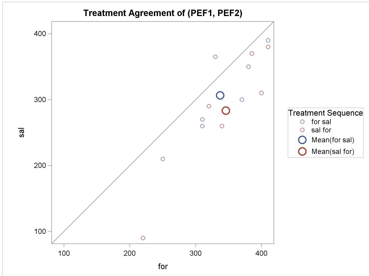
Output 119.4.9 Agreement of Treatments Plot
