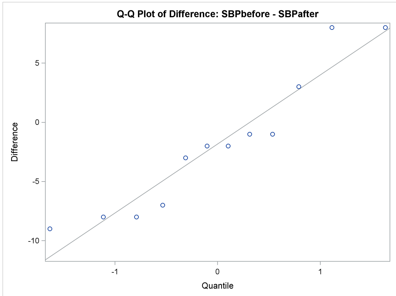
Output 119.3.5 Q-Q Plot
