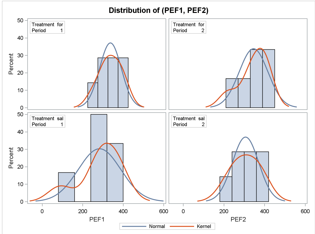
Output 119.4.7 Comparative Histograms
