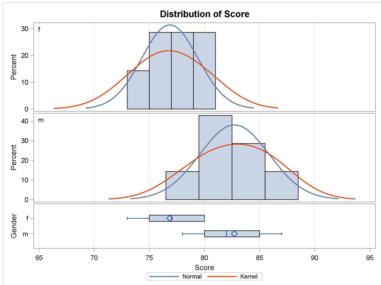
Figure 119.8 Summary Panel
