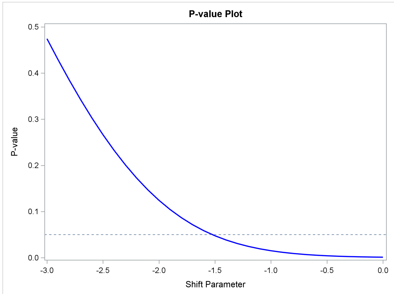
Output 76.13.3 Finding Tipping Point for Shift Parameter between -3 and 0
