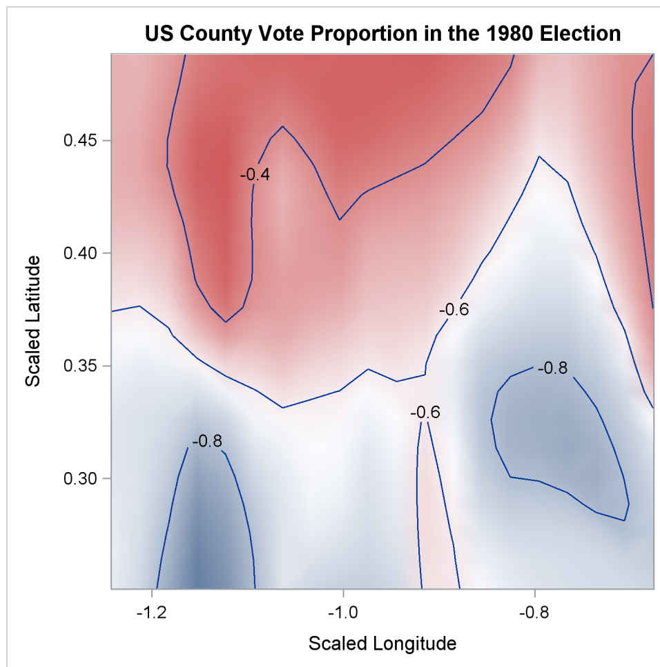
Figure 42.1 US County Vote Proportion in the 1980 Election
