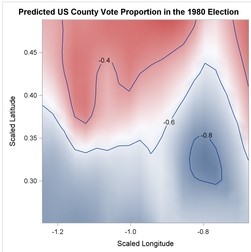
Figure 42.11 Predicted US County Vote Proportion in the 1980 Election
