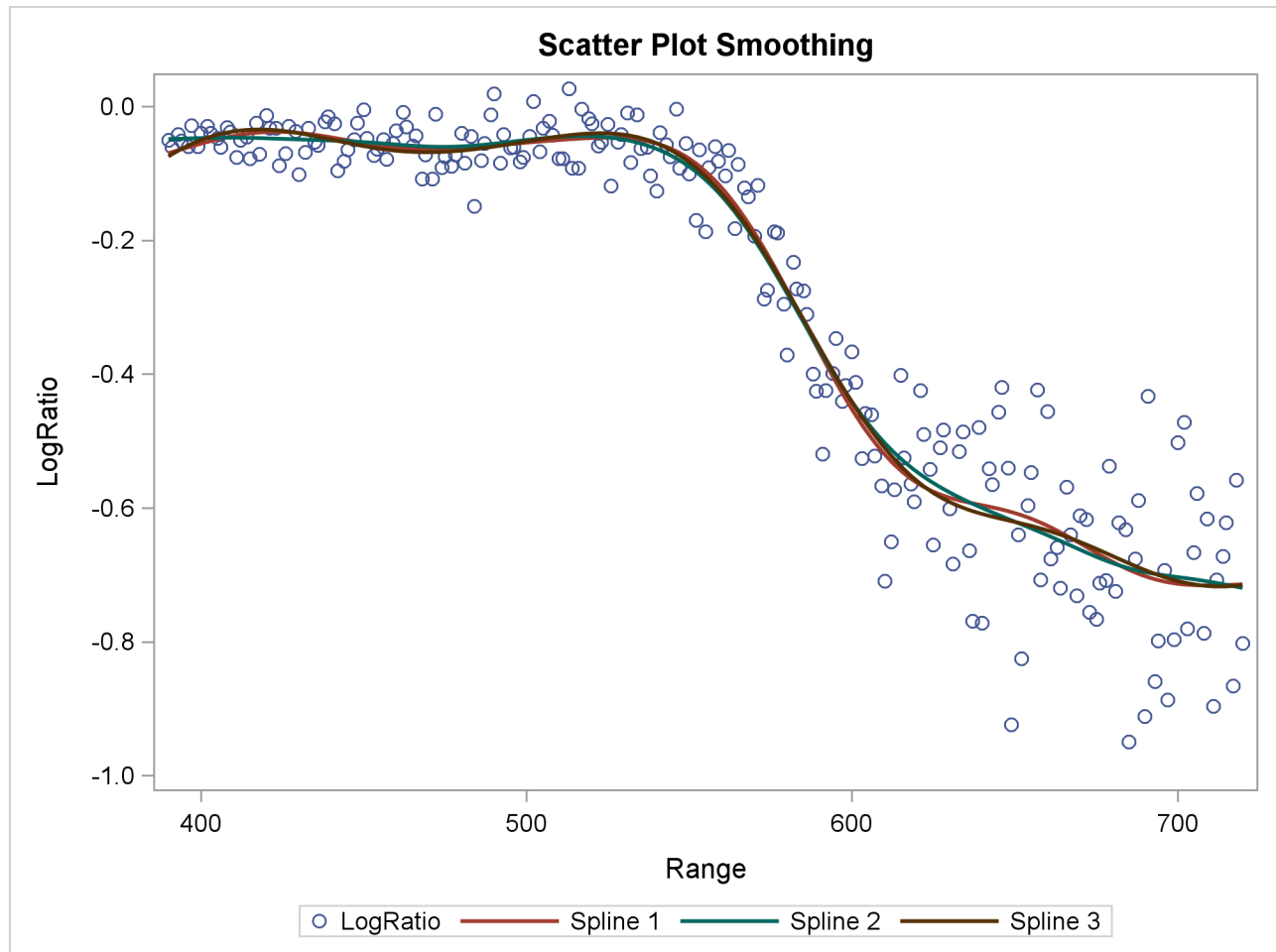
Output 42.1.9 Scatter Plot Smoothing
