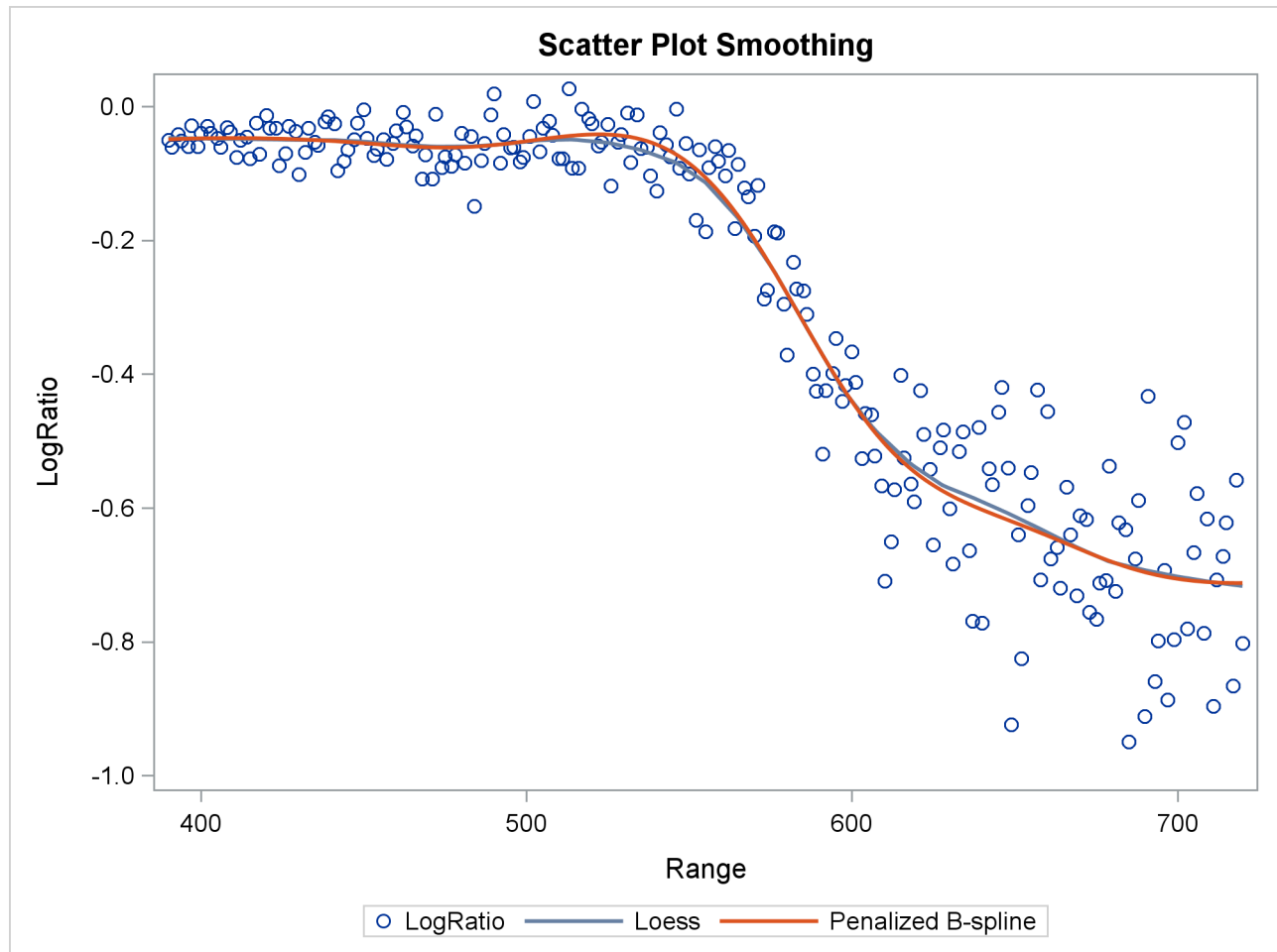
Output 42.1.1 Scatter Plot Smoothing
