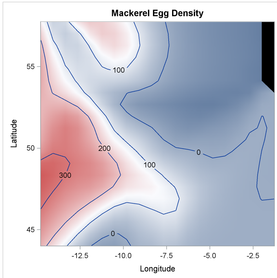
Output 42.3.1 Mackerel Egg Density
