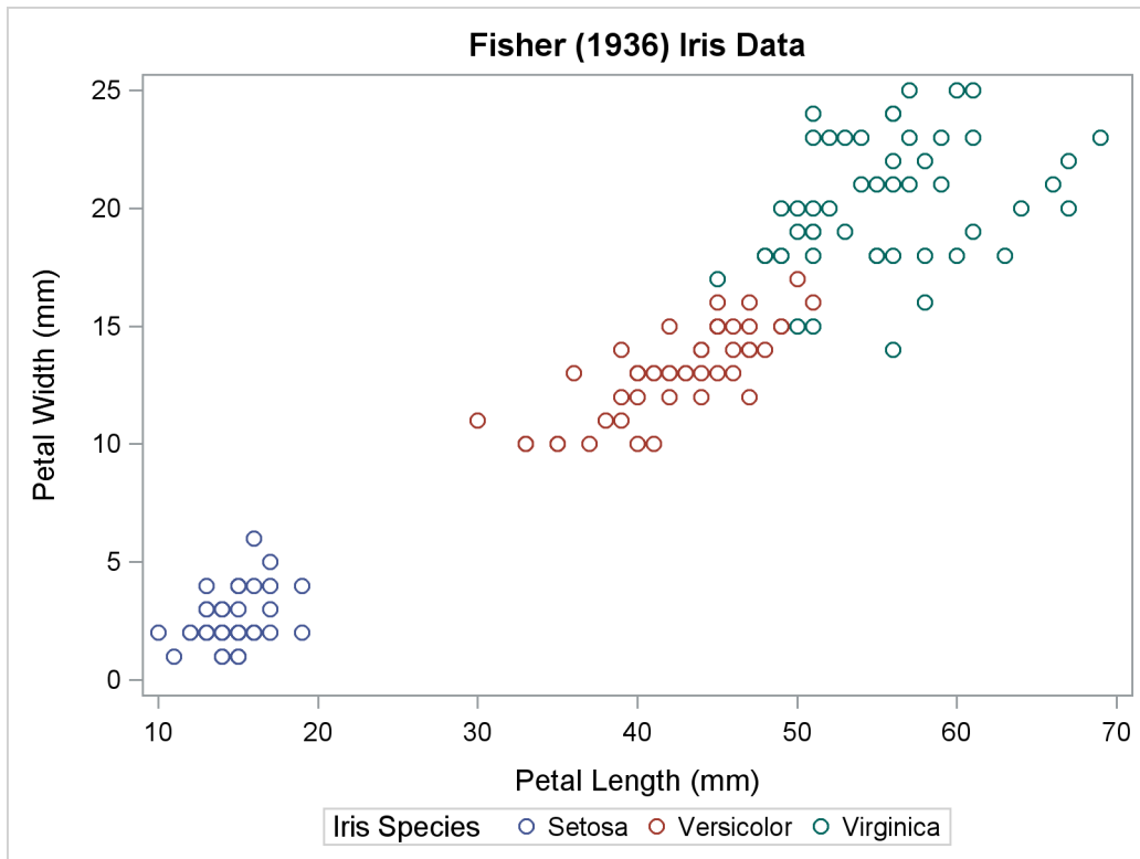
Figure 21.12 Iris Data
