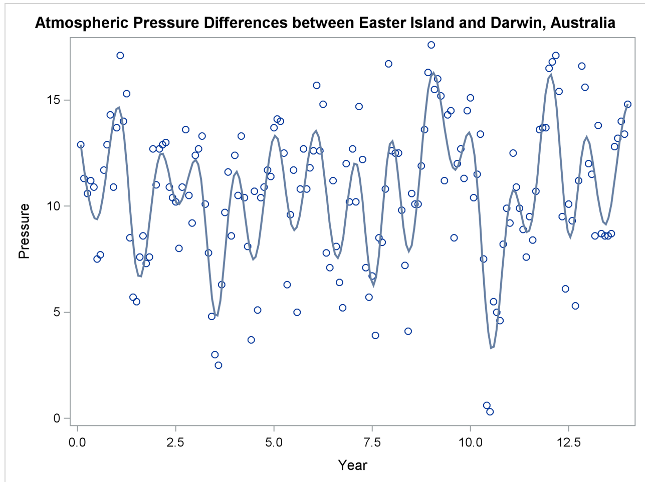
Figure 21.61 Penalized B-Spline Fit with PROC SGPLOT
