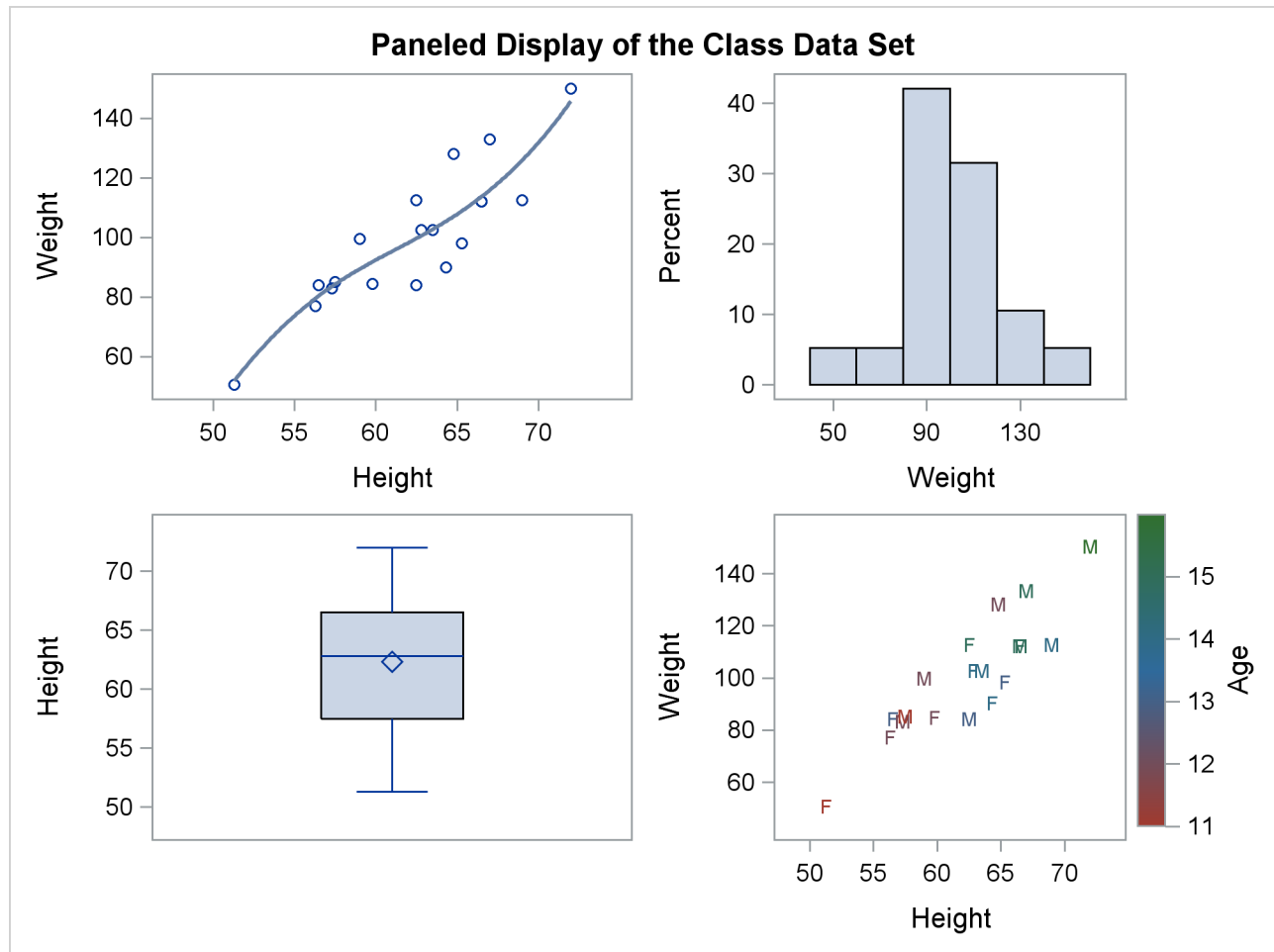
Figure 21.66 Multiple Panels Using PROC SGRENDER
