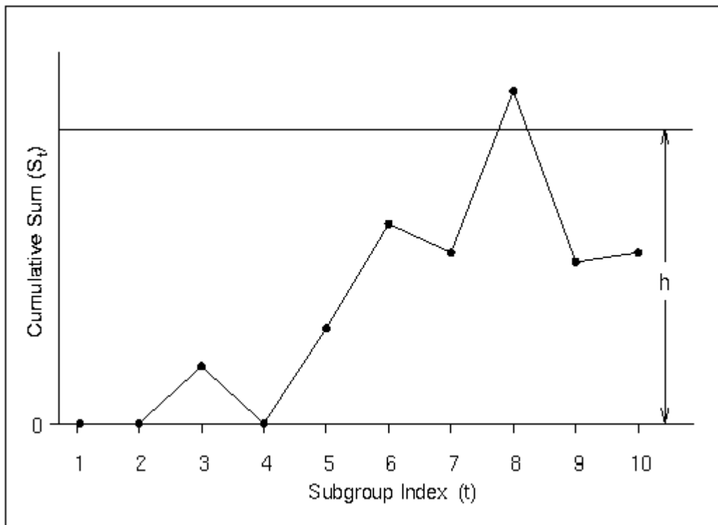
Figure 7.13 Decision Interval
