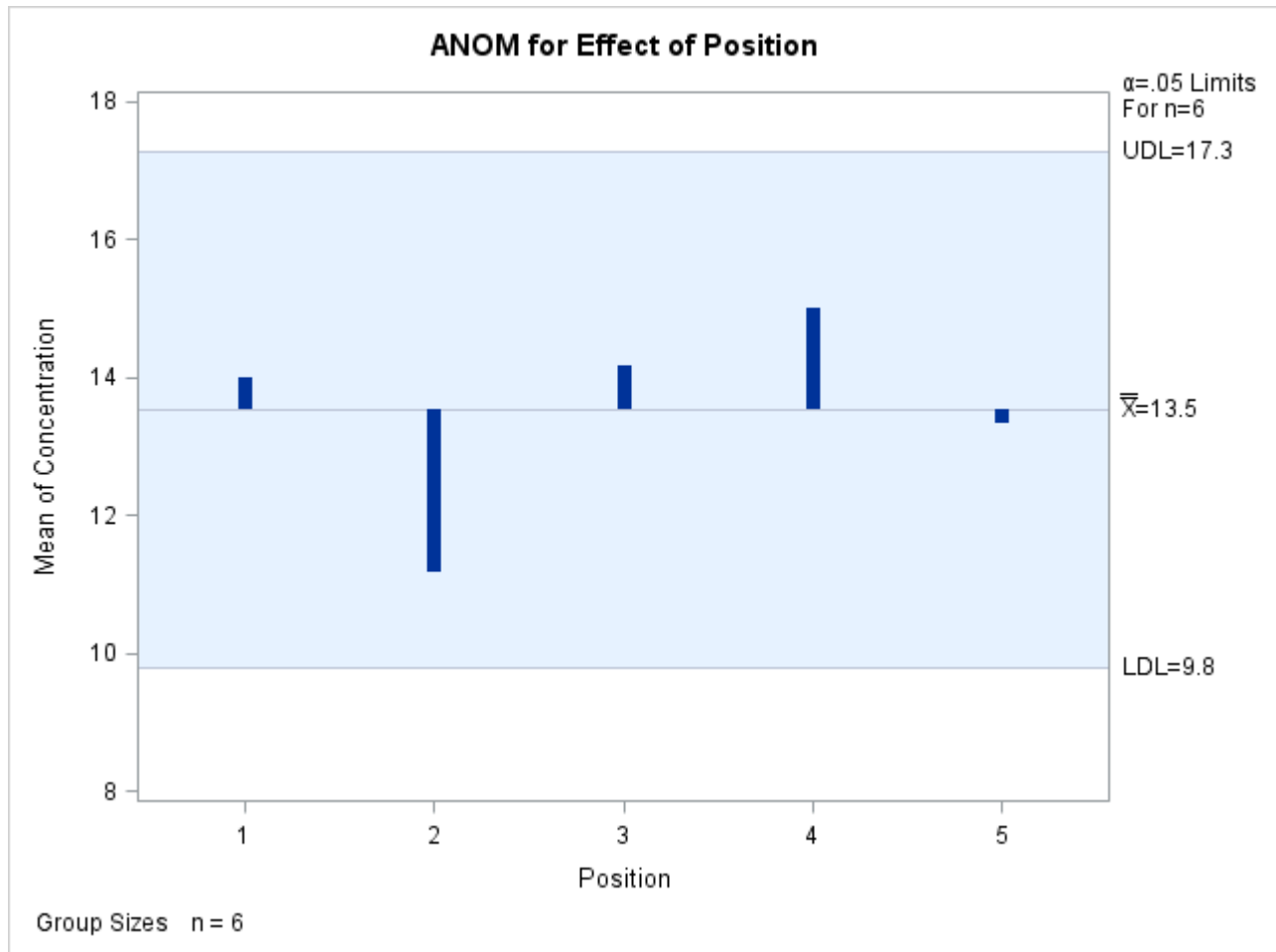
Output 5.5.2 ANOM for Effect of Position
