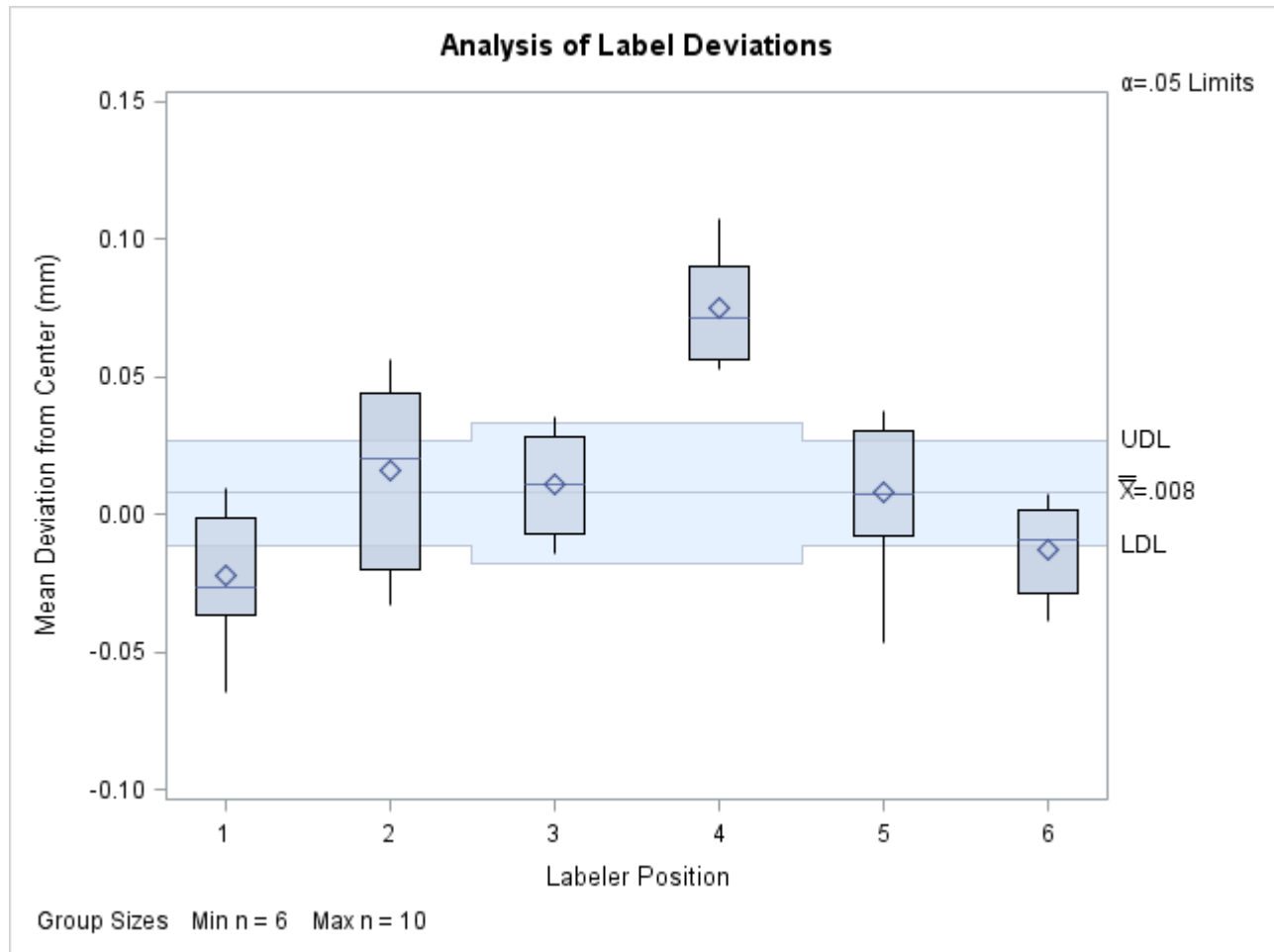
Output 5.1.1 ANOM Chart with Unequal Group Sizes
