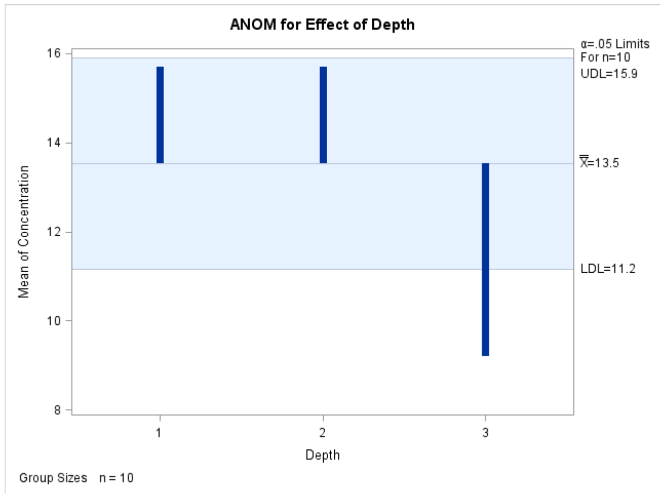
Output 5.5.3 ANOM for Effect of Depth
