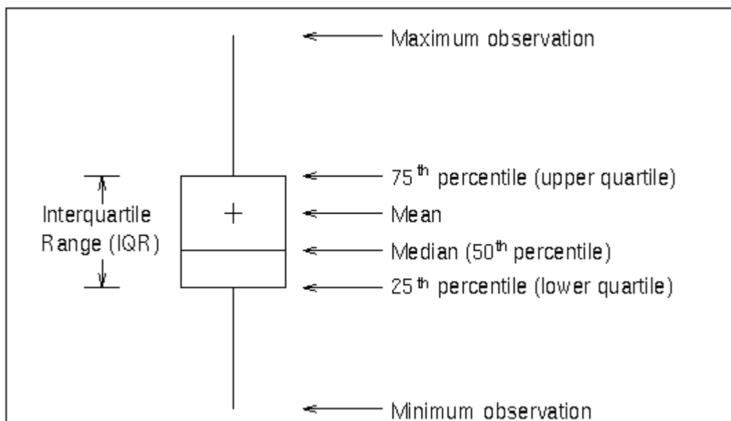
Figure 5.9 Box-and-Whisker Plot
