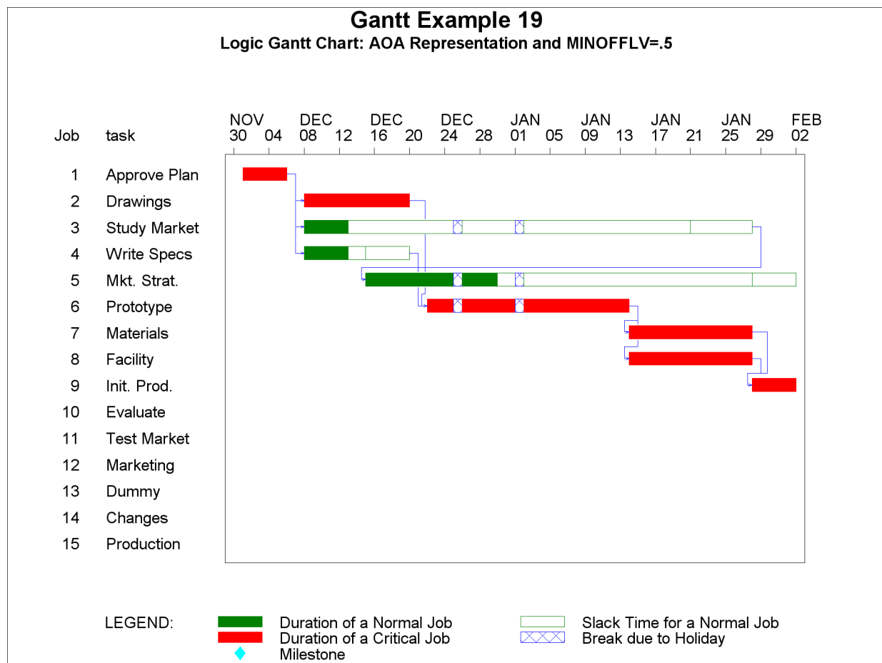
Output 8.19.5 Specifying the MINOFFLV= Option
