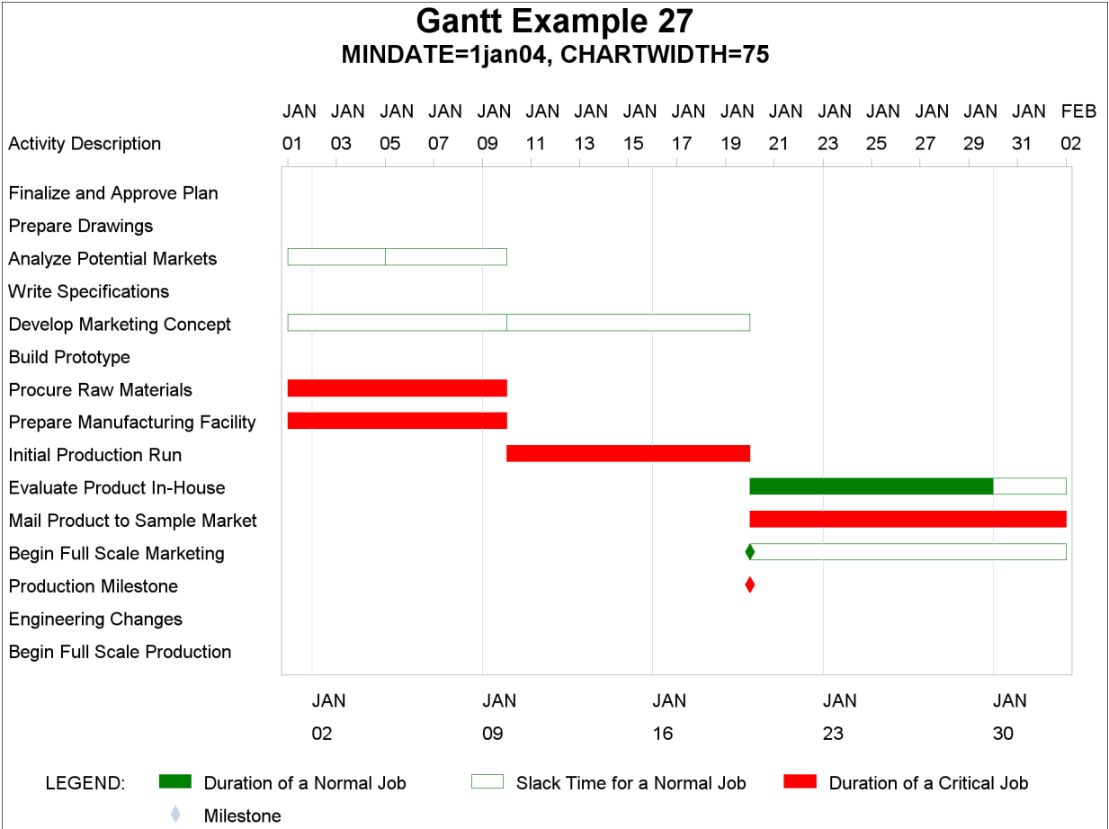
Output 8.27.3 Using the CHARTWIDTH= Option (MINDATE=1Jan04)
