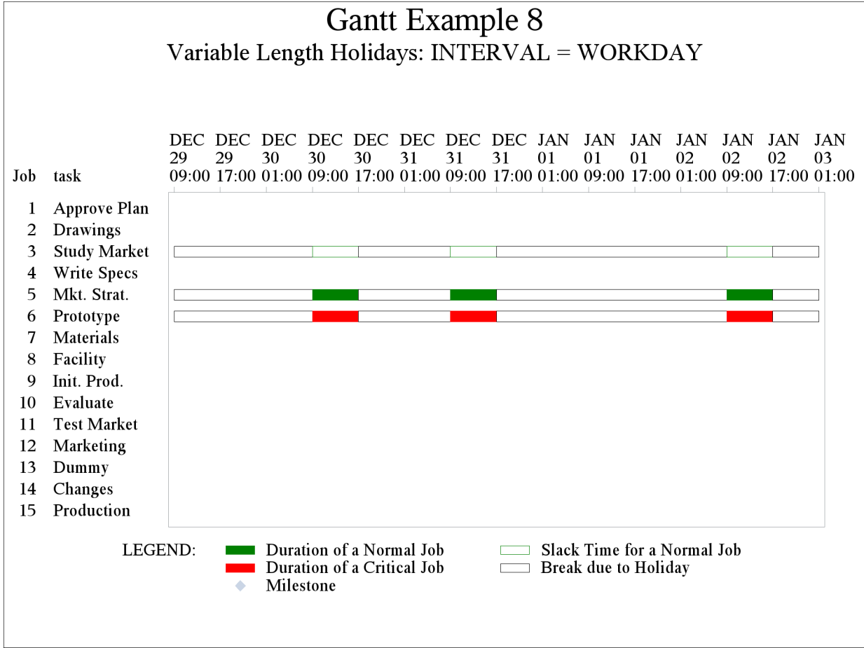
Output 8.8.3 Variable Length Holidays: INTERVAL=WORKDAY
