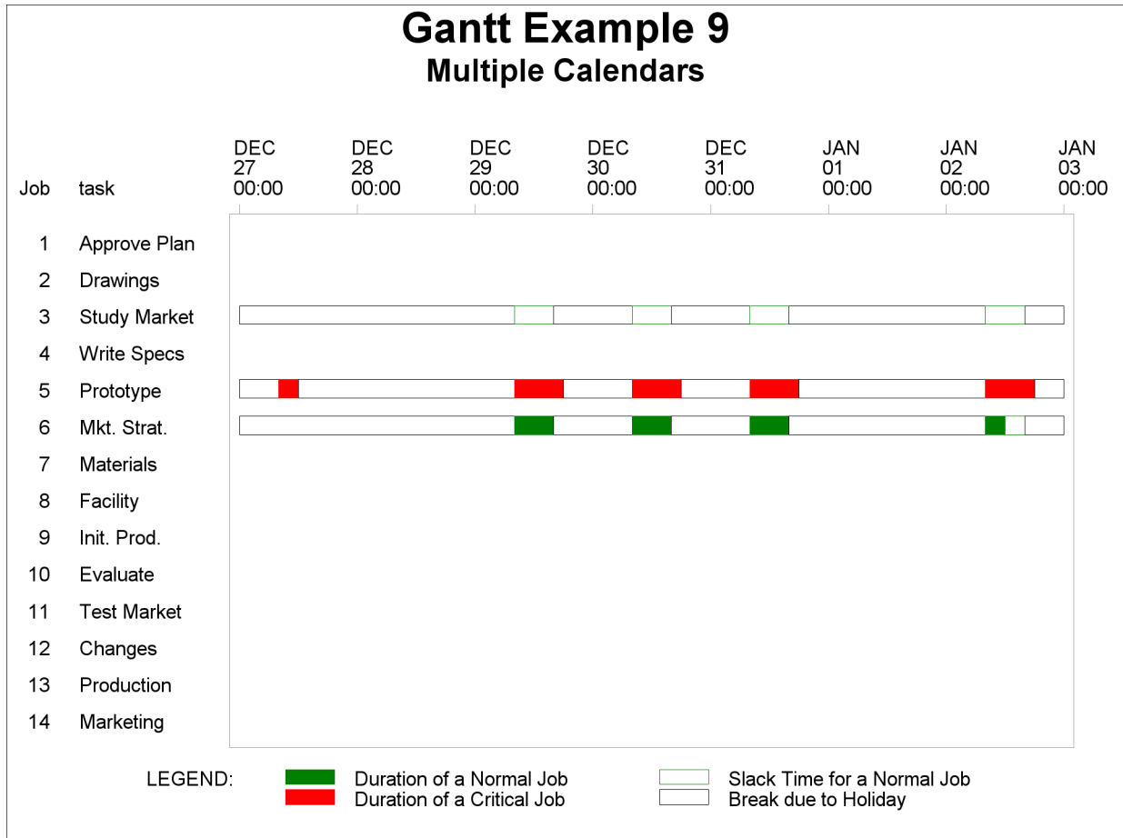
Output 8.9.2 Multiple Calendars
