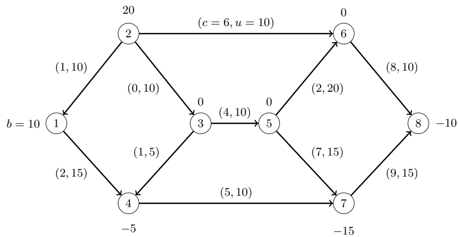
Figure 2.39 Minimum-Cost Network Flow Problem: Data
