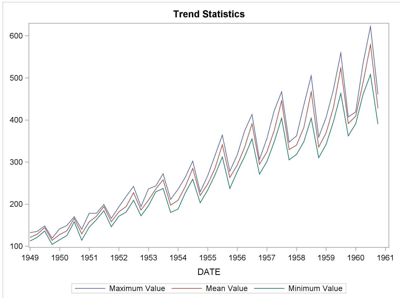
Output 39.2.2 Trend Statistics Plot
