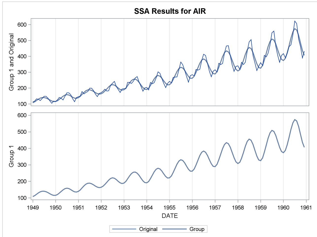
Output 39.5.2 Singular Value Grouping #1 Plot
