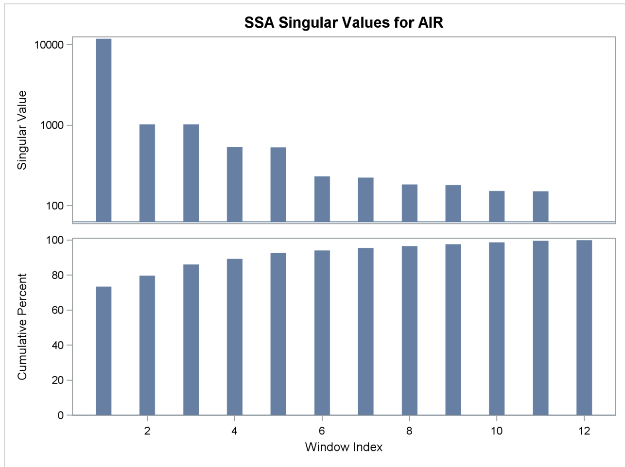
Output 39.5.1 Singular Values Plot
