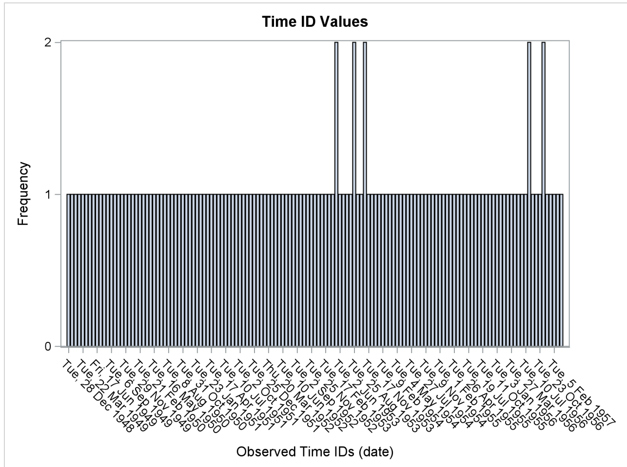
Output 38.1.10 Unaligned Time ID Histogram
