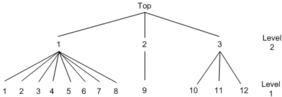
Figure 24.30 Decision Tree for Two-Level Nested Logit
