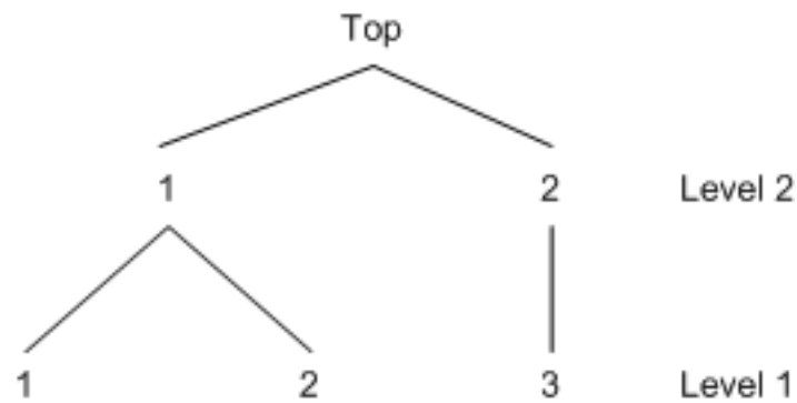
Figure 24.29 Nested Tree Structure
