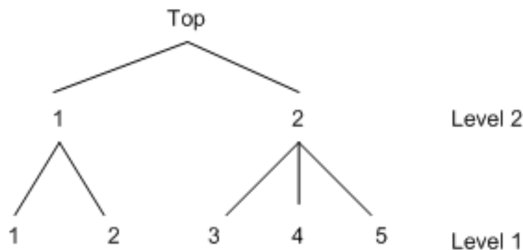
Figure 24.27 Two-Level Decision Tree
