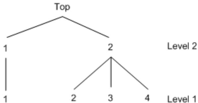
Figure 24.25 An Alternate Two-Level Tree
