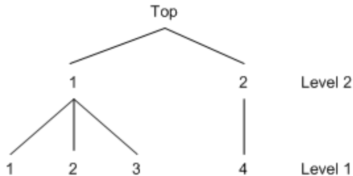
Figure 24.24 A Two-Level Tree
