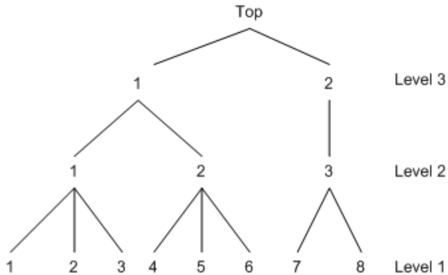
Figure 24.22 A Three-Level Tree
