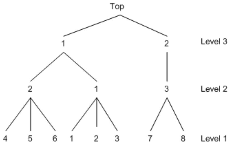
Figure 24.23 An Alternative Three-Level Tree
