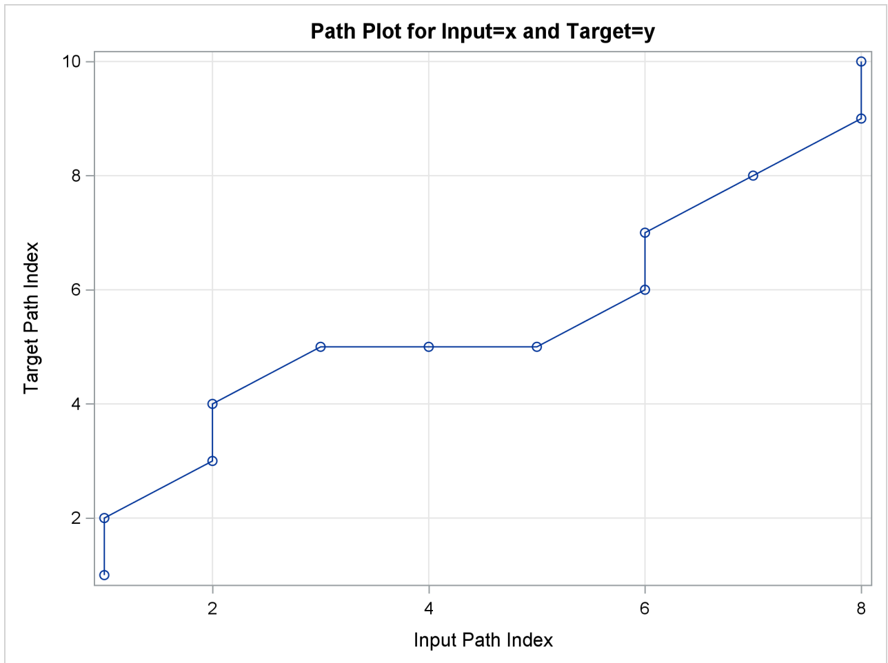
Output 31.2.5 Path Plot
