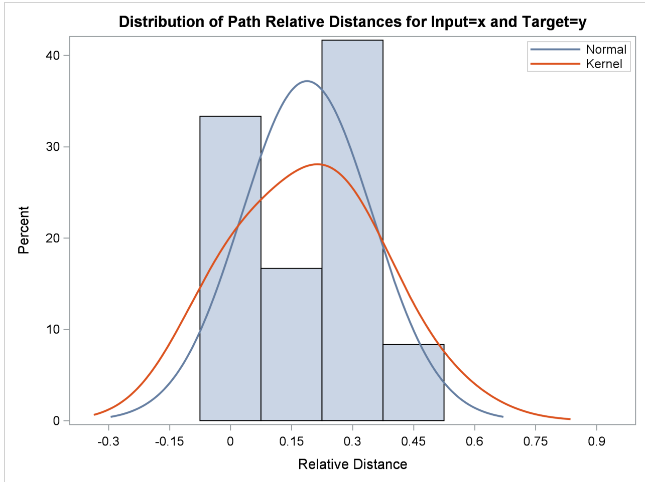
Output 31.2.11 Path Relative Distance Histogram
