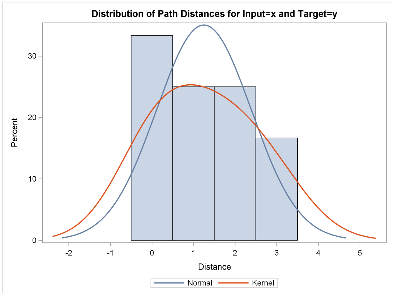
Output 31.2.9 Path Distance Histogram
