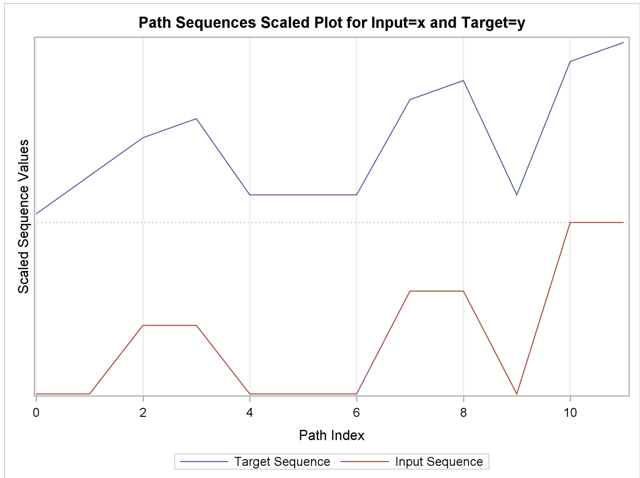
Output 31.2.7 Path Sequences Scaled Plot
