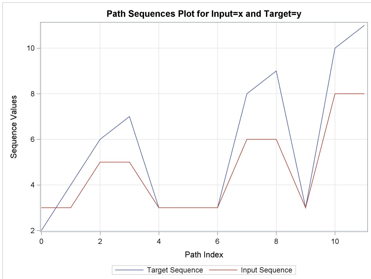
Output 31.2.6 Path Sequences Plot
