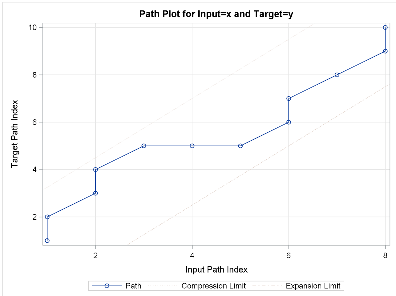
Output 31.2.18 Path Plot with Warping Limits
