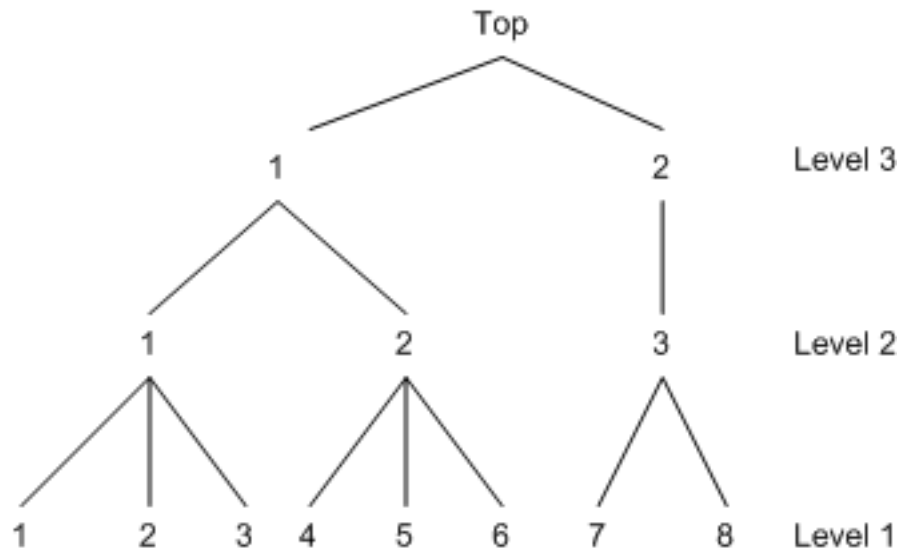
Figure 25.22 A Three-Level Tree
