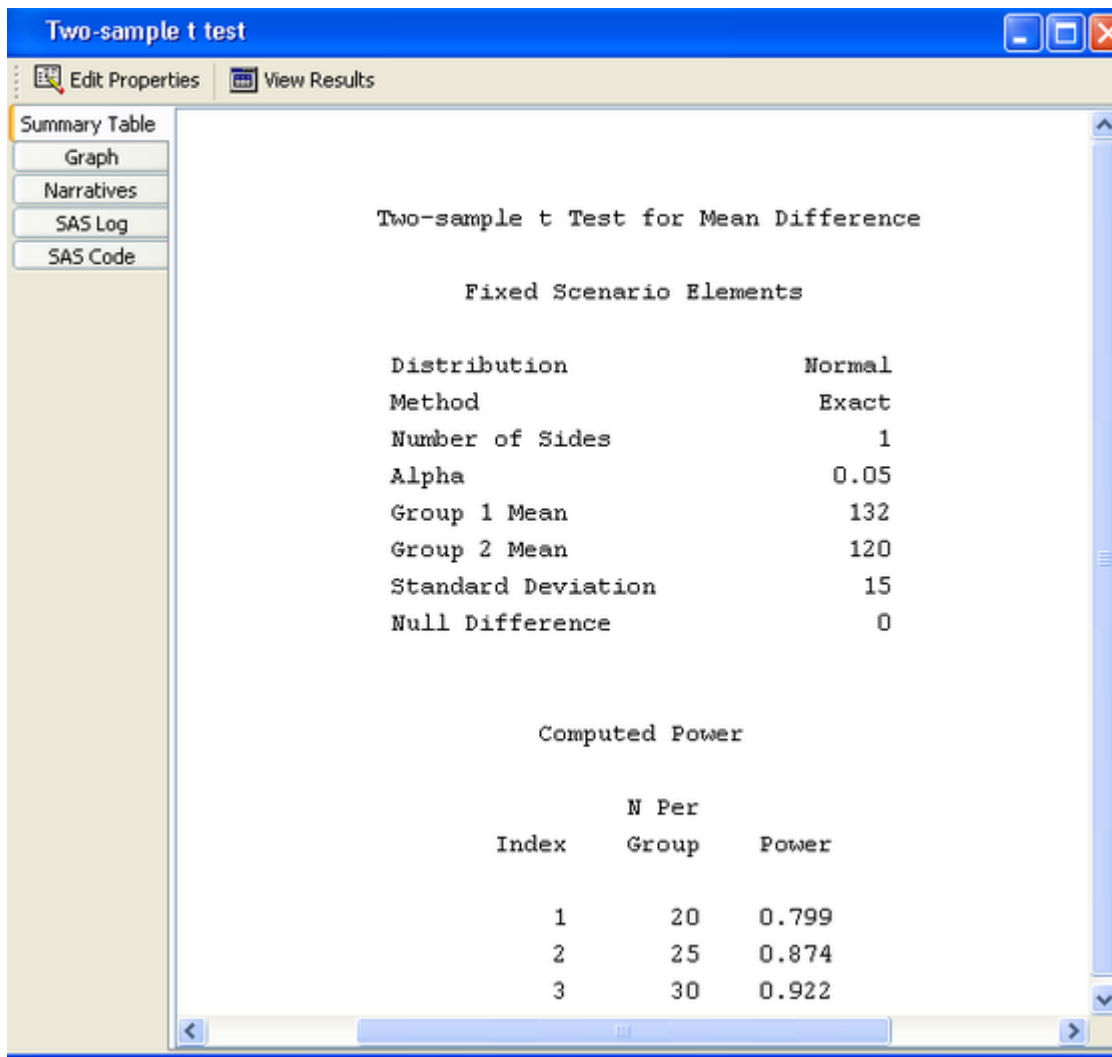
Figure 68.43 Results Page with Summary Table
