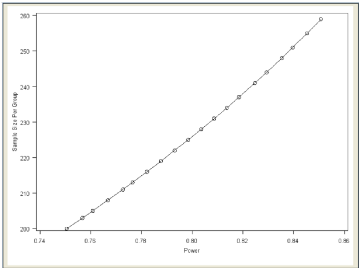
Figure 68.89 Power by Sample Size Graph
