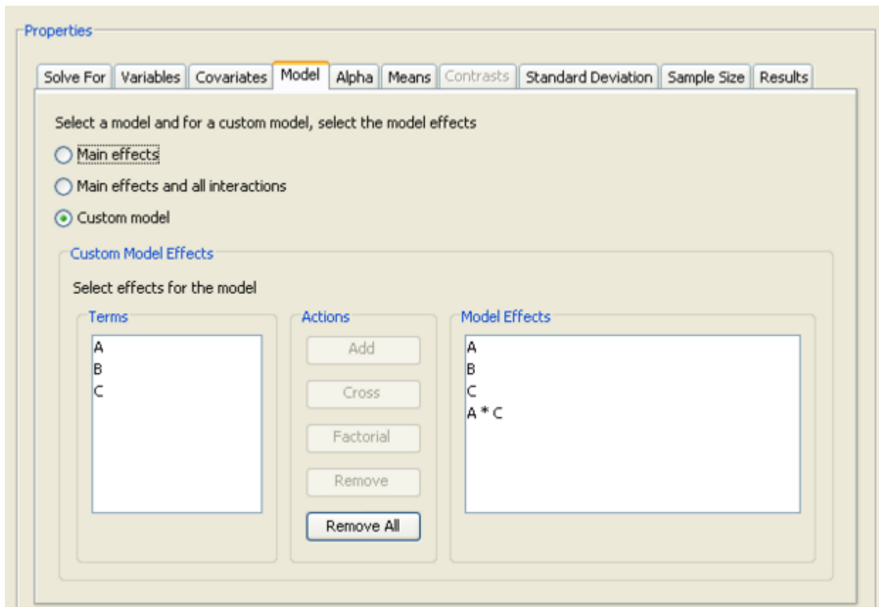
Figure 68.76 Model Tab with Custom Model Builder Displayed
