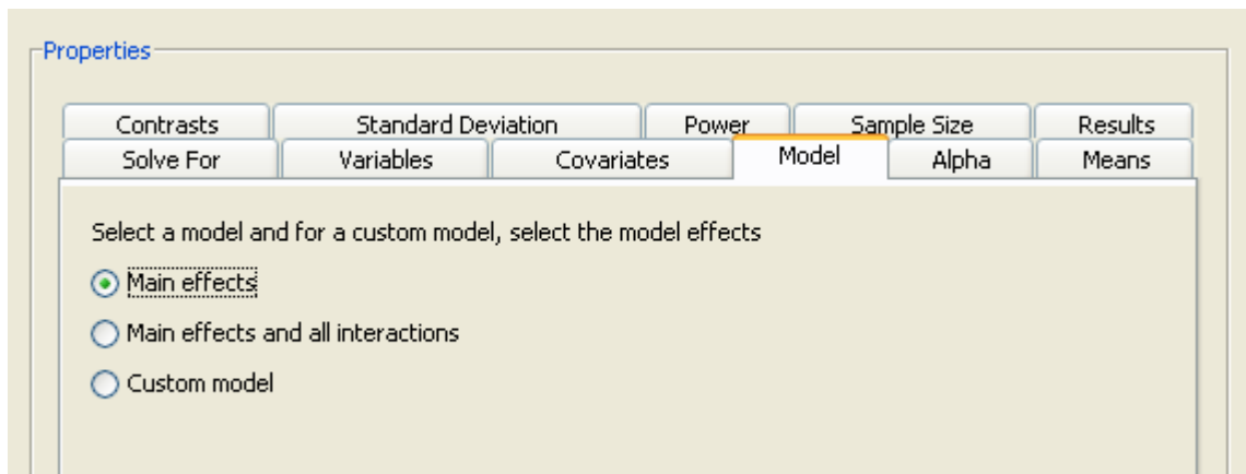
Figure 68.62 Model Tab with Main Effects Selected
