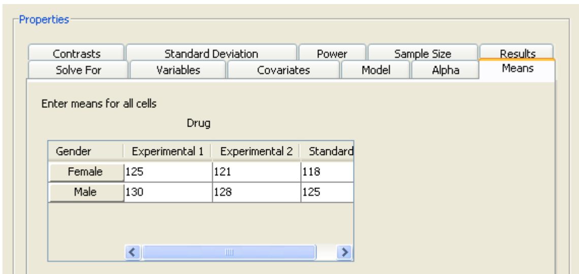
Figure 68.63 Means Tab with Cell Means
