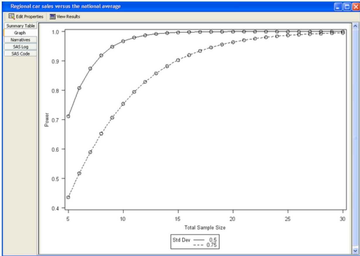
Figure 68.15 Graph Tab with Power by Sample Size Graph
