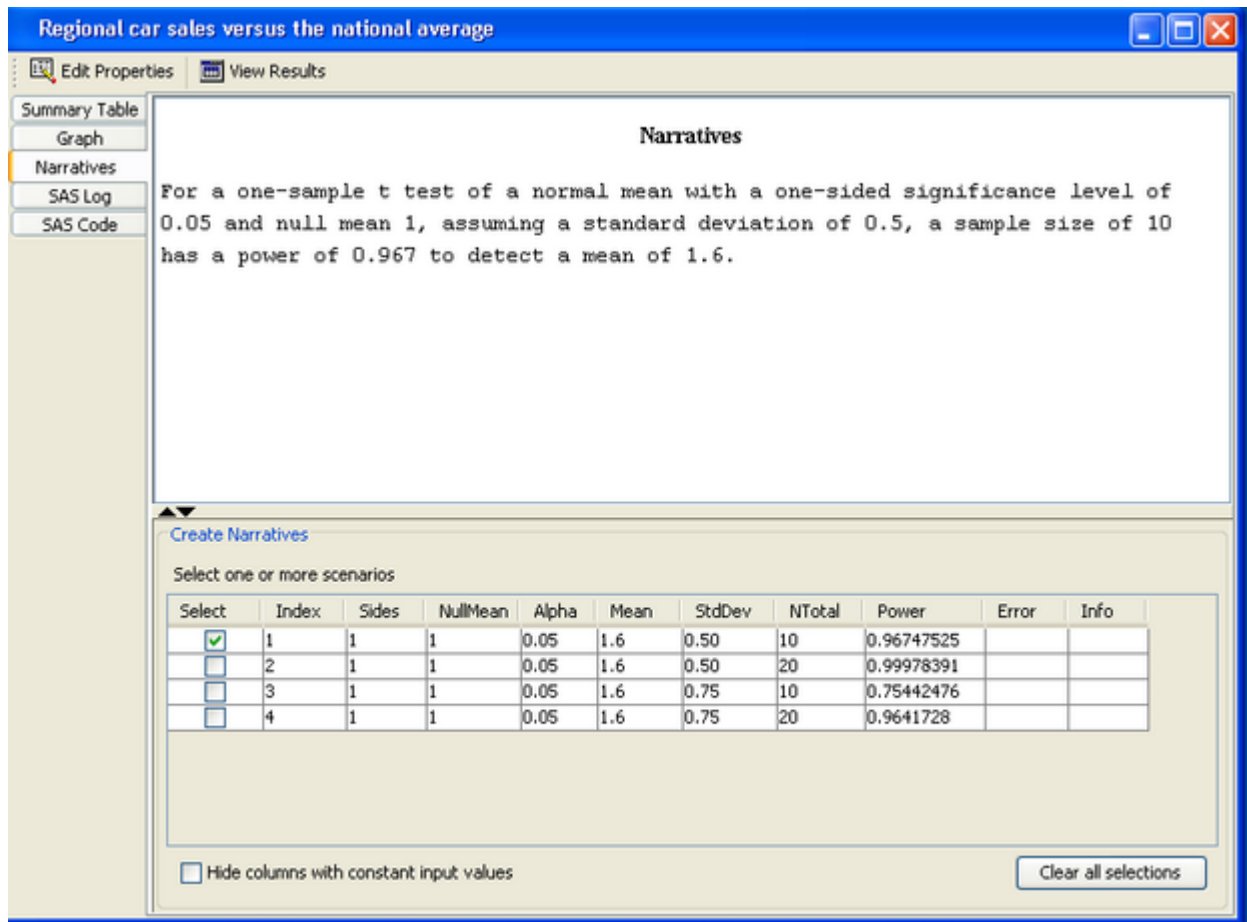
Figure 68.32 Narrative Selector and Display
