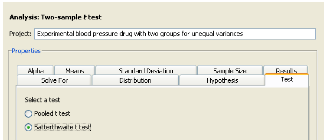
Figure 68.46 Satterthwaite t Test Option
