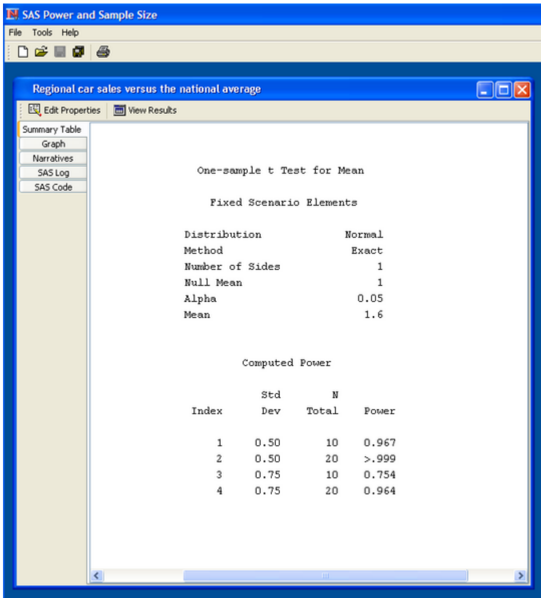
Figure 68.31 View Results Page with Summary Table
