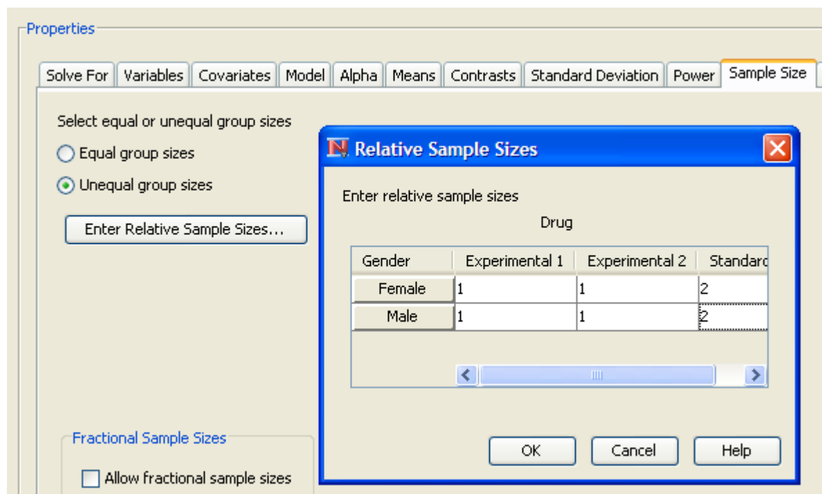
Figure 68.73 Relative Sample Sizes Window
