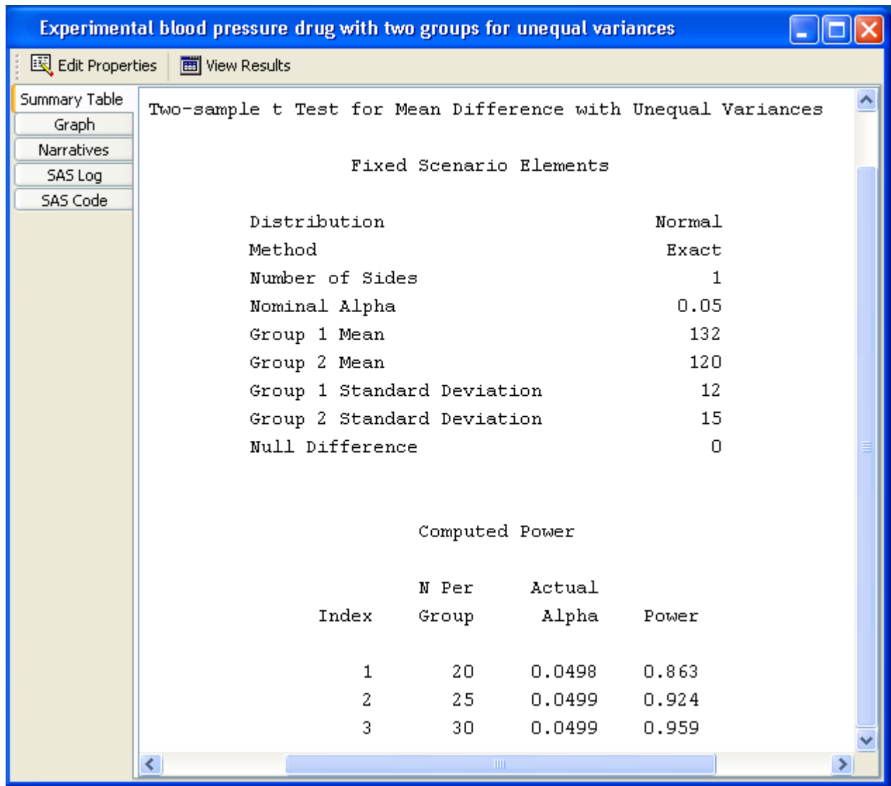
Figure 68.48 Satterthwaite Test Results
