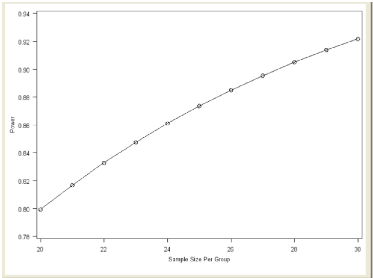
Figure 68.44 Power by Sample Size Graph
