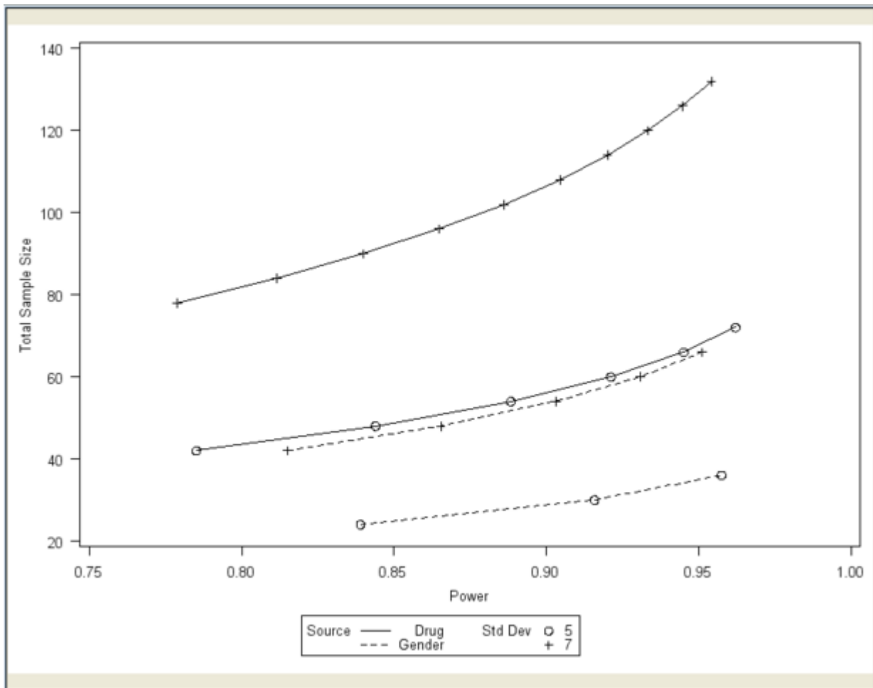
Figure 68.69 Power by Sample Size Graph
