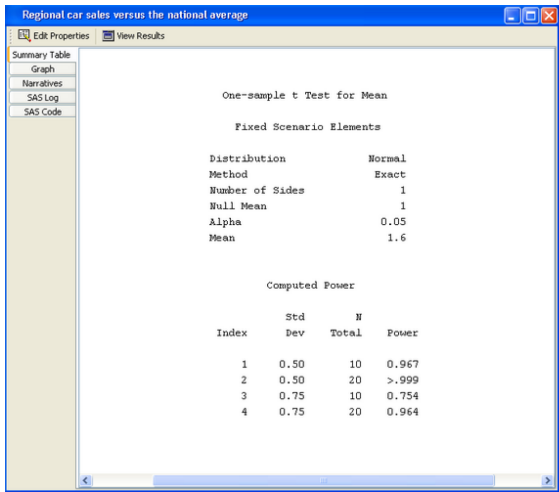
Figure 68.14 Summary Table Tab with Fixed Scenario Elements and Computed Power Tables
