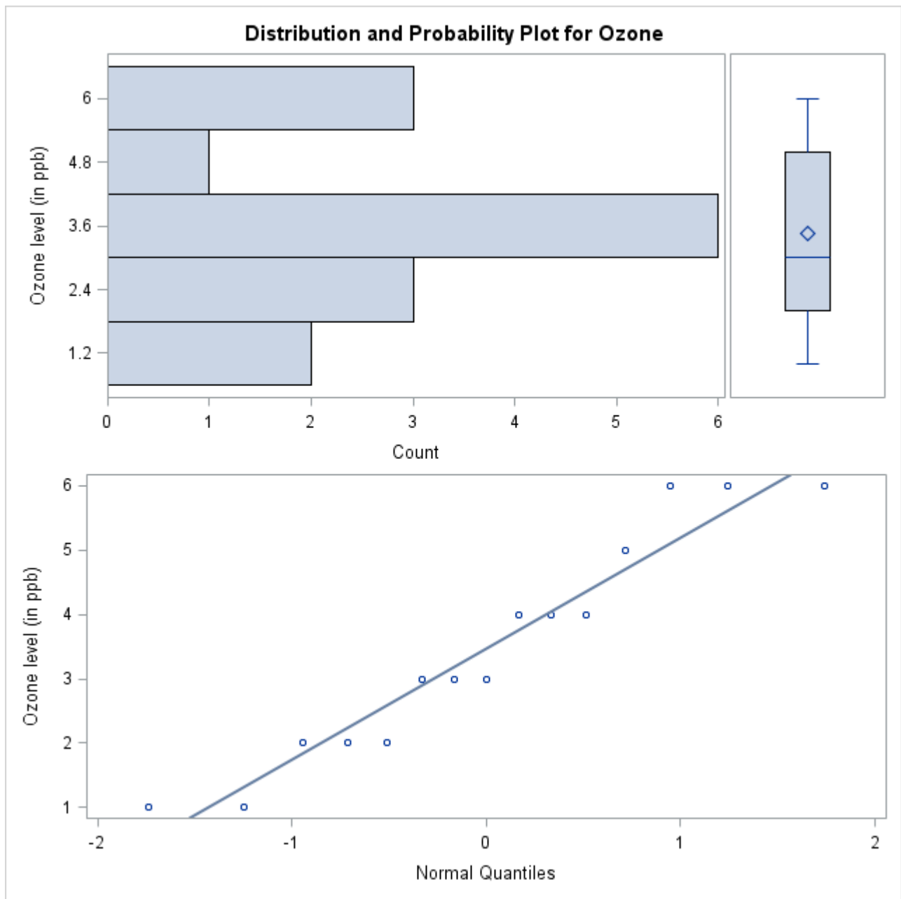
Output 4.5.6 Ozone Plots for BY Group Site = 134
