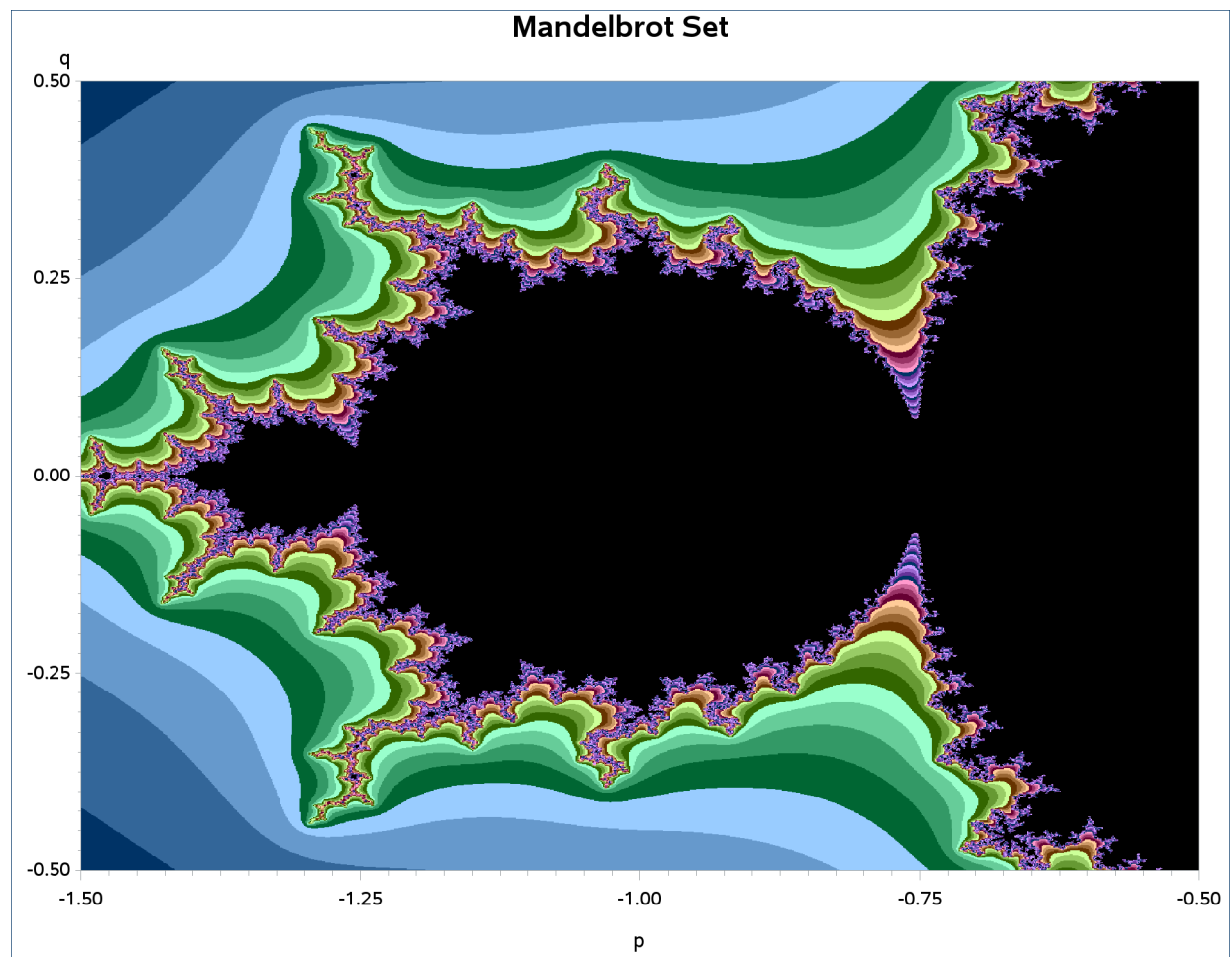
Output 7.1.1 Computed Mandelbrot Set
