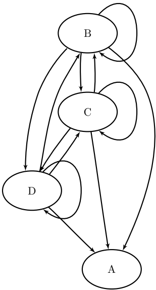
Figure 2.68 Transitive Closure of G
