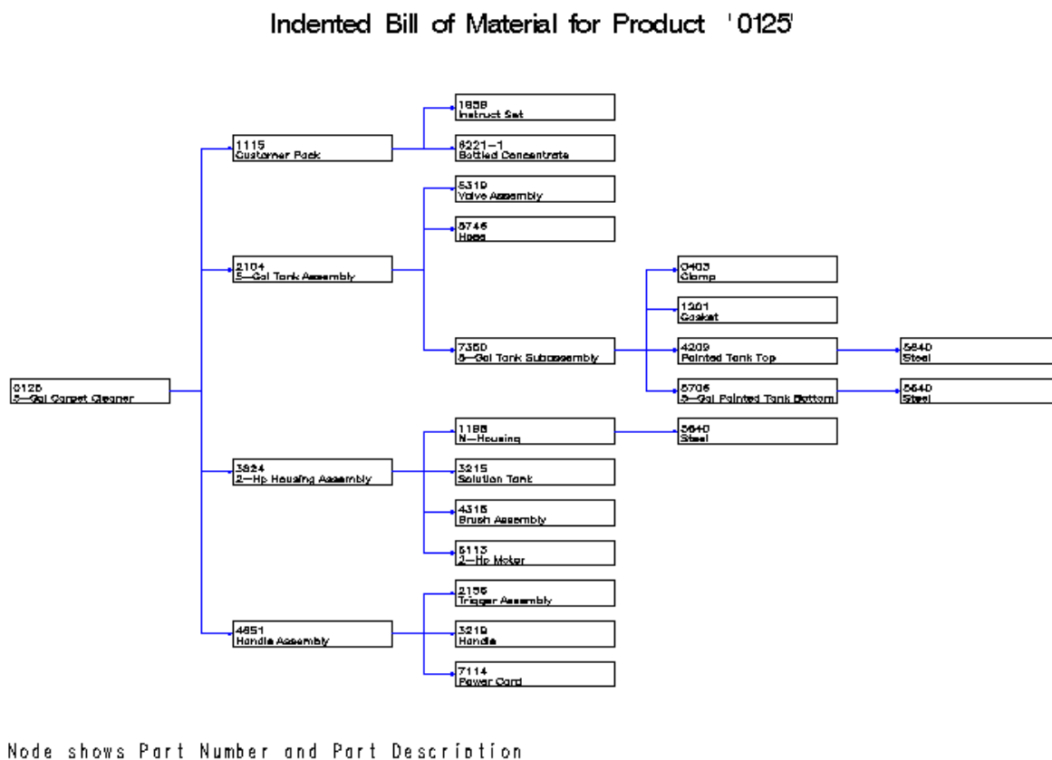
Figure A.6 Indented BOM, Diagram View
