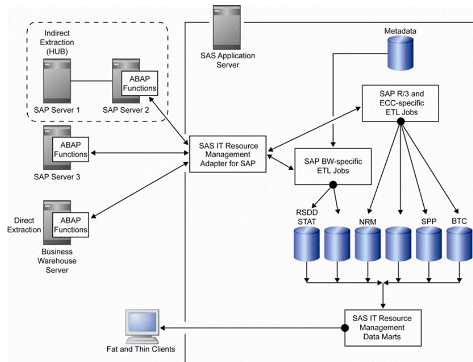
Figure A2.1 Solution Architecture
