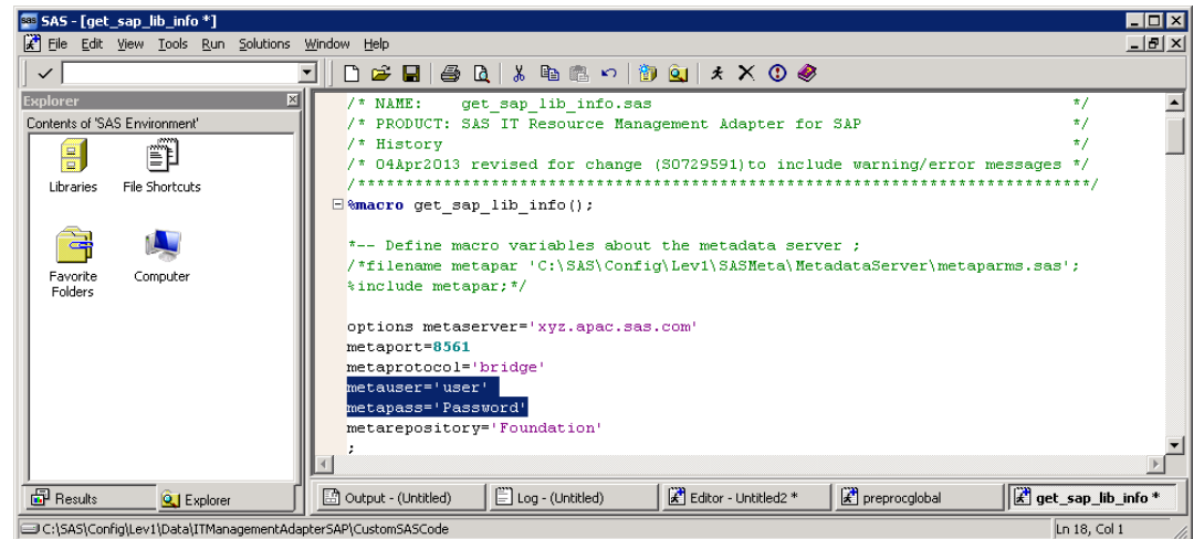
Display 4.9 Program to Get SAP Library Information
