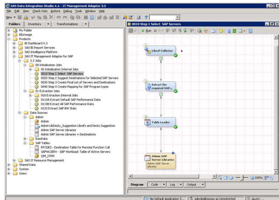
Display 5.2 0010 Step 1 Select SAP Servers
