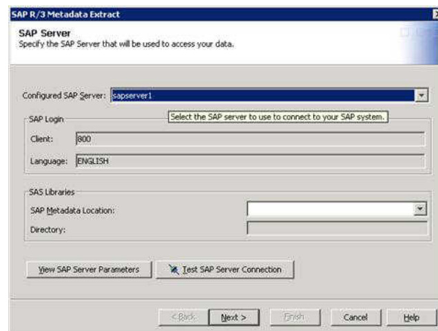
Display 3.17 SAP R/3 Metadata Extract
