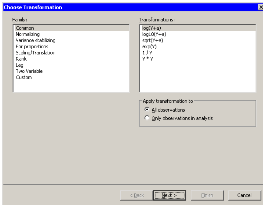
Figure 32.11 Common Transformations
