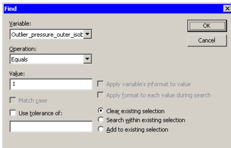
Figure 17.6 Finding Outliers
