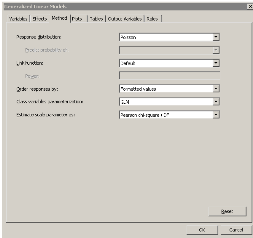
Figure 24.21 Modeling Overdispersion
