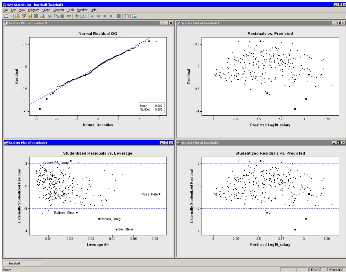
Figure 21.12 Residual Plots
