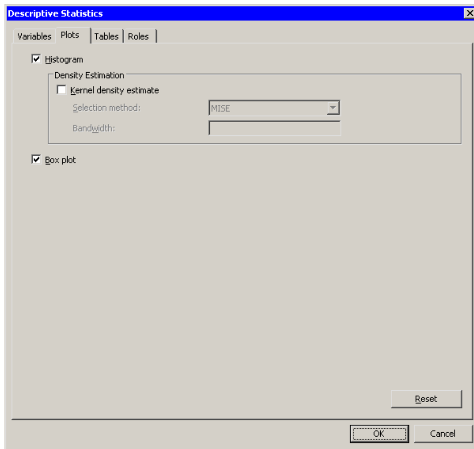
Figure 13.5 Selecting Plots
