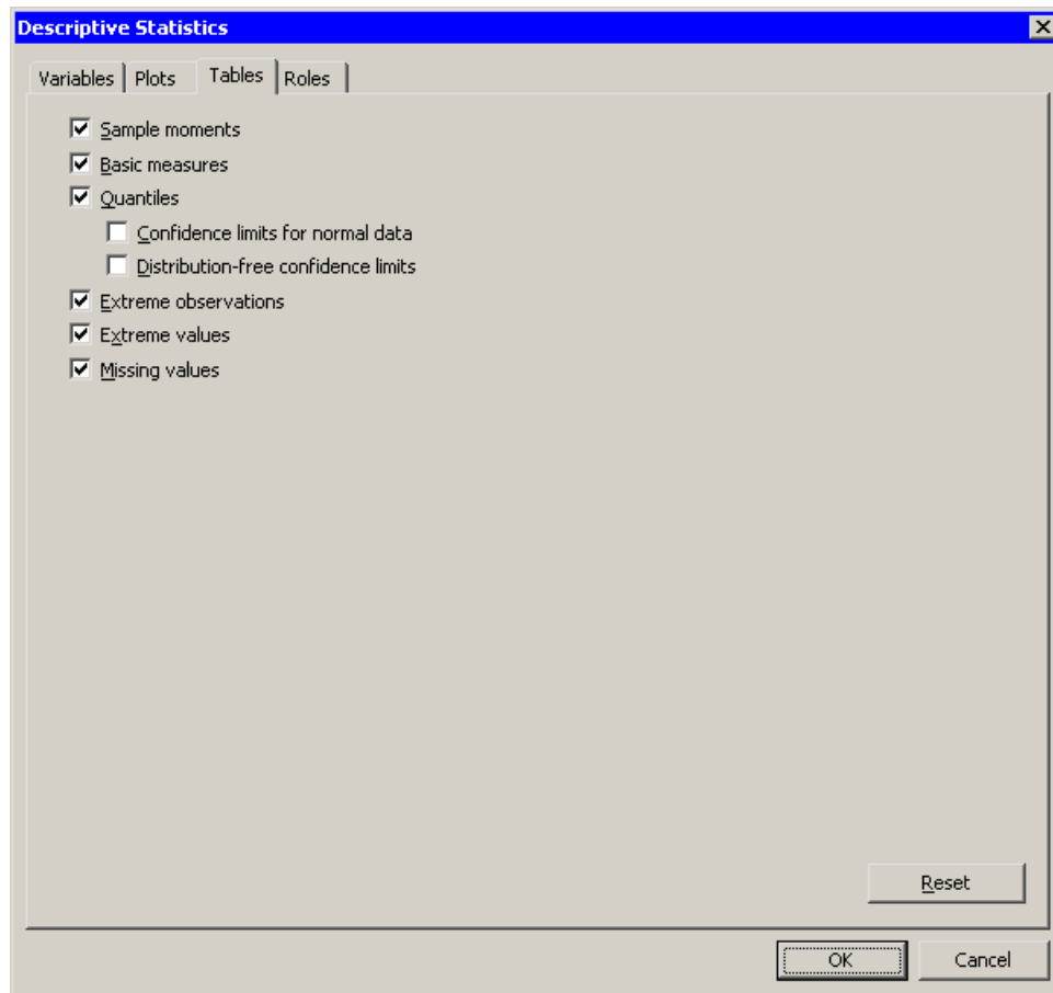
Figure 13.3 Selecting Tables
