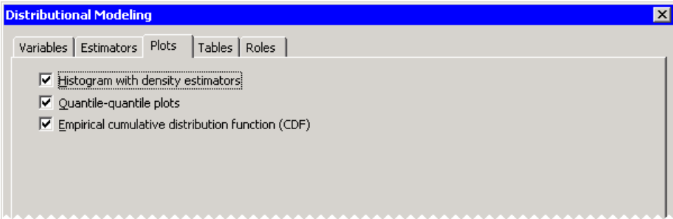
Figure 15.5 Selecting Plots
