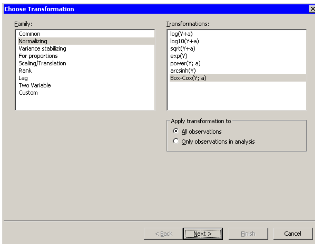
Figure 32.12 Normalizing Transformations
