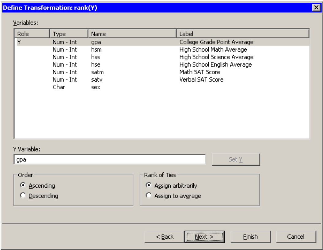
Figure 32.17 Rank Transformations
