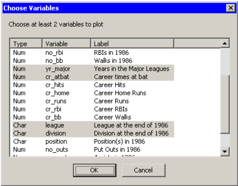
Figure 33.3 Selecting Variables
