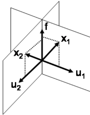
Figure 27.1 The Geometry of Factor Analysis
