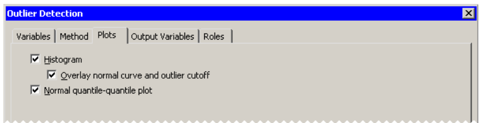
Figure 17.4 Selecting Plots
