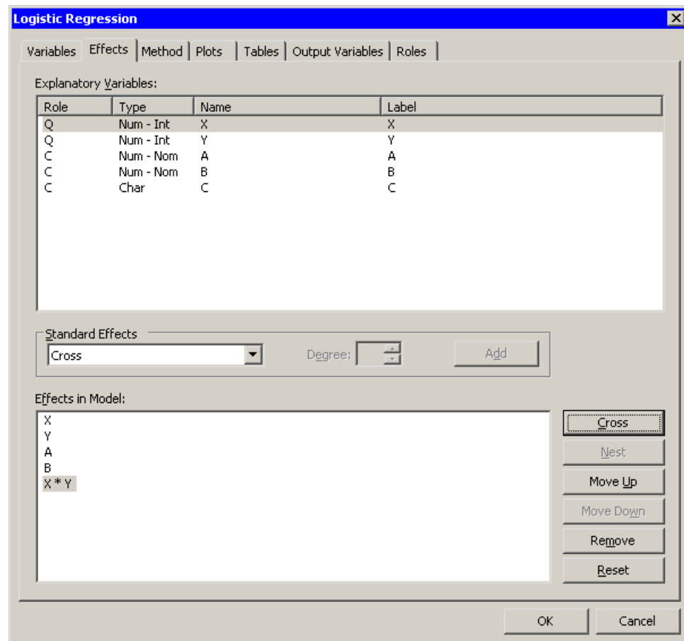
Figure 23.7 Specifying Crossed Effects
