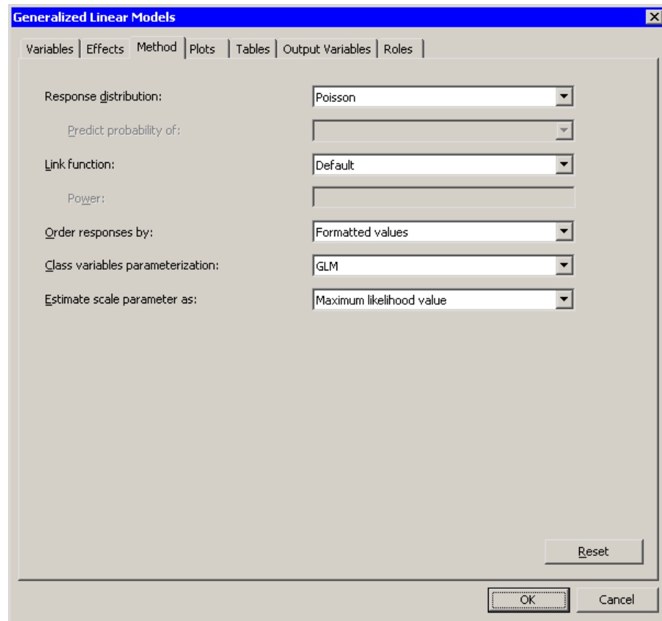
Figure 24.19 The Method Tab
