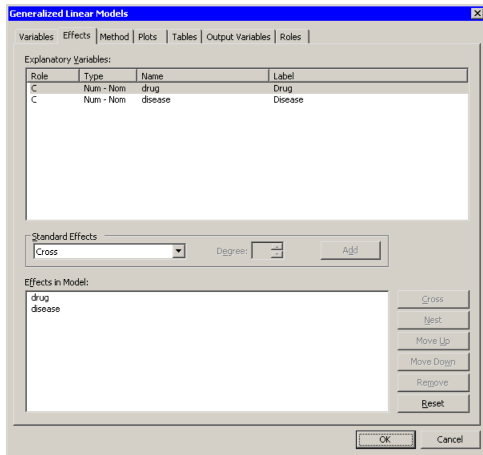
Figure 24.11 Revising the Model
