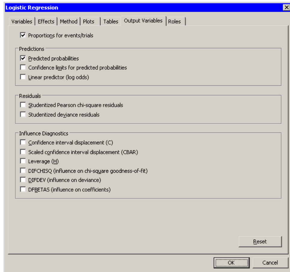
Figure 23.13 The Output Variables Tab
