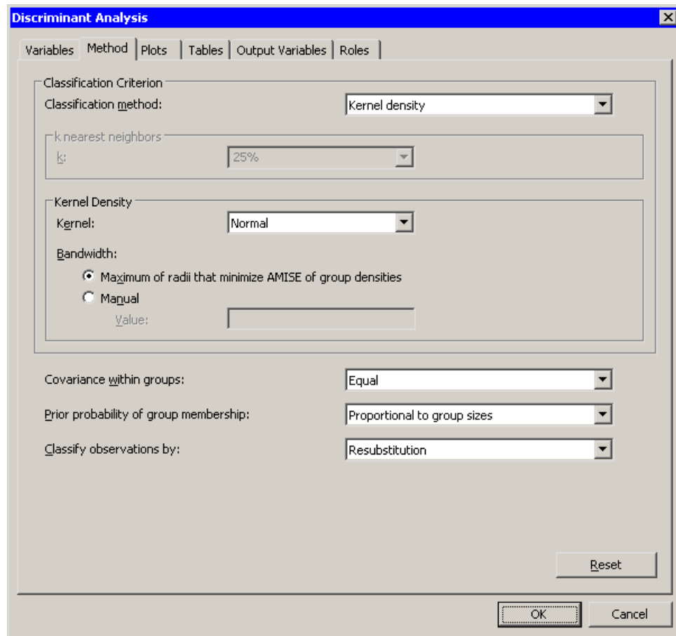
Figure 30.3 The Method Tab
