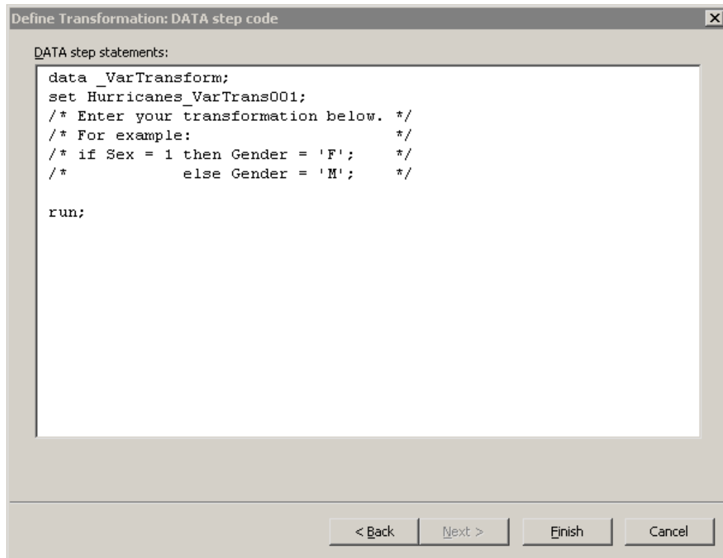
Figure 32.22 A Wizard Page Where You Can Enter DATA Step Statements
