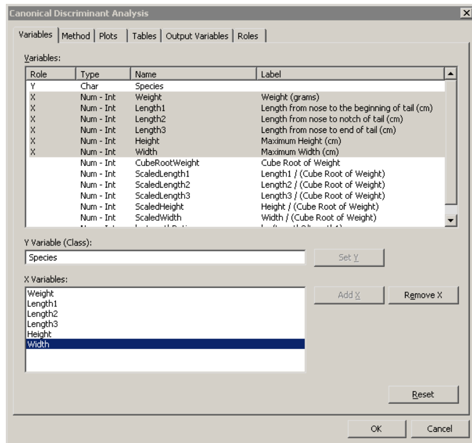
Figure 29.2 The Variables Tab
