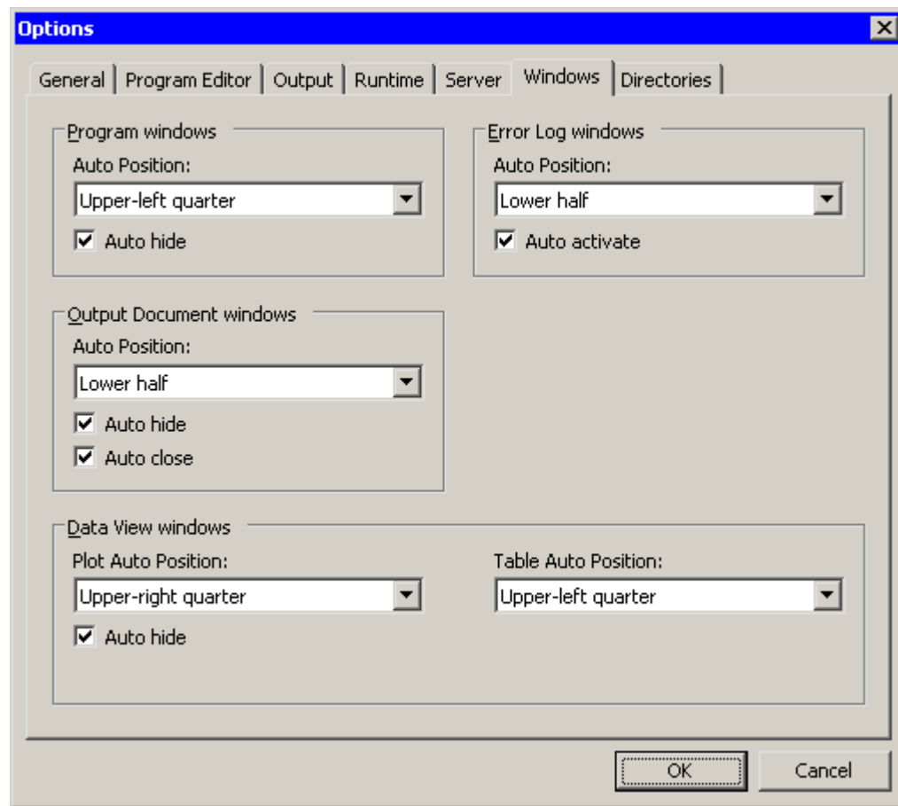
Figure 34.10 The Windows Tab
