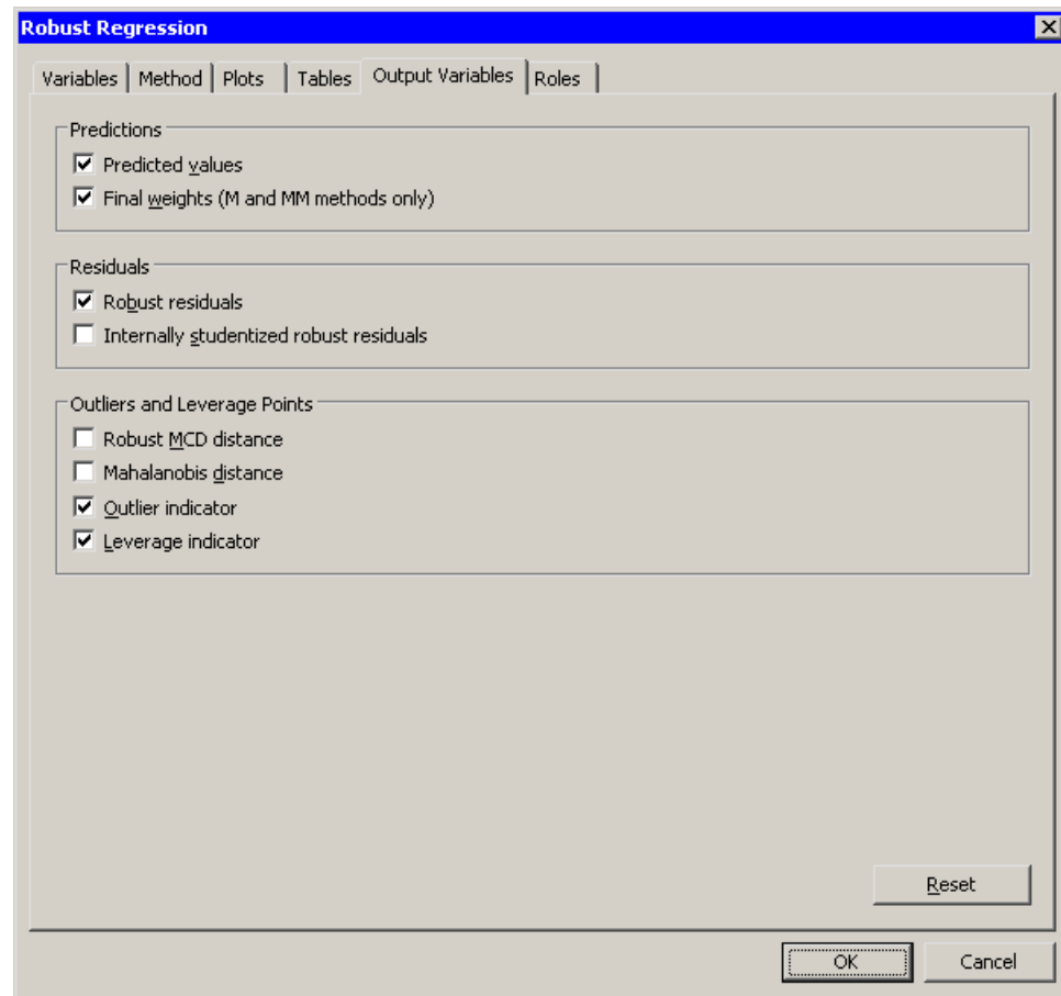
Figure 22.5 The Output Variables Tab
