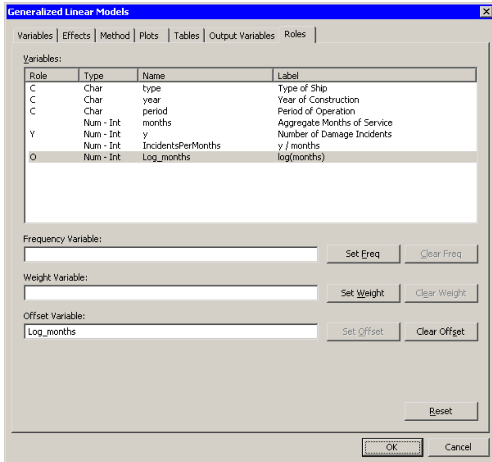
Figure 24.18 The Roles Tab
