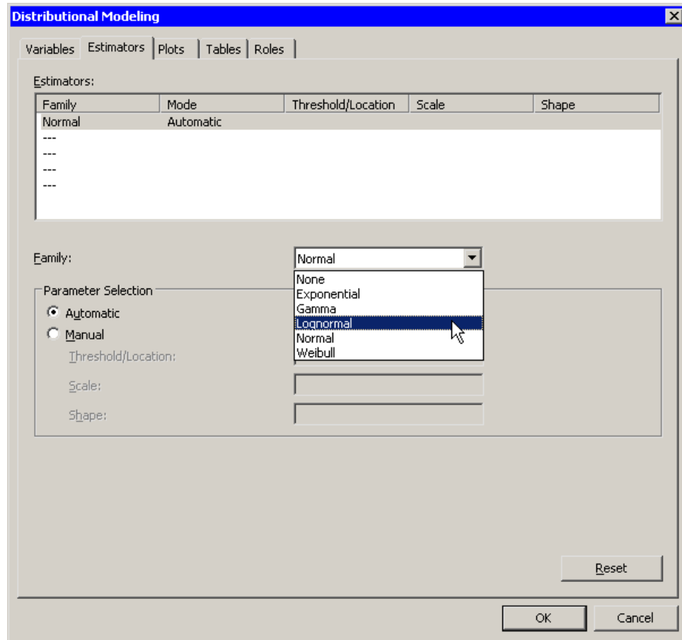
Figure 15.8 Selecting a Lognormal Distribution
