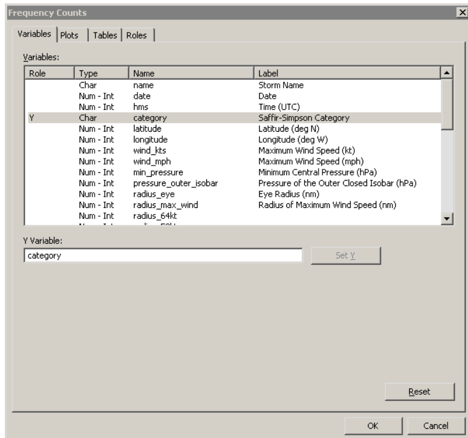
Figure 16.2 Specifying a Variable
