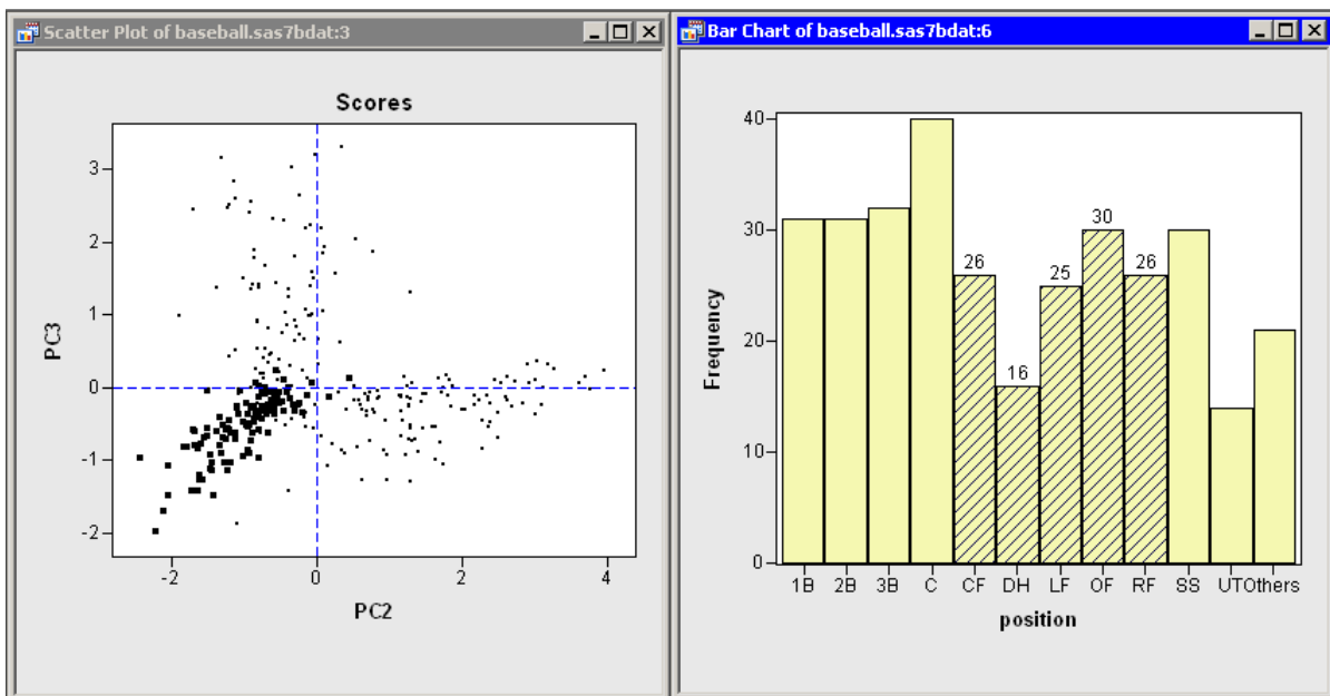
Figure 26.10 Fielding Scores for Outfielders and Designated Hitters
