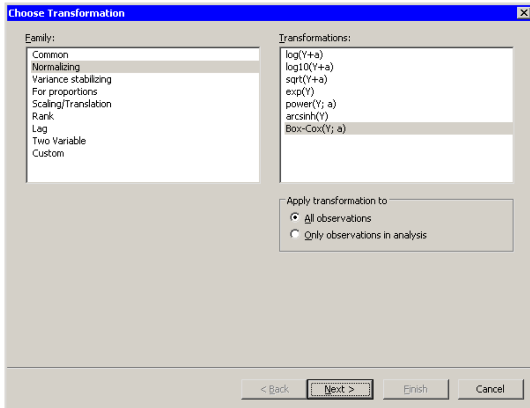
Figure 32.6 Selecting a Box-Cox Transformation
