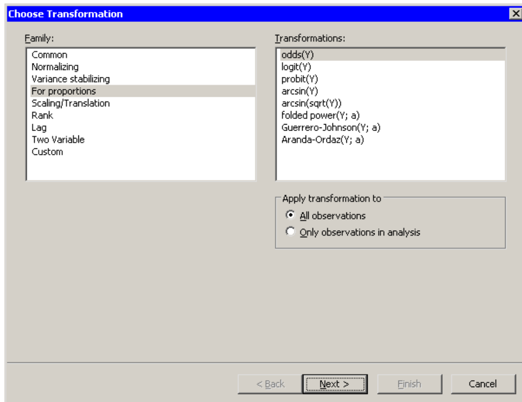
Figure 32.14 Transformations for Proportions
