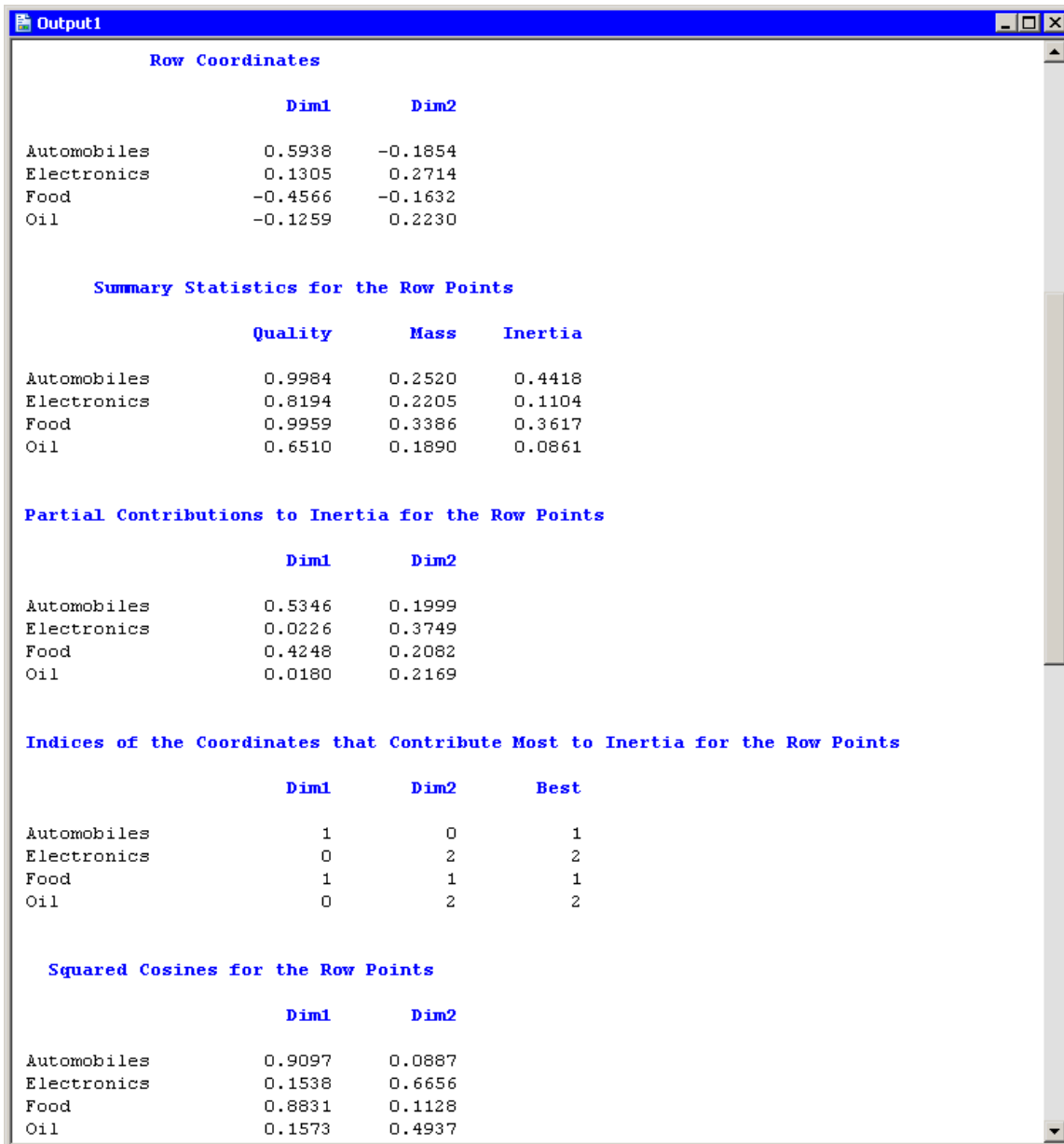
Figure 31.7 Output from a Correspondence Analysis
