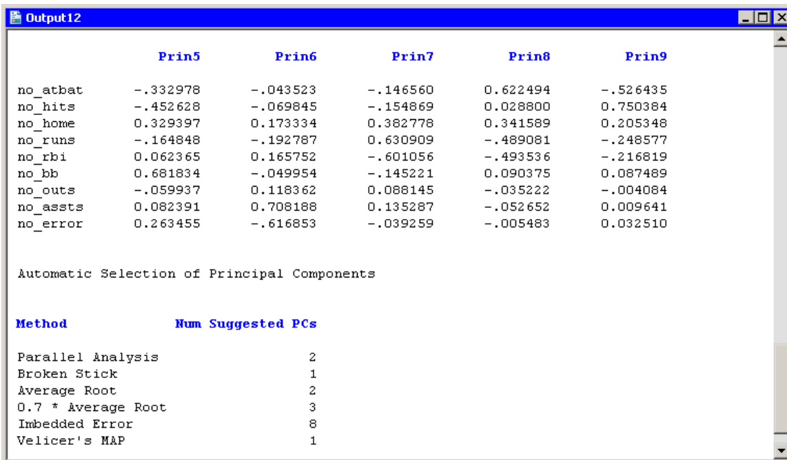
Figure 26.13 How Many Principal Components Are Needed?
