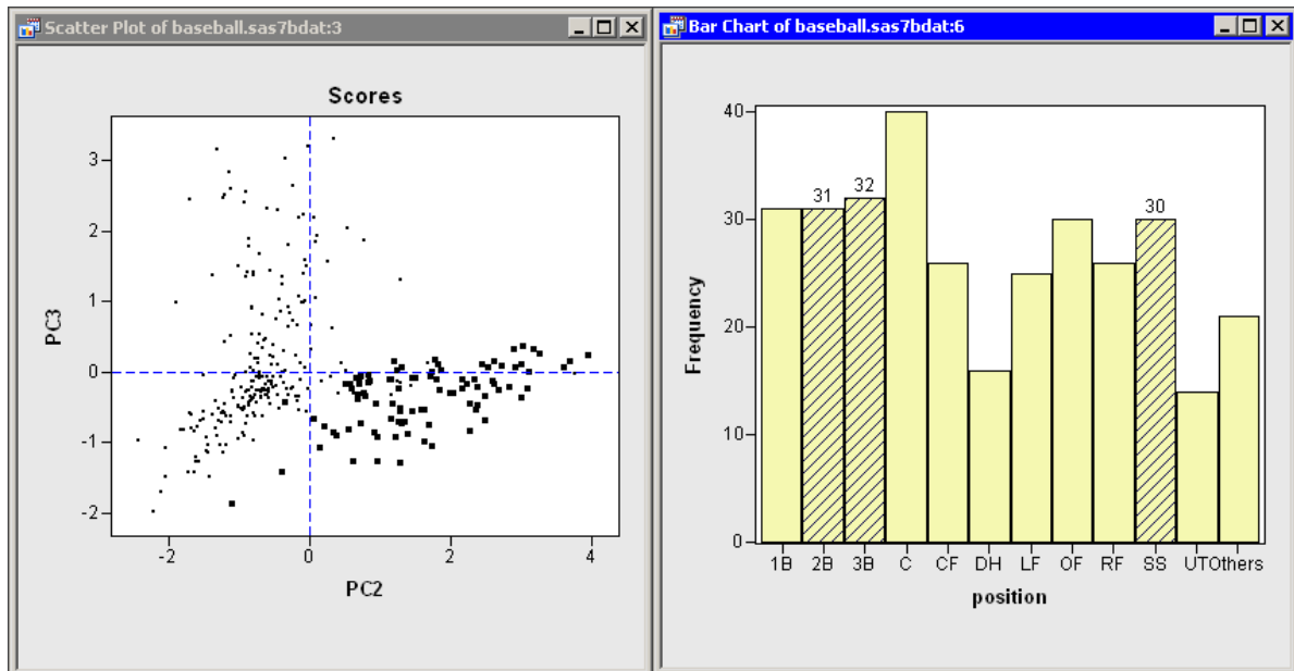
Figure 26.9 Fielding Scores for Some Infielders
