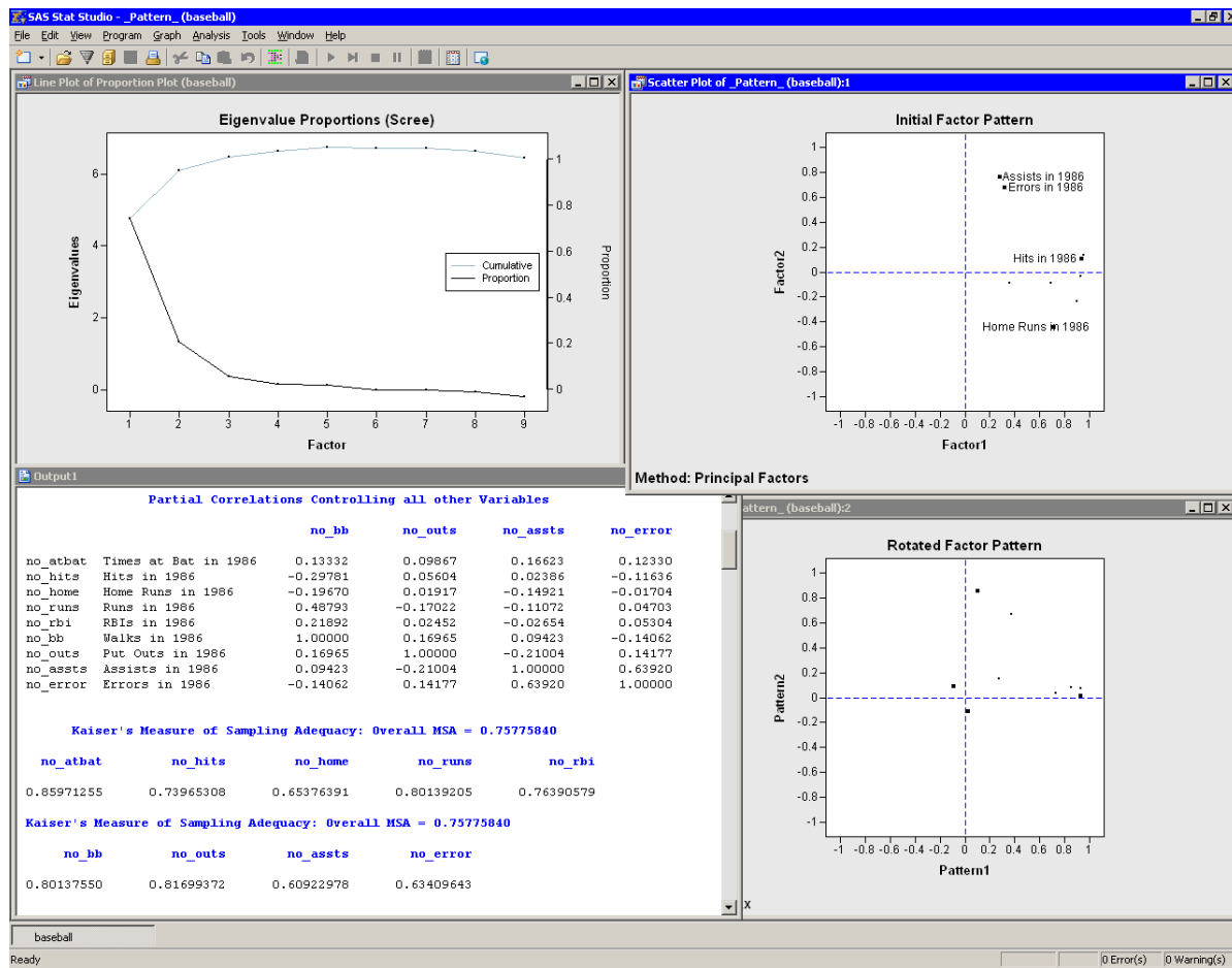
Figure 27.7 Output from a Common Factor Analysis
