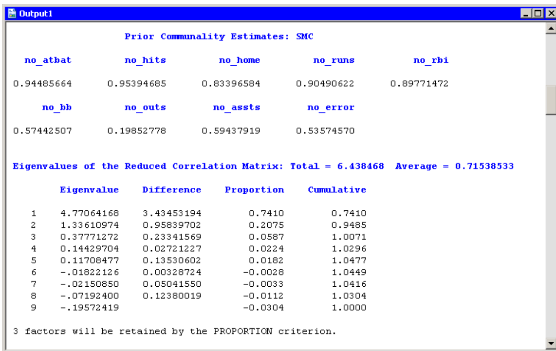
Figure 27.9 Output from a Common Factor Analysis
