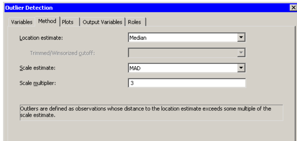
Figure 17.3 Specifying the Method
