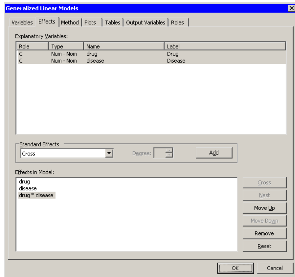
Figure 24.7 The Effects Tab
