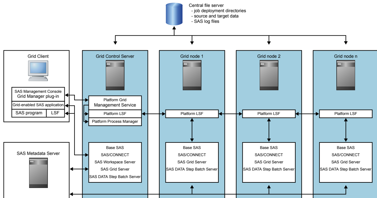
Figure 1.1 Grid Topology
