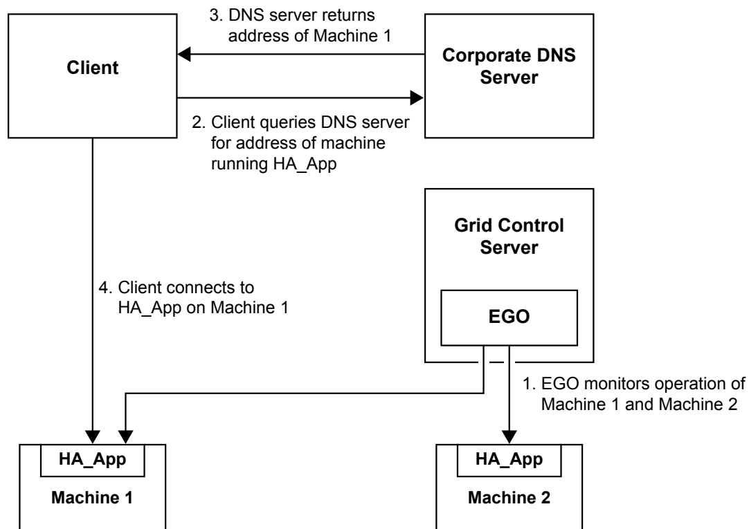
Figure 5.1 Normal Grid Operations
