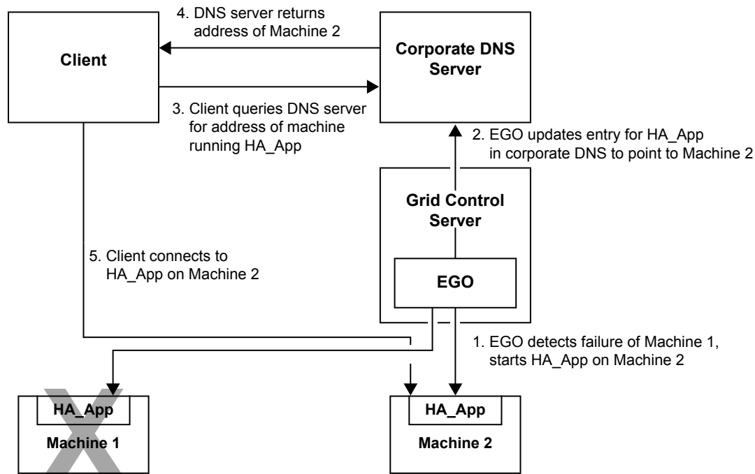
Figure 5.3 Grid Failover with EGO
